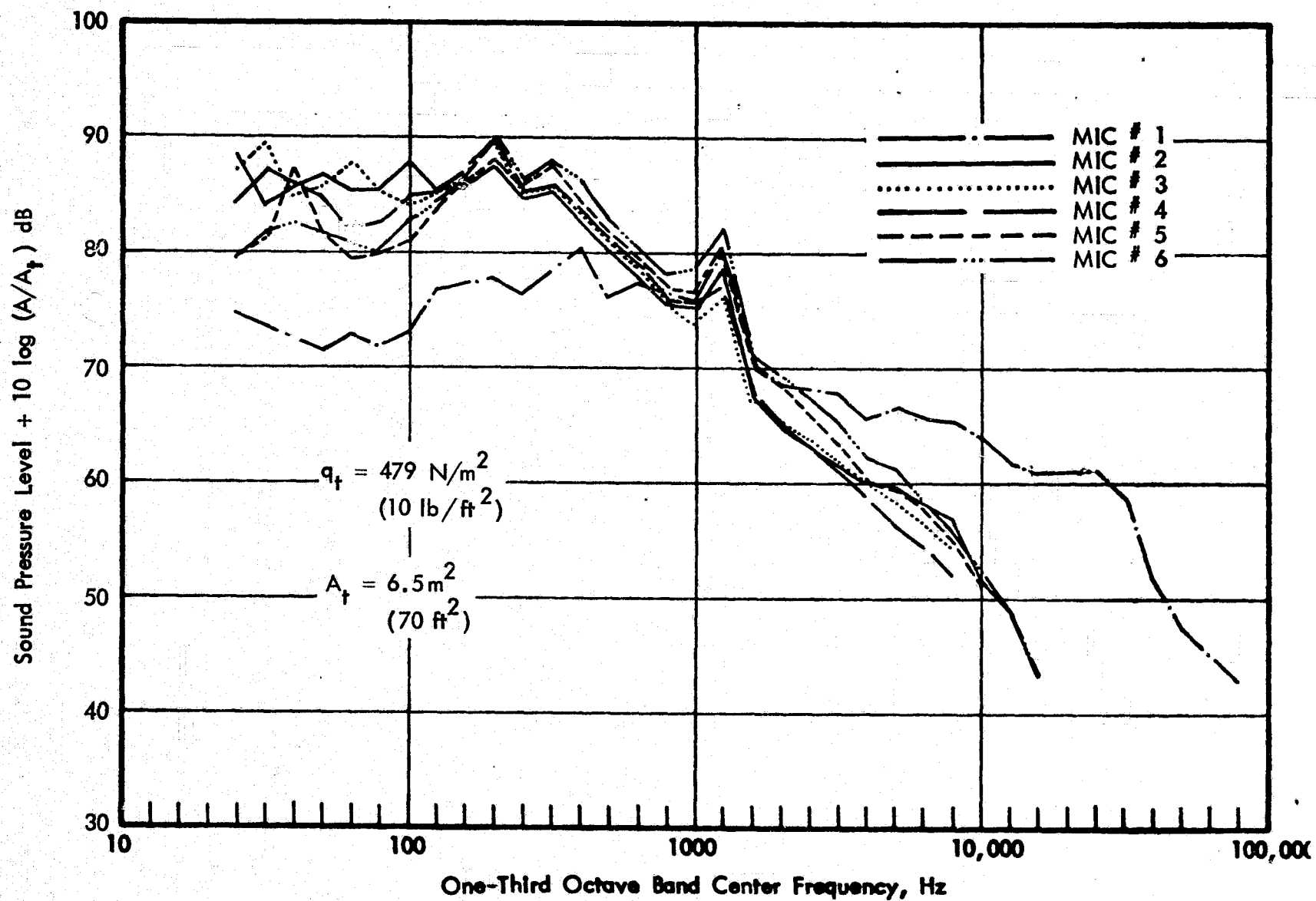
FIGURE 33. SOUND LEVELS NORMALIZED WITH RESPECT TO TUNNEL AREA (q_t = 479 \text{ N/m}^2)
