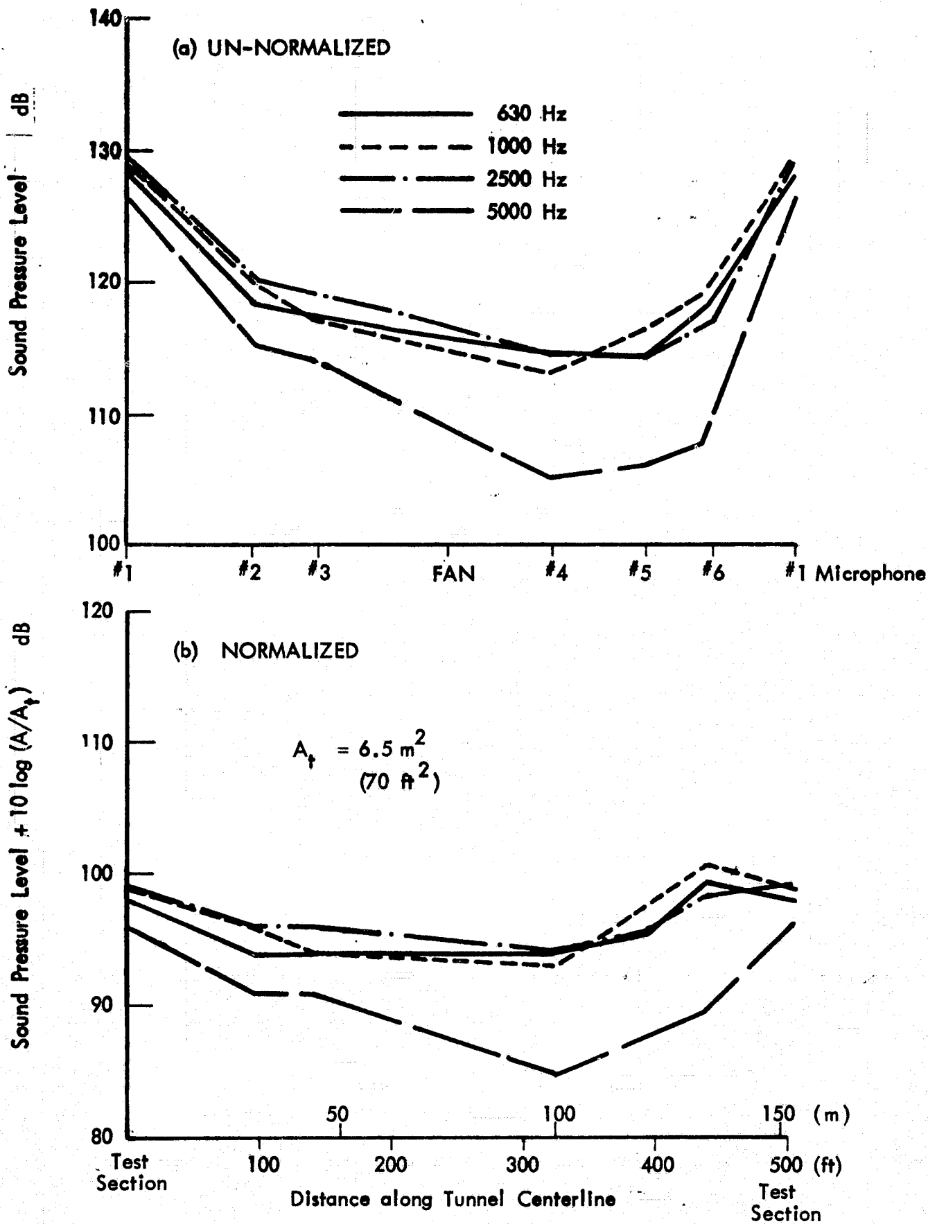
FIGURE 13. SPATIAL DISTRIBUTION OF SOUND LEVELS WITH SOURCE IN TEST SECTION
