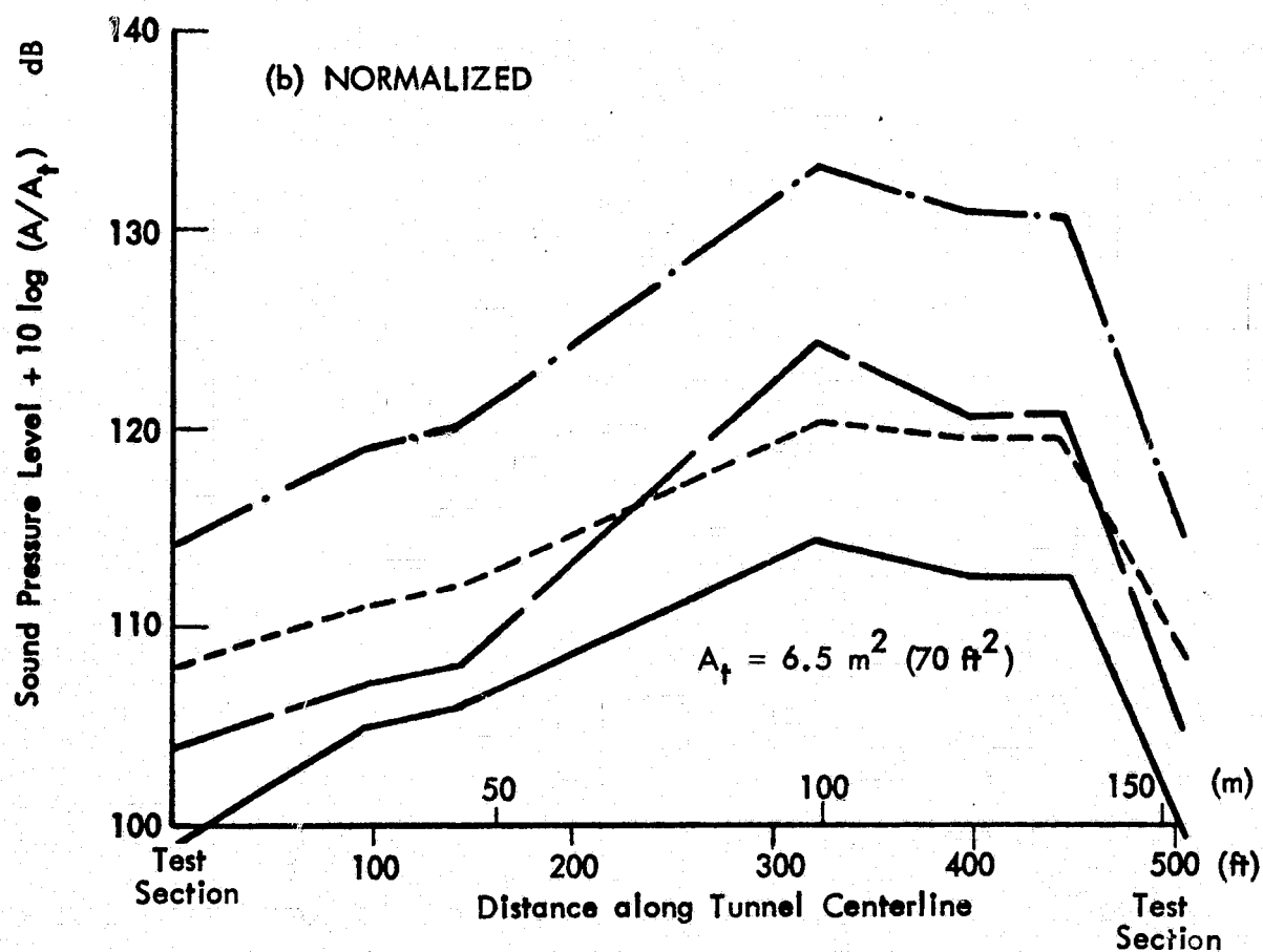
FIGURE 12. SPATIAL DISTRIBUTION OF SOUND LEVELS WITH SOURCE NEAR FAN
