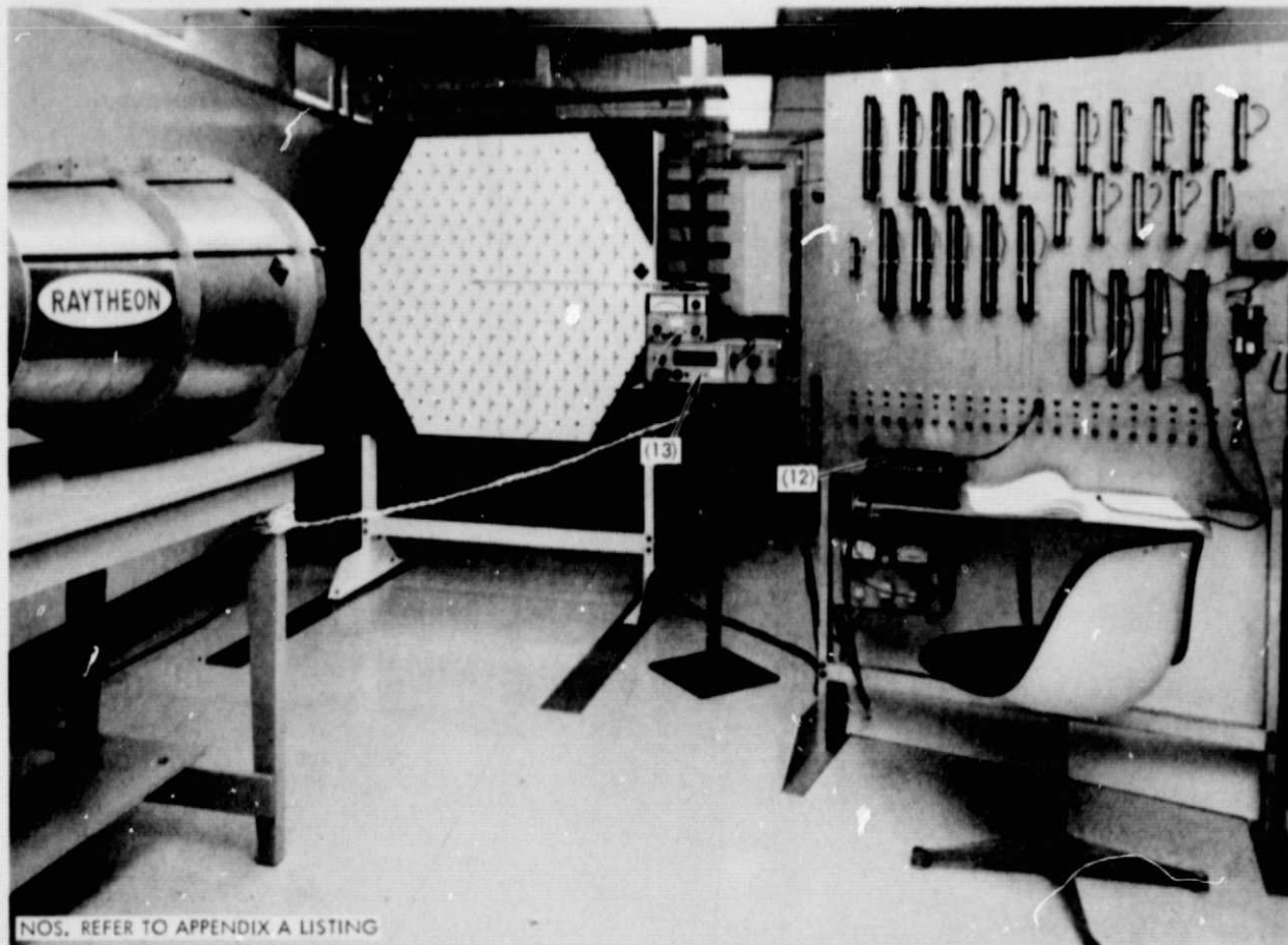
Fig. 7. Rectenna complex
