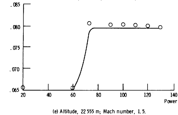
Figure 6. - Comparison of open-loop hybrid and baseline digital steady-state data for main-combustor pressure.
