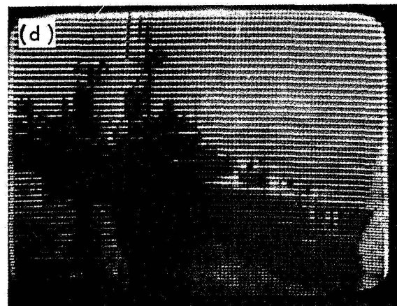
Figure 5. 100 x 100 CCD structure and image quality: (a) top view of the device; (b) cross-sectional view along a vertical transfer register; (c) pre-irradiation image; (d) image after 3 \times 10^4 rads
