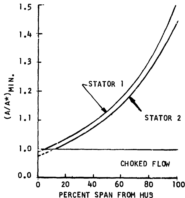
FIGURE 51. STATOR MINIMUM PASSAGE A/A^* DISTRIBUTION OF APPROACH FOR -20^\circ FIRST STATOR RESET ANGLE-- CONFIGURATION 3 RIG FLOW PATH
