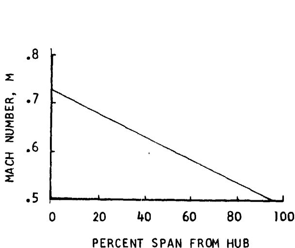
FIGURE 61. STATOR INLET MACH NUMBER DISTRIBUTION AT APPROACH--ENGINE FLOW PATH
