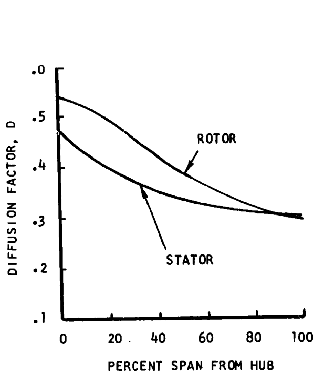
FIGURE 34. BLADE ROW DIFFUSION FACTOR DISTRIBUTIONS AT TAKEOFF--CONFIGURATION 1 RIG FLOW PATH
