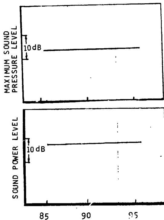
FIGURE 15. EFFECT OF INTERACTION ANGLE ON UPSTREAM PROPAGATED NOISE. SEARS COMPRESSIBLE MODEL
