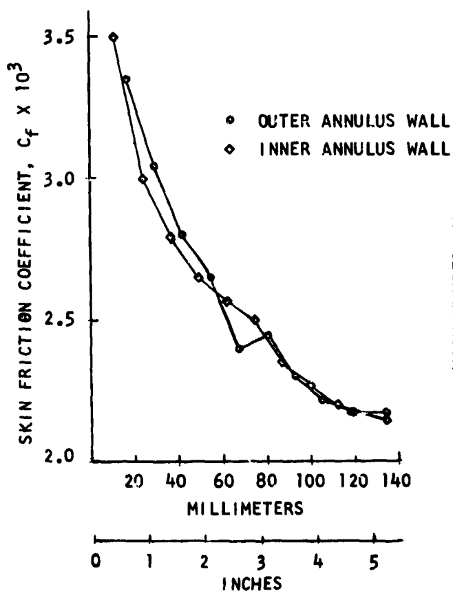
AXIAL DISTANCE FROM ROTOR TRAILING EDGE FIGURE 48. SKIN FRICTION COEFFICIENTS FOR INNER AND OUTER ANNULUS WALLS BETWEEN ROTOR AND STATOR AT TAKEOFF-- CONFIGURATION 3 RIG FLOW PATH
