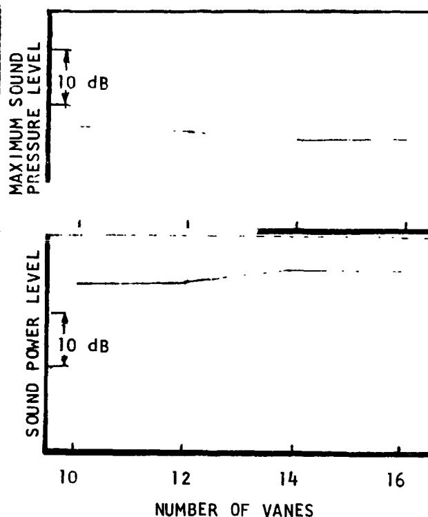
FIGURE 10. EFFECT OF VANE NUMBER ON DOWNSTREAM PROPAGATED DISCRETE NOISE, NAUMANN-YEH RESPONSE MODEL
