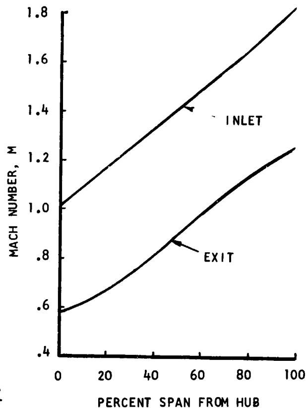
FIGURE 35. ROTOR INLET AND EXIT RELATIVE MACH NUMBER DISTRIBUTIONS AT TAKEOFF--CONFIGURATION 1 RIG FLOW PATH
