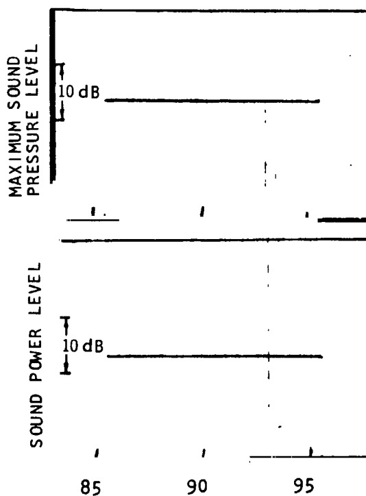
FIGURE 16. EFFECT OF INTERACTION ANGLE ON DOWNSTREAM PROPAGATED NOISE. SEARS COMPRESSIBLE MODEL
