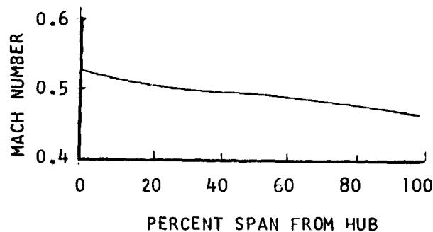
FIGURE 60. STATOR INLET MACH NUMBER DISTRIBUTION AT TAKEOFF--ENGINE FLOW PATH
