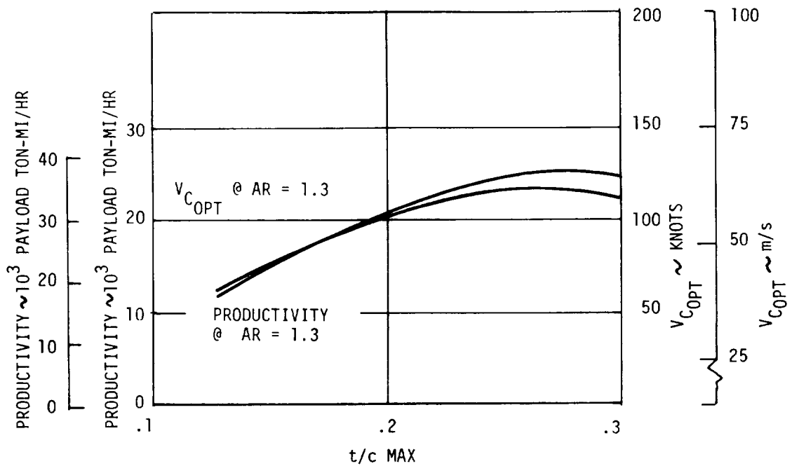
Figure 39 - Variation of Hybrid Vehicle Productivity with Aspect and Thickness Ratio ( \beta = 0.1 , GW = 1.5 \times 10^6 lb)
