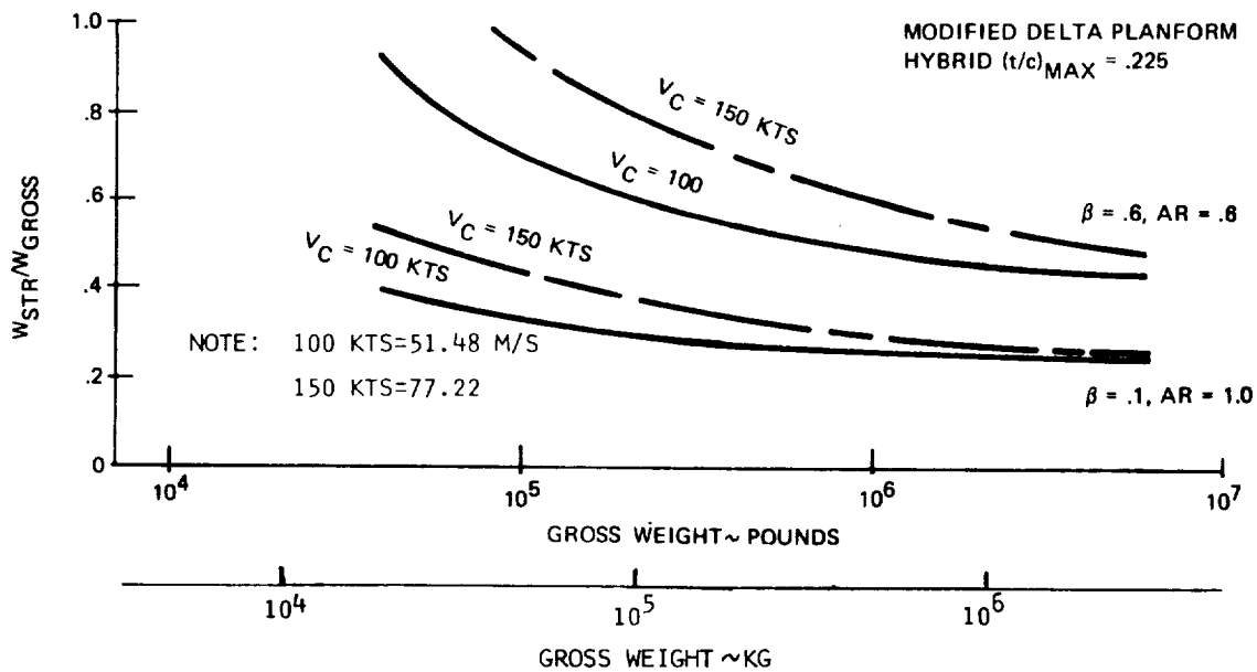
Figure 51 - Representative Structural Efficiency Characteristics of Lifting Body Hybrid
