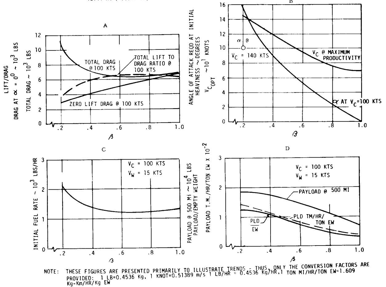
Figure 31 - Resulting Vehicle Performance/Productivity as a Function of \beta
