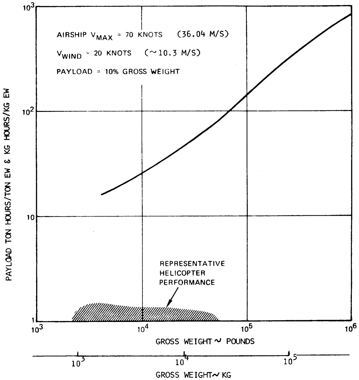
Figure 56 - Typical Endurance Capability of Neutrally Buoyant Airships
