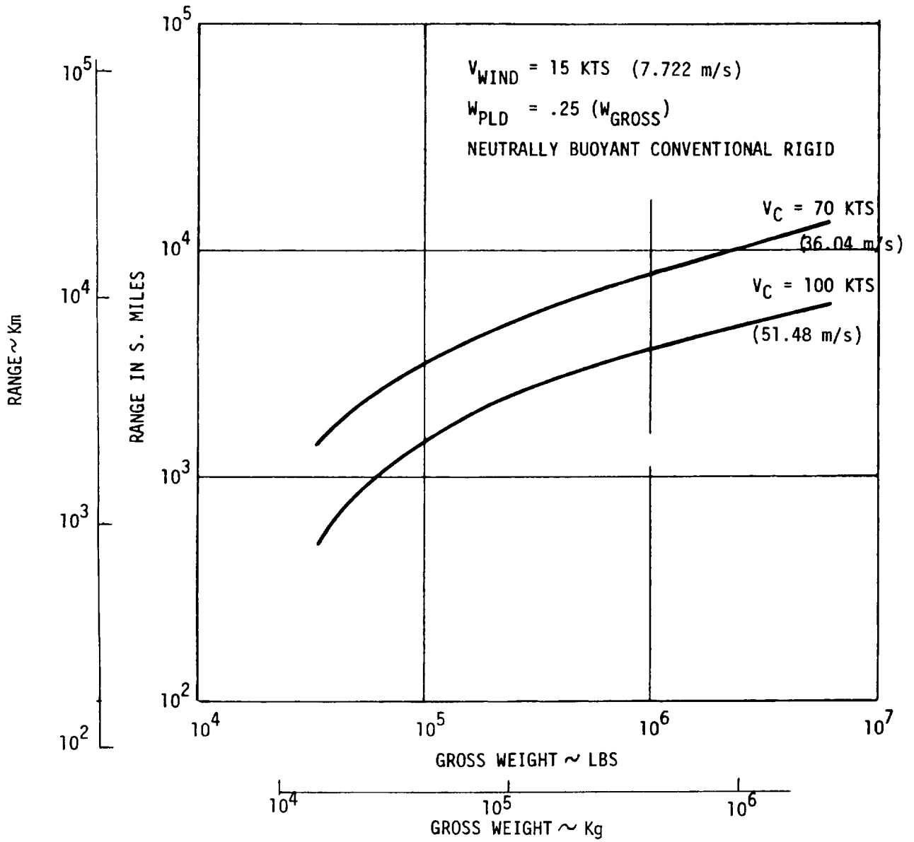
Figure 57 - Representative Payload-Range Capability of Conventional Neutrally Buoyant Airships
