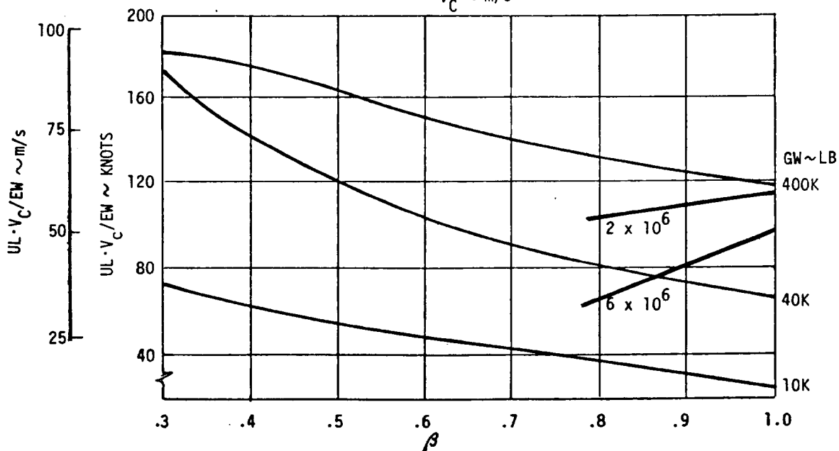
Figure 16 - Conventional Rigid Heaviness Trade Study Results Based on UL \cdot V_C / EW
