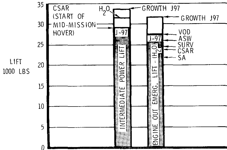
Figure 16. Hover and VTOL Operation Lift Capabilities
