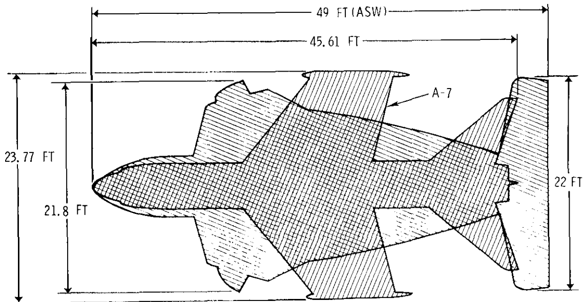
Figure 6. Multi-Mission Aircraft Spotting Comparison With A-7
