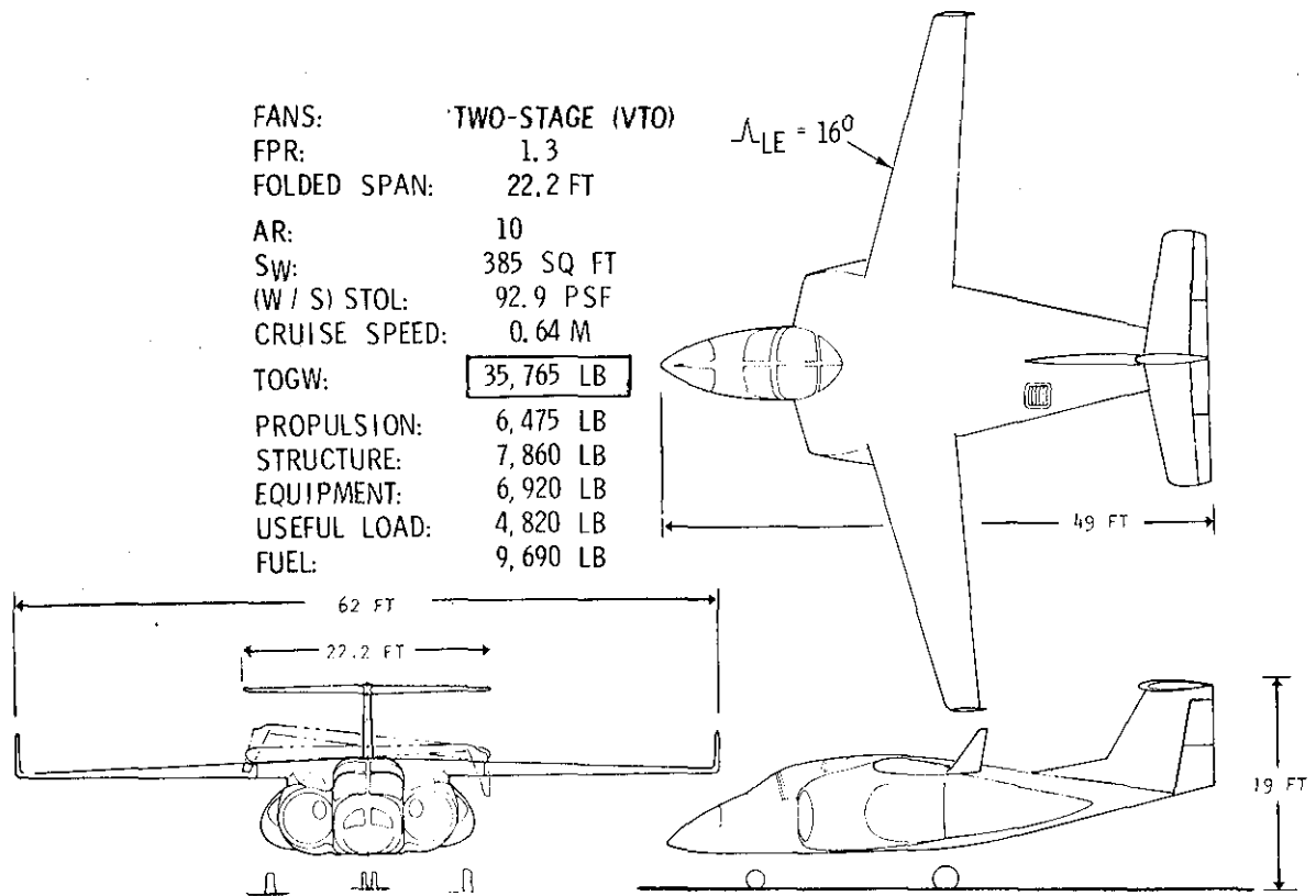
Figure 28. Optimized ASW Aircraft Design Brief
