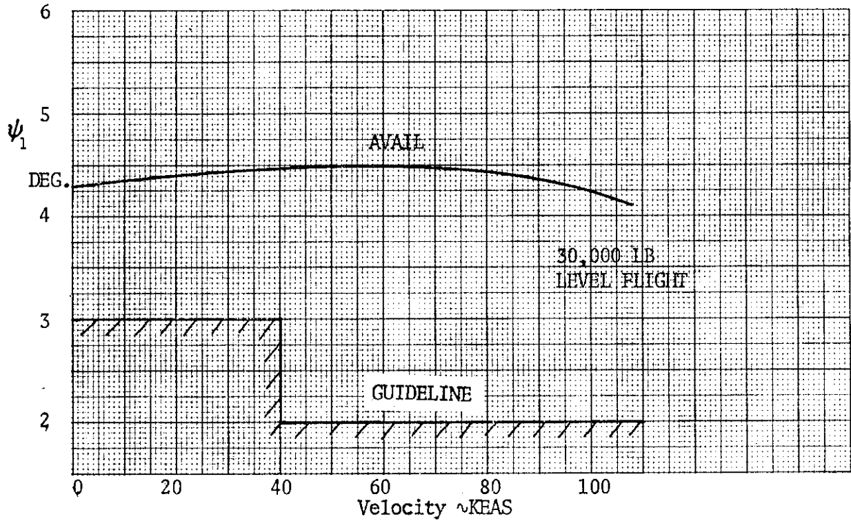
Figure 26. Emergency Yaw Attitude Angle Attained in One Second
