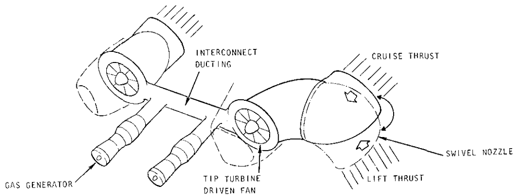
Figure 14. Basic Lift-Cruise Fan System Installation
