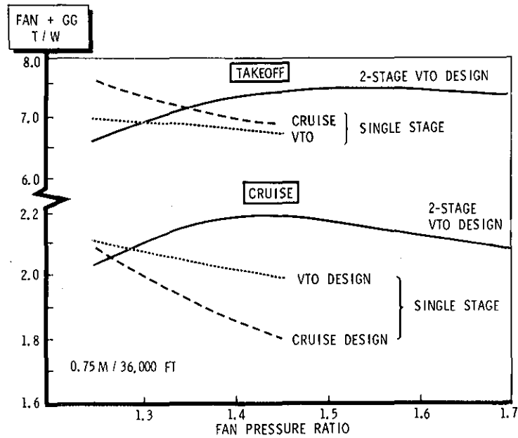
Figure 39. Takeoff and Cruise Thrust to Weight Ratio Characteristics of Lift-Cruise Fan Systems
