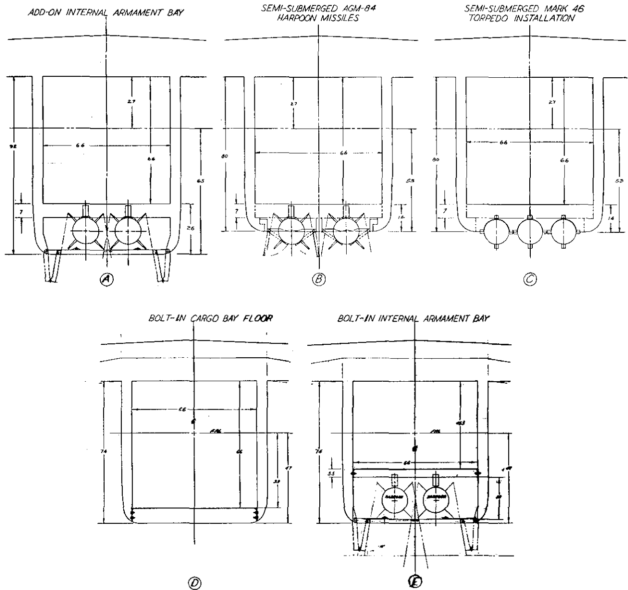
Figure 45. Candidate Fuselage Cross-Section Designs
