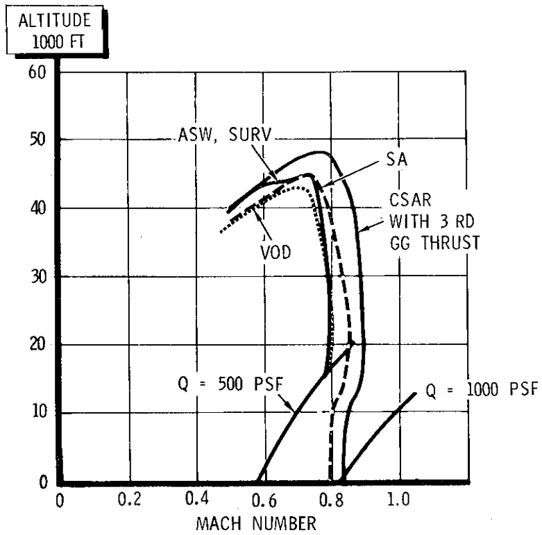
Figure 12. Multi-Mission Aircraft Speed-Altitude Capability
