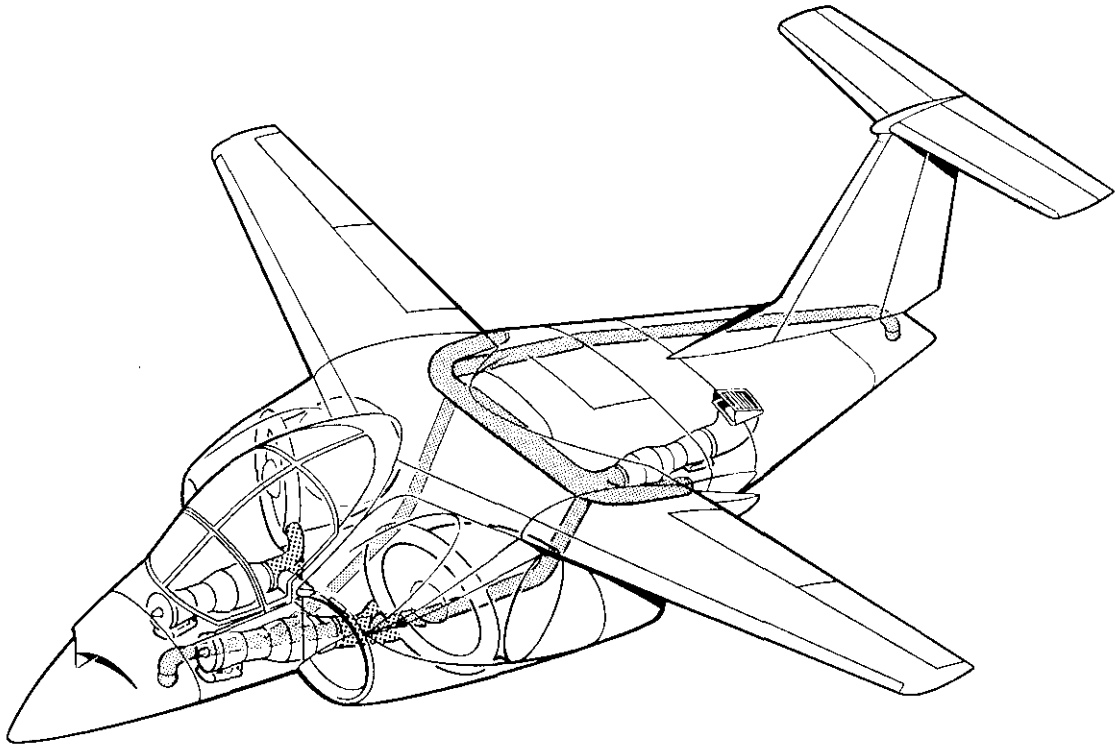
Figure 15. Complete Propulsion/Hover Control System Installation
