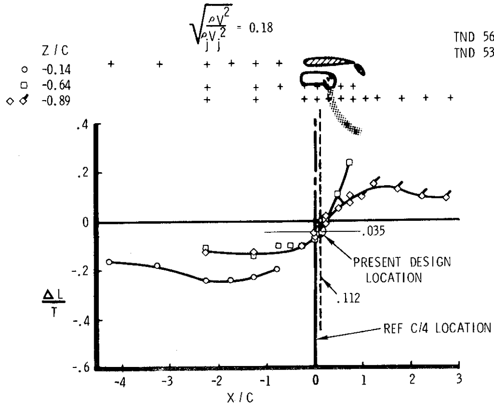
Figure 20. Low Speed Propulsion/Aerodynamic Interaction Characteristics
