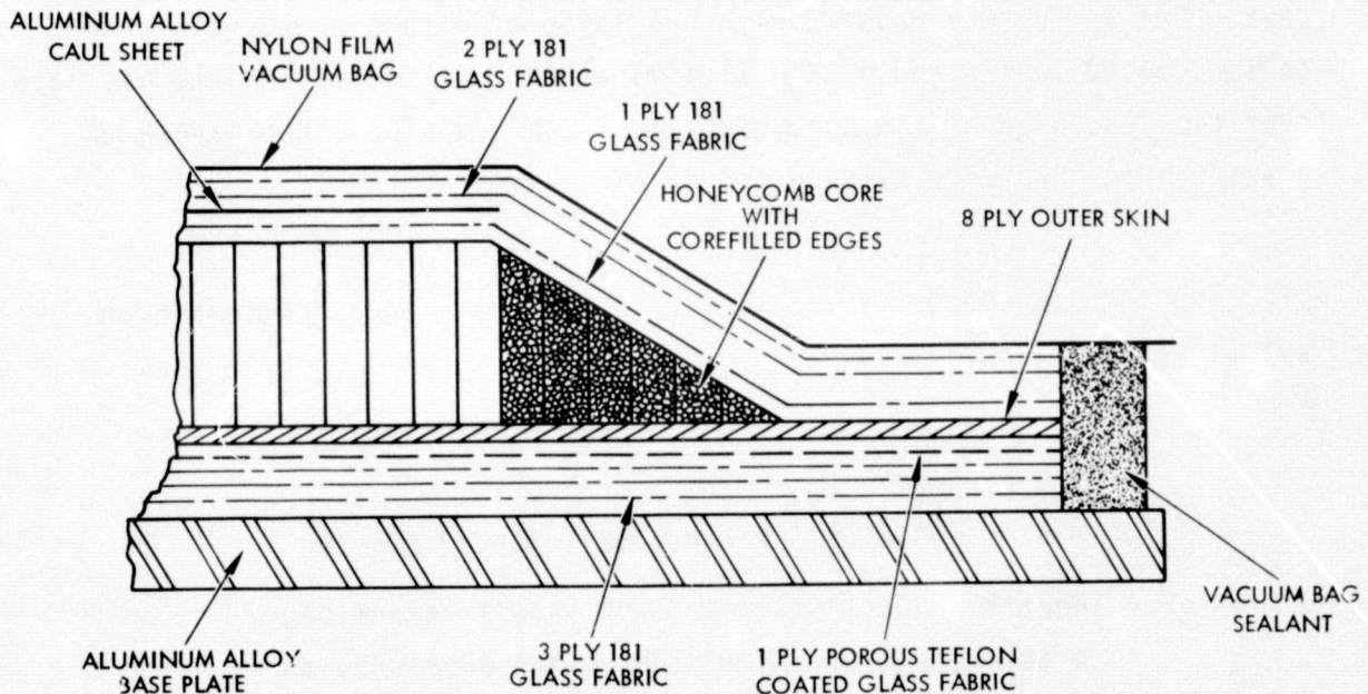
Figure 7. Outer Skin Lay-up
