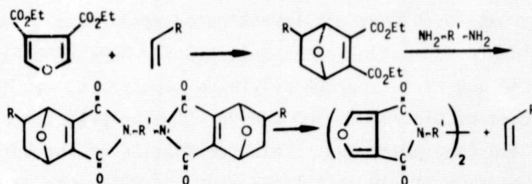
Equation 3.
