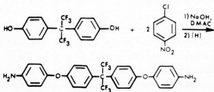
Equation 2.
