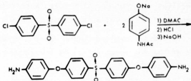
Equation 1
