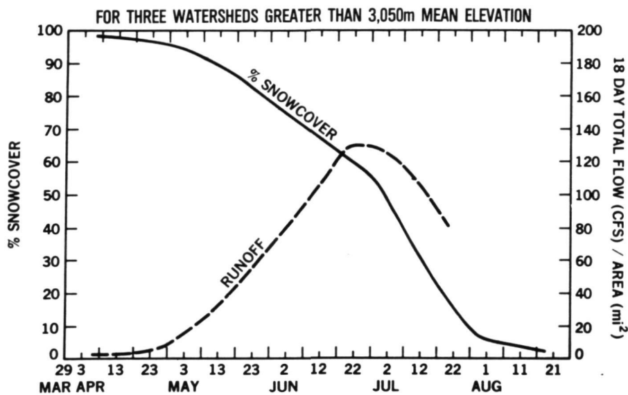
Fig. 6—1973 average snowcover depletion and runoff curves for the Wind River Mountains, separated on the basis of mean elevation. Snowcover area obtained from LANDSAT-1 0.6-0.7 \mu m observations.
