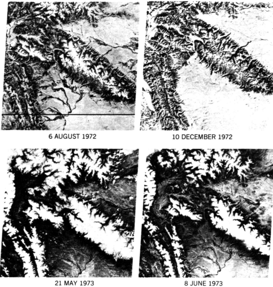
Fig. 4—Snowcover changes in northwestern Wyoming, 1972-1973.
