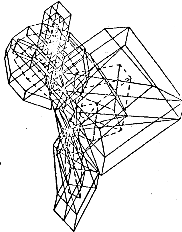
Figure 5.- Total model NASTRAN type bulk data and resistance network.
