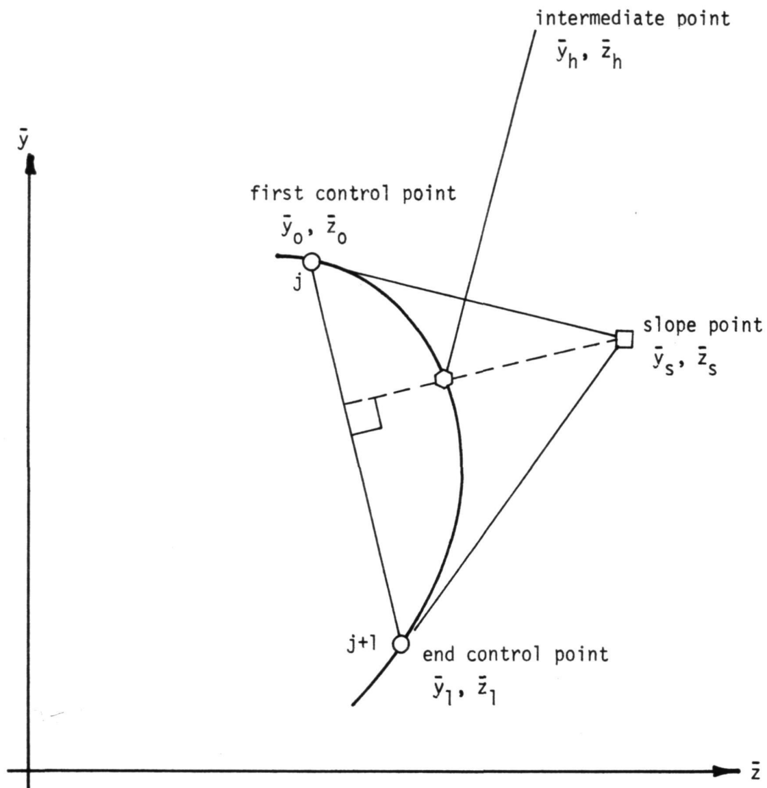
Figure 6. Four points used to define a segment of a conic section.
