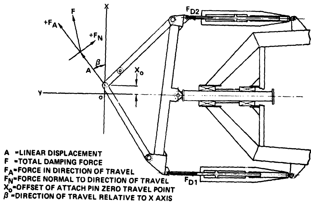
Figure 4. Damper force response to attach pin displacement.
