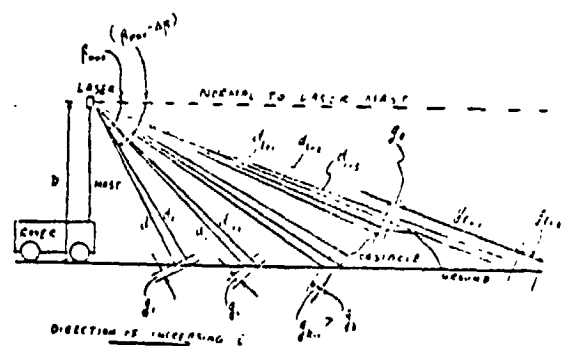
Figure 1 - Side View of Rover and Terrain
