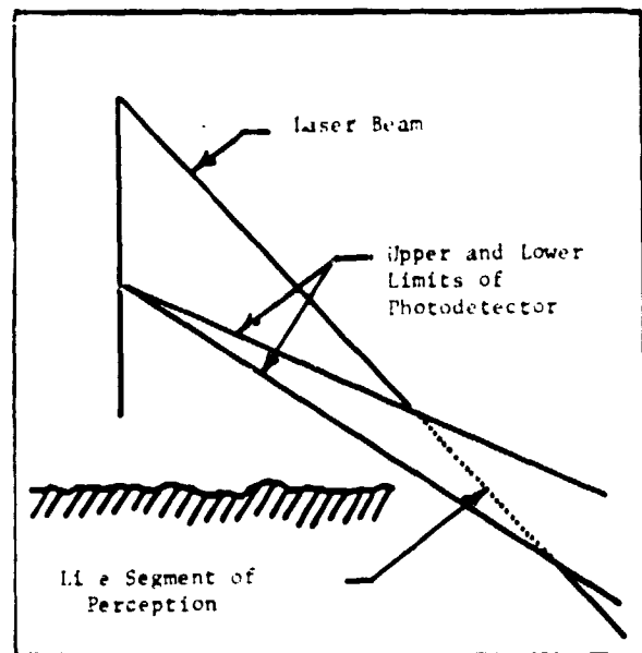
Figure 3 Terrain Detection by Triangulation
