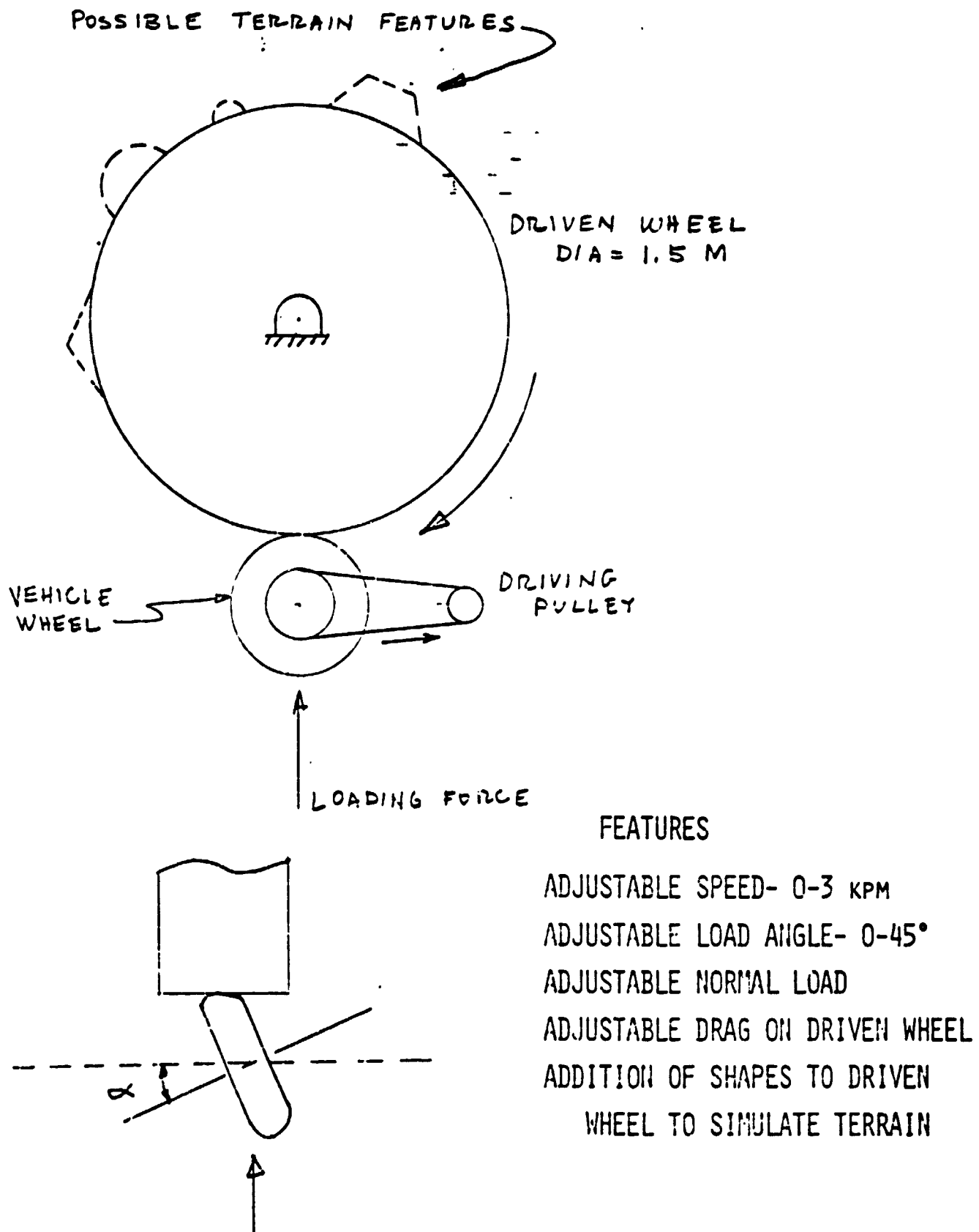
FIGURE 2. Wheel Fatigue and Dynamic Load Tester Details
