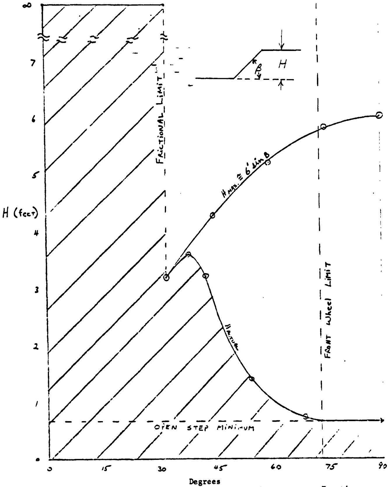
FIGURE 12. Height of Closed Step Which Can Be Overcome as a Function of the Slope in the Step
