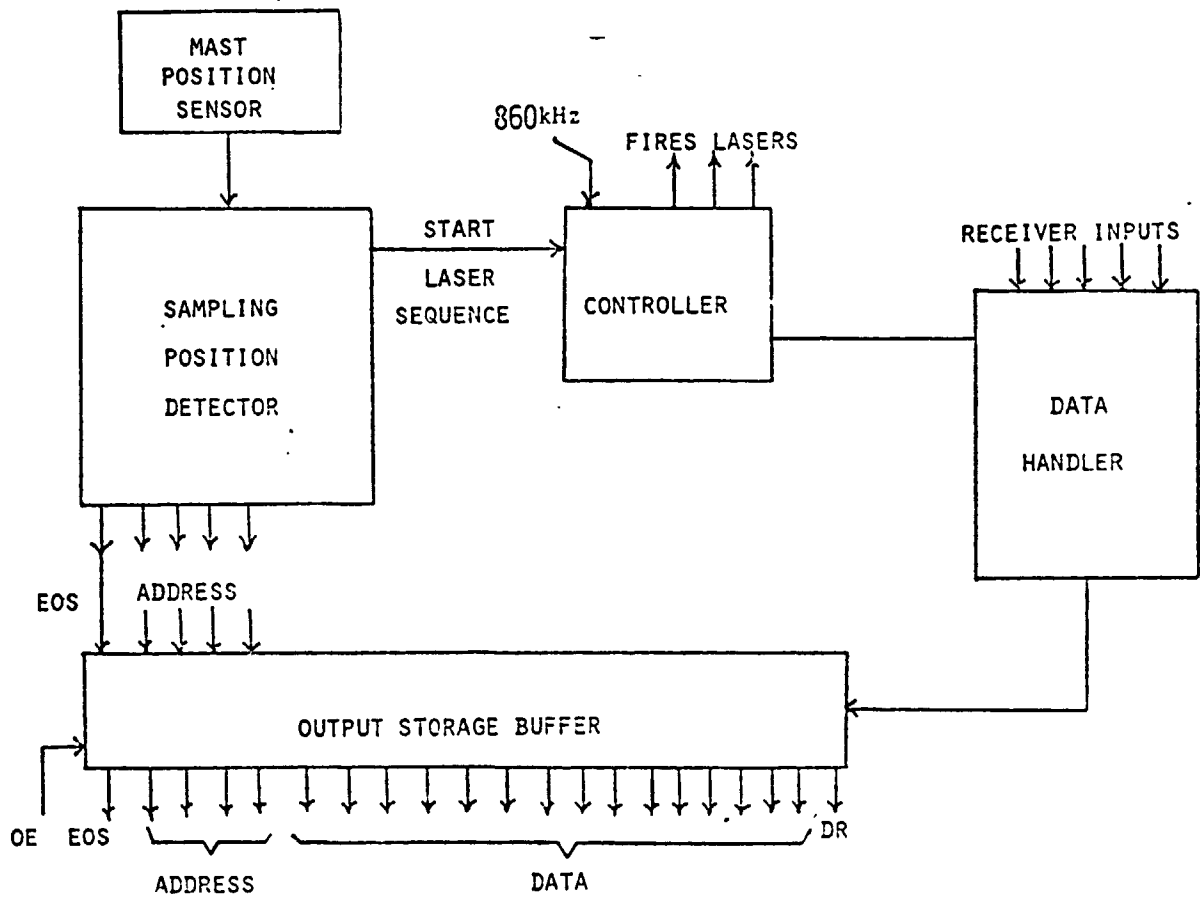
FIGURE 25. DATA HANDLER/CONTROLLER
