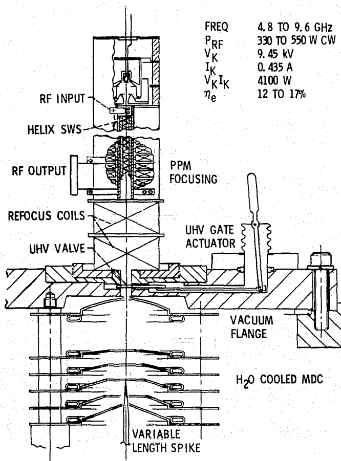
Figure 8. - MEC TWT typ. no. M5897C schematic.
