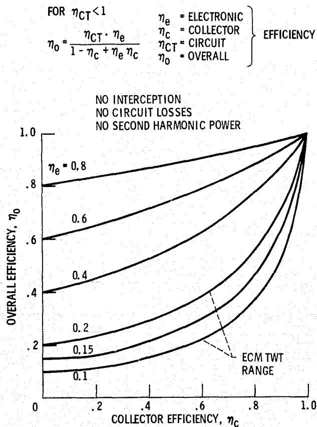
Figure 7(a). - Overall efficiency vs. collector efficiency.
