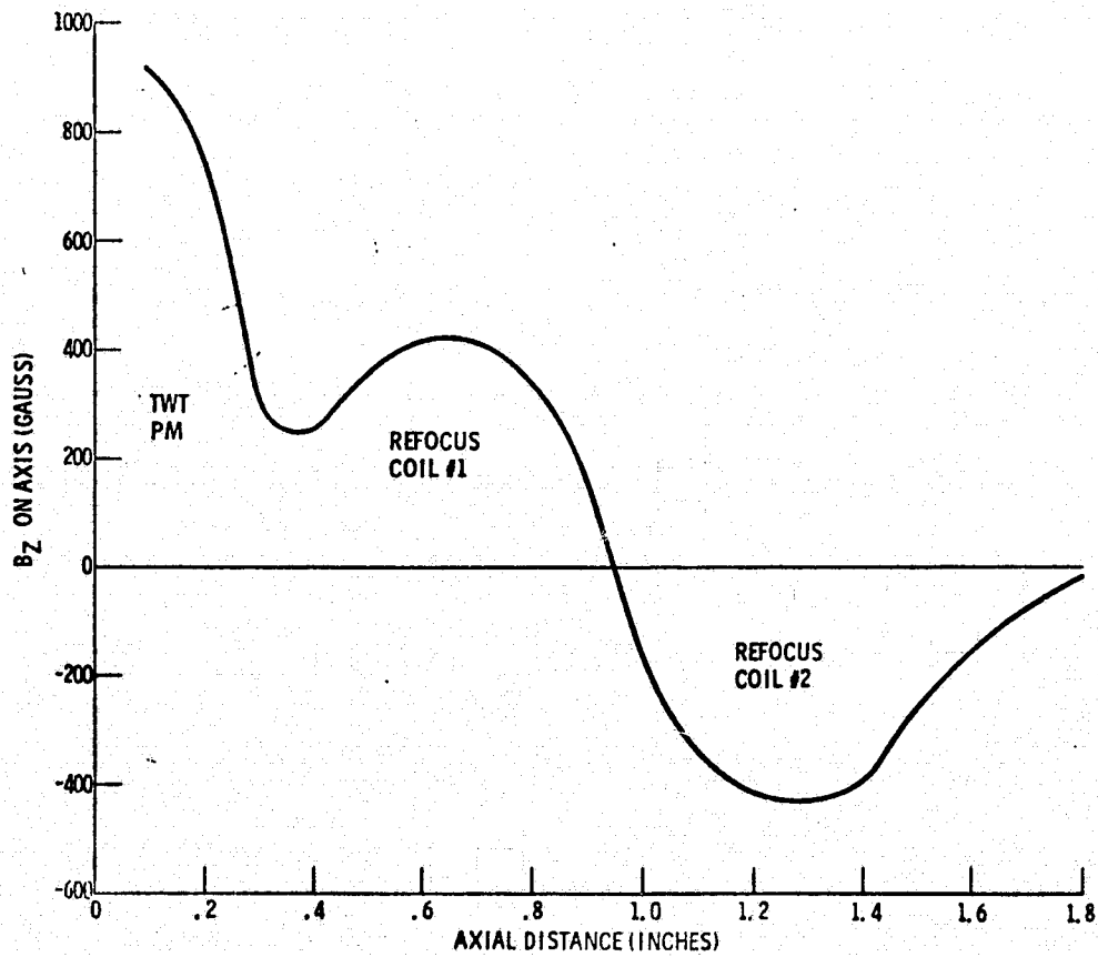
Typical refocusing field profile B_z on axis vs. Z .
