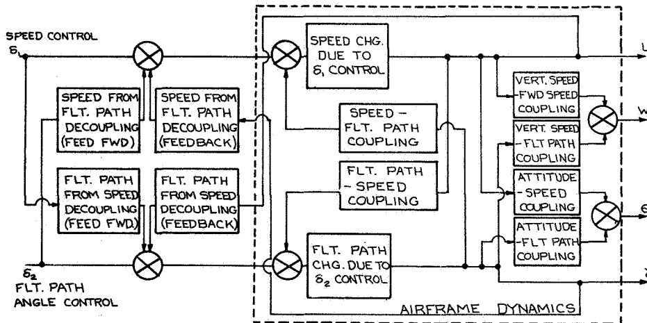
FIG. 4 DECOUPLED-LONGITUDINAL CONTROL
