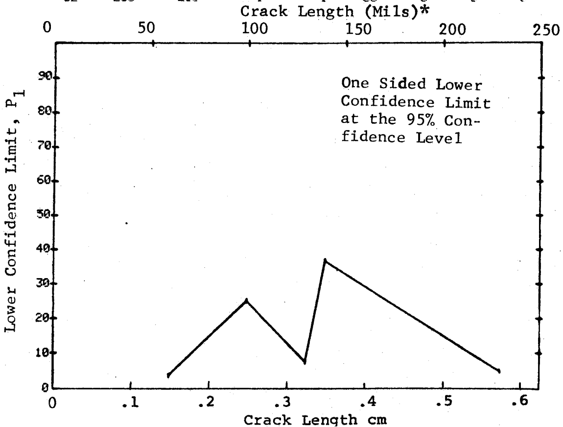
Figure D-68 Probability of Detection for 4340M Steel Using Liquid Penetrant. Compressed Notch Flaws in Filleted Hollow Cylinder. Lab. Env.
