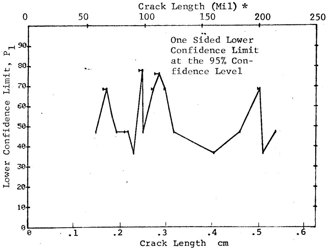
Figure D-46 Probability of Detection for PH17-4 Steel Using Ultrasonic Shear Wave. Simulated Flaws in Wrought Steel. Prod. Env.
