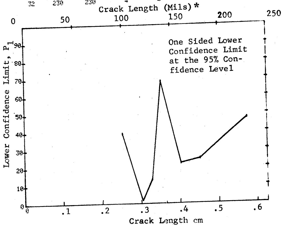
Figure D-112 Probability of Detection for 4340M Steel Using Eddy Current. Compressed Notch Flaws in Hollow Cylinder. Laboratory Environment.
