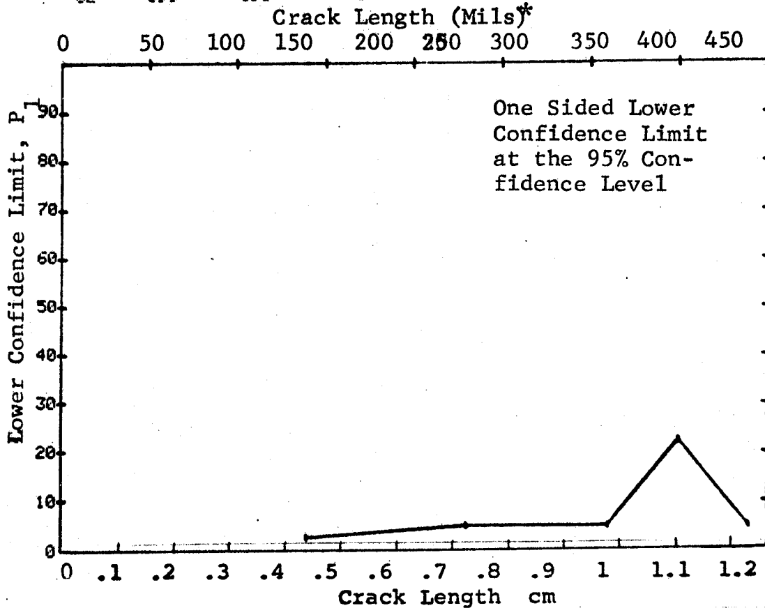
Figure D-91 Probability of Detection for 4340M Steel Using X-ray. Compressed Notch Flaws in Hollow Filleted Cylinder. Lab. Inv.
