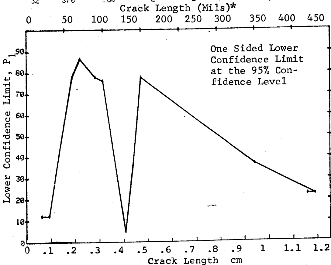
Figure D-75 Probability of Detection for 4340M Steel Using Ultrasonic Shear and Surface Waves. Compressed Notch Flaws in Filleted Solid Cylinder. Prod Env. D-231
