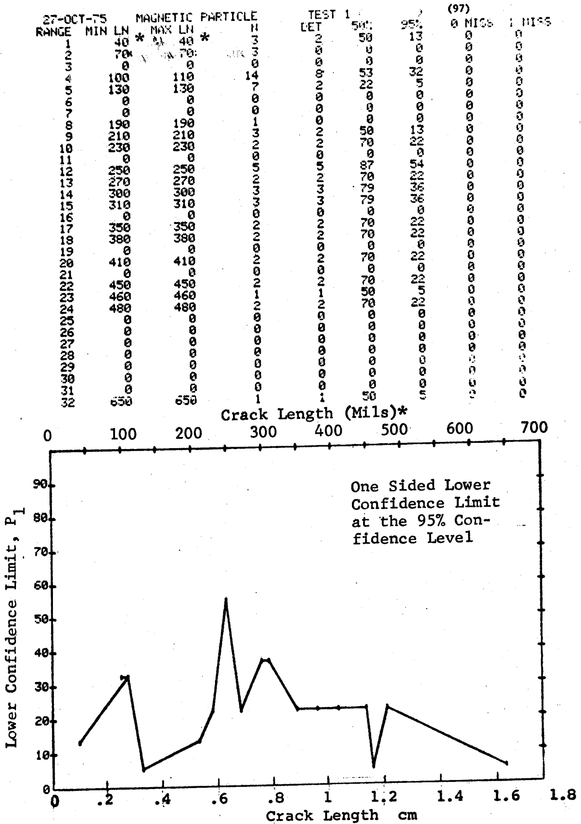
Figure D-97 Probability of Detection for 4340M Steel Using Magnetic Particles. Compressed Notch Flaws in Solid Threaded Cylinder. Prod. Env. D-297
