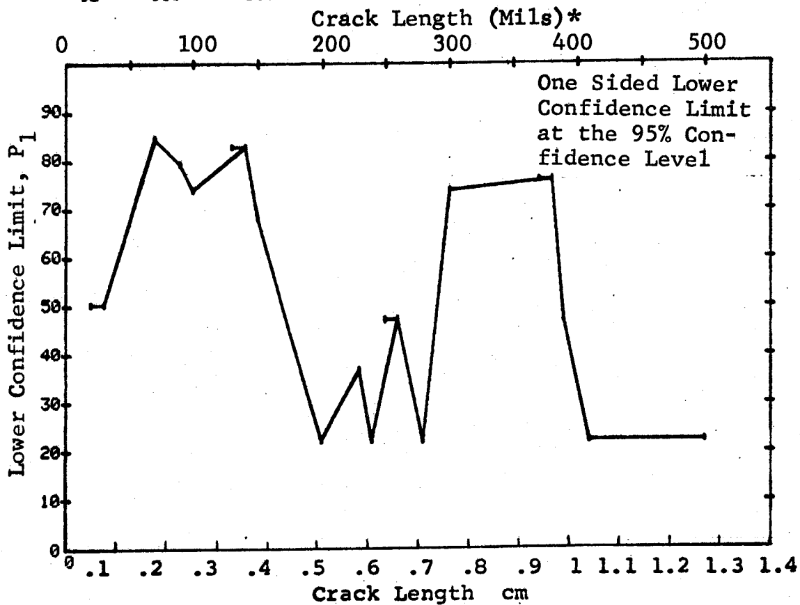
Figure D-101 Probability of Detection for 4340M Steel Using Magnetic Particles. Compressed Notch Flaws in Solid Filleted Cylinder. Lab. Env.
