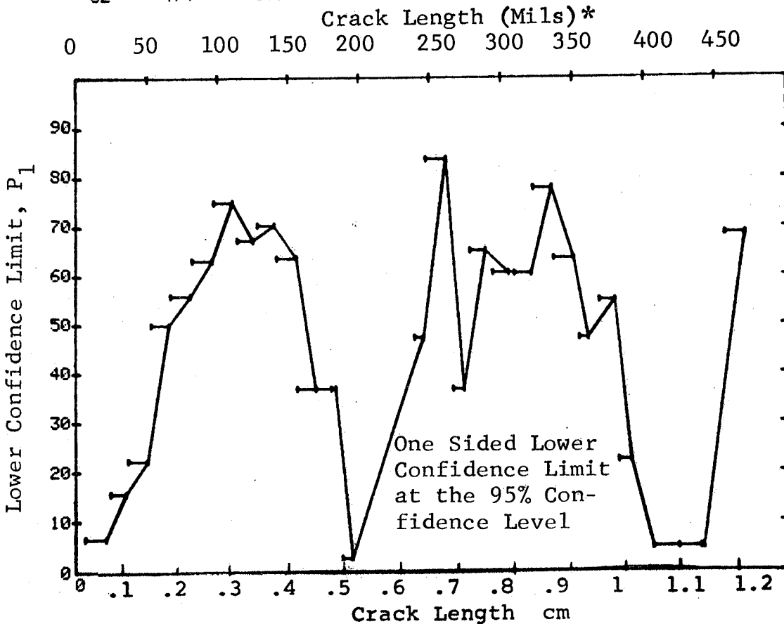
Figure D-16 Probability of Detection for 2219-T87 Al Using Liquid Penetrant. Etched Fatigue Cracks in Flat Plates Measured by Operator J D-48 Lab. Env.
