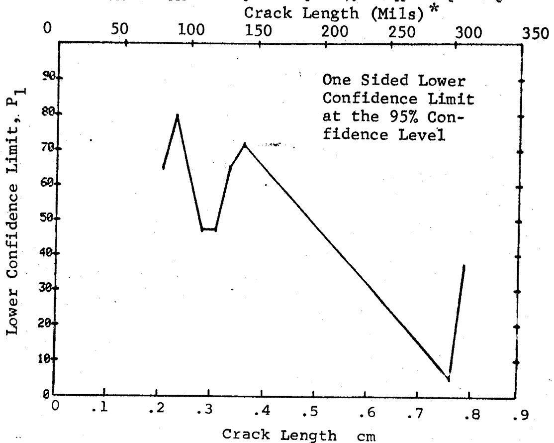
Figure D-80 Probability of Detection for 4340M Steel Using Ultrasonic Shear and Surface Waves. Compressed Notch Flaws in Filleted Hollow Cylinder. Lab. Env.
