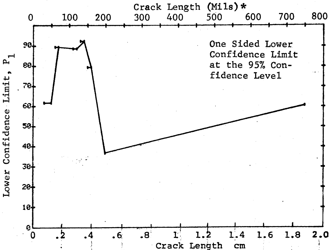
Figure D-98 Probability of Detection for 4340M Steel Using Magnetic Particles. Compressed Notch Flaws in Solid Cylinder. Lab. Env.
