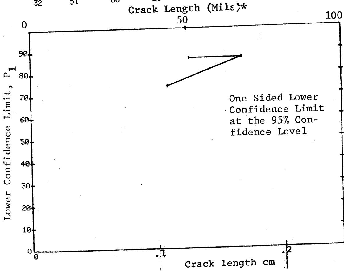
Figure D-41 Probability of Detection for 7075-T6511 Al Using Liquid Penetrant. Fatigue Cracks in Flat Plates. Prod. Env. D-127
