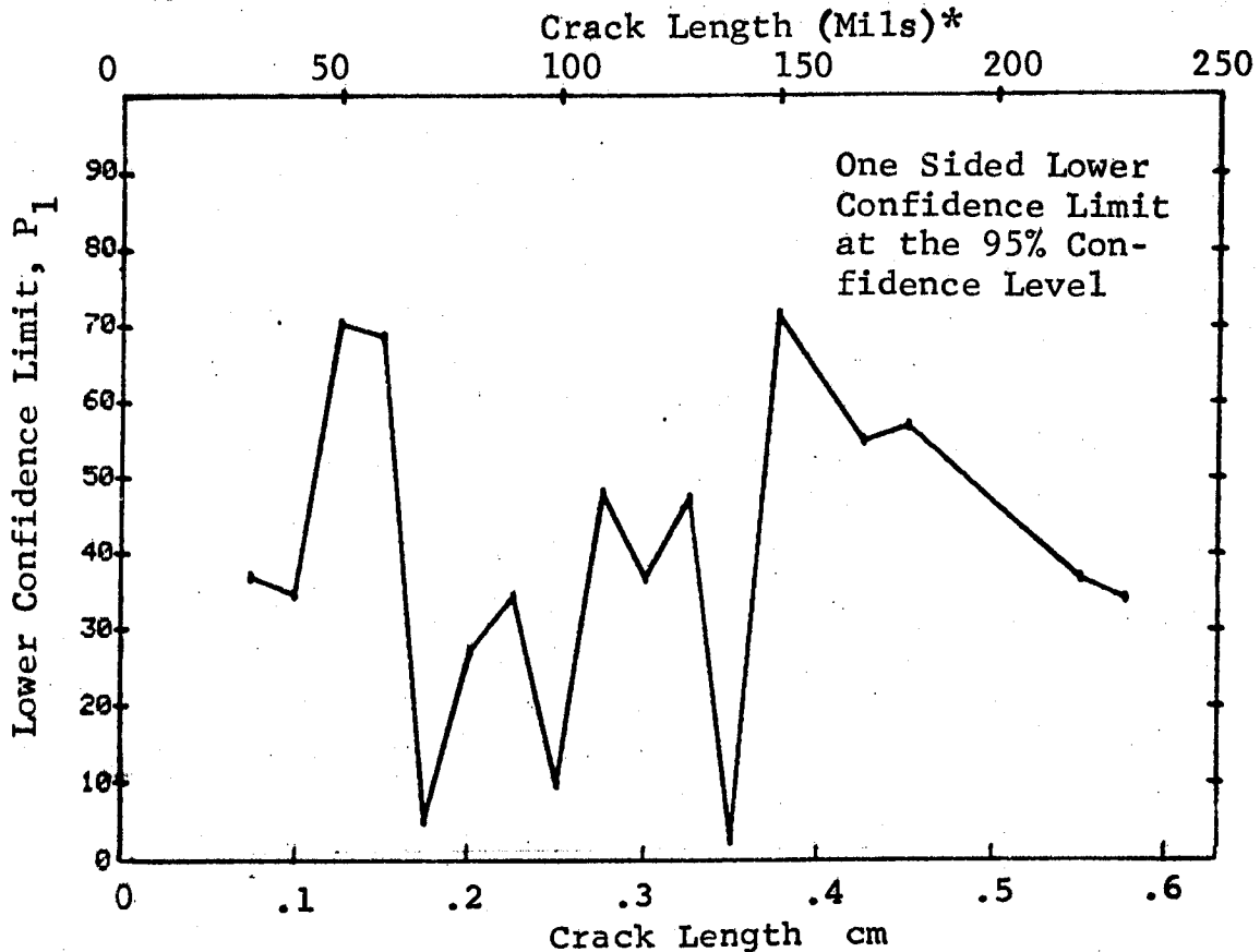
Figure D-87 Probability of Detection for 2024-T6 Al Using X-ray. Compressed Notch Flaws in Tandem-T Specimen. Prod. Env.
