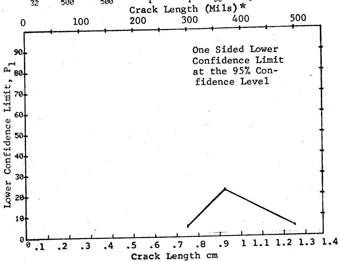
Figure D-83 Probability of Detection for 4340M Steel Using X-ray. Compressed Notch Flaws in Filleted Solid Cylinder. D-255 Prod. Env.
