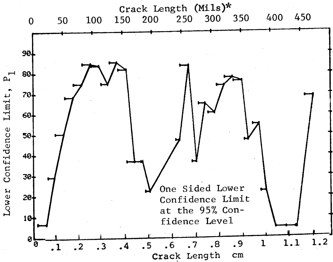
Figure D-17 Probability of Detection for 2219-T8/ Al Using Liquid Penetrant. Etched Fatigue Cracks in Flat Plates Measured by Operator K Lab. Env.
