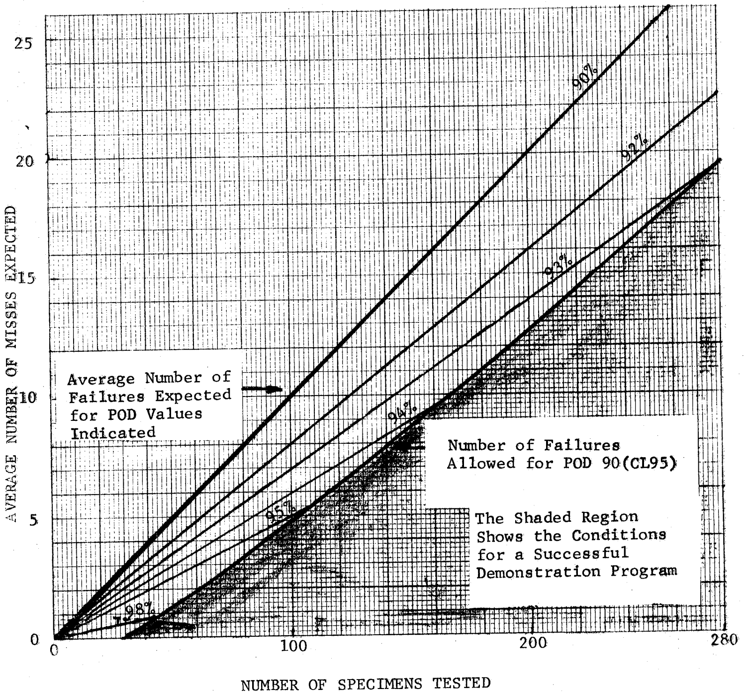
Figure 6-2 Conditions for Success in Selecting a Sample Size that will Potentially Demonstrate POD90(CL95)
