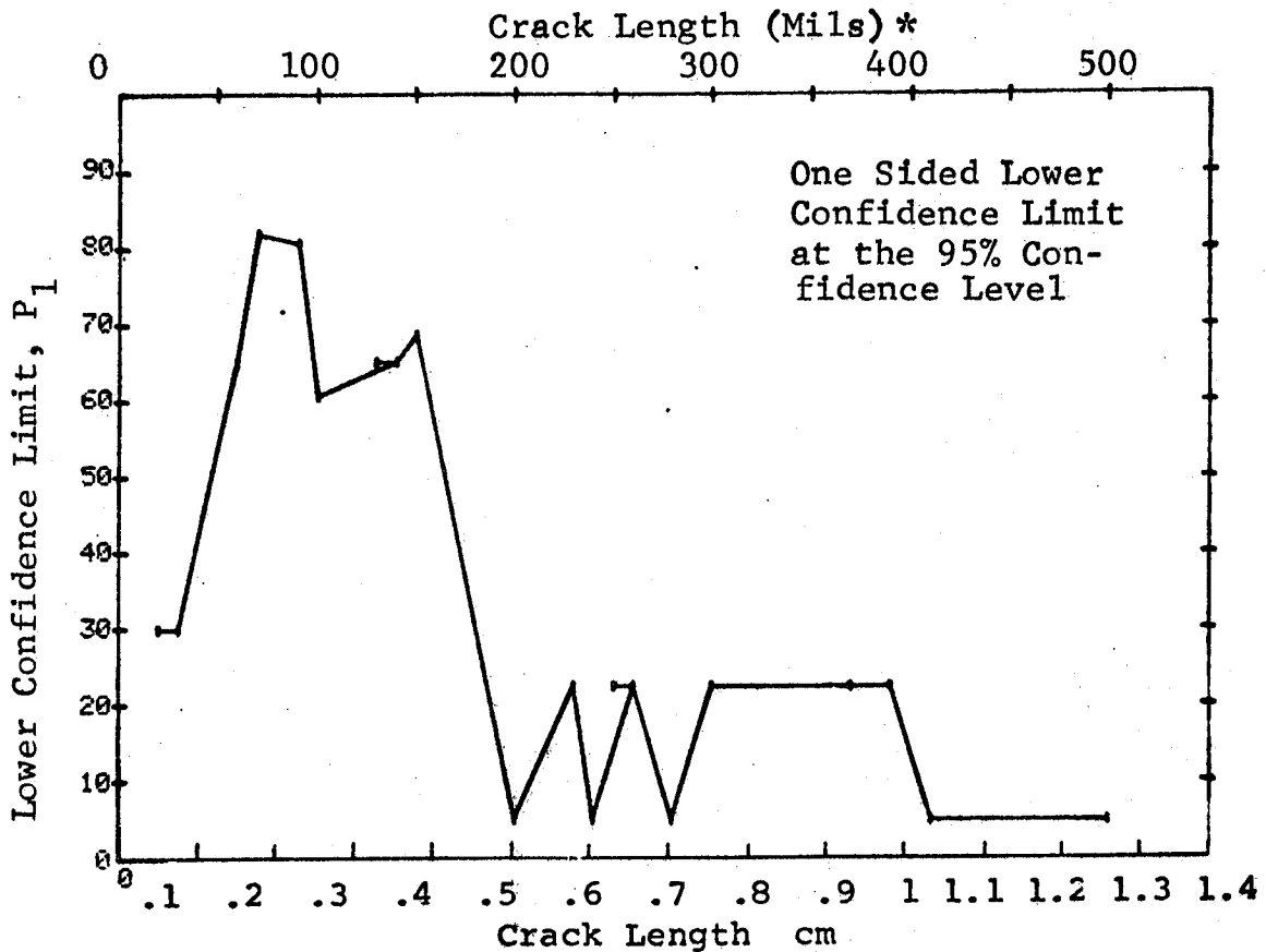
Figure D-78 Probability of Detection for 4340M Steel Using Ultrasonic Shear and Surface Waves. Compressed Notch Flaws in Filleted Solid Cylinder. Lab. Env.
