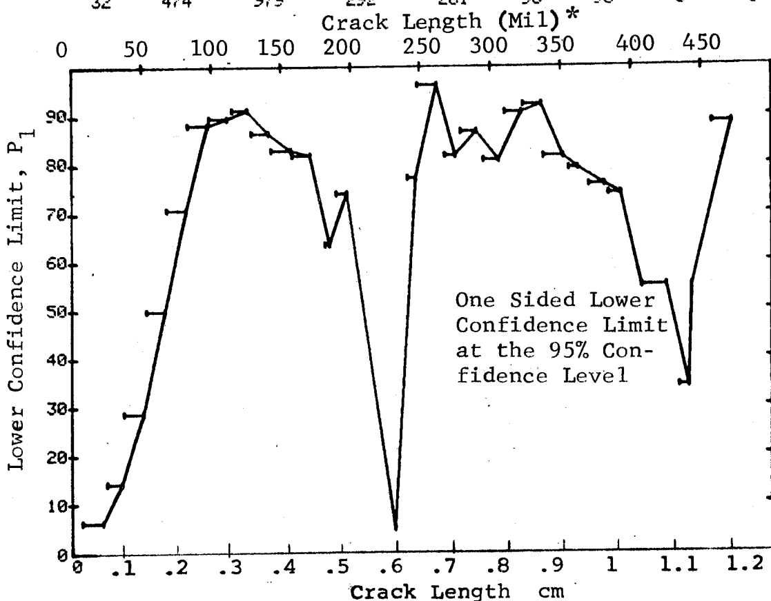
Figure D-35 Probability of Detection for 2219-T87 Al Using Eddy Current. Etched Fatigue Cracks in Flat Plates Merged for 5 Operators. D-108 Lab. Env.
