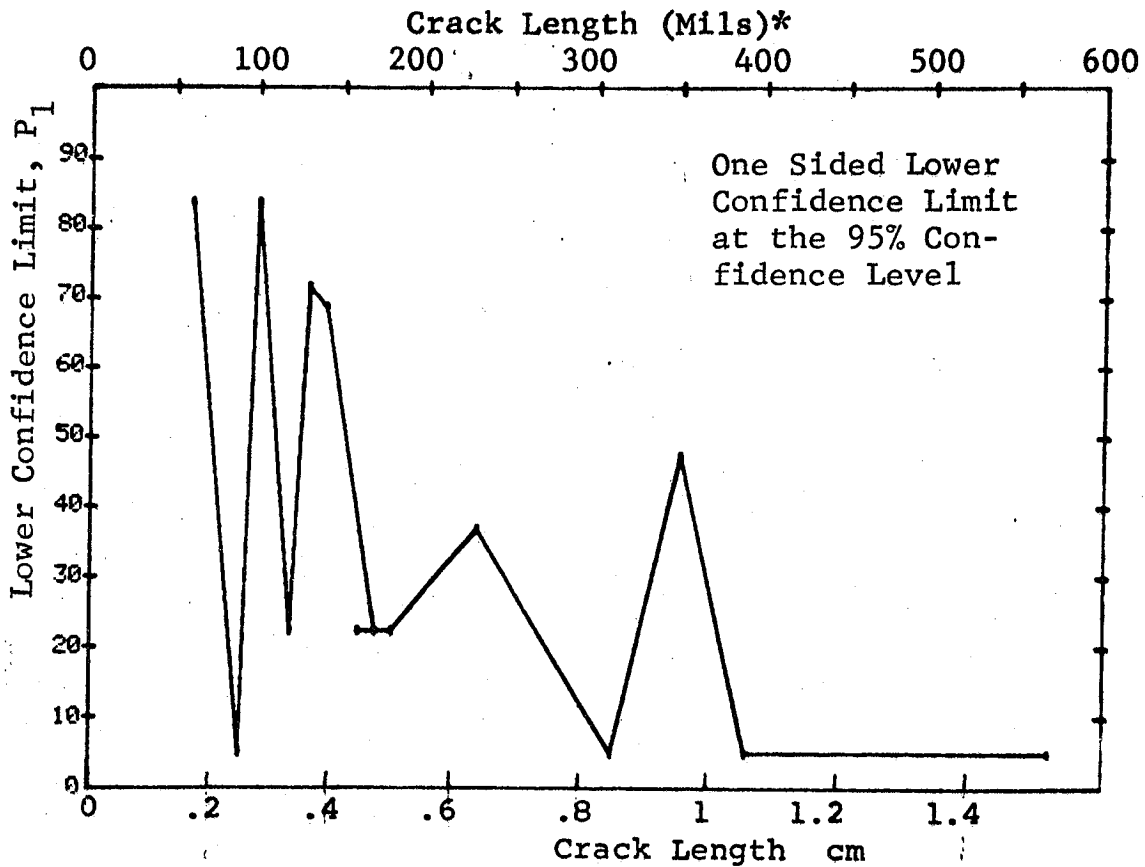
Figure D-102 Probability of Detection for 4340M Steel Using Magnetic Particles. Compressed Notch Flaws in Hollow Cylinder. Lab. Env.
