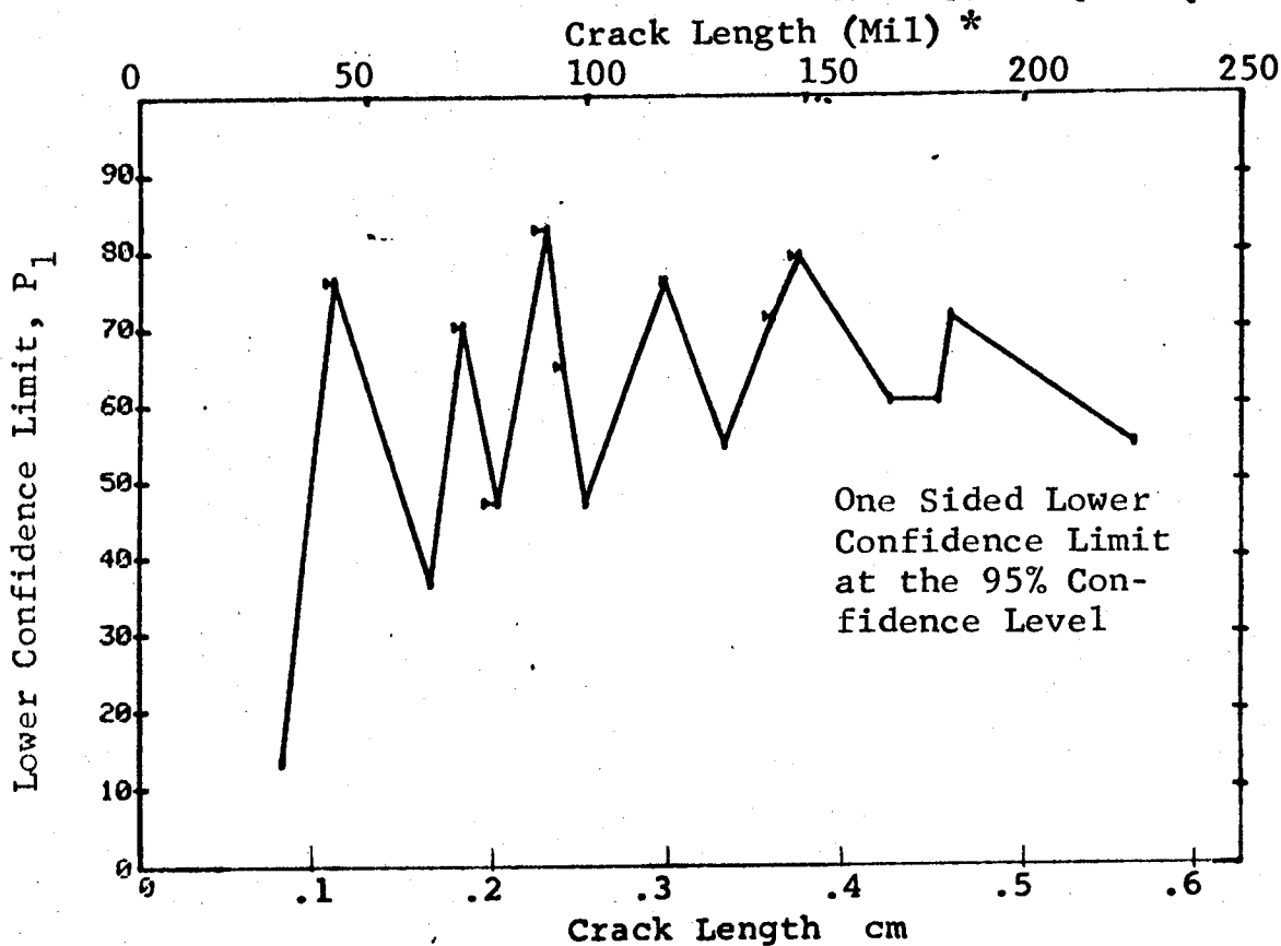
Figure D-47 Probability of Detection for PH17-4 Steel Using Ultrasonic Shear Wave. Fatigue Cracks in Flat Plates. Prod. Env. D-145
