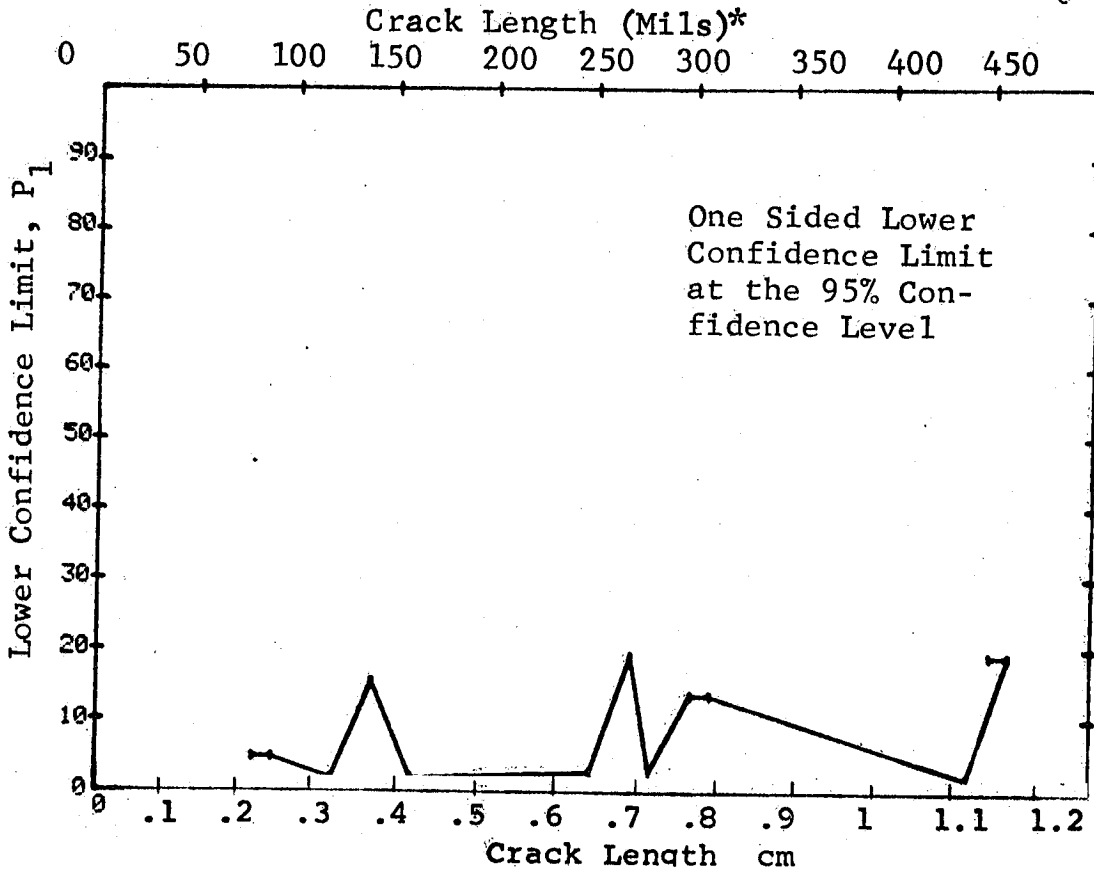
Figure D-62 Probability of Detection for 4340M Steel Using Liquid Penetrant. Compressed Notch Flaws in Hollow Cylinder. Prod. Env.
