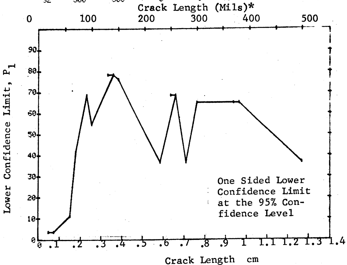
Figure D-111 Probability of Detection for 4340M Steel Using Eddy Current. Compressed Notch Flaws in Solid Filleted Cylinder. Laboratory Environment
