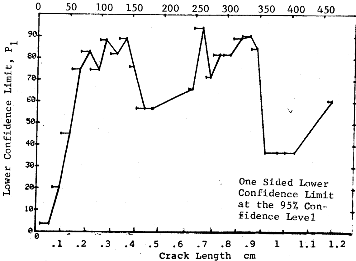
Figure D-1 Probability of Detection for 2219-T87 Al Using Ultrasonic Surface Waves. Fatigue Cracks in Flat Plates. Lab. Env. D-β
