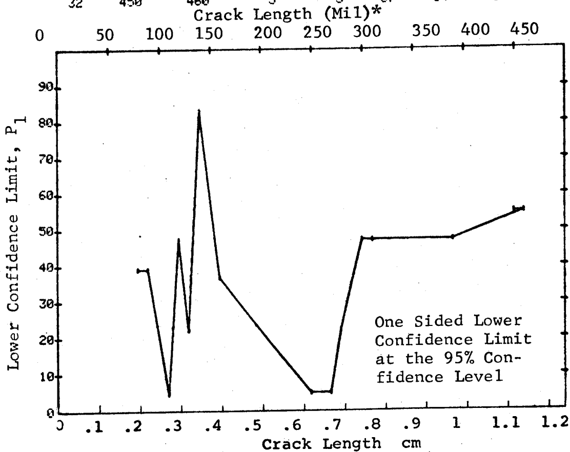
Figure D-67 Probability of Detection for 4340M Steel Using Liquid Penetrant. Compressed Notch Flaws in Hollow Cylinder. Lab. Env.
