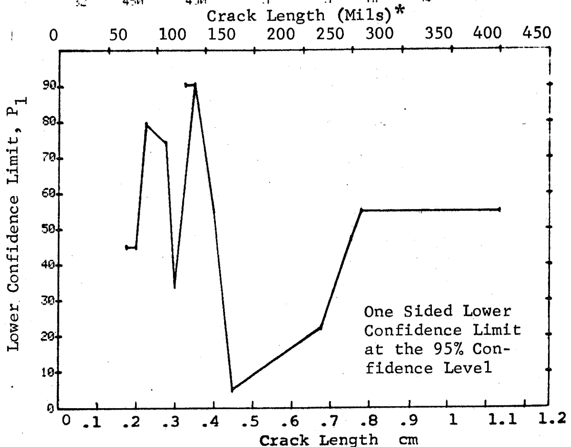
Figure D-110 Probability of Detection for 4340M Steel Using Eddy Current. Compressed Notch Flaws in Hollow Filleted Cylinder. Laboratory Environment.
