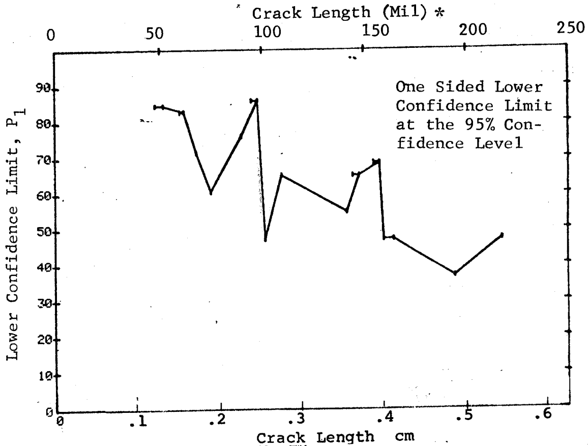
Figure D-44 Probability of Detection for Ti-6Al-4V Using Ultrasonic Shear Wave. Fatigue Cracks in Welded Flat Corroded Plates. Prod. Env.
