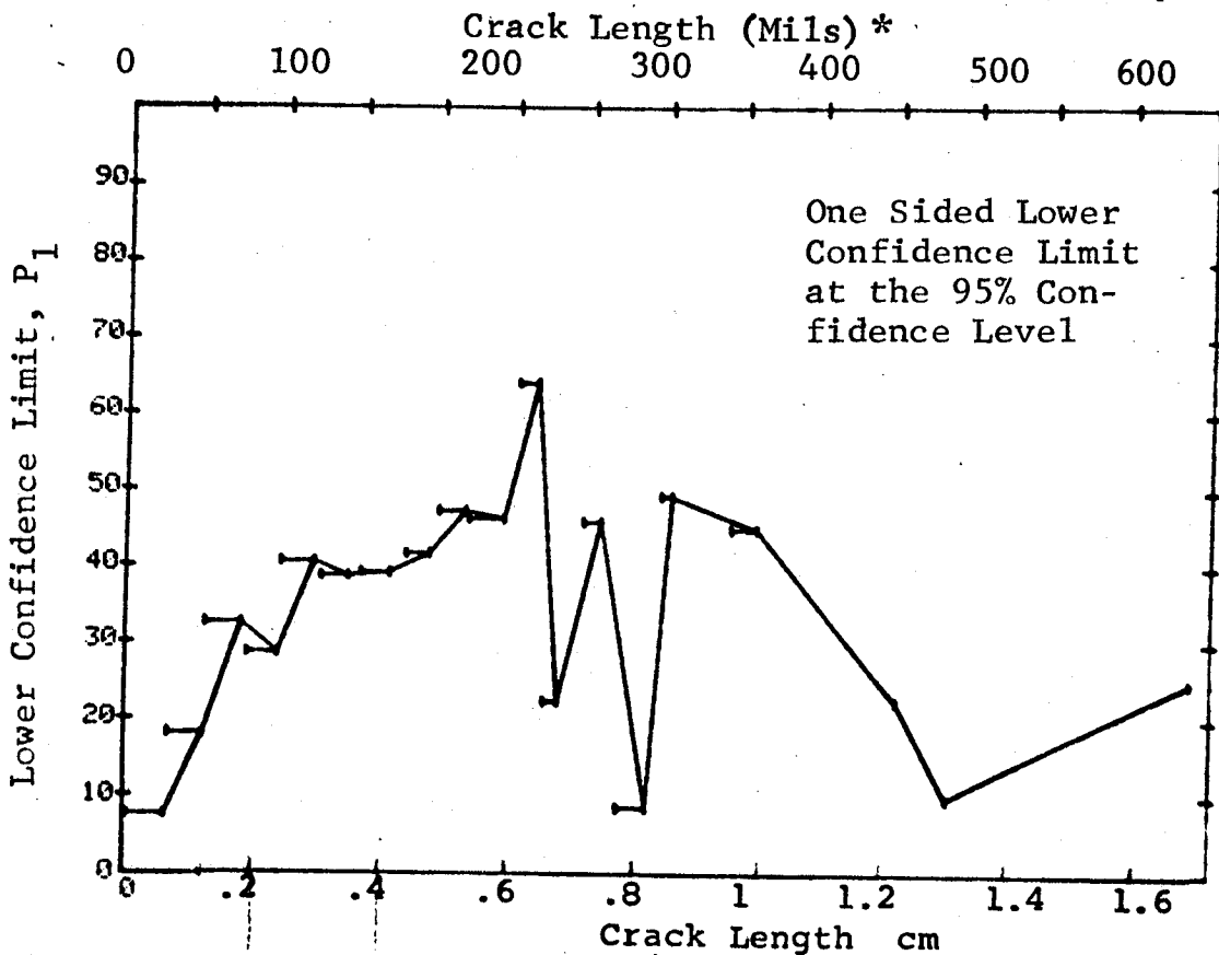
Figure D-59 Probability of Detection for 7178-T651 Al Using Eddy Current. Fatigue Cracks in Fastener Holes Measured by 5 Merged Teams. Field Env.
