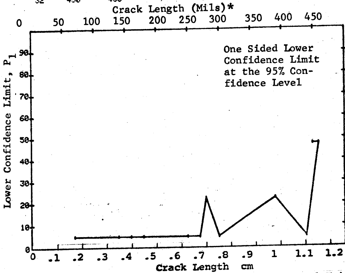
Figure D-89 Probability of Detection for 4340M Steel Using X-ray. Compressed Notch Flaws in Hollow Filleted Cylinder. Lab. Env. D-273
