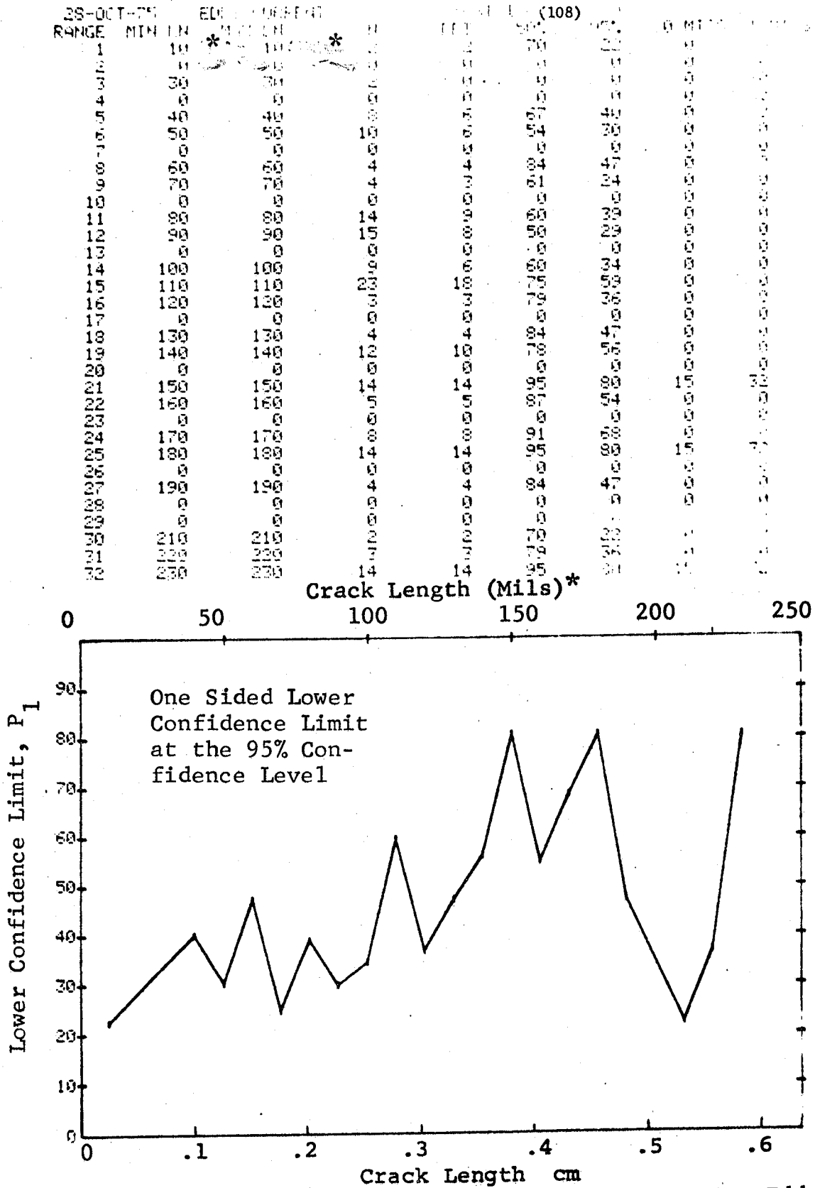
Figure D-108 Probability of Detection for 2024-T6 Al Using Eddy Current. Compressed Notch Flaws in Tandem T Specimen. Laboratory Environment.
