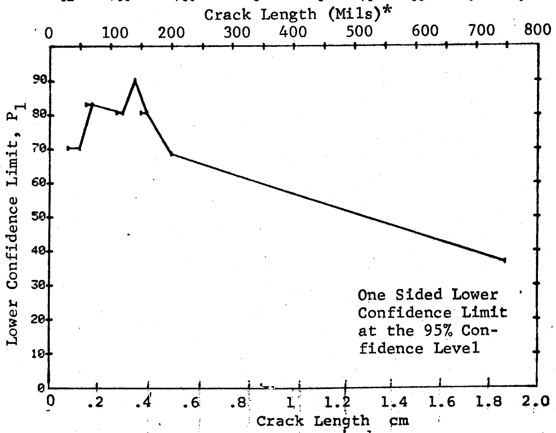
Figure D-76 Probability of Detection for 4340M Steel Using Ultrasonic Shear and Surface Waves. Compressed Notch Flaws in Filleted Solid Cylinder. Prod. Env.
