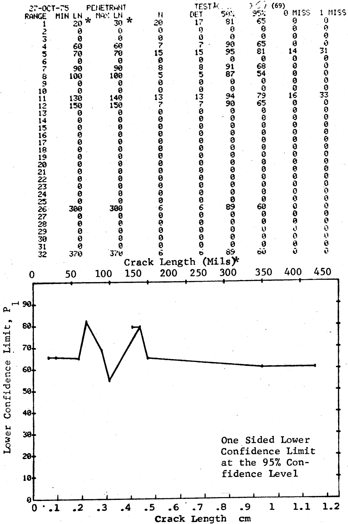
Figure D-69 Probability of Detection for 4340M Steel Using Liquid Penetrant. Compressed Notch Flaws in Filleted Solid Cylinder. Lab. Env. D-213
