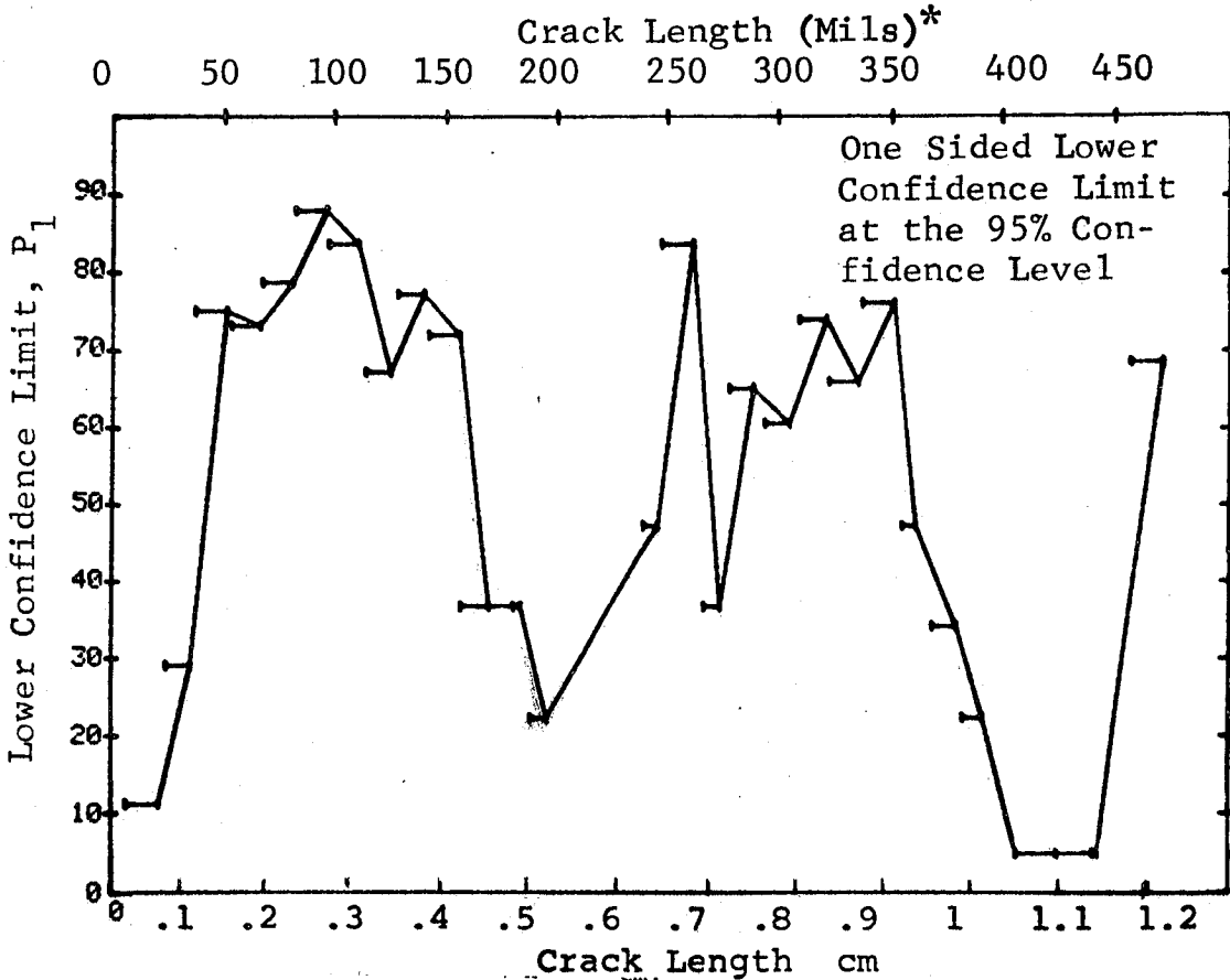
Figure D-14 Probability of Detection for 2219-T87 Al Using Liquid Penetrant. Etched Fatigue Cracks in Flat Plates Measured by Operator H. Lab. Env.
