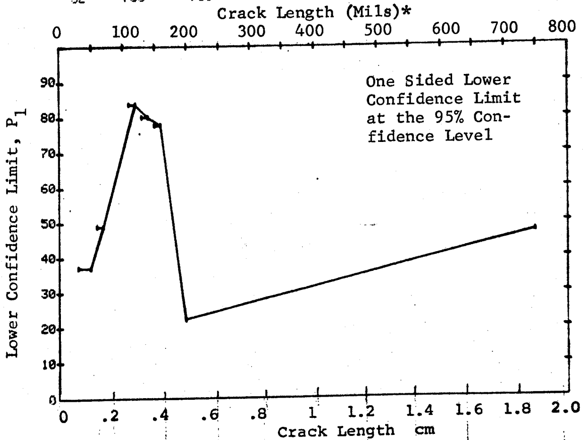
Figure D-103 Probability of Detection for 4340M Steel Using Eddy Current. Compressed Notch Flaws in Solid Cylinder. Prod. Env.
