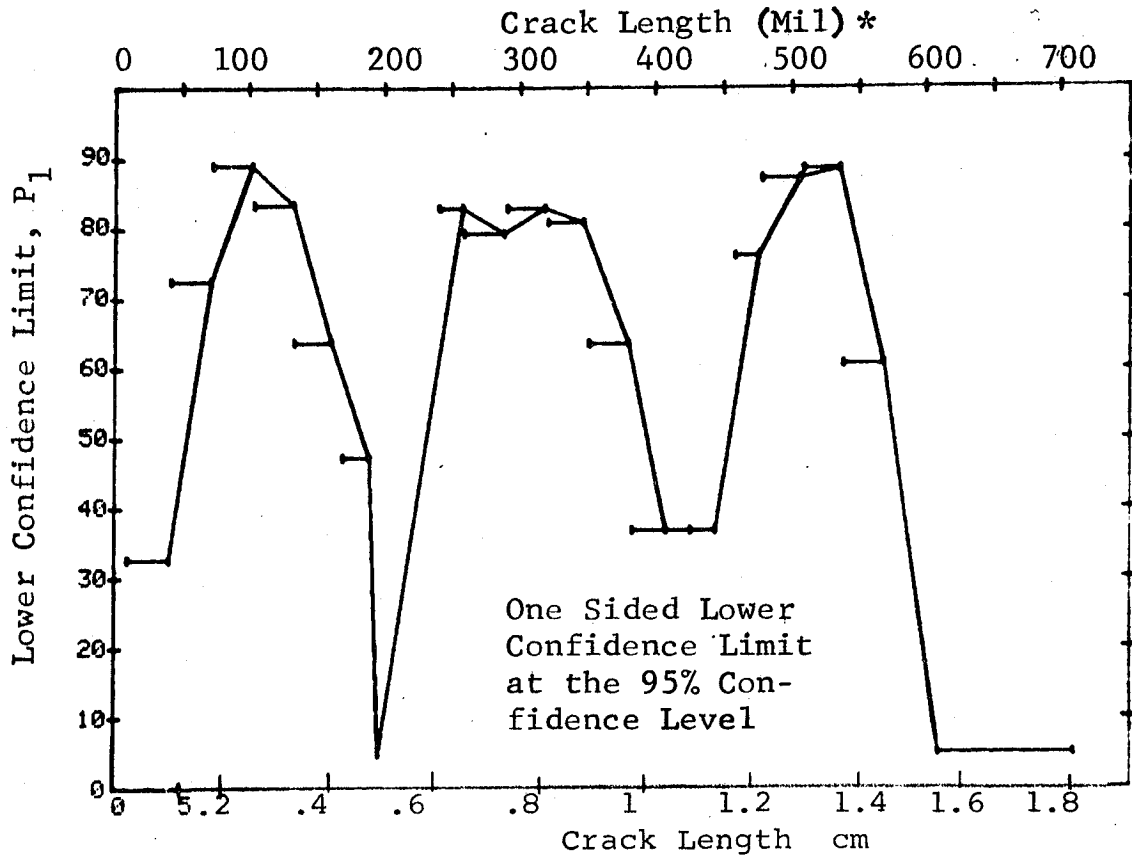
Figure D-19 Probability of Detection for 2219-T87 Al Using Liquid Penetrant. Etched Fatigue Cracks in Flat Plates Measured by Operator M. Lab. Env.
