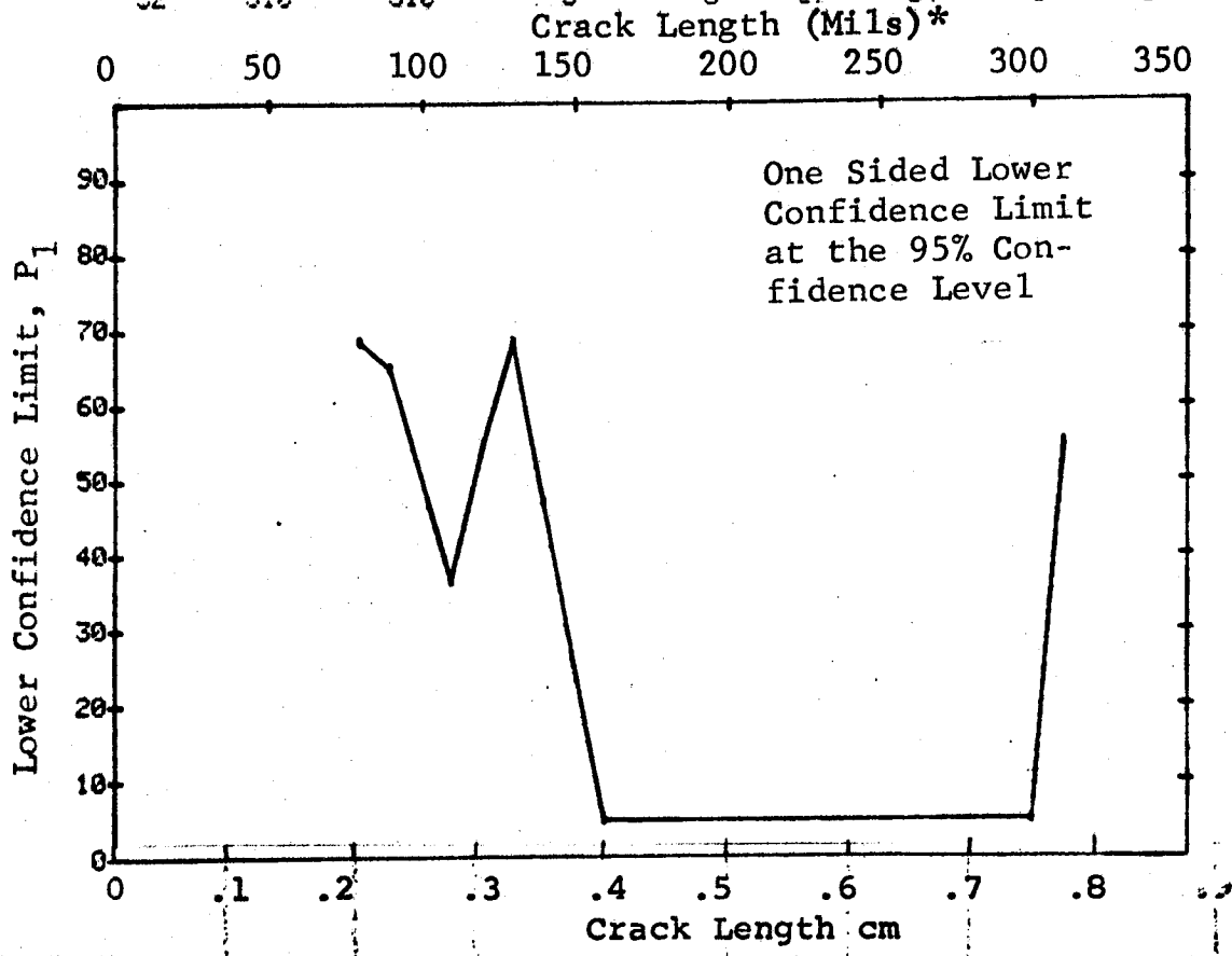
Figure D-73 Probability of Detection for 4340M Steel Using Ultrasonic Shear and Surface Waves. Compressed Notch Flaws in Hollow Cylinder. Prod. Env.
