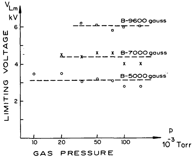
FIGURE 21.8.2.—The limiting value V_{Lm} of the burning voltage as a function of gas pressure for hydrogen in the homopolar experiment. V_{Lm} is independent of pressure, but proportional to the magnetic field B . (From Angerth et al., 1962.)
