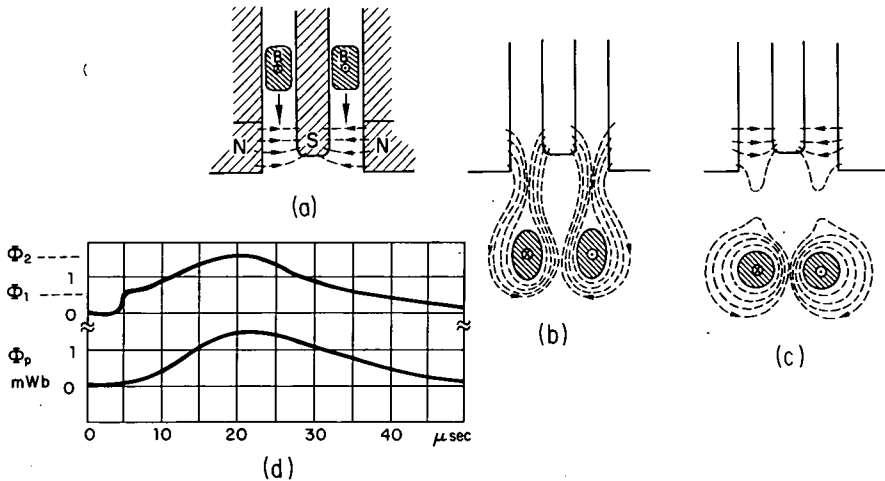
FIGURE 15.3.3.—Geometry of the Lindberg plasma ring experiment. (a) Before leaving the gun, the plasma has a toroidal magnetization B . It is shot through the radial field N-S . (b) On leaving the gun, the plasma ring pulls out the lines of force of the static magnetic field. (c) Plasma ring with captured poloidal field. If the toroidal magnetic energy is too large, a part of it is transferred to poloidal magnetic energy (through kink instability of the current). (d) The poloidal magnetic flux \Phi_p during the above experiment. The upper curve shows how the ring, when shot out from the gun, first acquires a poloidal flux \Phi_1 . An instability of the ring later transforms toroidal energy into poloidal energy thus increasing the flux from \Phi_1 to \Phi_2 . The upper and lower curves represent the flux measured by two loops at 15 and 30 cm distance from the gun, respectively.
