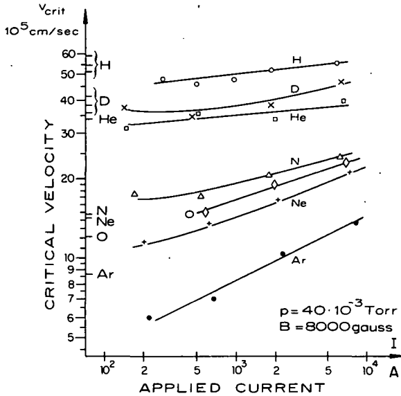
FIGURE 21.8.5.—Critical velocity v_{crit} versus applied current for seven gases studied in the homopolar experiment. (The slope of the Ar curve is related to the magnetic field's being too weak to make the ion gyro-radii small enough). The theoretical v_{crit} for each gas, as calculated from eq. (21.6.1), is indicated on the ordinate. (From Angerth et al., 1962.)
