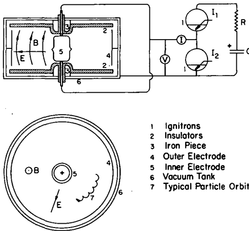
FIGURE 21.8.1.—Homopolar apparatus. A voltage V is applied across an inner electrode (5) and an outer electrode (4) to give a radial electric field E . The electric field, in the presence of an axial magnetic field B , acts on the ionized portion of the gas to set it into rotation (7). The interaction between the rotating magnetized plasma and the nonionized, nonrotating gas (in contact with the wall) produces a voltage limitation indicating that the relative velocity of the two components attains a critical velocity v_{crit} . (From Angerth et al., 1962.)
