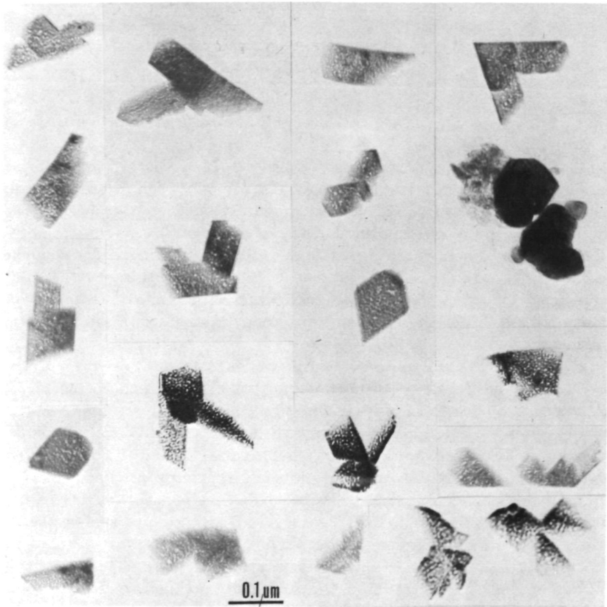
FIGURE 7.1.1.—Freely grown crystals of olivine and pyroxene forming aggregate material in the carbonaceous chondrite Allende. The delicate crystals are frequently twinned and have a thickness of the order of a few hundred Å, thinning toward the edge. The growth of the crystals and chemical composition of the material suggest that they condensed from a vapor phase and subsequently evolved into orbits with relative velocities sufficiently low to permit accretion by electrostatic adhesion. (From Alfvén and Arrhenius, 1974.)
