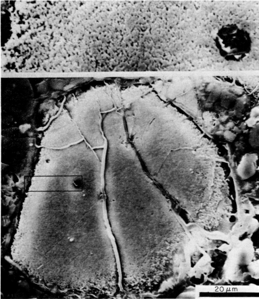
FIGURE 22.9.1. —Etched cross section through magnesium silicate (olivine) chondrule from the meteorite Fayetteville. The etching reveals a high concentration of cosmic-ray particle tracks at the surface, rapidly falling off toward the interior, reflecting the hardness spectrum of the radiation. The track distribution shows that the chondrule was turned around and irradiated from all sides before it was permanently embedded in the grain aggregate that now, in compacted form, constitutes the meteorite material. Before the preserved irradiation dose was received, the left part of the chondrule was broken off, presumably in a collision event. The area on the fracture edge, framed in the lower photograph, is shown in five times higher magnification in the upper photograph, illustrating the tracks and the radial track gradient in greater detail. The track density at the edge is 10^{10} \text{ cm}^{-2} . (From Maccougall et al., 1974.)
