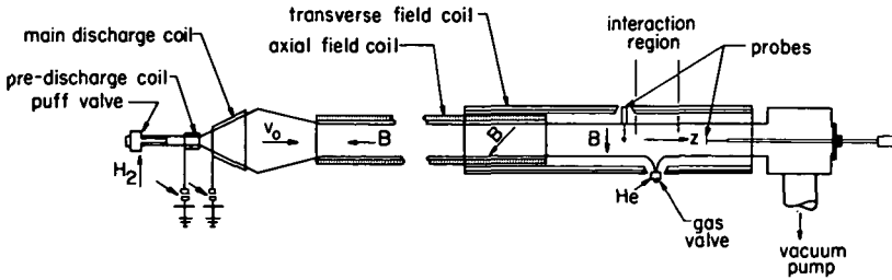
FIGURE 21.8.6.—Experimental arrangement for critical velocity measurement used by Danielsson. The left part is a plasma gun, emitting a magnetized plasma with a velocity v_0 . In a long drift tube, the longitudinal magnetization is changed to transverse magnetization. A thin cloud of gas is injected through the gas valve. If v_0 is below the critical velocity, the plasma beam passes through the gas cloud with very little interaction because the mean free path is long. If v_0 is above the critical velocity, there is a strong interaction, bringing the velocity to near the critical value. At the same time, the gas cloud becomes partially ionized. (From Danielsson, 1969b.)
