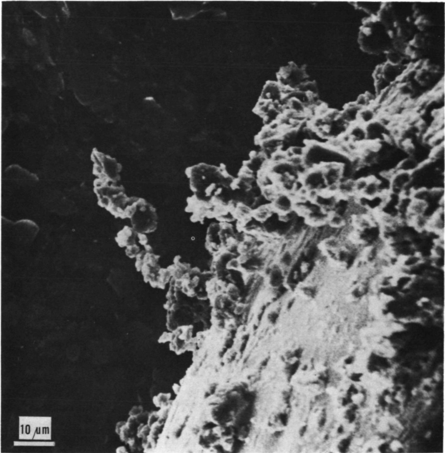
FIGURE 7.4.2.—Grains clustering to form a flexible chain extending about 40 \mu\text{m} from the base of the aggregate. The chain structure illustrates the electric dipole nature of the individual microparticles. (From Arrhenius and Asunmaa, 1973.)
