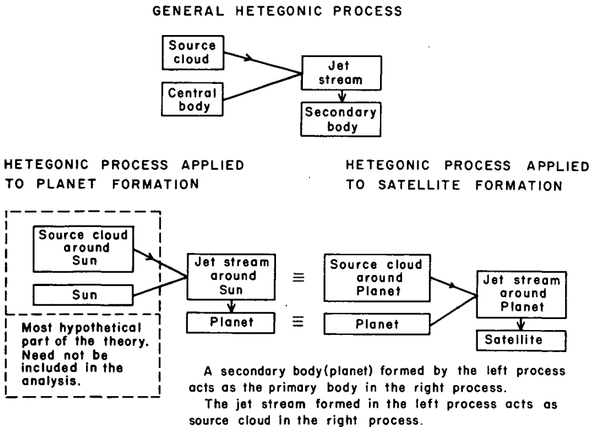
FIGURE 16.9.1.—Diagram showing how the speculative character of a theory is reduced by the hetegonic principle which implies that all theories should be applicable to both planetary and satellite systems. This eliminates the need to rely on hypotheses about the early Sun and ties the theory closer to observations.
