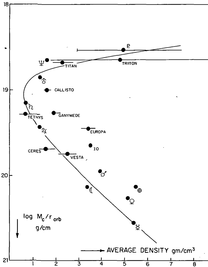
FIGURE 20.7.1c.—Average density as a function of gravitational potential energy, M_c/r_{orb} , for the planets and better known satellites. The distribution indicates that heavy substances accumulated both in the inner and outermost regions of the systems, whereas light substances dominate in the intermediate region. Symbols are those used in figs. 20.7.1a and b. Data from table 20.5.1.
