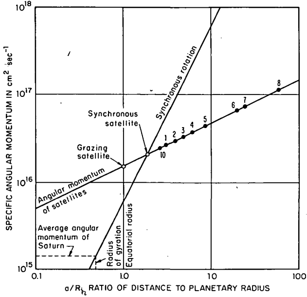
FIGURE 2.3.3.—Specific angular momentum of Saturn and its prograde satellites.
