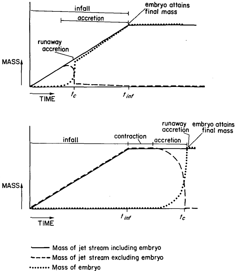
FIGURE 12.6.1.—Schematic representation of the accretion of an embryo from a jet stream. Plasma emplacement and infall of grains to the jet stream occurs during the time t_{inf} . The accreting embryo at first acquires mass slowly but then reaches catastrophic accretion at time t_c when all mass present in the jet stream is accreted by the embryo. For the case t_{inf} > t_c , a slow rate of accretion continues after the runaway accretion occurs. The slow accretion continues until plasma emplacement has ceased. For the case t_{inf} < t_c , as illustrated in the lower graph, after emplacement ceases and contraction of the jet-stream volume by negative diffusion increases the density in the jet stream, accretion commences and culminates in catastrophic accretion.
