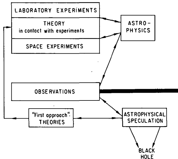
FIGURE 15.4.2.—An illustration of the present strategic situation in astrophysics. Before we are allowed to combine them with observations, the “first-approach” theories must be processed through the laboratory where many of their ingredients will no doubt be filtered away. This is the only way of building up astrophysics with a minimum of speculation. We have to learn again that science without contact with experiments is an enterprise which is likely to go completely astray into imaginary conjectures.
