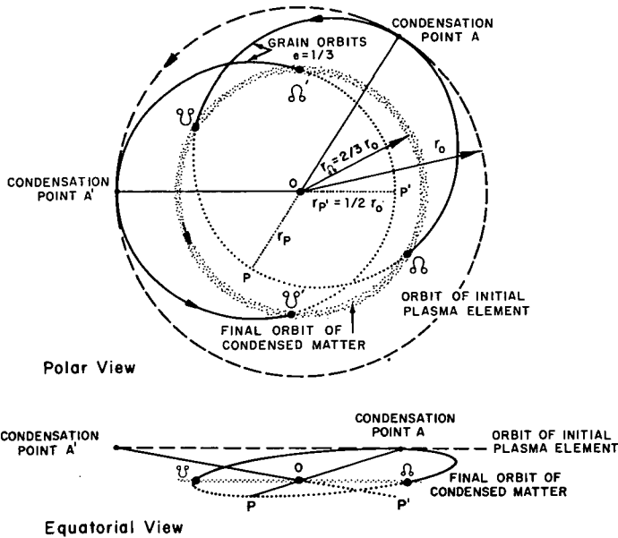
FIGURE 17.5.1.—The condensation process. The outer dashed line represents the circular orbit of a plasma element in the partially corotating plasma. Condensation produces small solid grains which move in Kepler ellipses with eccentricity e = 1/3 . Two such grain orbits are shown, one originating from condensation at A and the other, at A'. The condensation point A, which hence is the apocenter of the former orbit, has the spherical coordinates (r_0, \lambda_0, \phi_0) . The pericenter P is at r_P = r_0/2 , \lambda_P = -\lambda_0 , \phi_P = \phi_0 + \pi , and the nodal points are at r_\Omega = 2r_0/3 , \lambda_\Omega = 0 , and \phi_\Omega = \phi_0 \pm \pi/2 . Collisions between a large number of such grains result in the final (circular) orbit of solid particles in the equatorial plane. The eccentricity 1/3 of the initial grain orbit and the radius 2r_0/3 of the final orbit of condensed matter are direct consequences of the plasma being in the state of partial corotation (see secs. 17.3–17.5).
