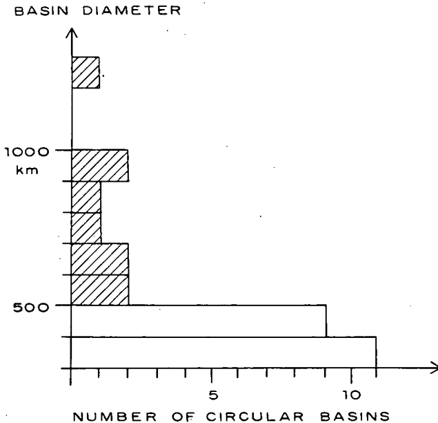
FIGURE 24.6.1.—Size distribution of circular basins on the Moon. The few large basins (indicated by diagonal stripes) may be the final resting places of either large lunar or terrestrial planetesimals or of the small "normal" satellites of the Earth. (From Stuart-Alexander and Howard, 1970.)
