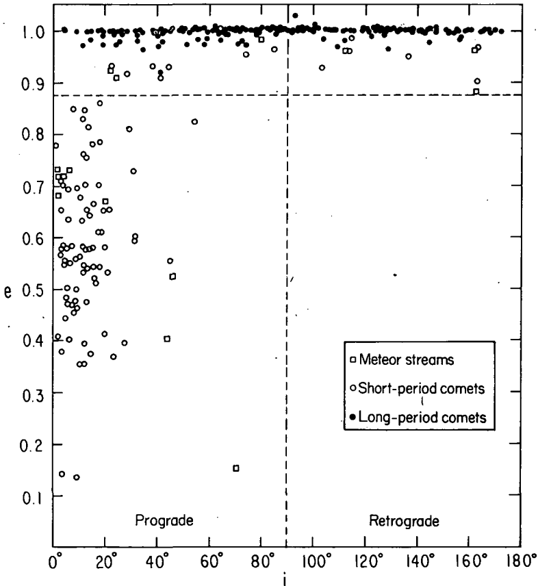
FIGURE 4.6.1.—Meteor streams, short-period comets, and long-period comets. Retrograde bodies are only found in almost parabolic orbits ( e > 0.85 ). Data from Porter (1961).
