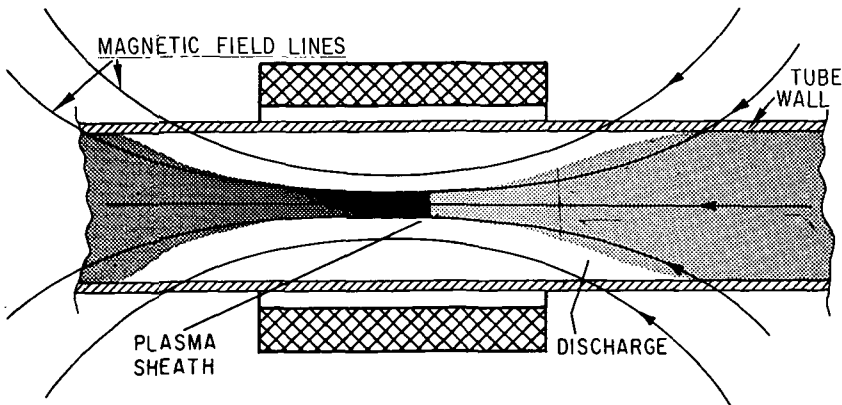
FIGURE 15.3.1.—Electrostatic double layers or sheaths are often produced in a plasma. The figure shows an electrostatic discontinuity produced spontaneously. The only function of the magnetic field is to keep the discharge away from the walls in order to ensure that the observed phenomena are not due to wall effects. Over the double layer a voltage drop is produced which sometimes suddenly becomes large ( \sim 10^6 V) and may disrupt the discharge.
