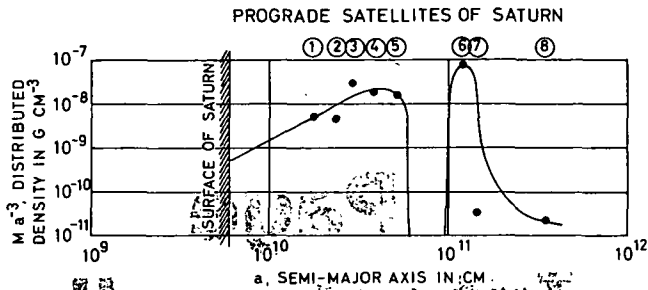
FIGURE 2.5.4 — Distributed density versus semimajor axis for the prograde satellites of Saturn.
