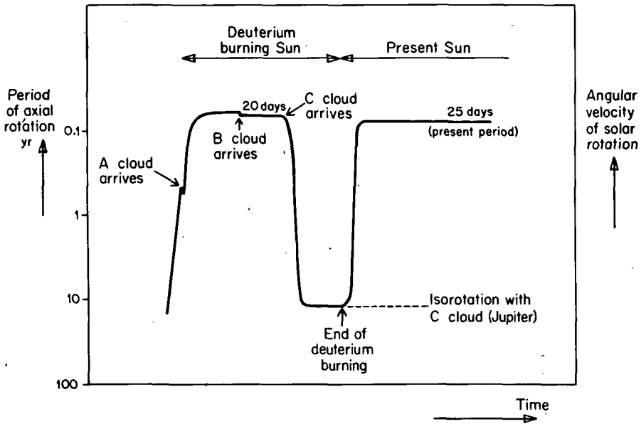
FIGURE 25.6.3.—Angular velocity of the Sun as a function of time. It is assumed that the solar system does not lose any angular momentum to infinity (angular momentum is conserved within the solar system). As the Sun contracts, its moment of inertia decreases, so that its angular velocity increases. The contraction during deuterium burning is small and the angular velocity remains constant. The B cloud (forming the Earth, Venus, and Mercury) forms during this period but does not change the solar angular momentum appreciably. (The A cloud may have formed earlier). When the C cloud (from which the giant planets accrete) forms, the Sun loses most of its angular momentum, and is brought into isorotation with Jupiter (period 12 yr). When the deuterium is totally consumed, the Sun contracts to its present state, with the moment of inertia decreasing by a factor of 200. The angular velocity increases by the same factor, accounting for the present angular velocity of the Sun.
