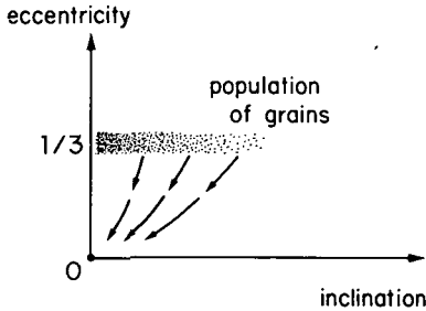
FIGURE 18.2.1.—Development of a population of grains originally orbiting in ellipses with eccentricity e = 1/3 and varying inclinations i . The final state with e = 0 and i = 0 is either a thin disc of grains or a group of planets (or satellites), in circular orbits in an equatorial plane.
