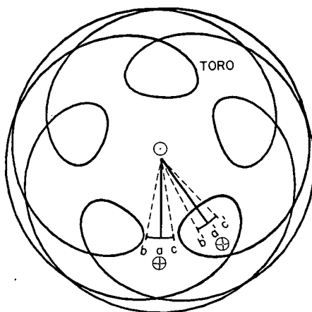
FIGURE 8.5.2.—Projection of 1685 Toro on the ecliptic plane in a coordinate system rotating with the Earth. Between 1600 AD and 1800 AD, the Earth-Sun line librates in the b'a'c' domain about the equilibrium position a' . The libration makes the transit to the bac domain around 1850 AD and remains there until 2200 AD. After 2200 AD the Earth-Sun equilibrium position will shift back from a to a' . The orbital pattern of Toro librates relative to the Earth, but for the sake of clarity the Earth is depicted as librating in relation to the orbital pattern of Toro. (From Ip and Mehra, 1973.)
