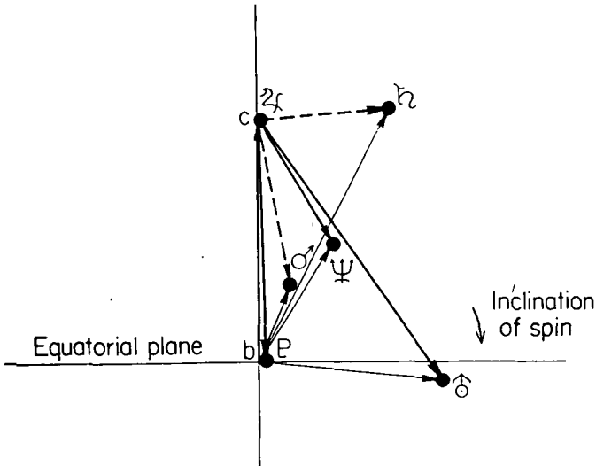
FIGURE 13.6.1.—Spin vectors of the planets are represented by the light lines (length \alpha \approx \Omega/\Theta^{1/2} ). The Giuli-type accretion gives a vector bc equal to Jupiter's spin. The statistical accretion should give the vectors from c to the dots representing the different planets. Dashed lines represent "late runaway accretion," the heavy lines, "delayed runaway accretion."
