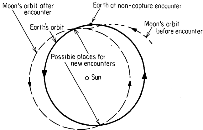
FIGURE 24.4.2.—If initially the orbits of the Earth and the planet Moon intersected, there would have been frequent encounters between the two bodies. Capture at any given encounter is unlikely. The most probable result is a deflection leading to a new orbit. However, this new orbit would also intersect the Earth's orbit so that a large number of new encounters would occur. The most probable final result is capture. (From Alfvén and Arrhenius, 1972a.)
