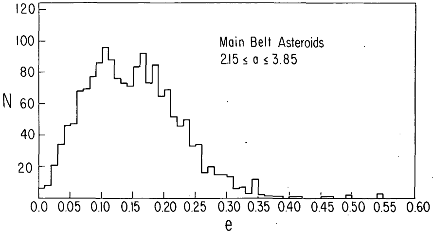
FIGURE 4.3.1.—Number of asteroids as a function of eccentricity. Data from the Ephemerides of Minor Planets for 1968 are shown for 1670 asteroids.
