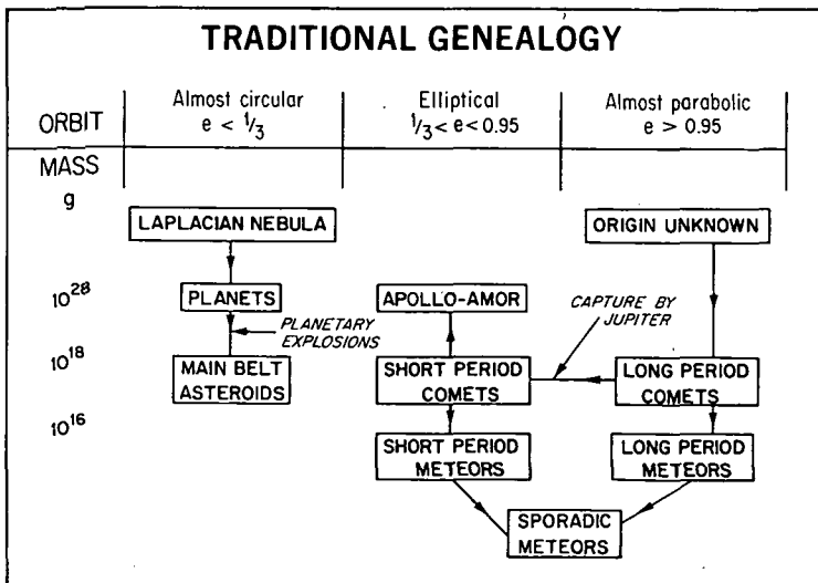
FIGURE 19.8.1.—Traditional view of genetic relationships between different types of bodies in the solar system.
