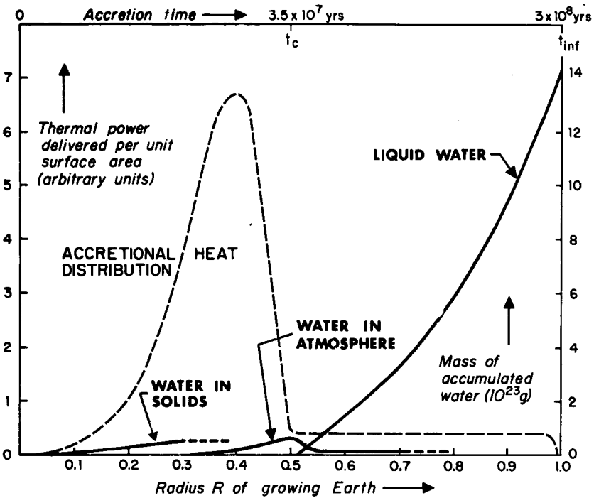
FIGURE 26.3.1.—The dashed curve and the left-hand ordinate show the thermal power (in arbitrary units) delivered per unit surface area of the growing Earth by impacting planetesimals (ch. 12). The lower abscissa shows the radius of the growing Earth in fractions of the present radius. The upper (nonlinear) abscissa scale shows the time elapsed from inception of accretion. The three solid curves show the accumulation of water on Earth. The left curve represents the amount retained in the coolly accreted inner core (arbitrary units). The middle curve shows the accumulated water in the atmosphere and the right-hand curve shows the accumulated liquid water; both in units of 10^{23} g. The final mass of accumulated water has been adjusted to equal the present ocean mass. (From Arrhenius et al., 1974.)
