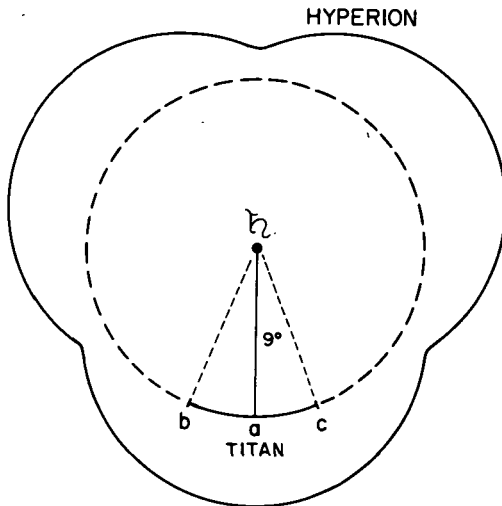
FIGURE 8.5.5.—The orbital pattern for the 4/3 resonance of Titan-Hyperion in the Saturnian satellite system. Titan librates with an amplitude of 9^\circ about the equilibrium position at a . The orbit of Hyperion is strongly perturbed by Titan.
