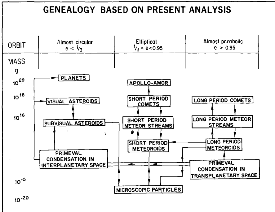
FIGURE 19.8.2.—Genetic relationships between the different types of bodies in the solar system. This genealogy is based on the present analysis.
