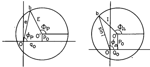
FIGURE 4.3.5.—Geometric illustration of the relationship of the osculating elements ( e , \phi_P , i , \phi_\Omega ) to the proper elements ( E , \Phi_P , I , \Phi_\Omega ) of motion for asteroids. As the representative point b describes a circle of typical period of 20 000 yr about point O , point O' migrates such that E and I remain constant. The
