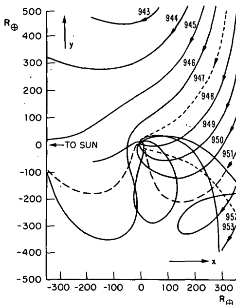
FIGURE 13.4.1—Planetesimal orbits in a rotating coordinate system x, y , in Earth radii, centered on the Earth (according to Dole). Small bodies (planetesimals) which originally move in circular orbits around the Sun with orbital radii greater than 1 AU will gradually be overtaken by the Earth. In a rotating coordinate system which fixes the Earth at the origin and the Sun on the abscissa to the left at a distance of 1 AU (thus assuming the Earth has a circular orbit), the particles will approach the Earth and will move in the complicated trajectories depicted in the figure. If their heliocentric orbital radii fall within seven ranges of values ("bands") all very close to the dashed line, they will hit the Earth. Otherwise, they will depart from the neighborhood of the Earth and return to heliocentric (but noncircular) orbits. Seven similar bands exist for particles with initial orbital radii less than 1 AU. (From Dole, 1962.)
