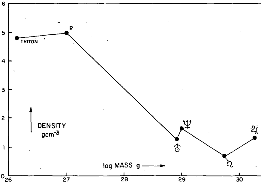
FIGURE 20.5.2.—Density of the outer planets as a function of their mass. It is difficult to believe that the density variation can be due to only the difference in mass.
