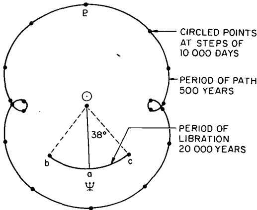
FIGURE 8.5.1.—The orbit of Pluto with respect to the Sun and to Neptune. The orbital pattern of Pluto librates relative to Neptune, but for clarity the Plutonian orbit is held stationary and the libration of Neptune relative to it is shown. The equilibrium position of Neptune is at a and Neptune librates between extreme positions at b and c with an amplitude of 38^\circ . (From Cohen and Hubbard, 1965.)
