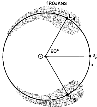
FIGURE 8.5.3.—The typical regions of libration of the Trojans around the Lagrangian points L_4 and L_5 of Jupiter.
