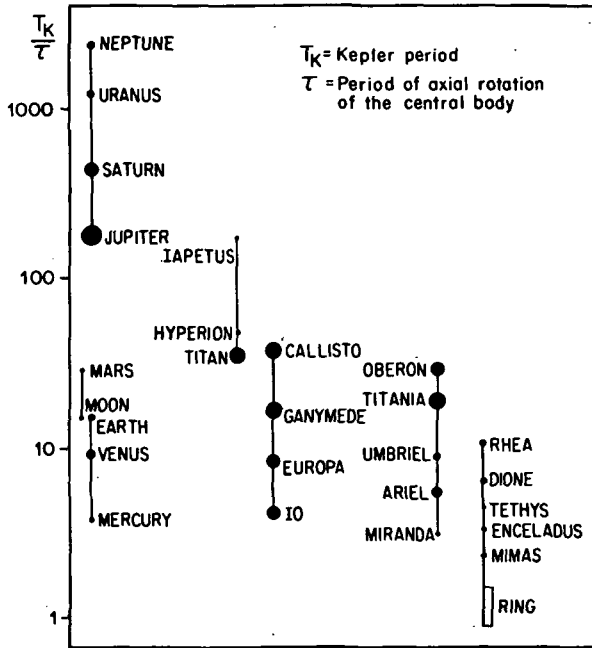
FIGURE 23.5.1.—Ratio between the orbital period T_K of secondary bodies and the spin period \tau of the central body. The latter quantity may have changed for the Sun, but not for the planets. The secondaries are grouped according to the cloud in which they formed. From left to right are the terrestrial planets, the giant planets, outer Saturnian satellites, Galilean satellites of Jupiter, the Uranian satellites, and the inner satellites of Saturn. (From Alfvén, 1962.)
