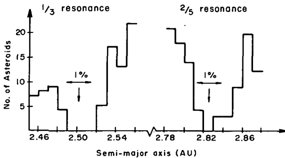
FIGURE 18.6.2.—The number of asteroids as a function of the semimajor axis showing gaps in the asteroid belt. The vertical arrows mark the orbital distances where the period of an asteroid is 1/3 or 2/5 of the period of Jupiter. The horizontal arrows extend 1 percent of the orbital distance for each resonance indicating the close correspondence of resonance points to these Kirkwood gaps. The reason why there are resonance gaps in the asteroid belt but not in the Saturnian rings is that the mass ratio Jupiter/Sun is 10 000 times larger than the mass ratio Mimas/Saturn.
