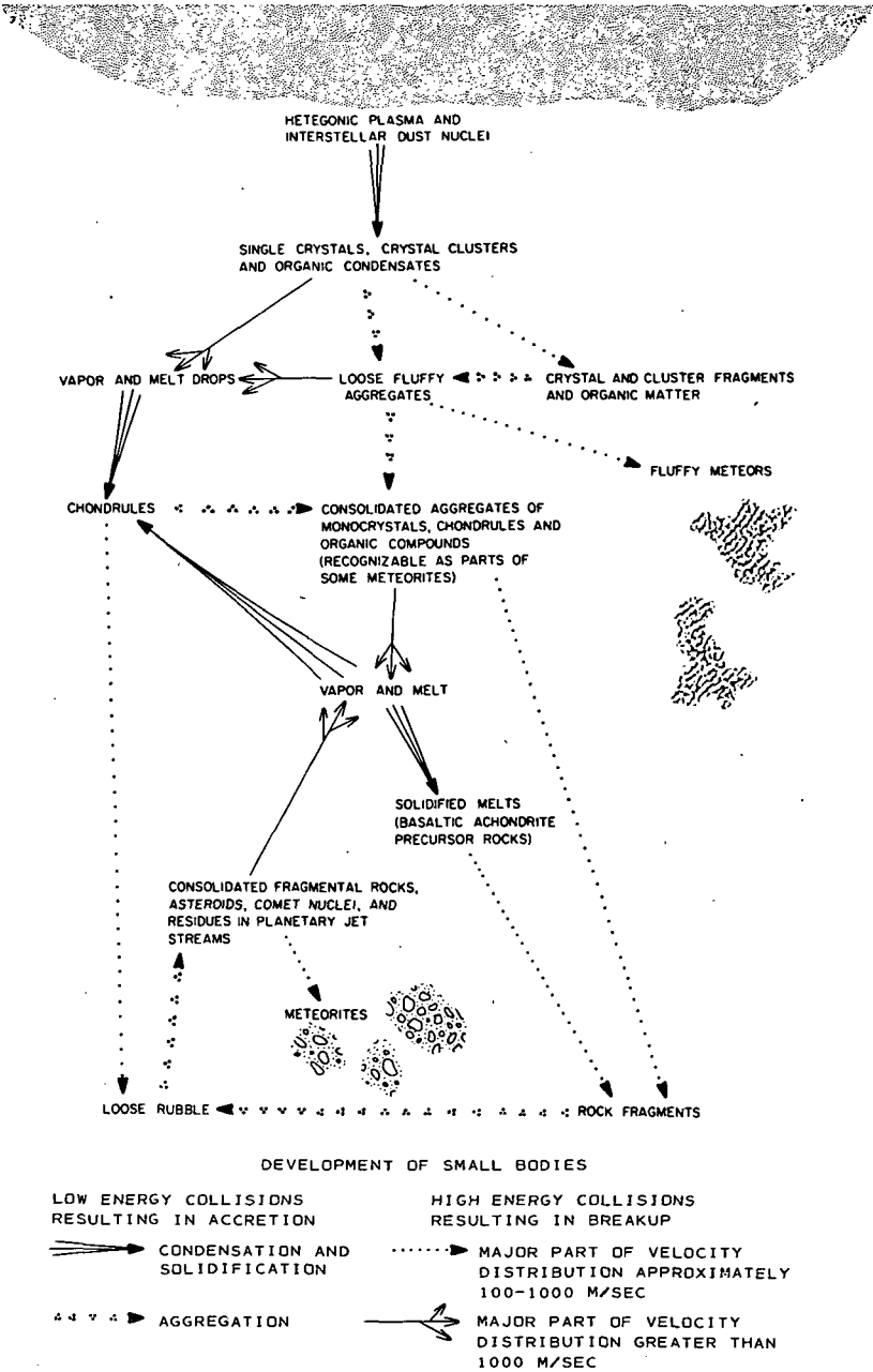
FIGURE 22.8.1.—Flow diagram of collision processes (indicated by directional arrows) in assemblages of particles and particle aggregates moving in Kepler orbits (jet streams).
