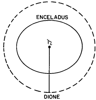
FIGURE 8.5.6.—The orbital pattern of the 2/1 resonance of Enceladus-Dione in the Saturnian system. The ellipticity of the orbit of Enceladus is exaggerated for the purpose of illustration. The perisaturnian of Enceladus precesses due to Dione.
