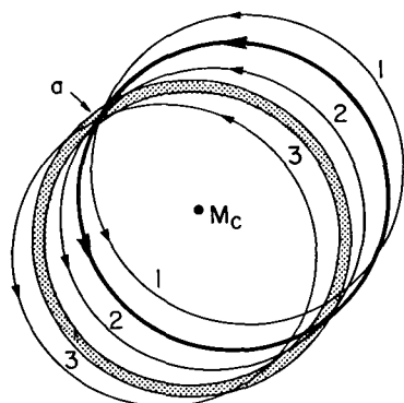
FIGURE 6.9.1.—The capture of a grain by a jet stream. The shaded area represents the jet stream. The orbit of a grain (thick curve) intersects the jet stream at a . Collisions lead to fragmentation and fragments are ejected mainly in orbits like 2, but some fragments may move in orbits like 1 or 3. All these orbits carry them back to the point a . Subsequent collision at a may lead to further fragmentation, but, if the collisions are at least partly inelastic, the final result is that all the fragments will be captured by the jet stream.
