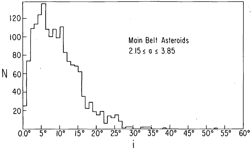
FIGURE 4.3.2.—Number of asteroids as a function of inclination. Data from the Ephemerides of Minor Planets for 1968 are shown for 1670 asteroids.
