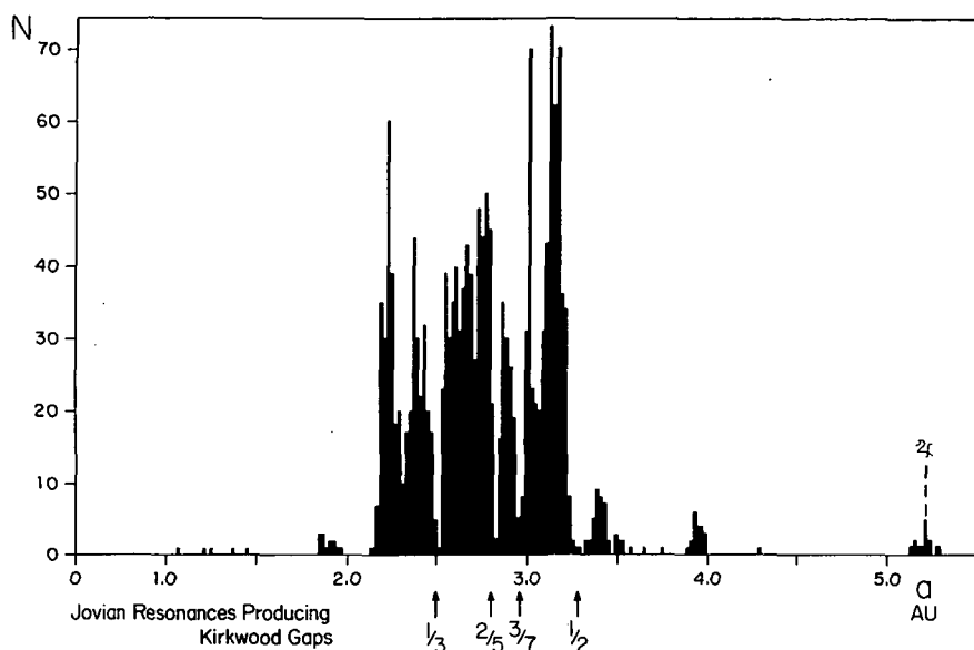
FIGURE 4.3.3.—The (N, a) diagram (number of asteroids as a function of semimajor axis). Most asteroids are located between 2.1 and 3.5 AU, constituting the main belt. The groups at 1.9, 3.9, and 5.2 AU are the Hungaria, Hilda, and Trojan asteroids, respectively. The sharp minima in the main belt are the Kirkwood gaps which occur at the \frac{1}{3} , \frac{2}{5} , \frac{3}{7} , and \frac{1}{2} resonances of Jupiter.
