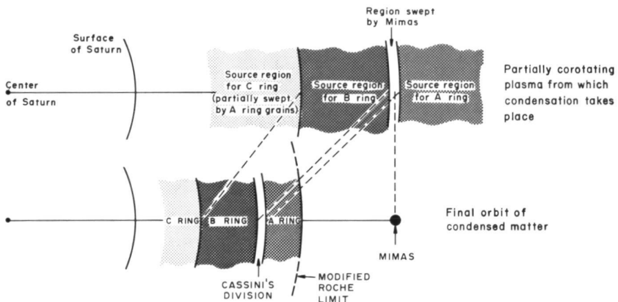
FIGURE 18.6.3.—Condensation of grains from a partially corotating plasma in the environment of Saturn. The condensation is assumed to take place essentially from the neighborhood of the equatorial plane (but only a negligible part in the plane itself). The figure refers to a state in which part of the plasma has already condensed so that Mimas (or its parent jet stream) and the rings already exist, although with only a small part of their present masses. The upper part of the figure refers to the plasma which has not yet condensed. The plasma near the orbit of Mimas condenses on this satellite (or on the jet stream in which it accretes), leaving the "region swept by Mimas" void of plasma. Similarly, the plasma in the region of the extant A ring (and B ring) condenses directly on the grains of the ring. When the grains produced by condensation fall down to \frac{2}{3} of their original central distances, the state depicted in the lower part of the figure is produced. Cassini's division is derived from the region swept by Mimas. The C ring has a reduced intensity because part of the plasma has condensed on the already existing grains of the A ring.
