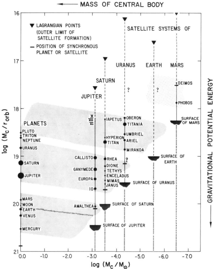
FIGURE 21.2.1.—Structure of the solar system in terms of the mass of the central bodies and the gravitational potential energy of the bodies orbiting around them. For a detailed analysis refer to secs. 21.2, 21.3, and 23.9.2. (From Alfvén and Arrhenius, 1972.)
