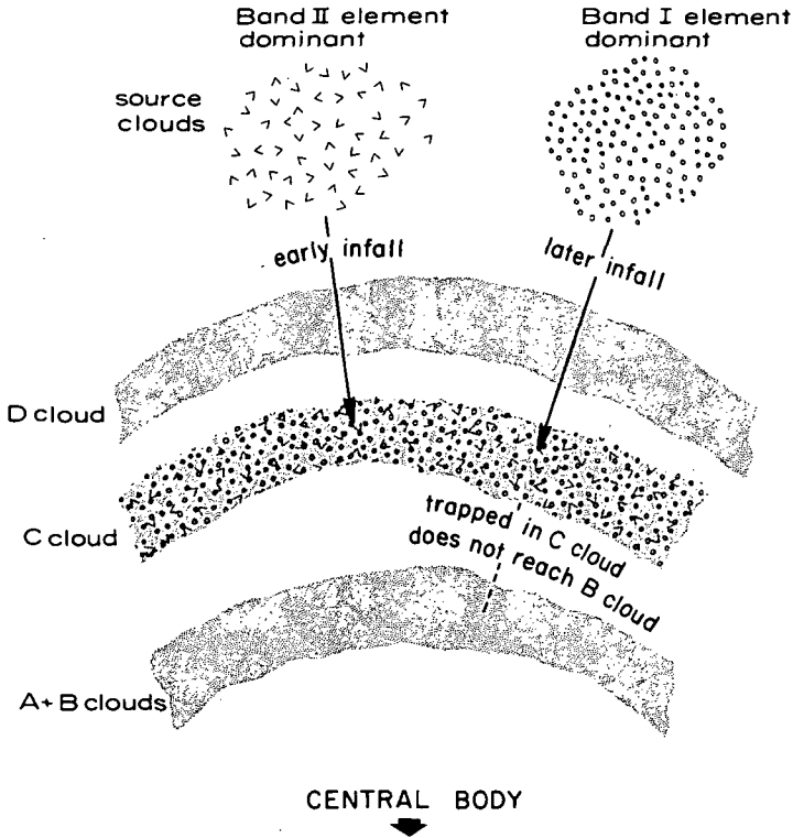
FIGURE 21.12.2. —Infall pattern for source clouds active during the same time period. A gas infall from a Band II element-dominated source cloud will be ionized and stopped in the C cloud. If this plasma has not had time to condense, it will interact with any infall from a Band I element-dominated source cloud. The Band I gas infall will be trapped in the C cloud by the plasma there and not reach its own r_{ion} in the B cloud.
