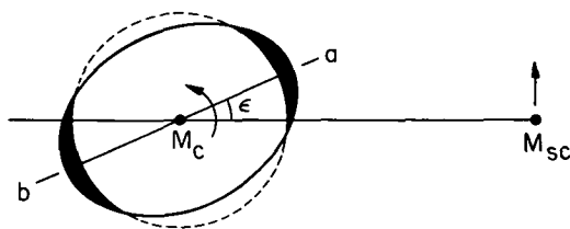
FIGURE 9.3.1.—Classical but inadequate model of momentum transfer due to tides. The force of attraction between the satellite M_{sc} and the near tidal bulge a exceeds that between M_{sc} and b ; a component of the net torque retards the rotation of the planet M_c and accelerates the satellite in its orbit. The actual situation in the case of the Earth is illustrated in fig. 9.4.1. In the case of Mars, Jupiter, Saturn, and Uranus, the angle \epsilon is probably negligible.
