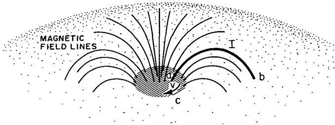
FIGURE 15.4.1.—The rotational motion v and the magnetic field in a sunspot may give rise to a voltage between the points a in the sunspot and b outside the sunspot, causing a discharge current I to flow along the magnetic field line from a to b . The circuit is closed through currents below the photosphere from b to c (and back to a ).
