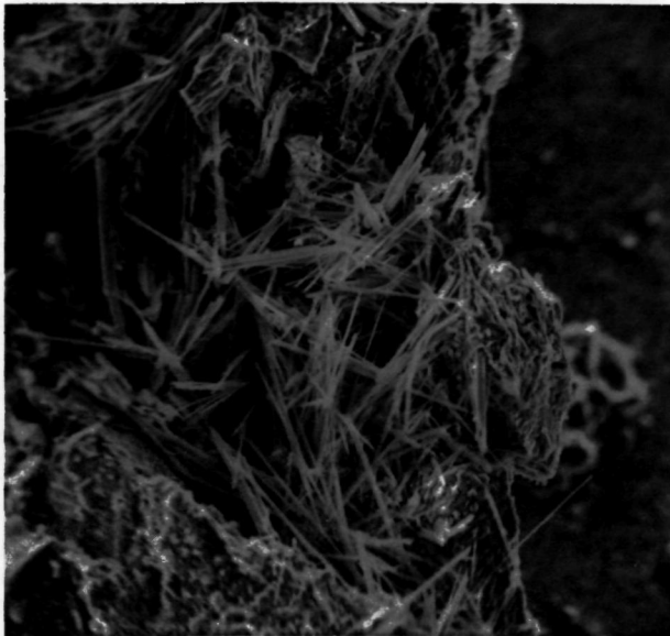
FIGURE 22.3.1.—Loose fiber aggregates of wollastonite ( \text{CaSiO}_3 ) in cavity from the meteorite Allende. Width of field is 0.4 mm. (From Fuchs, 1971.)
