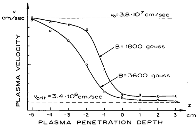
FIGURE 21.8.7.—Velocity retardation to near the critical value in the Danielsson experiment. Plasma deceleration with depth of penetration z in a neutral gas cloud of helium is shown. The front of the cloud is located at z = -5 cm, and the center, at z = 0 cm. The plasma undergoes deceleration from the impinging velocity v_0 to near the critical velocity v_{crit} of helium. Data for two values of the magnetic field B are shown. (From Danielsson, 1969b.)
