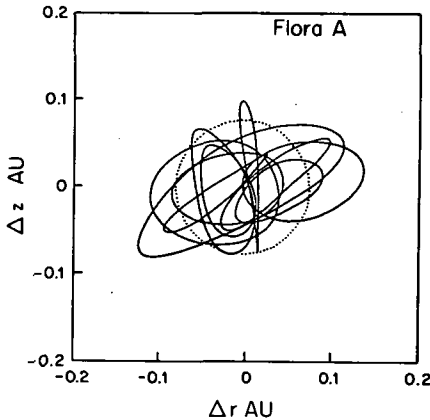
FIGURE 4.3.6.—Profile of the Flora A jet stream. Diagram shows the intersections of the individual orbits of these asteroids with a heliocentric meridional plane as this plane is rotated one cycle around the ecliptic polar axis. The positions of the orbits are shown relative to the mean orbit of the jet stream. The dotted circle shows the cross section of the jet stream as theoretically calculated in secs. 12.2 and 12.7. Most of the asteroid orbits in Flora A fall within the dotted circle. Profiles of other asteroidal jet streams show less concentration. (From Danielsson, 1971.)
