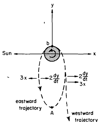
FIGURE 13.4.2.—Particles shot out tangentially to the east with approximately the escape velocity from the point b on the Earth's equator (at 0600 hrs local time) will move in an ellipse with apogee at A . The motion is disturbed only minimally by the Coriolis force ( 2dy/dt ) and by the tidal effect from the Sun ( 3x ) because these forces are antiparallel. Particles shot out tangentially to the west under the same conditions experience parallel Coriolis and solar gravitational forces which deflect the trajectory from the elliptic orbit. (From Alfvén and Arrhenius, 1970b.)
