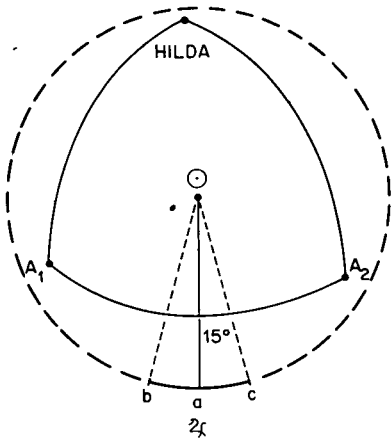
FIGURE 8.5.4.—Idealized orbit of 153 Hilda in the Jupiter-Sun rotating coordinate system. Due to the 3/2 resonance, Hilda describes a triangular trajectory in a time interval of 24 yr. Due to systematic perturbations the whole orbital pattern will oscillate with an amplitude of 15^\circ and a period of 260 yr. Points A_1 and A_2 are the aphelia of Hilda and also her points of closest approach to Jupiter. The distance between Hilda and Jupiter at close approach is never less than 4 AU. (From Ip, 1974a.)
