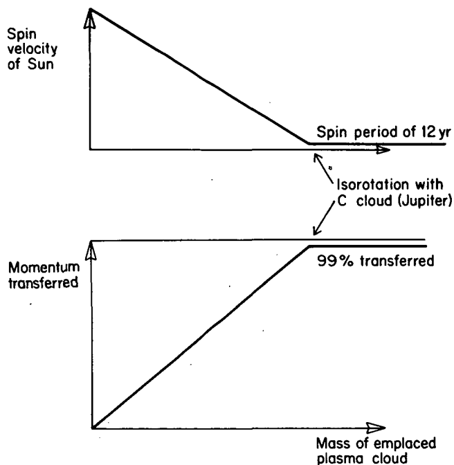
FIGURE 25.6.2. —Below: Angular momentum transferred to the C cloud as a function of the mass processed through this cloud. The transfer of momentum is proportional to the cumulative mass until a saturation is reached, when almost all the momentum is transferred. Above: Angular velocity of the Sun after the transfer. When saturation is reached, the solar angular velocity equals the Kepler velocity of Jupiter. If the transfer takes place when the Sun is in the deuterium-burning state with a moment of inertia 200 times the present value, the angular velocity increases by a factor of 200 as the Sun contracts, producing the present spin period (25 days) of the Sun when contraction is completed.
