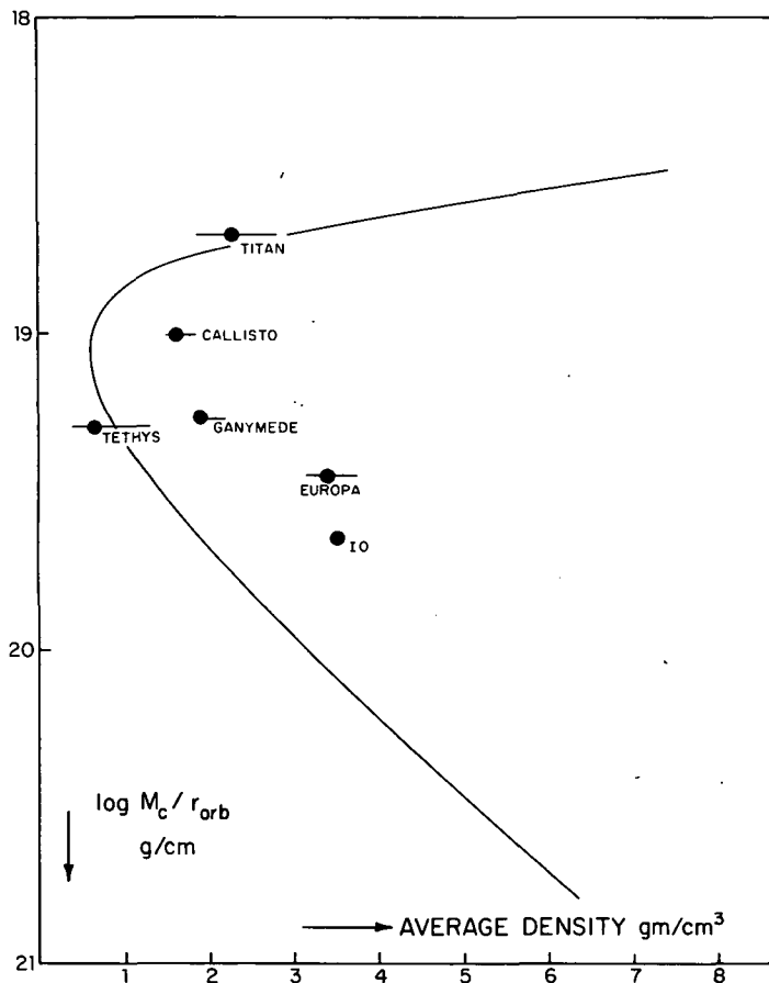
FIGURE 20.7.1b.—Average density as a function of gravitational potential energy, M_c/r_{orb} , for the regular satellite system of Jupiter and the two best known Saturnian satellites, Titan and Tethys. Solid circles denote density values based on the best estimates of radius and mass; horizontal lines indicate the estimated range of uncertainty. Data from table 20.5.1.
