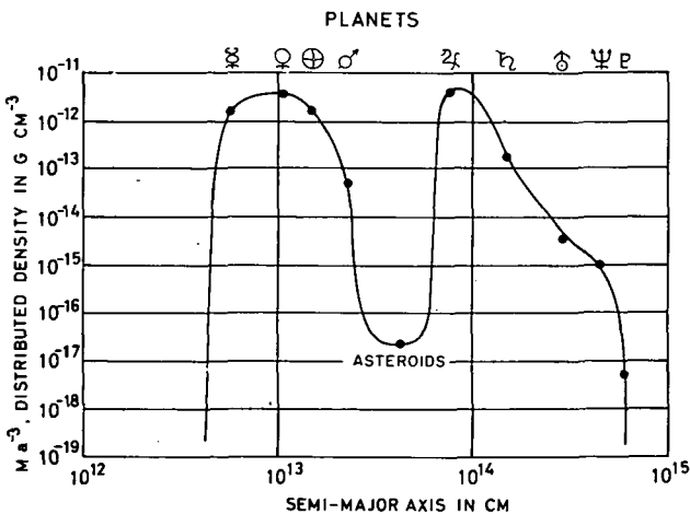
FIGURE 2.5.1.—Distributed density versus semimajor axis for the planets.
