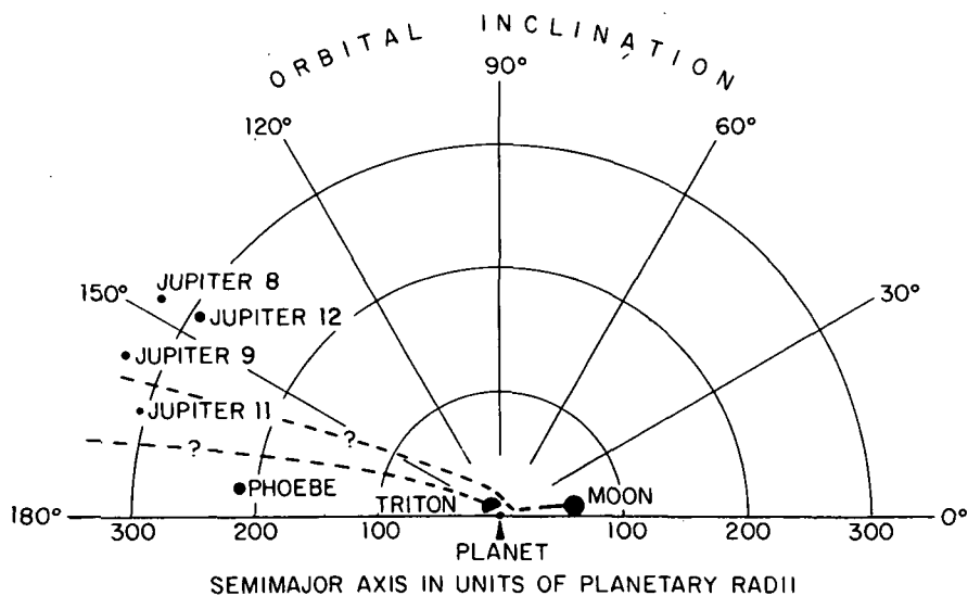
ORBITAL PARAMETERS OF CAPTURED SATELLITES AND POSSIBLE ORBITAL EVOLUTION OF MOON AND TRITON
