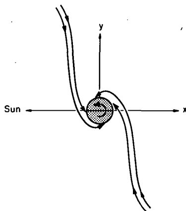
FIGURE 13.4.3.—Planetesimals originally moving in slightly eccentric Kepler ellipses in the solar field may hit the Earth in two jets, both giving prograde rotation.
