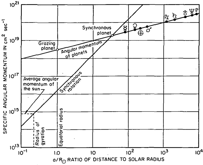
FIGURE 2.3.1.—Specific angular momentum of the Sun and planets. (From Alfvén and Arrhenius, 1970a.)
