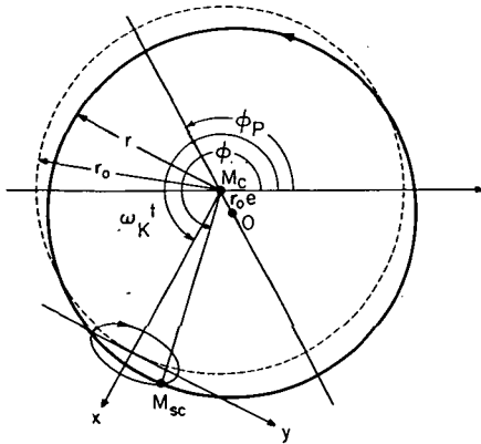
FIGURE 3.3.1.—The guiding-center method of approximating the Kepler motion. The guiding center moves with constant velocity along the dashed circle of radius r_0 in the center of which the gravitating mass M_c is situated. The body M moves in an “epicycle” around the guiding center. The epicycle is an ellipse with the axis
