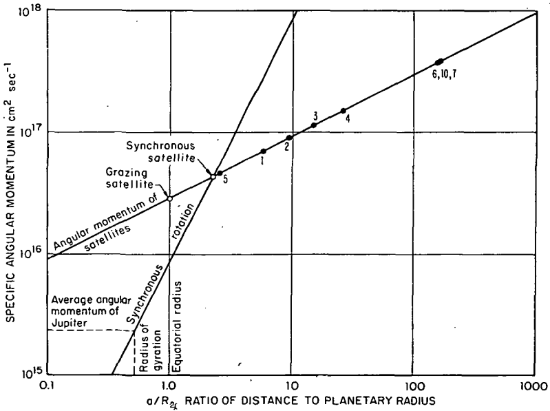
FIGURE 2.3.2.—Specific angular momentum of Jupiter and its prograde satellites.
