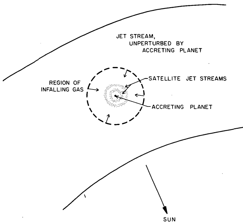
FIGURE 21.4.1.—Qualitative picture of the infall of gas from a jet stream toward a planet. The gas becomes ionized, is brought into partial corotation, and eventually forms satellite jet streams.
