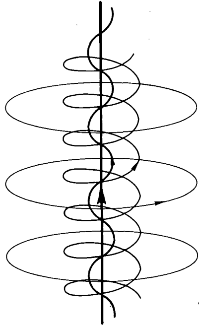
FIGURE 15.3.2.—Simple model of a filamentary current structure in a low-density plasma. Currents flow parallel to the magnetic field. The lines in the figure represent both current paths and magnetic field lines. The magnetic field derives partly from an external axial field and partly from the toroidal field produced by the current itself (see Alfvén and Fälthammar, 1963). The current is strongest at the axis and becomes weaker further away from the axis as depicted by the decreasing thickness of the lines.
