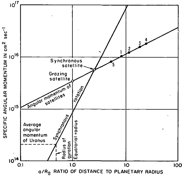
FIGURE 2.3.4.—Specific angular momentum of Uranus and its satellites.
