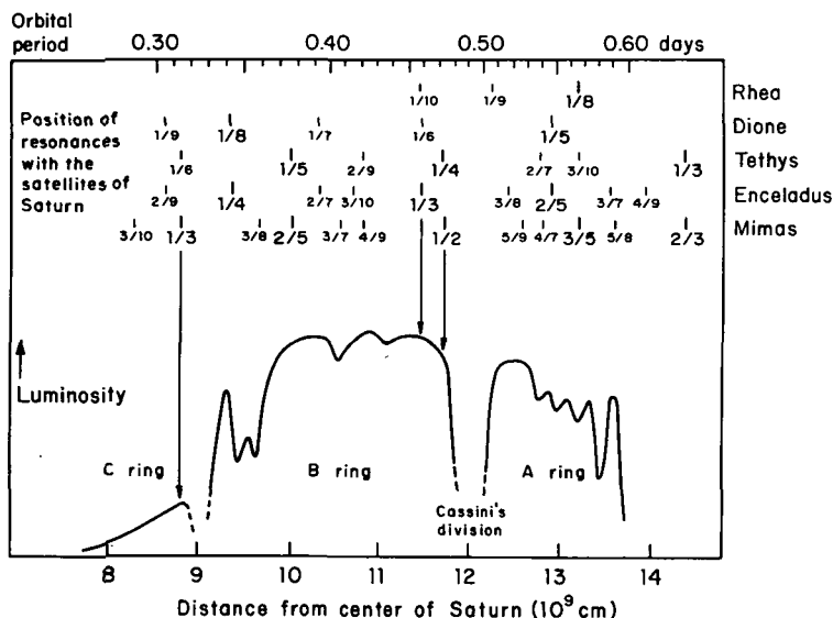
FIGURE 18.6.1.—Photometric curve of the Saturnian rings (according to Dollfus, 1961). The abscissa gives the distance from the center of Saturn in cm. The top scale gives the orbital period of the particles. The periods, which are integral fractions of the periods of the inner Saturnian satellites, are marked in the upper part of the diagram. According to the resonance theory, the density minima in the ring system should be produced by resonance with these satellites. The lack of correlation between low-integer resonances and structural features shows that this is not the case.
