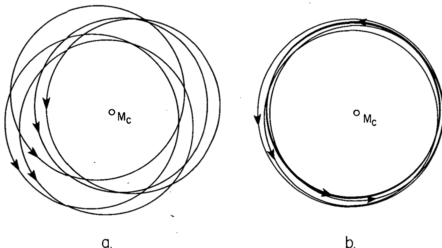
FIGURE 6.6.1.—Interaction of a large number of particles in Kepler orbits (a). In the discussion of collisions between particles in interplanetary space (e.g., evolution of the asteroidal belt or meteor streams) it is usually taken for granted that the state b will evolve into state a (positive diffusion). This is usually not correct. Collisions between the particles will not spread the orbits since the diffusion coefficient is negative (Baxter and Thompson, 1971, 1973). Instead, collisions will lead to equalization of the orbital elements, leading from state a to state b so that a jet stream is formed. (From Alfvén and Arrhenius, 1972.)
