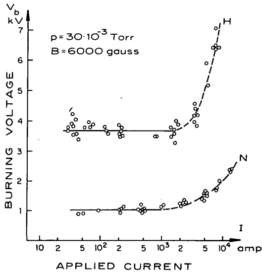
FIGURE 21.8.4.—Burning voltage V_b versus applied current I , for hydrogen and nitrogen in the homopolar experiment. V_b is independent of current (degree of ionization) up to a maximum value related to the complete ionization. The plateau defines the limiting voltage V_{Lm} related to the critical velocity. (From Angerth et al., 1962.)
