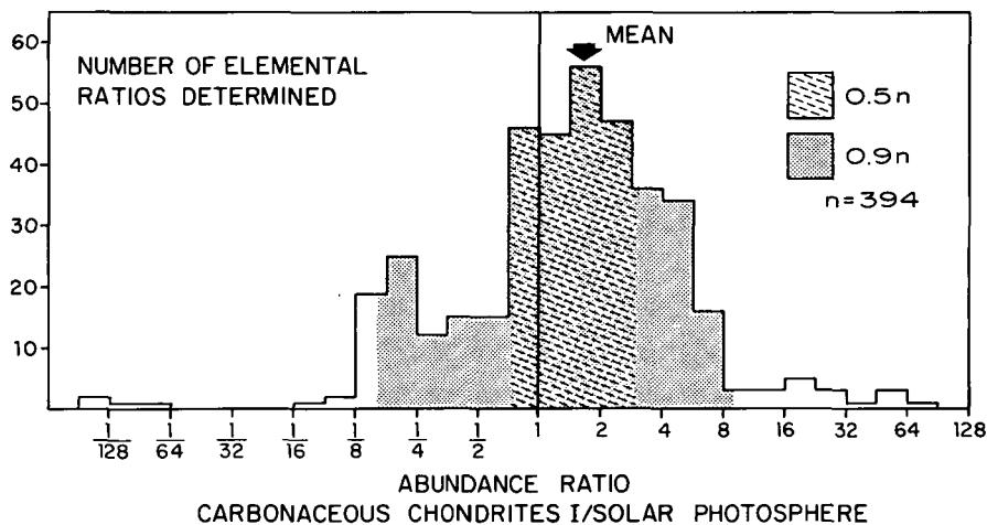
FIGURE 20.6.2b.—Frequency distribution of abundance ratios from fig. 20.6.2a. The diagram shows that on the average there is about 50 percent probability for solar photospheric observations to agree within a factor of five with their meteorite counterparts, and a 90 percent probability for agreement within a factor of 60. Ratios for elements with atomic number \leq 10 are not included in this diagram since they are affected by preferential nuclear instabilities or are highly volatile. Neither are the noble gases included because their abundances in solids are strongly permuted due to volatility and other factors; furthermore their photospheric abundances are not known. Two abundance ratios exceed 128 and are not shown in the graph. Data compiled by L. Shaw.
