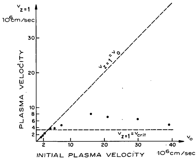
FIGURE 21.8.8.—Plasma deceleration as a function of impinging velocity in the Danielsson experiment. Plasma velocity v_{z=1} in the neutral gas cloud of helium, 1 cm beyond the cloud center, as a function of the initial plasma vacuum velocity v_0 is shown. The critical velocity v_{crit} for helium is indicated. For v_0 less than v_{crit} there was no change in velocity; v_{z=1} = v_0 . For v_0 greater than v_{crit} deceleration was marked; v_{z=1} remained close to v_{crit} . (From Danielsson, 1969b.)
