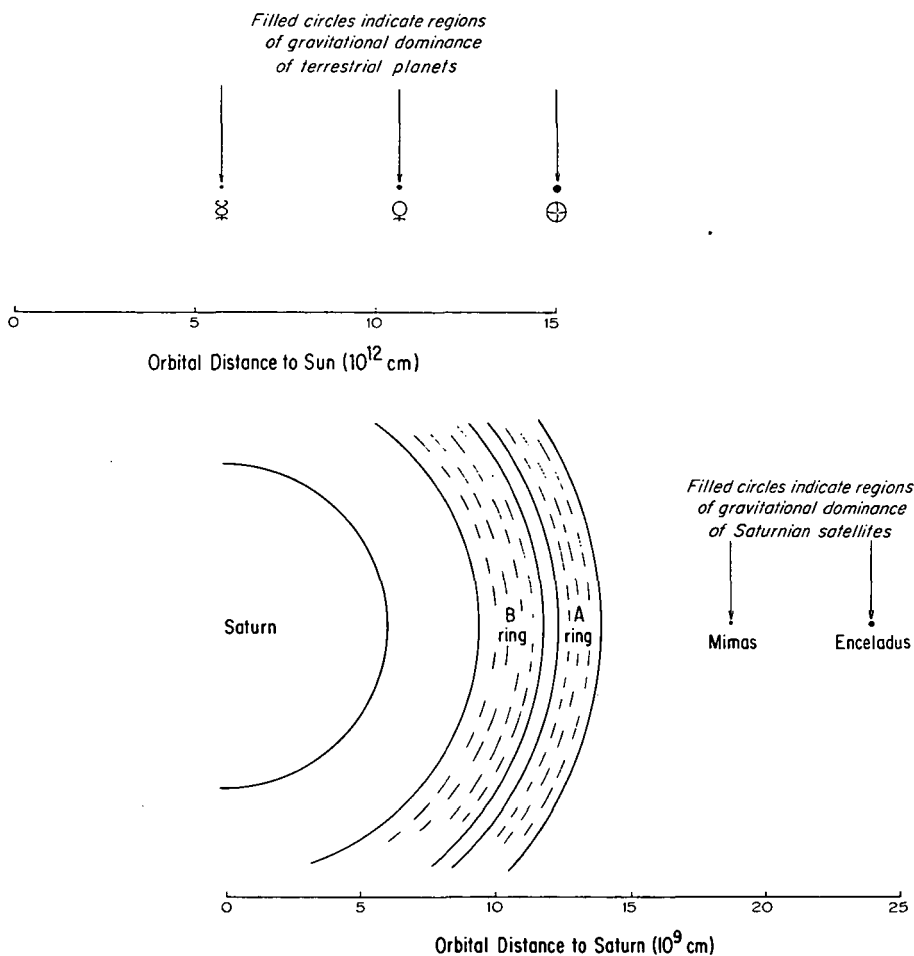
FIGURE 11.2.1. —The inner region of the Saturnian satellite system (below). The small, filled circles (almost points) show the regions within which the gravitational fields of Mimas and Enceladus predominate. The regions of gravitational dominance of the terrestrial planets are shown above. The figure illustrates that gravitational collapse is not a reasonable mechanism for the formation of these bodies because of the minimal extension of their gravitational fields. The same conclusion holds for all satellites and planets, with the possible exception of Jupiter.
