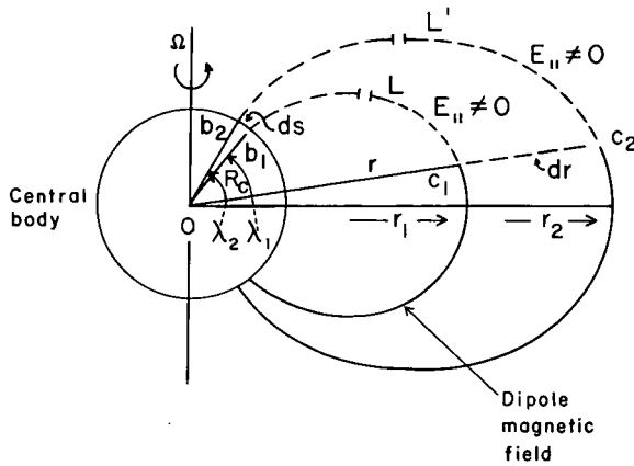
FIGURE 16.3.1.—In the absence of Ferraro isorotation, the angular velocity \omega in the outer regions of the magnetosphere is different from the angular velocity \Omega of the central body. This results in a current flow in the loop b_1b_2c_2c_1b_1 (shown by broken lines) which may result in the electrostatic double layers L and L' . Along part of the paths b_1c_1 and b_2c_2 , the electric field has nonzero parallel components resulting in a decoupling of the plasma from the magnetic field lines.
