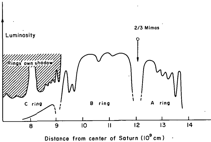
FIGURE 18.6.4.—Heterogenic effects in the Saturnian ring system. Dollfus' photometric profile compared with Mimas' orbital distance reduced by a factor 2/3 (or 0.65). Cassini's division may be the "heterogenic shadow" of Mimas. In the left corner, the photometric profile is turned upside down and reduced by the factor 2/3 ("ring's own shadow"). The rapid drop in intensity between the B ring and C ring coincides with the beginning of this shadow.
