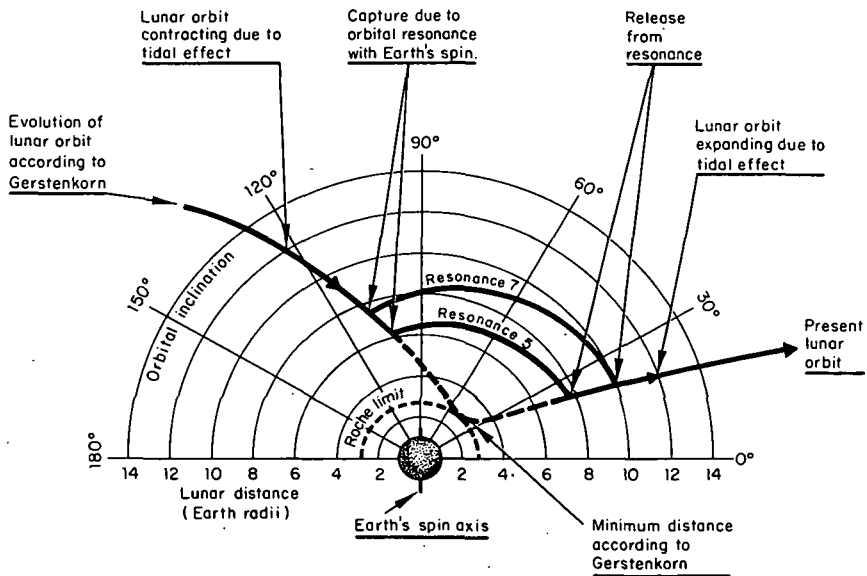
FIGURE 24.5.1. —Noncatastrophic alternative; spin-orbit resonance prevents the Moon from reaching the Roche limit. The retrograde lunar capture orbit contracts due to tidal dissipation until resonance between the lunar orbital period and the spin period of the Earth locks the Moon in a slowly expanding orbit. Since the Moon never comes very close, no breakup or autoejection of debris occurs and the tides do not reach catastrophic heights. When the orbital inclination has decreased below a critical angle (suggested in the diagram at about 25^\circ ), the resonance locking is broken and the Moon recedes to its present orbit at 60 Earth radii. The dotted curve represents the catastrophic alternative (Moon reaching the Roche limit). (From Alfvén and Arrhenius, 1969.)
