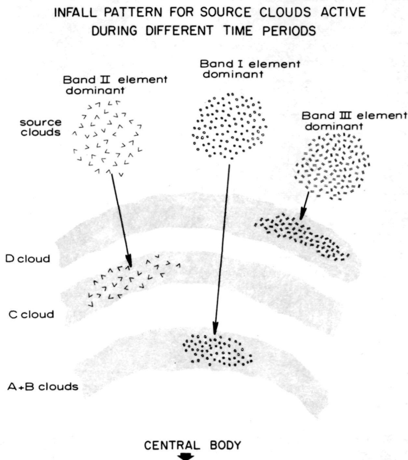
FIGURE 21.12.1. —Infall pattern for source clouds active during different time periods. The infalling gas from one source cloud will be dominated by one element. The mass of infalling gas will be stopped when the dominant element is ionized; i.e., in the cloud corresponding to the critical velocity value of that element's band. For example, a Band II element reaches its critical velocity at a value r_{ion} which falls within the C cloud.
