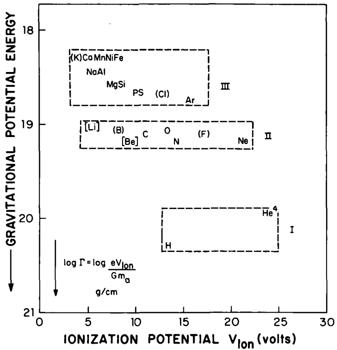
FIGURE 21.5.1.—The gravitational energy \Gamma and ionization potential of the most abundant elements. Roman numerals refer to row in the periodic table, with “III” including the fourth row. All elements in a band have approximately the same gravitational energy and v_{ion} , as discussed in secs. 21.4 and 21.5. Minor and trace elements are indicated, respectively, by parentheses and brackets.
