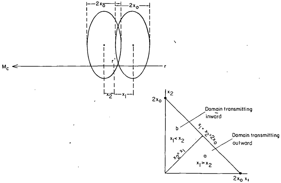
FIGURE 6.7.1.—Simple model of negative diffusion. The region of collision is shown (above) for two particles, one with guiding center at x_1 = r - r' and another with guiding center at x_2 = r' - r . Both particles are oscillating radially with amplitude x_0 . In the x_1x_2 diagram (below) collisions can take place if x_1 + x_2 is located inside the triangle. If a perfectly inelastic collision takes place in the domain a the guiding center at x_2 is transmitted outward through r' . If the collision takes place in domain b , a similar inward transmission of the guiding center at x_1 takes place. If the density increases with r , the collision frequency is larger in domain a than in domain b , with the result that the diffusion goes outward; i.e., toward the higher density region. Hence the diffusion coefficient is negative .
