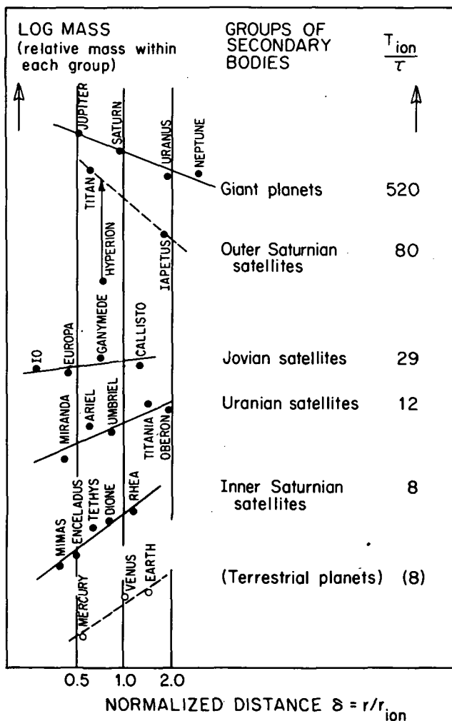
FIGURE 23.6.1.—Mass distribution within the groups of secondary bodies as a function of their normalized distances \delta = r/r_{ion} . The figure shows that within a group characterized by a large value of T_{ion}/\tau , the mass decreases outward. For a value of T_{ion}/\tau which is small, the mass decreases inward. (From Alfvén, 1962.)
