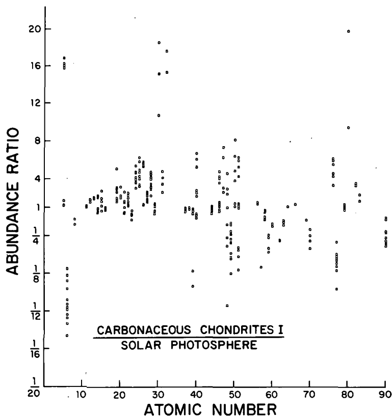
FIGURE 20.6.2a.—Comparison of solar photospheric abundance estimates with measurements on carbonaceous meteorites of Type I. Each analytical chondrite value, normalized to silicon, has been divided by each of the several current photospheric values. Four of the ratio values for mercury ( Z=80 ) exceed 20 and are not shown in the diagram. Data compiled by L. Shaw. It has commonly been assumed that these two materials can be regarded as splits from a chemically homogeneous body “the solar nebula” having “cosmic abundances” of elements. Except for components with high vapor pressures or nuclear instabilities the compositions of these meteorites and of the solar photosphere then ought to approach identity, and the elemental abundance ratios should be close to 1. The strong scatter of data in the figure shows, however, that they do not provide a basis for the assumption of a close agreement between the solar photosphere and this group of meteorites (see also fig. 20.6.2b).
