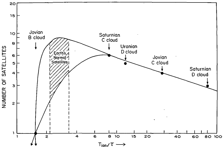
FIGURE 24.3.2.—Number of bodies in a satellite group is a function of T_{ion}/\tau (where \tau is the spin period of the central body and T_{ion} is a characteristic orbital period of the bodies in the group (sec. 23.5)). The groups of satellites are the outermost Saturnian satellites (Saturnian D cloud), Galilean satellites (Jovian C cloud), Uranian satellites (Uranian D cloud), inner Saturnian satellites (Saturnian C cloud), and innermost Jovian satellites (Jovian B cloud). Assuming that the Earth's satellite system would fall into the pattern established by these groups of satellites, the Earth may once have had just a few or as many as 9 or 10 normal satellites. (From Alfvén and Arrhenius, 1972a.)
