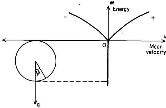
FIGURE 8.2.1.—Oscillations of a simple pendulum. If the energy is negative, the pendulum oscillates with an amplitude \psi_1 < \pi , and the mean velocity d\psi/dt is zero. If the energy is positive the motion consists of a constant revolution modulated by an oscillation of the same period. The angular velocity \omega of this revolution may be either positive or negative.
