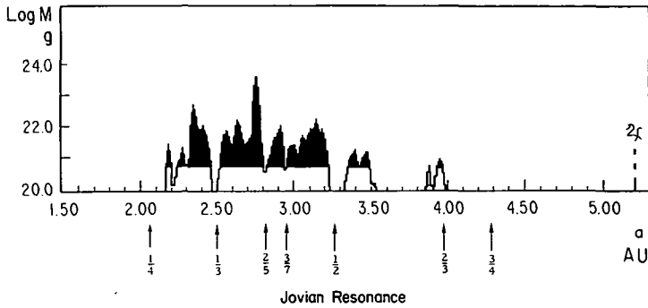
FIGURE 4.3.4.—The (M, a) diagram (mass of asteroids in g per 0.01 AU as a function of semimajor axis a in AU). To stress the logarithmic scale, the region of greatest mass density is shaded. These regions contain practically all the mass in the asteroid belt. Mass was calculated from magnitude using eq. (4.3.3). The diagram includes data for all asteroids of a < 5.0 AU listed in the Ephemerides of Minor Planets for 1968. The resonances are indicated as the ratio of the orbital period of a body at a specific value of a to the orbital period of Jupiter. The Kirkwood gaps correspond to the \frac{1}{3} , \frac{2}{3} , \frac{3}{7} , and \frac{1}{2} resonances. (From Alfvén et al., 1974.)
