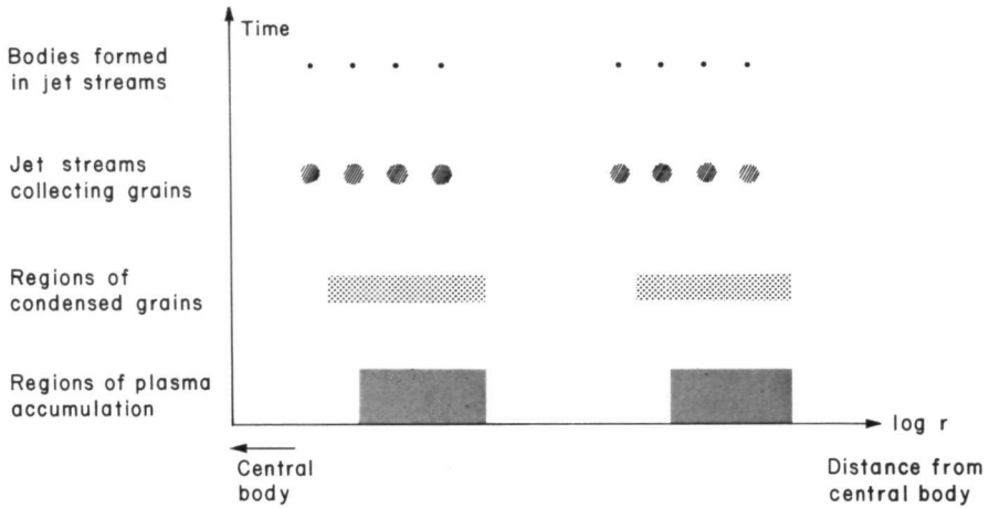
FIGURE 18.10.1.—Diagram of the formation of a group of bodies. Infalling gas is stopped and ionized at different distances from the central body. The two regions in the figure may receive plasma simultaneously or during different epochs. Condensation of the plasma is rapid during the total infall period. Condensed grains are collected in jet streams which increase their mass during the whole infall period. Grains are stored in the jet streams as single particles and embryos (often for a long period of time) until they are finally accreted by the largest embryo. In each region of plasma infall, 3–5 bodies are formed.
