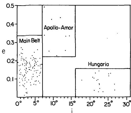
FIGURE 4.4.1.—The inner region of the asteroid belt ( a < 2.2 AU) The main-belt asteroids ( 2.0 < a < 2.2 ) have small eccentricities and inclinations; the Apollo-Amor asteroids, higher inclinations and eccentricities; and the Hungaria asteroids ( 1.8 < a < 2.0 ), high inclinations but small eccentricities. Data from the Ephemerides of Minor Planets for 1968.
