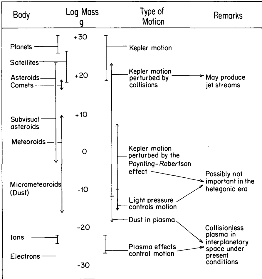
FIGURE 5.1.1.—Survey of forces governing the motion of bodies in space.
