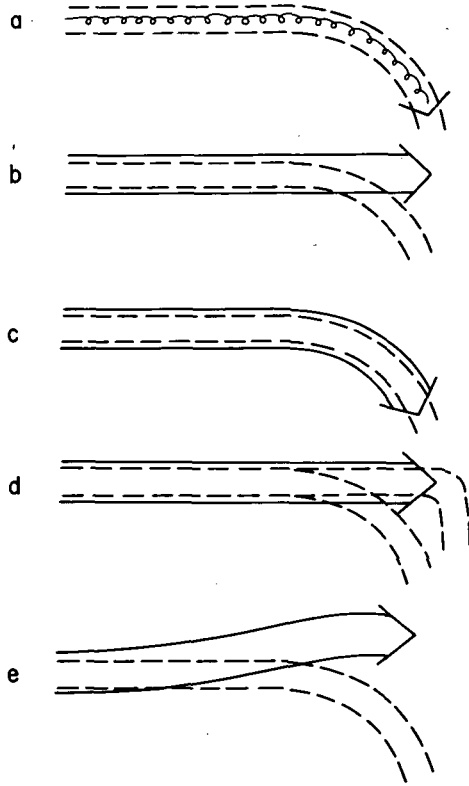
FIGURE 15.3.4.—(a) In a magnetic field which has a downward bend, charged particles shot parallel to the field will follow the bend. If instead a plasma beam is shot, one would expect either that it (b) produces an electric polarization so that it can continue along a straight line, (c) follows the bend as in (a), or (d) continues to move straight forward bringing the “frozen-in” field lines with it. (e) In the quoted experiment the plasma does not obey any of these theories; instead, the plasma bends in the opposite direction to that of the magnetic field. In hindsight, this is easily understood as being due to an electric field transmitted backward by fast electrons (Lindberg and Kristoferson, 1971.)
