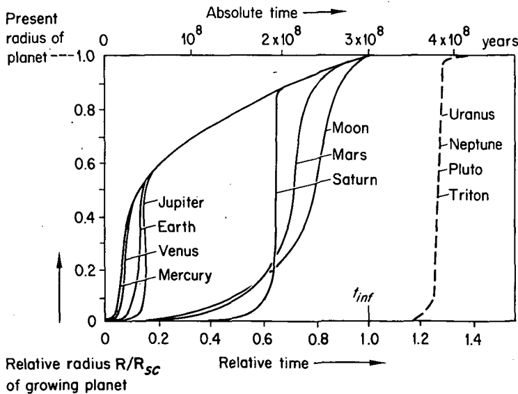
FIGURE 12.9.1.—The growth of planetary radii with respect to time. Runaway accretion occurs early for Mercury, Venus, Earth, and Jupiter. The time of runaway accretion approaches that of the duration of mass infall for Saturn, Mars, and the Moon. (From Ip, 1974c.) For Uranus, Neptune, Pluto, and Triton, runaway accretion occurs only after infall has ceased and the jet stream has contracted due to negative diffusion; this growth is schematically represented by the dashed curve.
