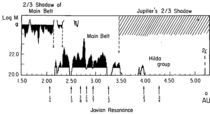
FIGURE 18.8.1. —The smoothed (M, a) diagram of fig. 4.3.4. Mass distribution in units of grams per radial distance interval of \Delta a = 0.01 AU. To emphasize the significance of the log scale, high-density regions are darkened. In analogy with fig. 18.6.4, the diagram, diminished by a factor 2/3 and turned upside down, is shown in the upper part of the diagram demonstrating the “hetegonic shadow” effect which produces the inner cutoff of the asteroidal belt. Similarly Jupiter’s shadow, which generates the outer cutoff, is shown, as well as the position of Jupiter. Kirkwood gaps from Jovian resonances are also marked. (From Alfvén et al., 1974.)
