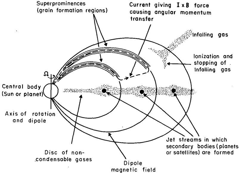
FIGURE 16.6.1.—A sketch of the series of hetegonic processes leading to formation of secondary bodies around a spinning magnetized central body (not drawn to scale). The dipole magnet is located at the center of the central body and is aligned with the spin axis. The gas falling from “infinity” into the environment of the central body becomes ionized by collision with the magnetized plasma when its free-fall velocity exceeds the critical velocity for ionization, and the ionized gas then remains suspended in the magnetic field. The rotation and magnetic field together with the conducting plasma surrounding the central body give rise to a homopolar emf which causes a current flow in the plasma. This current I together with the magnetic field B give rise to a force I \times B which transfers angular motion from the central body to the surrounding plasma. The current also produces prominence-like regions of gas (by pinch effect) which are denser and cooler than the surrounding regions, and in these regions the condensation of grains takes place. Through viscous effects, the population of grains evolves into a number of jet streams while the noncondensable gases form a thin disc in the equatorial plane.
