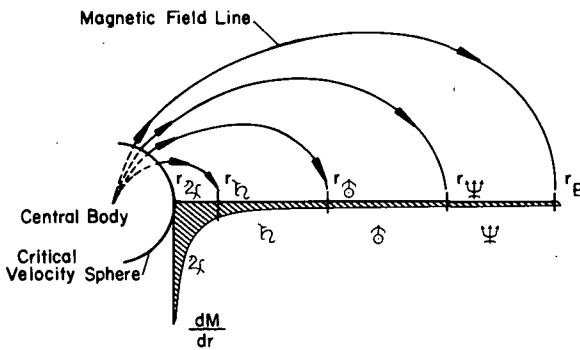
FIGURE 23.2.2.—Matter stopped at the critical velocity sphere is displaced outward along the magnetic field lines and condenses in the region of the equatorial plane. For a rough estimate it is assumed, rather arbitrarily, that all matter between the present orbits of Jupiter and Saturn is now included in Jupiter, etc. As shown by table 23.2.1, this gives roughly the observed mass distribution. The essence of the analysis is that the distributed density in the region of the giant planets is compatible with the model of sec. 23.2. (From Alfvén, 1962.)
