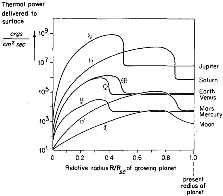
FIGURE 12.11.1.—Thermal profiles of the growing planets. (From Ip, 1974c.)
