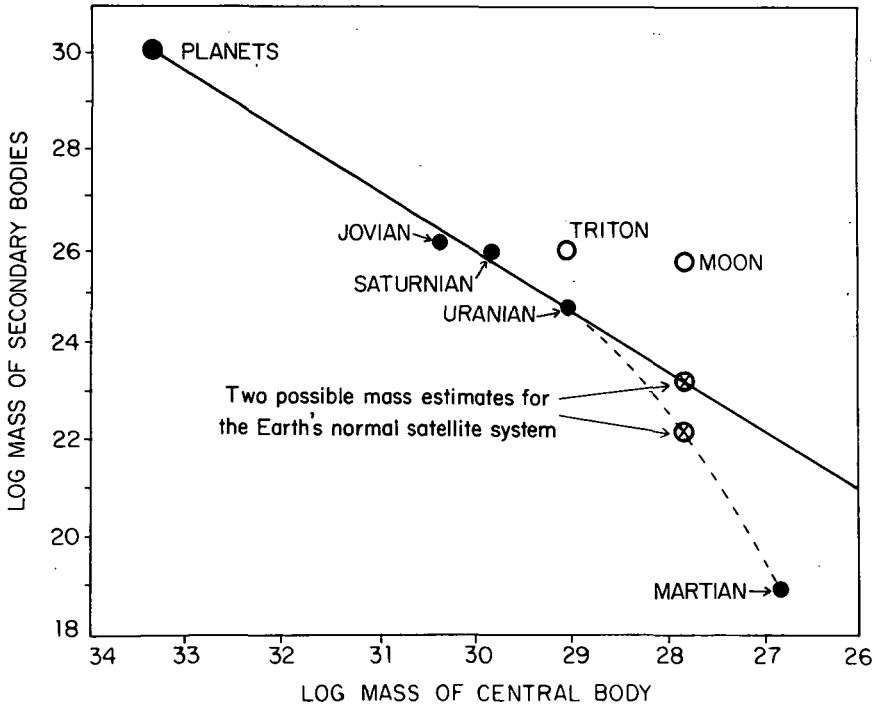
FIGURE 24.3.1.—Total mass of secondary body systems as a function of central body mass. Both Triton and the Moon have much larger masses than expected of normal satellites. Two possible mass estimates for a normal Earth satellite system are shown, one based on an extrapolation from the systems of Jupiter, Saturn, and Uranus, and the other, an interpolation also including the Martian satellite system. (From Alfvén and Arrhenius, 1972a.)
