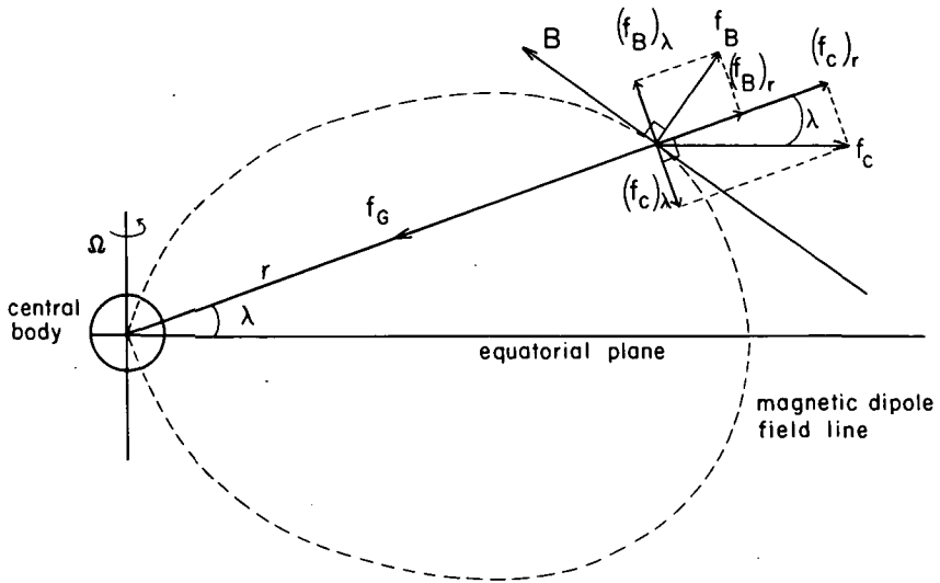
FIGURE 17.2.1.—Partial corotation. Equilibrium between gravitational force f_G , centrifugal force f_c , and electromagnetic force f_B implies that f_G + f_c + f_B = 0 . Because (f_c)_\lambda + (f_B)_\lambda = 0 , the geometry of the magnetic dipole field requires that (f_c)_r = 2(f_B)_r = 2/3(-f_G) . (From Alfvén et al., 1974.)
