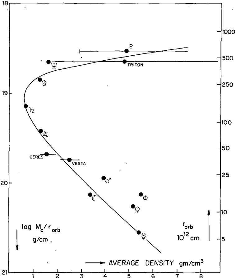
FIGURE 20.7.1a.—Average density of planets and former planets as a function of orbital distance r_{orb} from the Sun. The guideline through the population of density points is intended for intercomparison of this figure with figs. 20.7.1b and c. The ordinate is also given in terms of gravitational potential energy (mass, M_c , divided by orbital radius, r_{orb} ); this makes it possible to directly compare the distribution of satellites with that of the planets. The gravitational potential energy is also a parameter which enters in an important manner in the discussion of the critical velocity phenomenon (see chs. 21 and 23). Since the Moon and Triton are captured planets, the Sun is regarded as their central body. Hence the Moon and Triton have the approximate gravitational potential energy of the Earth and Neptune, respectively. The horizontal lines through the points for Ceres, Vesta, Triton, and Pluto indicate the estimated range of uncertainty, with the vertical bar designating the lower limit for the density of Pluto as discussed in the text. Data from table 20.5.1.
