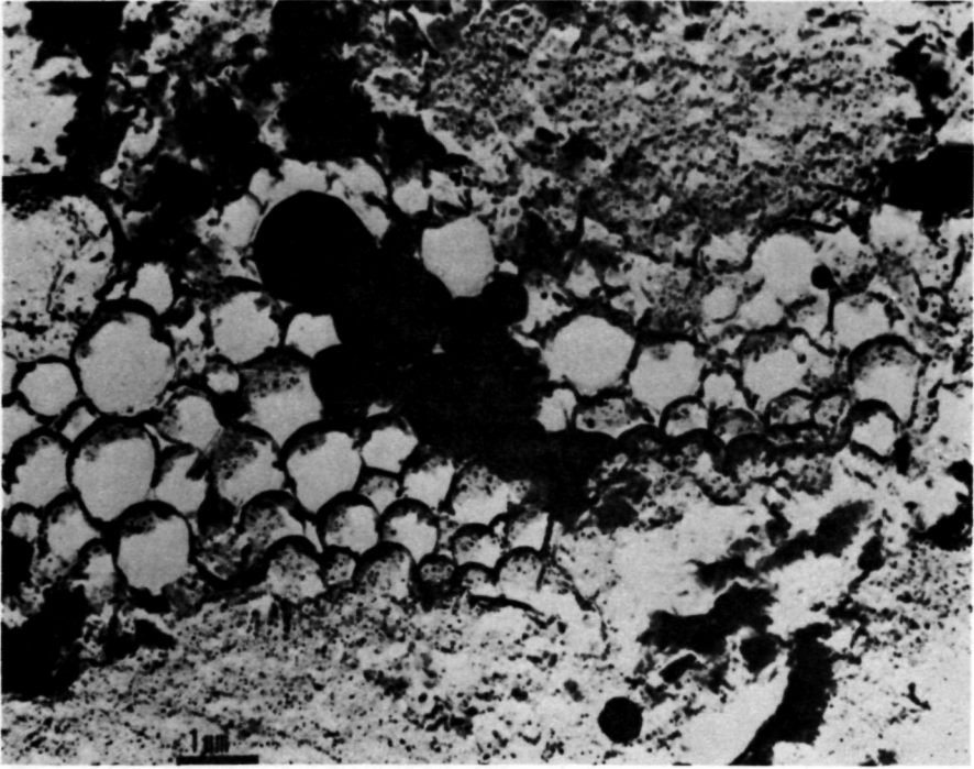
FIGURE 22.7.1. —Section through a cluster of spheroidal magnetite crystals in the carbonaceous chondrite Orgueil. (From Kerridge, 1970; replica electron micrograph.) Assuming that the cluster is as high as it is wide, it consists of at least a thousand spheroids. Each of these spheroids appears to be a single magnetite crystal with a faceted surface. The crystals are easily detachable from each other and are presumably held together magnetically. Loosely bonded clusters like these are likely to have accumulated at orbital relative velocities of the individual spheroids in the range below 10–100 m/sec.
