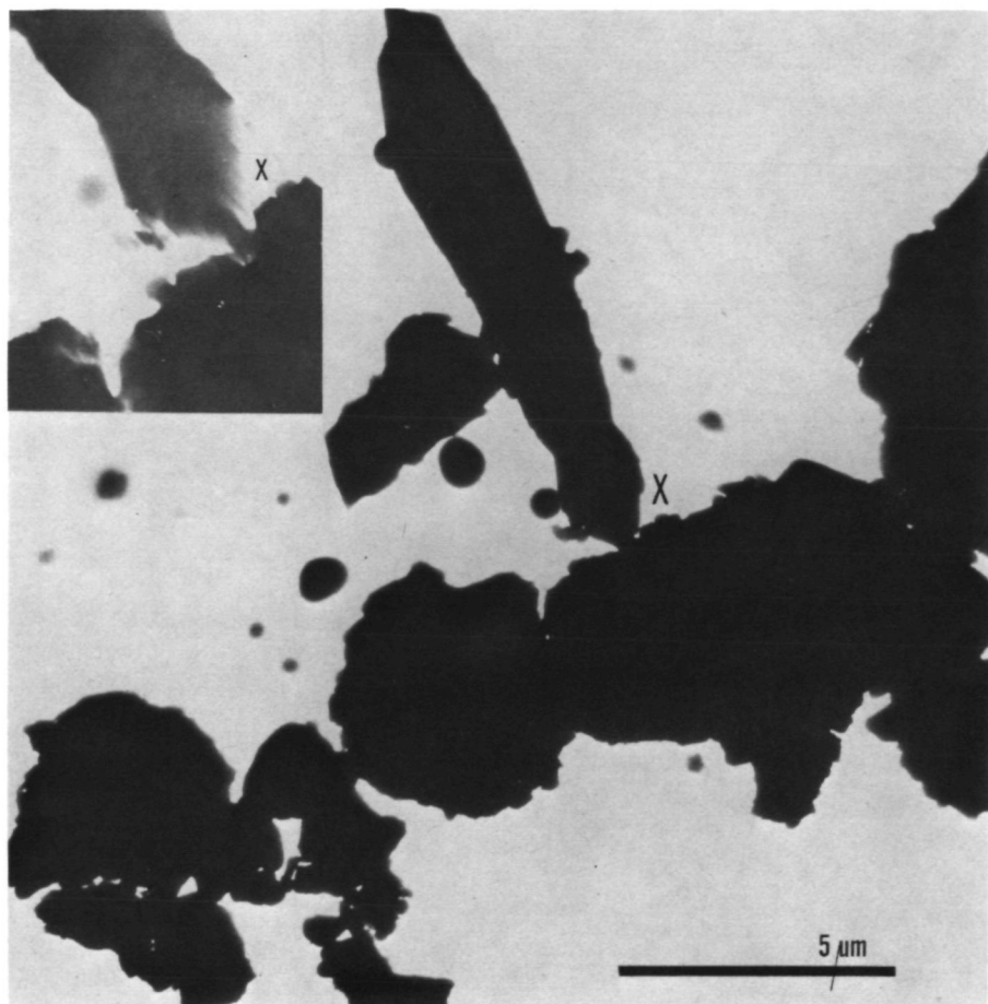
FIGURE 7.4.1.—Head-on contacts of elongated grains are characteristic of particle clustering in lunar soil caused by electrostatic field effects. Analysis of these effects indicates that they are due to persistent internal polarization of the dielectric grains, induced by irradiation. (From Arrhenius and Asunmaa, 1973.)
