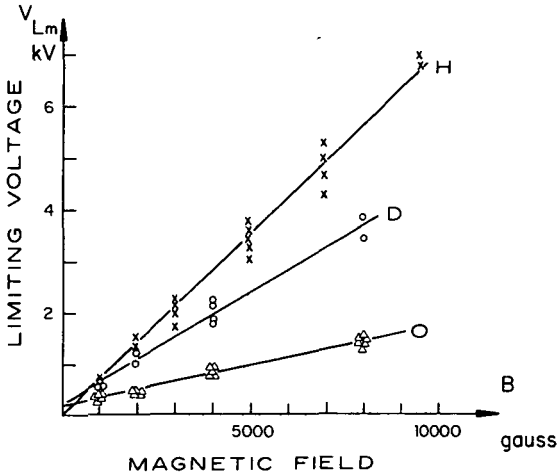
FIGURE 21.8.3.—Limiting voltage V_{Lm} versus the magnetic field B in the homopolar experiment. V_{Lm} is proportional to B and depends also on the chemical composition (O, D, H) of the gas being studied. (From Angerth et al., 1962.)
