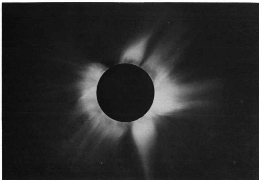
FIGURE 20.6.1—Coronal streamers, visible at solar eclipse. The photograph illustrates the inhomogeneous nature of emission of solar material. Homogeneous models of the Sun are often completely misleading.
