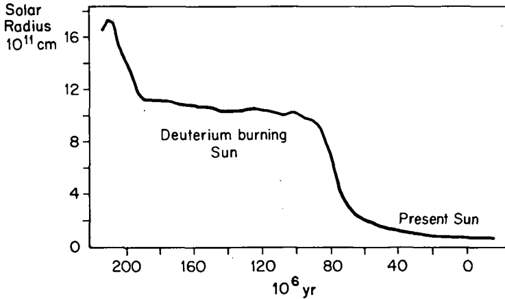
FIGURE 25.6.1.—The Brownlee-Cox model of solar evolution through a deuterium-burning stage. Under the assumptions that the initial content of deuterium corresponds to the deuterium/hydrogen ratio of the Earth and that the energy transport in the deuterium-burning Sun is nonconvective, the radius of the Sun would have remained at about 16 times the present value during the deuterium burning. This stage would last about 10^8 yr before contraction to the present size. A different initial content of deuterium (which is possible) would mainly change the duration of the deuterium-burning stage. (From Brownlee and Cox, 1961.)
