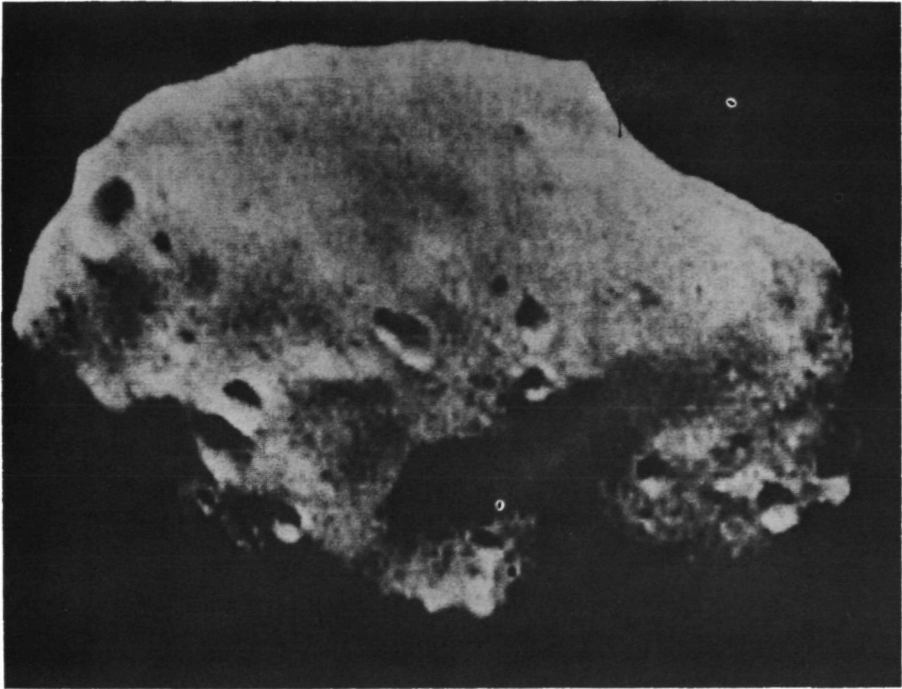
FIGURE 20.4.1.—Impact cratering of the Martian satellite Phobos. In suitable illumination craters such as A above can be seen to have rims of substantial height above the surrounding terrain. Since ejecta with velocities exceeding a few meters per second will leave the satellite, the crater cones cannot be generated by fallout from the impact as is the case on Earth, Mars, and the Moon. The dimensions of the cones also appear larger than the elevation of crater rims observed on the Earth as a result of shock rebound. A possible explanation of this phenomenon is that Phobos, or at least its outer regions, consists of aggregate material with low bulk density, and that impacting projectiles dissipate their energy largely below the target surface. (NASA Photograph 71-H-1832.)
