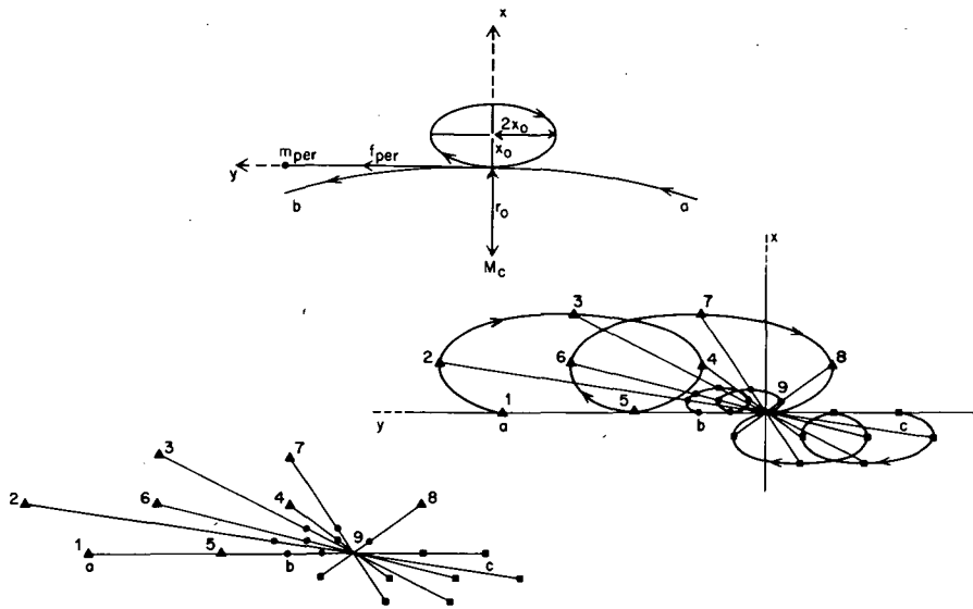
FIGURE 6.4.1.—Longitudinal apparent attraction. A particle initially moving along the arc ab with radius r_0 is suddenly perturbed by a tangential gravitational force f_{per} due to the mass m_{per} . The new motion consists of a retrograde epicycle motion in an ellipse, the center of which ("guiding center") moves in a circle with radius r_0 + x_0 (above). The perturbed motion of three particles, originally situated at a , b , and c , describes three epicycles (right). The numbers 1 through 9 indicate the positions of the particles at intervals of (T_K/4) . The unperturbed particles form the line abc (left). The perturbation makes this line turn and first lengthen and then shorten. The quantity n in eq. (6.4.16) is equal to 2 in this case and consequently after the time 2T_K has elapsed all particles simultaneously arrive at the point x=0, y=0 . Hence there is a longitudinal apparent attraction of the particles to the guiding center of the unperturbed motion. (From Alfvén, 1971.)
