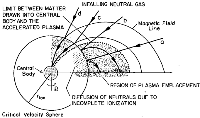
FIGURE 23.3.1.—Partial ionization of infalling gas. Small values of T_{ion}/\tau ( <20 ) imply an increase of the region near the axis of the central body from which matter is drawn into the central body. Incomplete ionization at r_{ion} is also implied and diffusion of neutral gas toward the central body will take place. The result is a displacement inward of the region of plasma emplacement and a change in the mass distribution within a group of secondary bodies.
