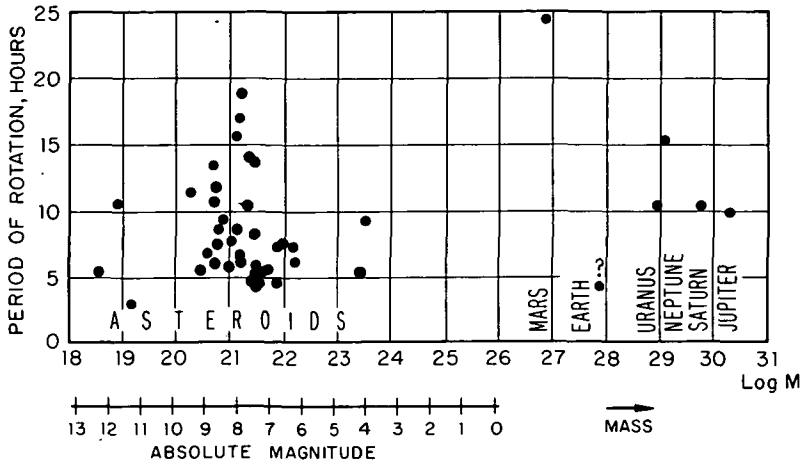
FIGURE 9.7.1.—Periods of axial rotation for some asteroids and some of the planets in relation to their masses. (From Alfvén, 1964.) The rotation period of Pluto is not well known and the rotation periods of Mercury and Venus are influenced by resonance effects; these three planets are thus not represented in the figure. The value of rotation period for the Earth is that prior to capture of the Moon. Data for asteroids is taken from table 9.7.1 and data for the planets from table 2.1.1. From the graph one concludes that spin period is not a function of mass. Indeed, most of the spin periods all fall within a factor of two of 8 hr. We refer to this similarity of periods of rotation as the law of isochronous rotation or the isochronism of spins.
