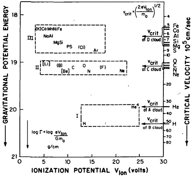
FIGURE 21.11.1.—Critical velocity and ionization potential of the most abundant elements. The left-hand ordinate showing gravitational potential energy \Gamma and the right-hand ordinate showing the critical velocities of the controlling elements of the A, B, C, and D clouds allow a comparison of \Gamma values and v_{crit} values.
