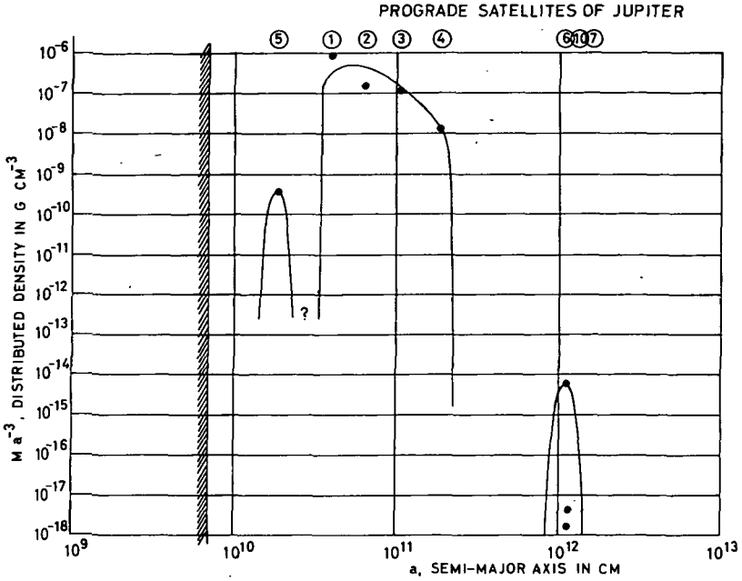
FIGURE 2.5.2.—Distributed density versus semimajor axis for the prograde satellites of Jupiter.
