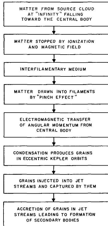
FIGURE 16.7.1.—Sequence of processes leading to the formation of secondary bodies around a central body.
