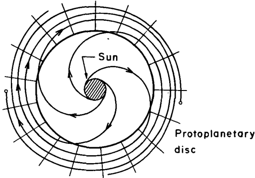
FIGURE 15.6.1.—Schematic representation of Hoyle's theory. According to Hoyle (1960), the rotation of the primeval Sun would have produced highly spiralized magnetic field lines both in the Sun and in its surroundings. The figure shows only five turns but Hoyle's theory requires 100 000 turns storing an energy of 5 \times 10^{45} ergs. Hoyle claims that this magnetic energy caused the protoplanetary disc to expand and form the planetary system. If Hoyle's mechanism were physically reasonable, it would have had important technological applications. But as shown both theoretically (Lundquist, 1951) and experimentally (Lindberg et al., 1960; see also fig. 15.3.3), such a configuration is unstable and can never be achieved.
