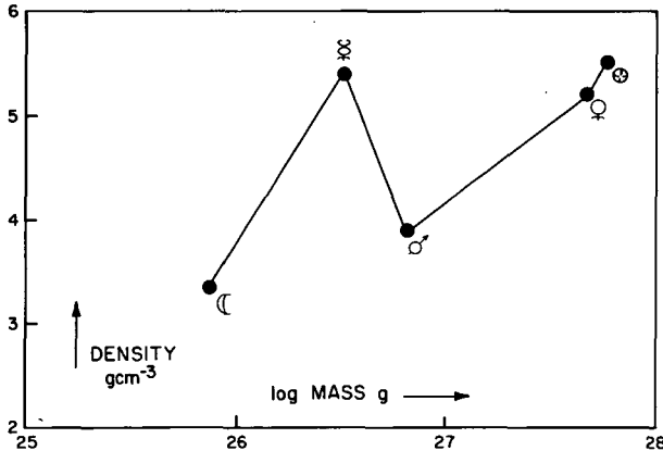
FIGURE 20.5.1.—Density of the terrestrial planets as a function of their mass. A smooth curve could be drawn through Moon-Mars-Venus-Earth indicating that all may have a similar composition. This would require the assumption that Moon-Mars-like material can be compressed to the high core densities indicated ( \sim 15\text{--}17 \text{ g/cm}^3 ) at the core pressures of Venus and the Earth ( \sim 1.5 \text{ Mb} ). But it is also possible that Moon and Mars have a heavy element content entirely different from that of Earth-Venus. The composition of Mercury must in any case be different from all the other bodies.
