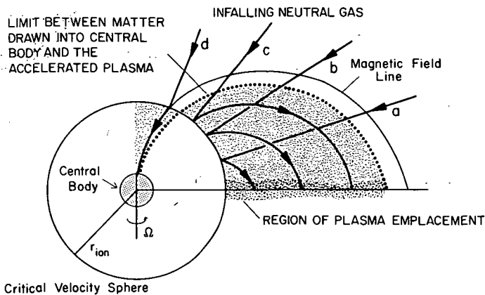
FIGURE 23.2.1.—Complete ionization of infalling gas. Gas falling in from infinity reaches the critical velocity at r_{ion} (the critical velocity sphere) and becomes partially ionized. It is rapidly included in “superprominences” which, if \zeta T_{ion}/\tau \gg 1 , are almost completely ionized. Matter falling in at low latitudes ( a , b , and c ) will be emplaced near the equatorial plane and condense there. Matter arriving at the critical velocity sphere at high latitudes ( d ) will be drawn into the central body. Note that the processes a , b , and c do not necessarily interfere because they may occur at different times or even simultaneously at different longitudes.
