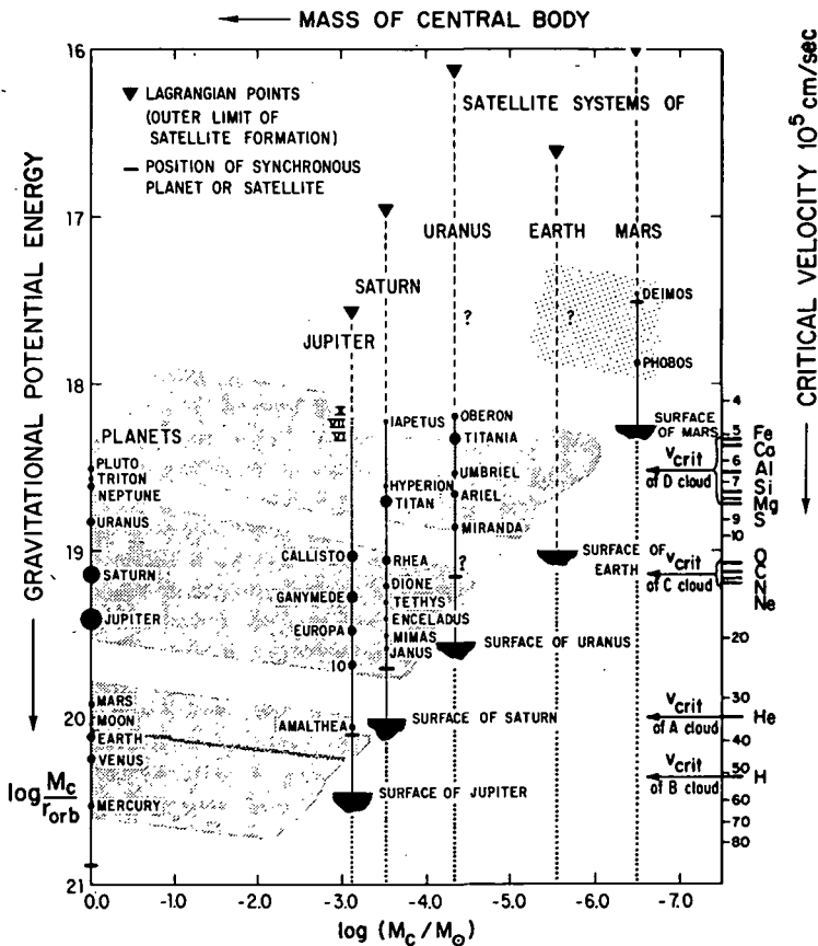
FIGURE 21.11.2.—Gravitational potential energy \Gamma as a function of the mass of the central body for the planetary and satellite systems. The right-hand ordinate showing critical velocity affords comparison of \Gamma values for the planets and satellites with v_{crit} values for abundant elements and the A, B, C, and D clouds.
