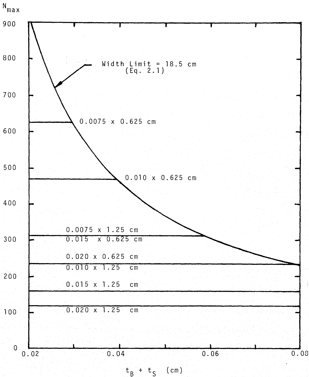
FIGURE 5 MAXIMUM NUMBER OF BLADES AS A FUNCTION OF BLADE AND SPACER THICKNESS AND BLADE CROSS SECTIONS
