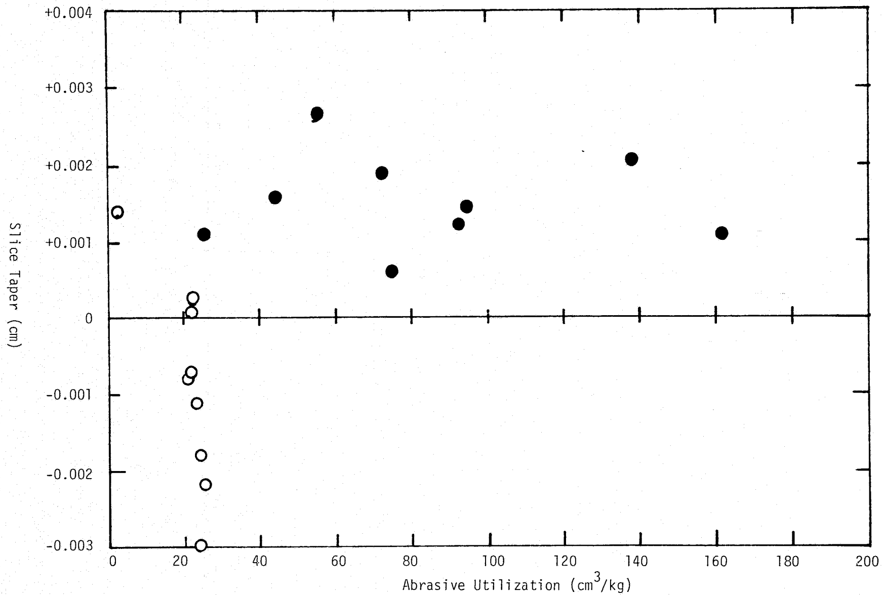
FIGURE 22 SLICE TAPER AS A FUNCTION OF ABRASIVE UTILIZATION
