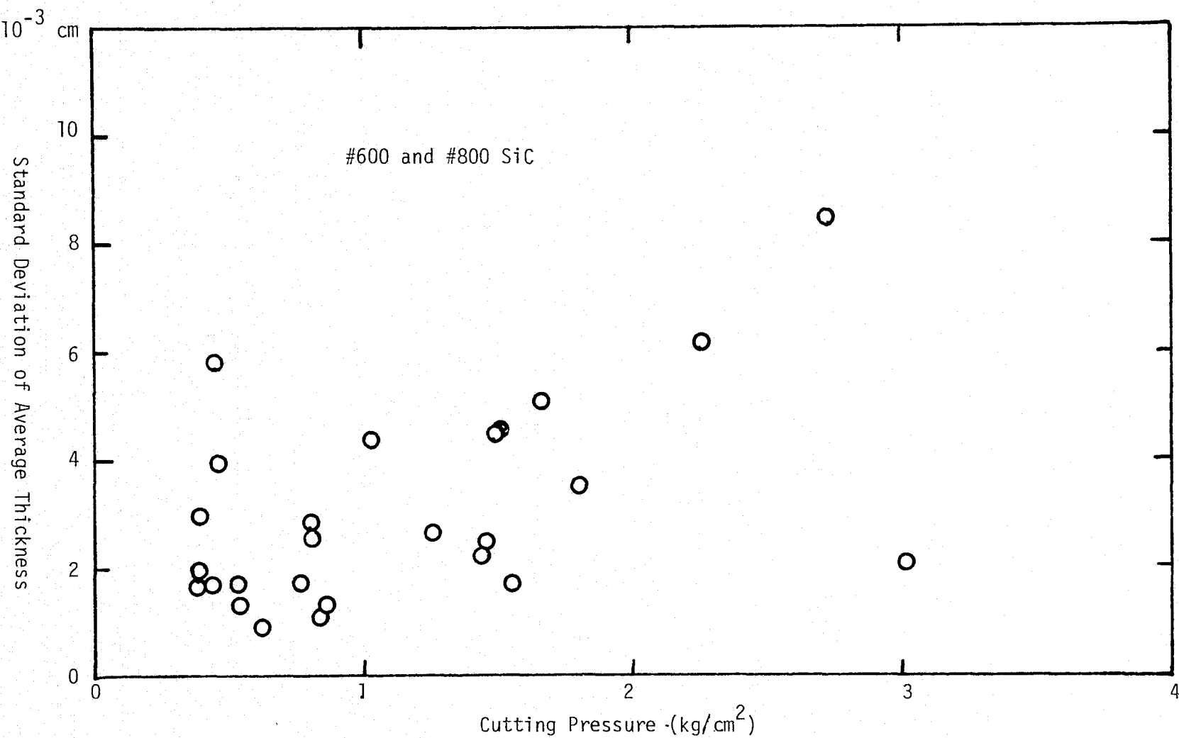
FIGURE 21 THICKNESS ACCURACY AS A FUNCTION OF CUTTING PRESSURE
