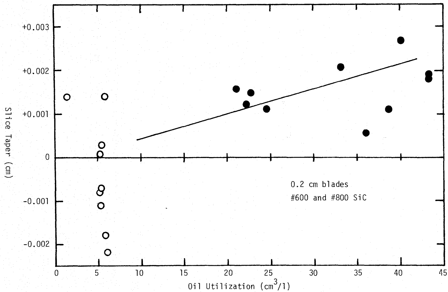
FIGURE 23 SLICE TAPER AS A FUNCTION OF OIL UTILIZATION
