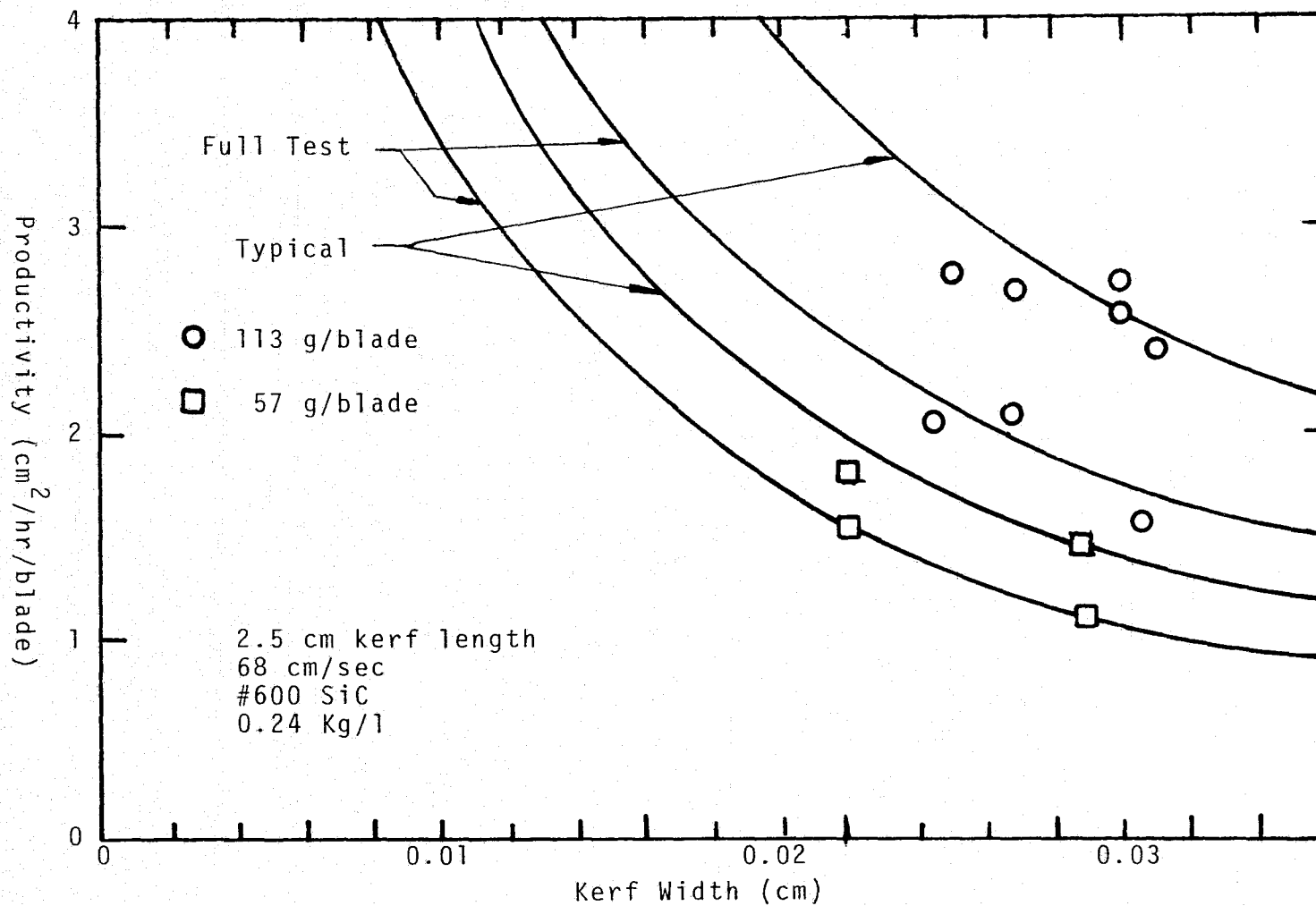
FIGURE 11 PRODUCTIVITY FOR VARIOUS KERF WIDTHS
