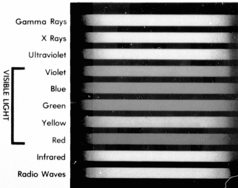
Figure 2. The radiation spectrum. The central part illustrates the visible light spectrum of the Sun with bands from the ultraviolet to the red. If we had a device that would record the spectrum of all radiation, not just visible light, there would be many bands of other "colors" above and below the familiar colors. This "extra" radiation constitutes the gamma rays, X rays, ultraviolet, infrared, and radio waves as indicated schematically. Visible light is actually a minute fraction of the total radiation spectrum.
