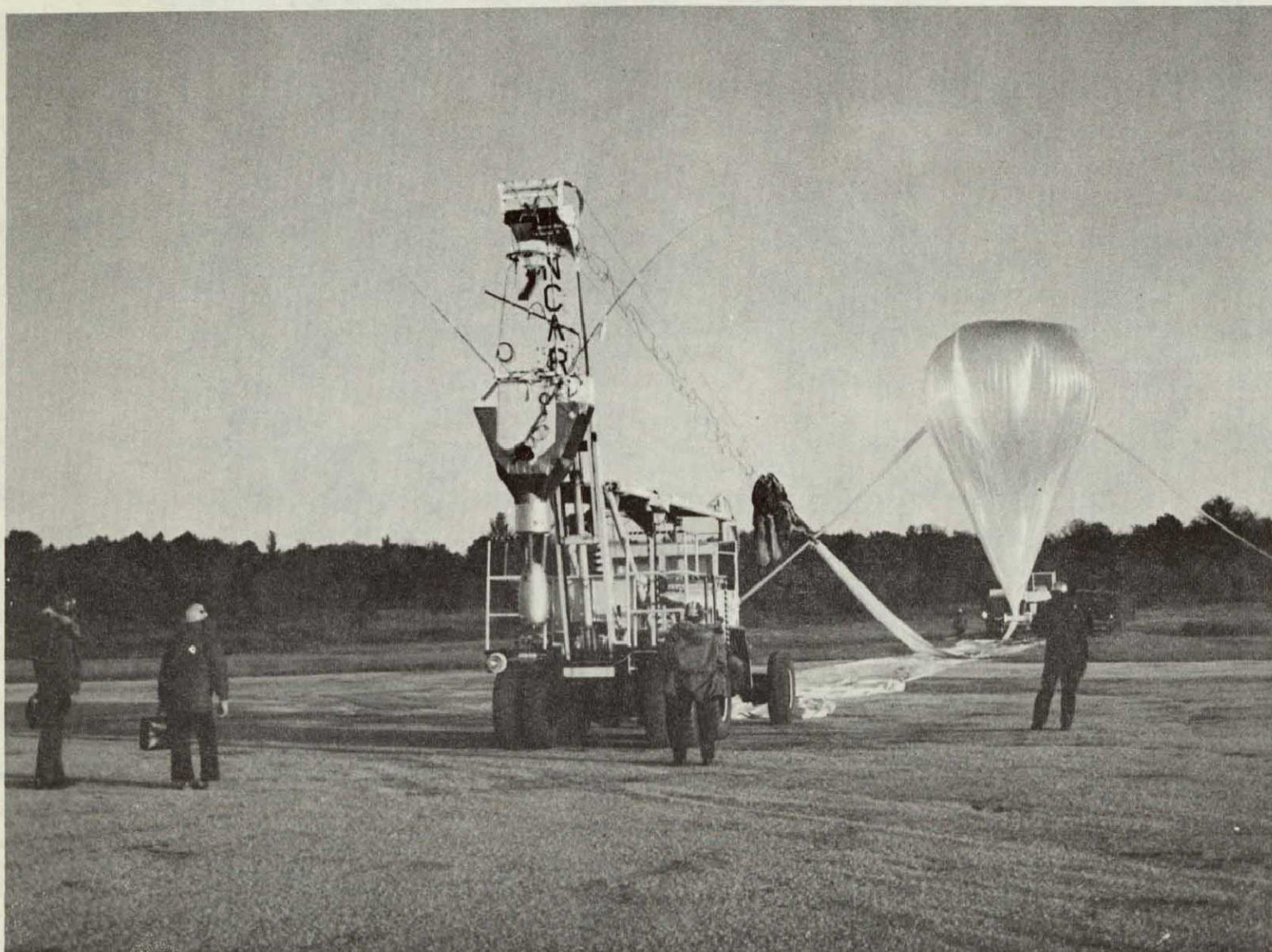
7 Figure 2. - Payload ready for flight with balloon being inflated in the background
