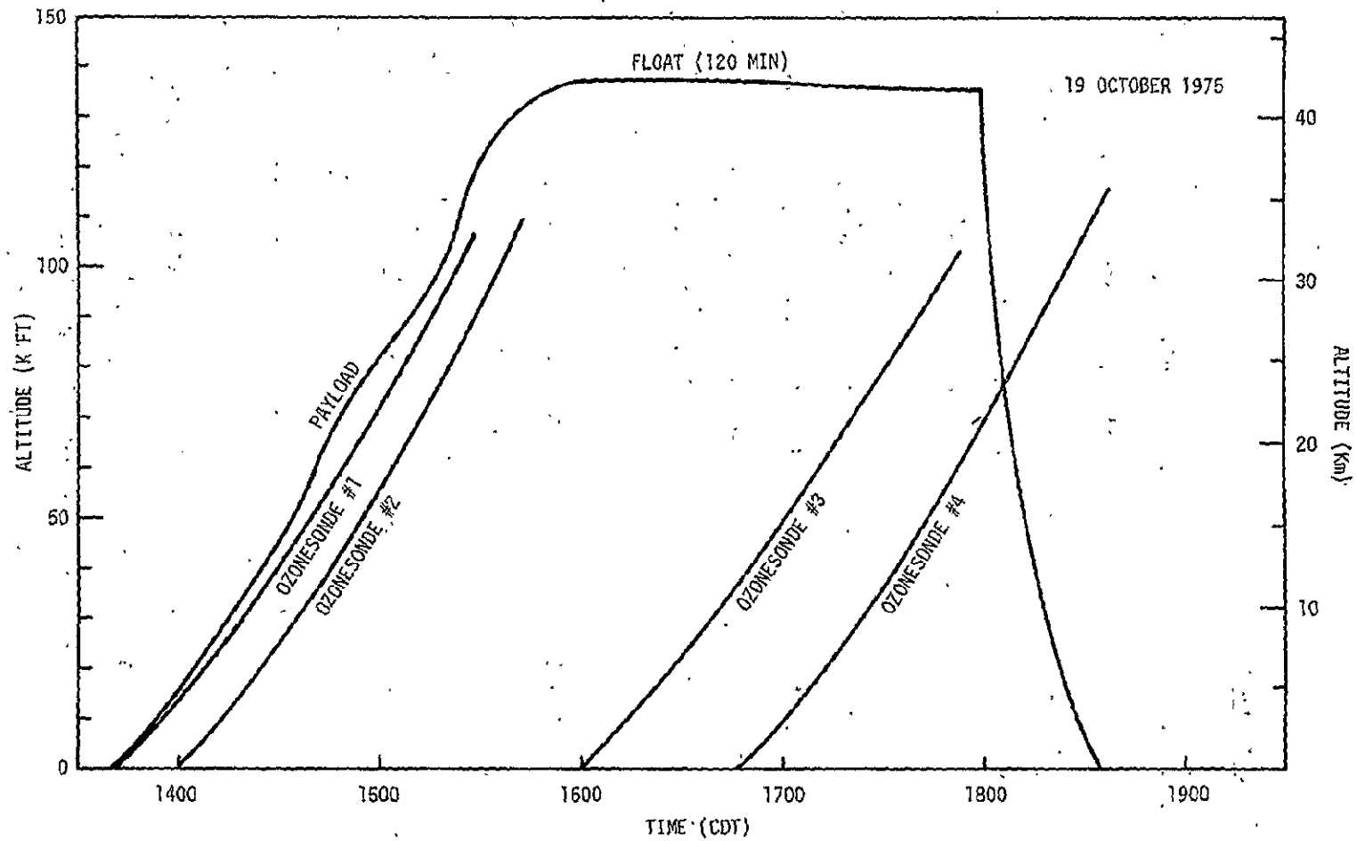
Figure 43.— Flight profile for second hydroxyl OH(X 2 Π) flight.
