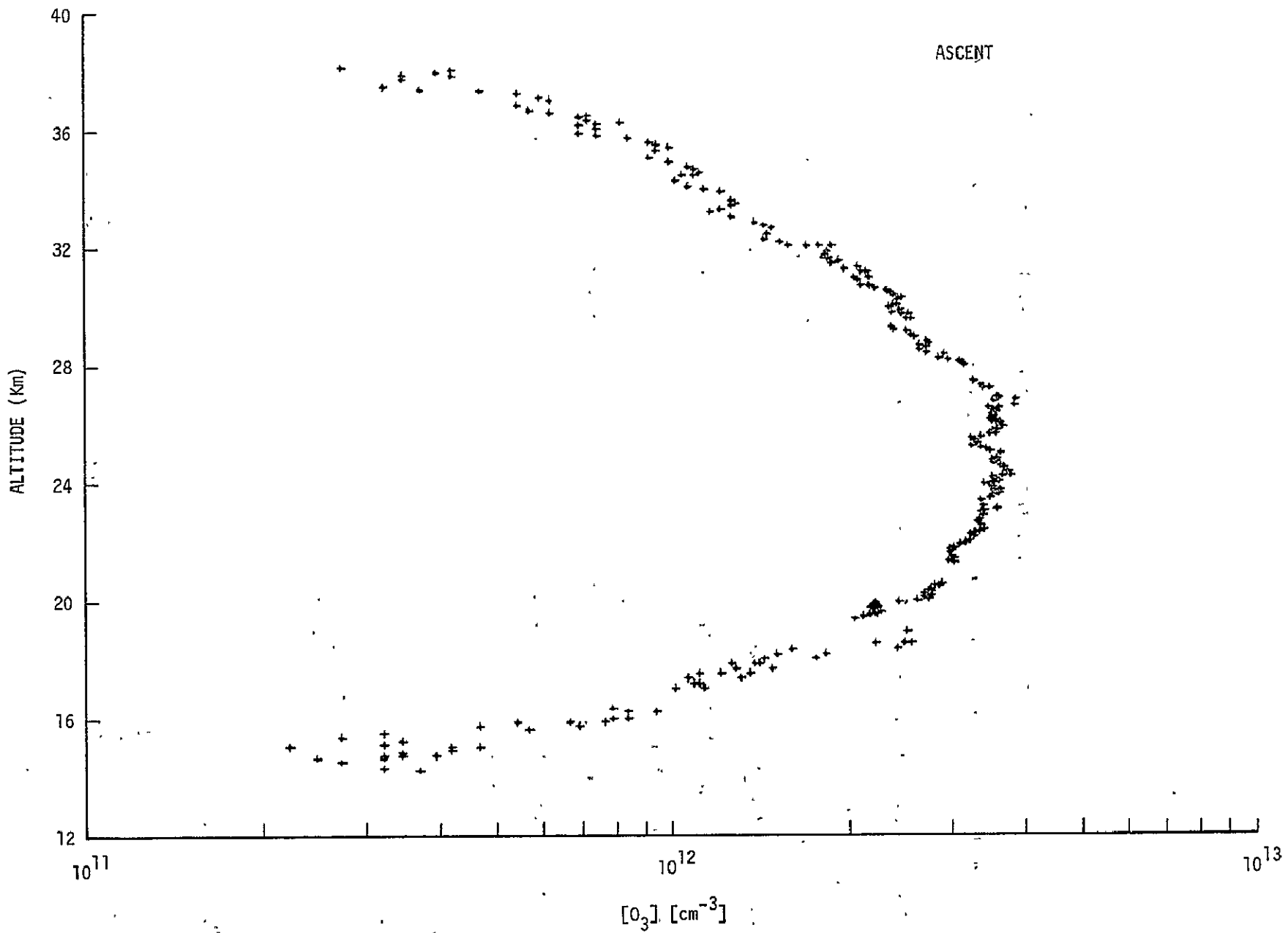
Figure 48.— Concentration of O 3 measured during ascent phase of the second Hydroxyl OH(X 2 π) flight.
