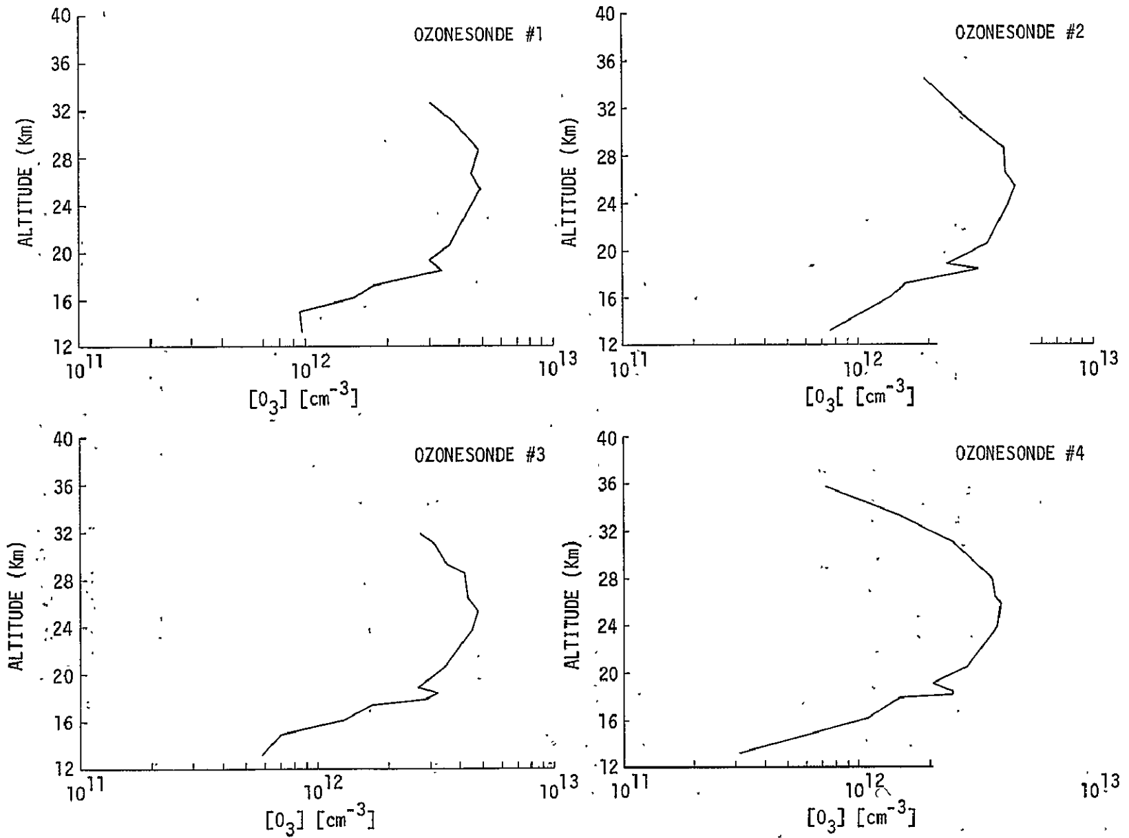
Figure 50.— Concentration of ozone determined by radiosondes released in conjunction with the second hydroxyl OH(X 2 π) flight.
