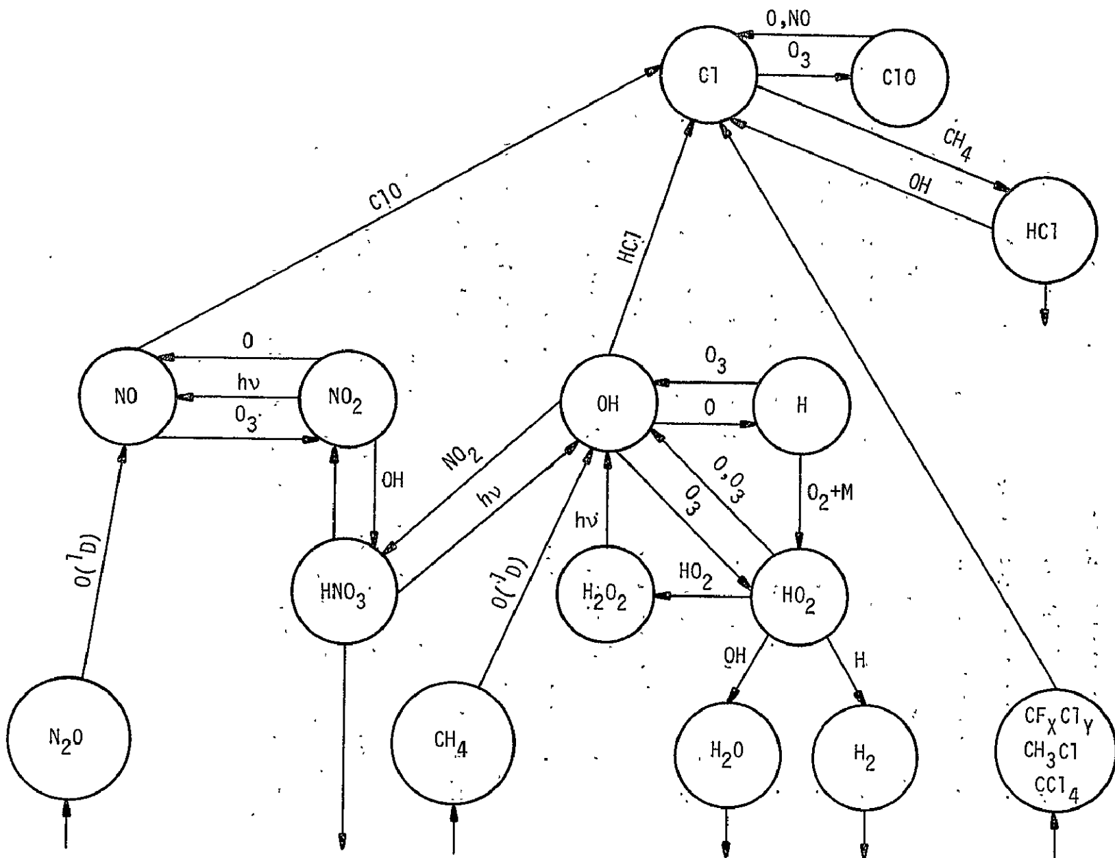
Figure 1.— Oxygen, hydrogen, nitrogen and chlorine photochemical systems.
