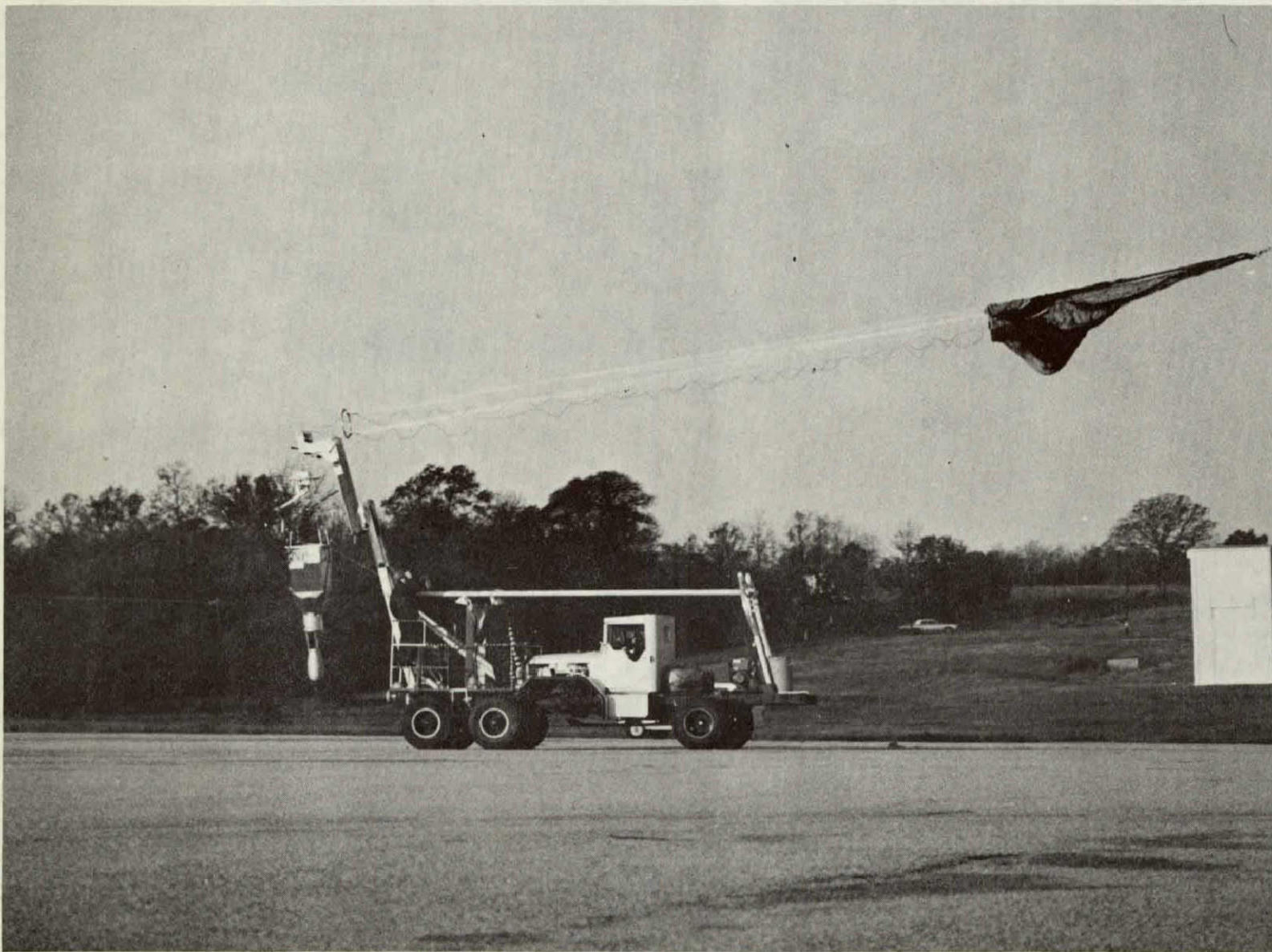
Figure 4. - Launch vehicle maneuvering to align balloon and payload
