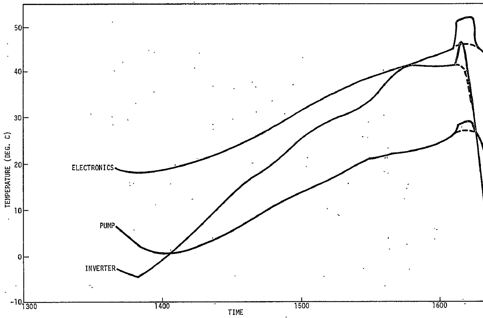
Figure 62.-- Thermal history of ozone monitor components for the third hydroxyl OH(X 2 Π) flight.
