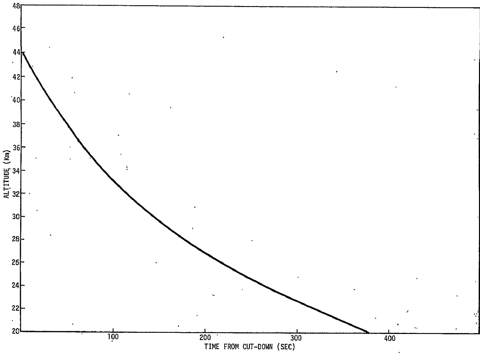
Figure 55.- Altitude/time profile of descending payload for the third hydroxyl OH( \chi^2\pi ) flight.
