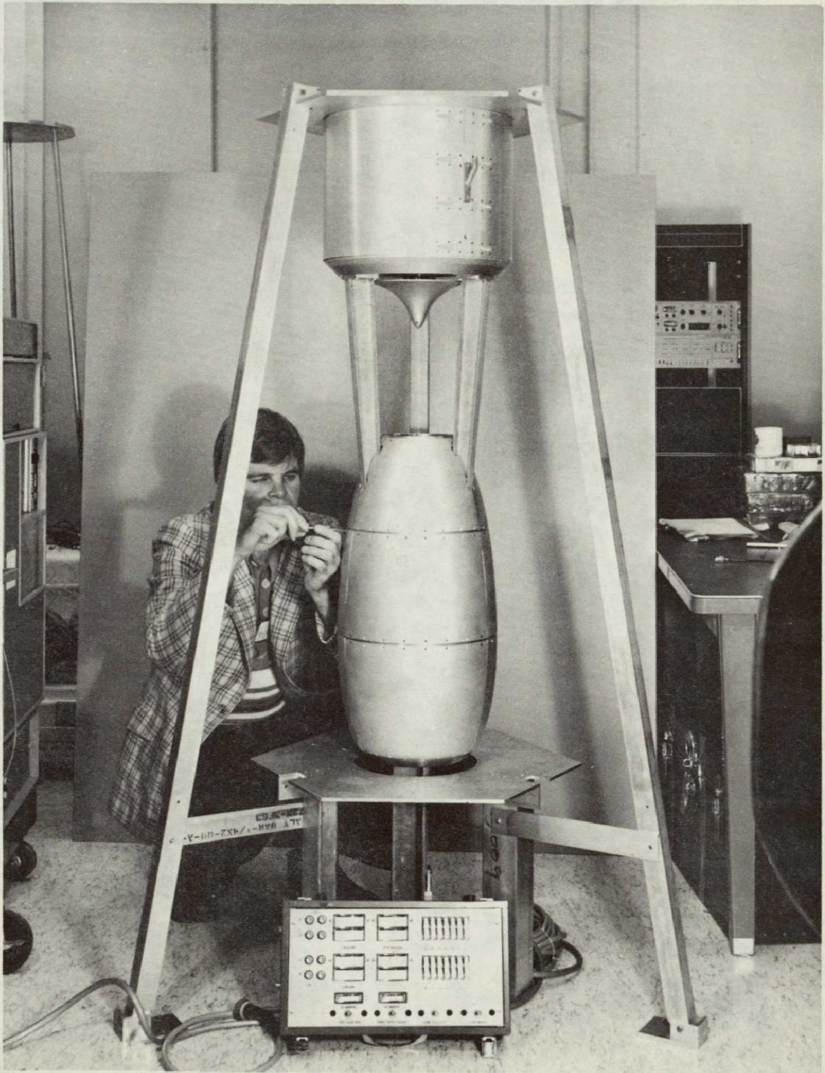
Figure 9. - Laminar flow through/resonance fluorescence instrument
