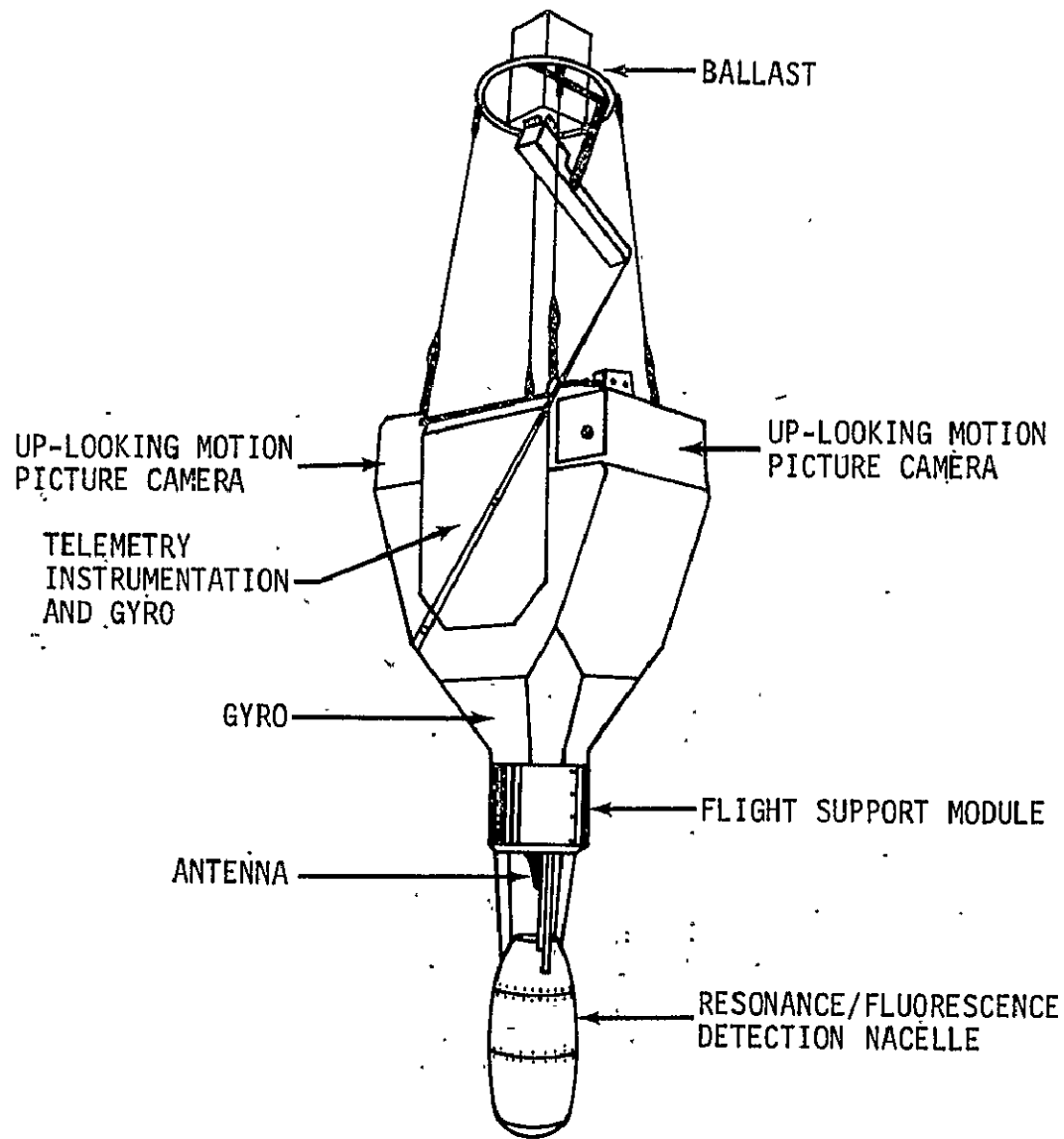
Figure 19.— Sketch of payload for the second atomic oxygen O(^3P) flight.
