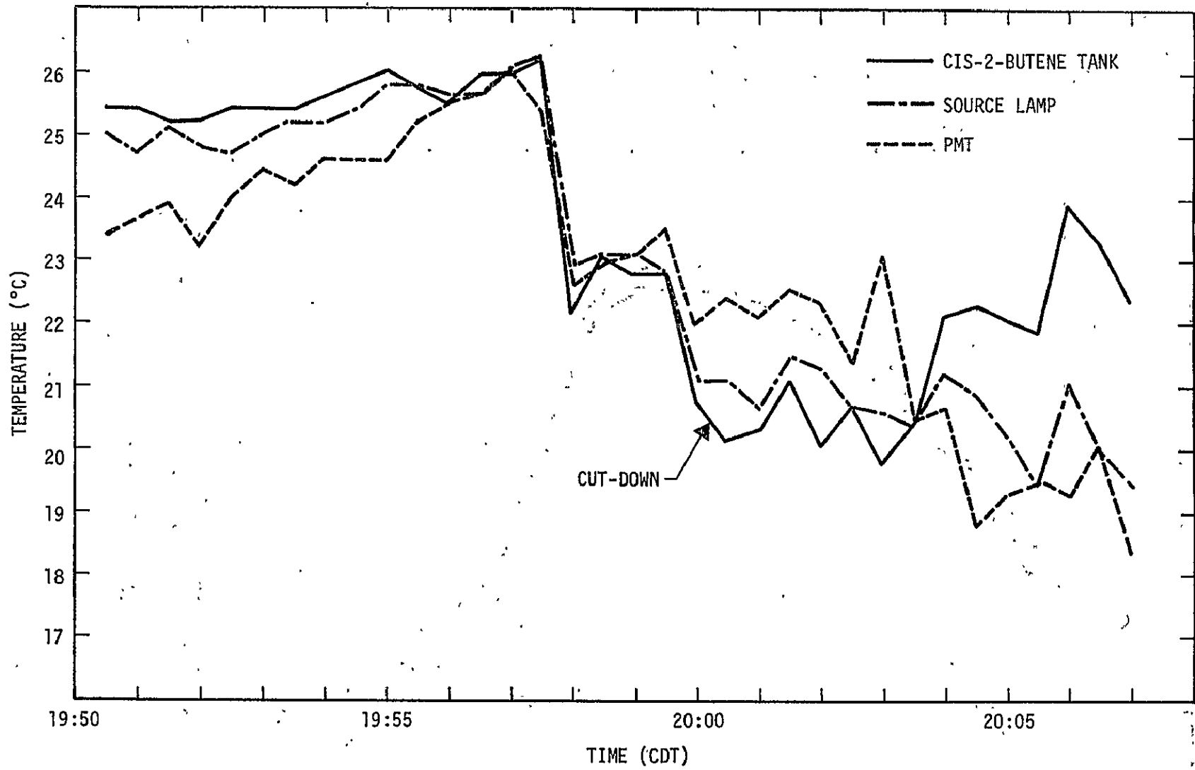
Figure 35.— Thermal histories (three locations on payload frame) for the first hydroxyl OH( \chi^2\pi ) flight ground time of cut-down.
