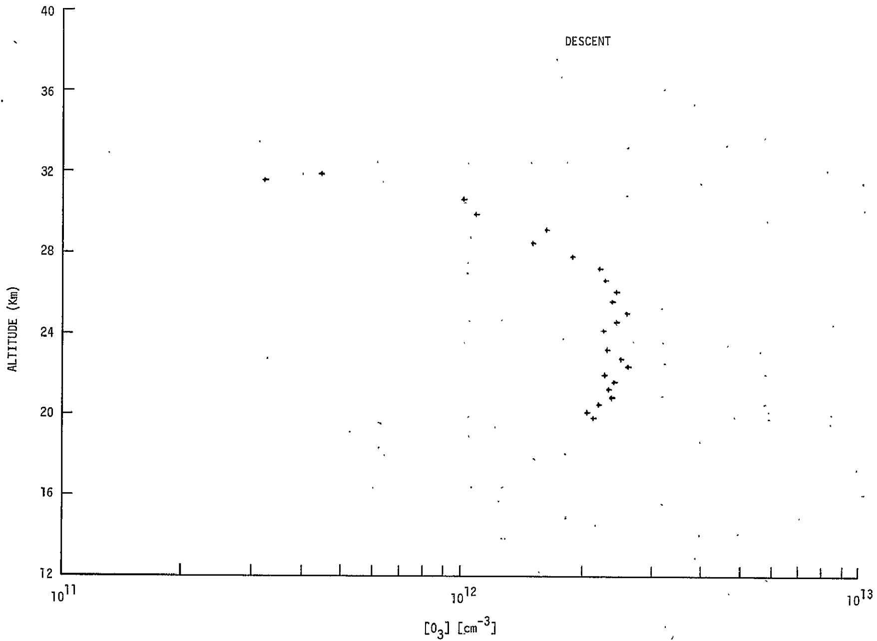
Figure 49.— Concentration of O 3 measured during descent phase of the second hydroxyl OH( \chi^2\pi ) flight.
