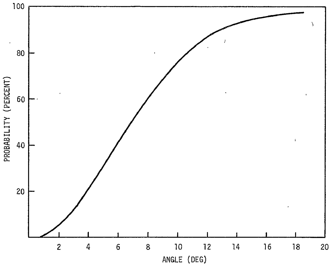
Figure 46.— Probability (percent) that the angular deviation of the payload from vertical is less than a given angle as a function of angle for the second hydroxyl CH( X^2\pi ) flight:
