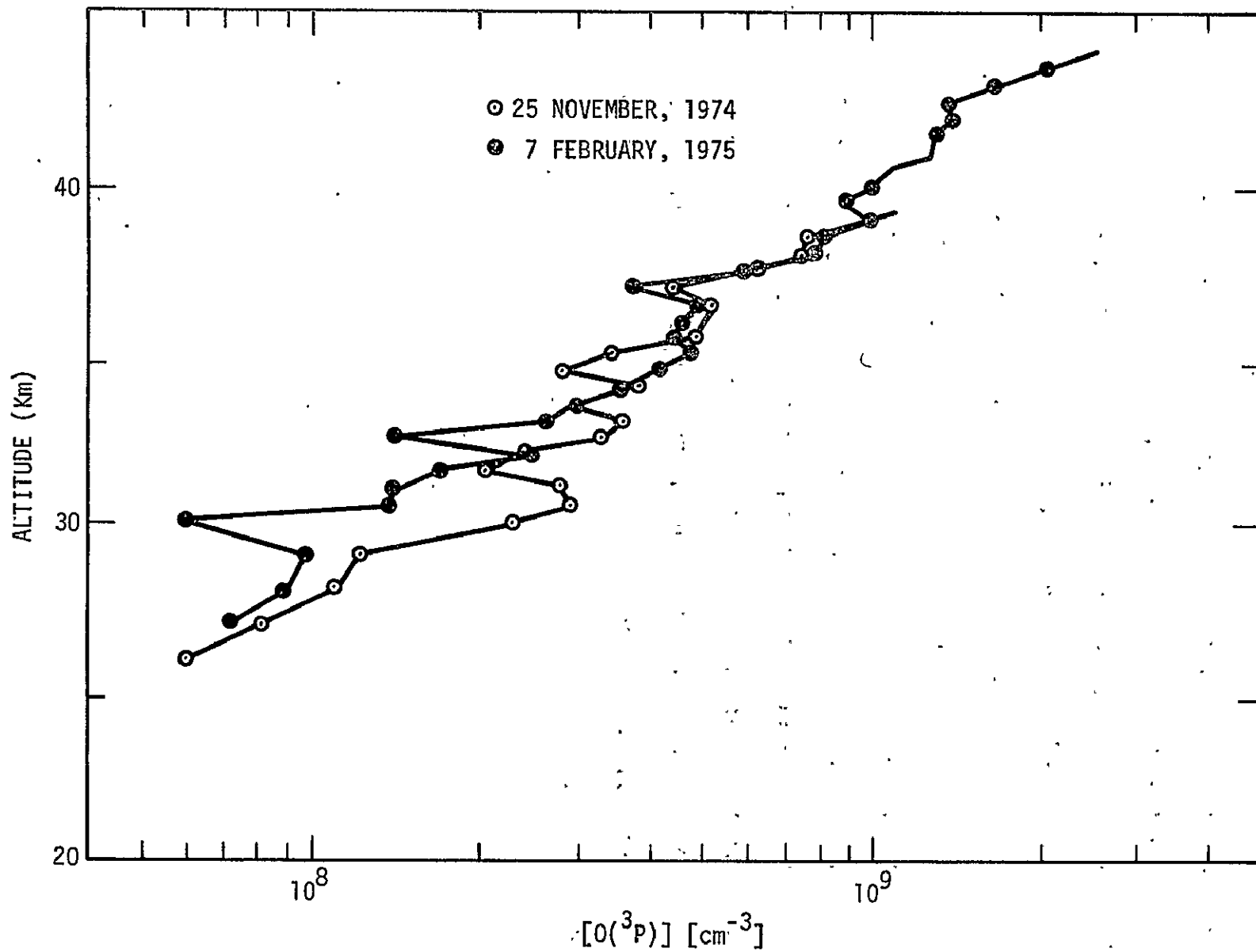
Figure 24.— Stratospheric concentration of atomic oxygen measured on the first and second atomic oxygen O( 3 P) flights.
