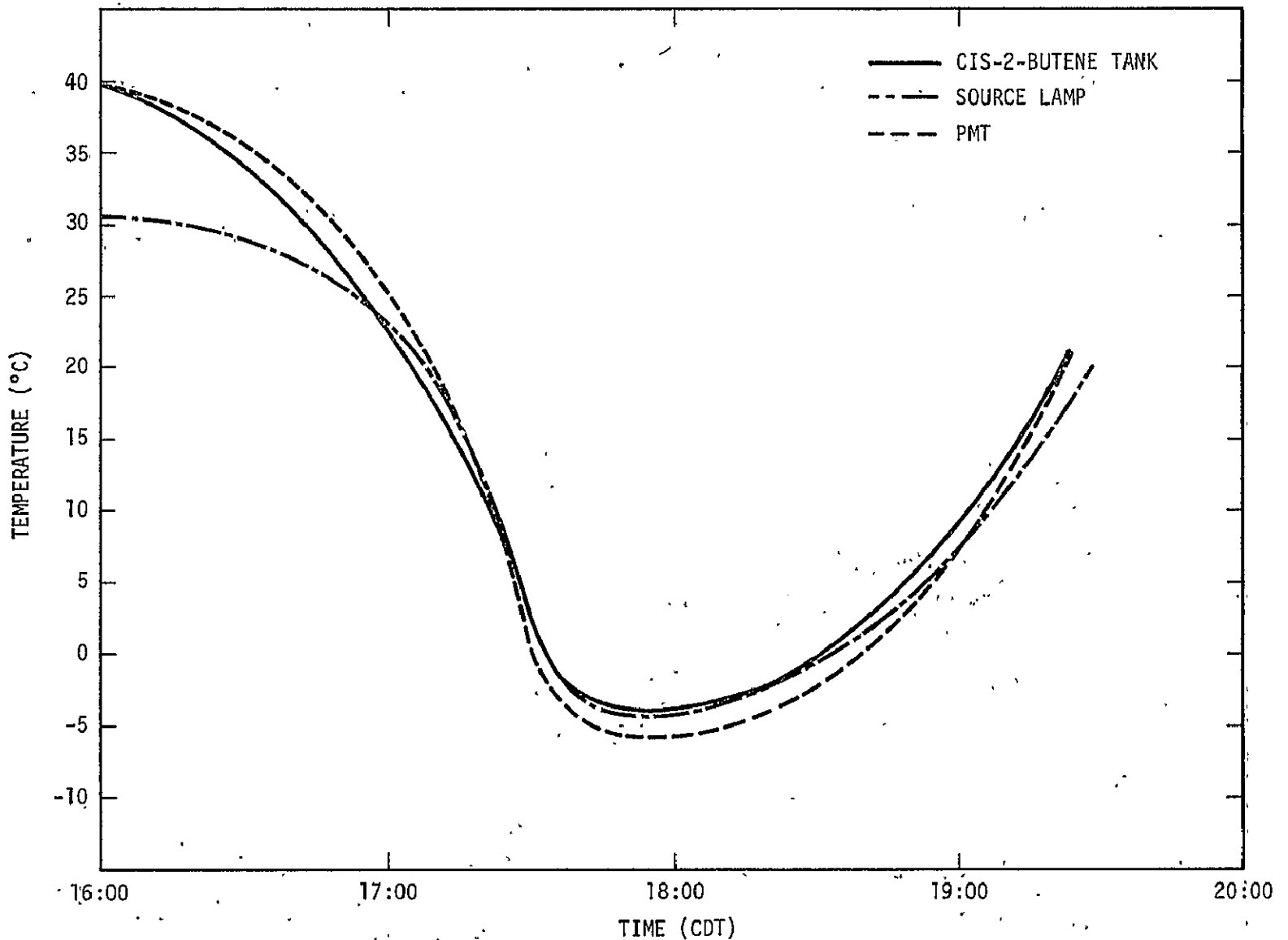
Figure 34.— Thermal histories (three locations on payload frame) for the first hydroxyl OH(X 2 π) flight during ascent.
