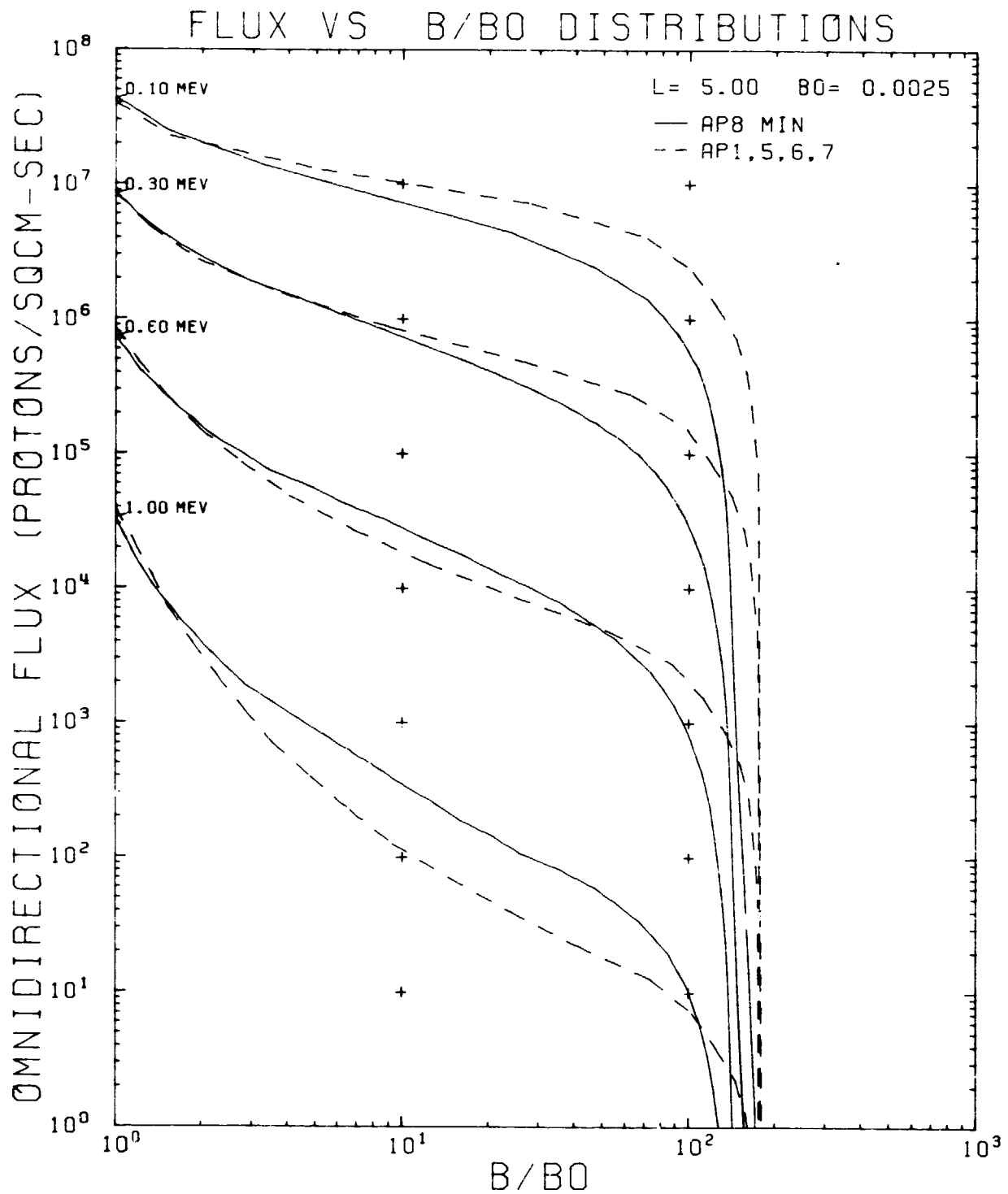
Figure 142. AP8MIN and AP-1, -5, -6, and -7 Flux vs B/B0 Comparison Plot for L = 5.00 R E
