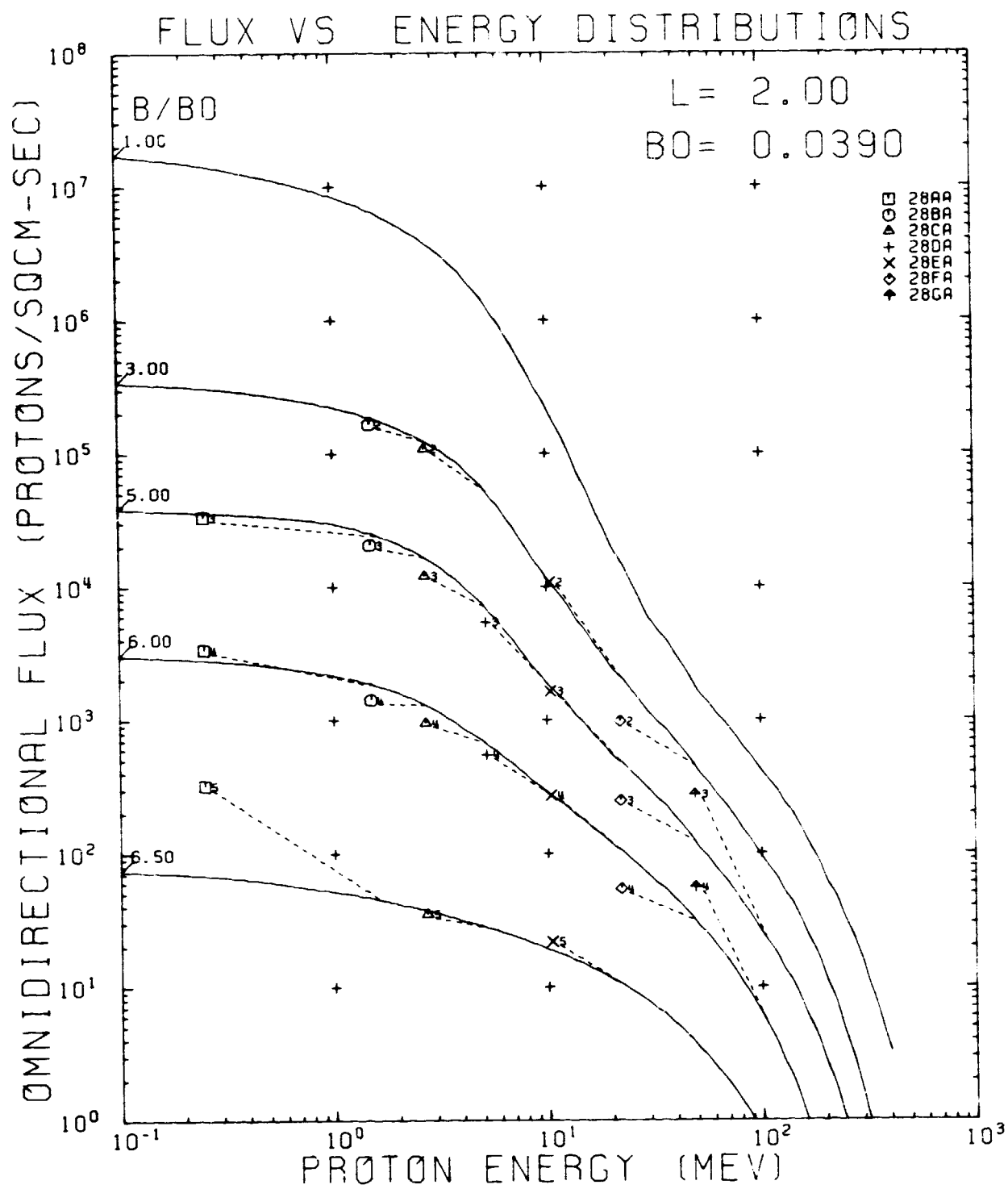
Figure 124. AP8MAX and Data Flux vs Energy Comparison Plot for L = 2.00 R_E
