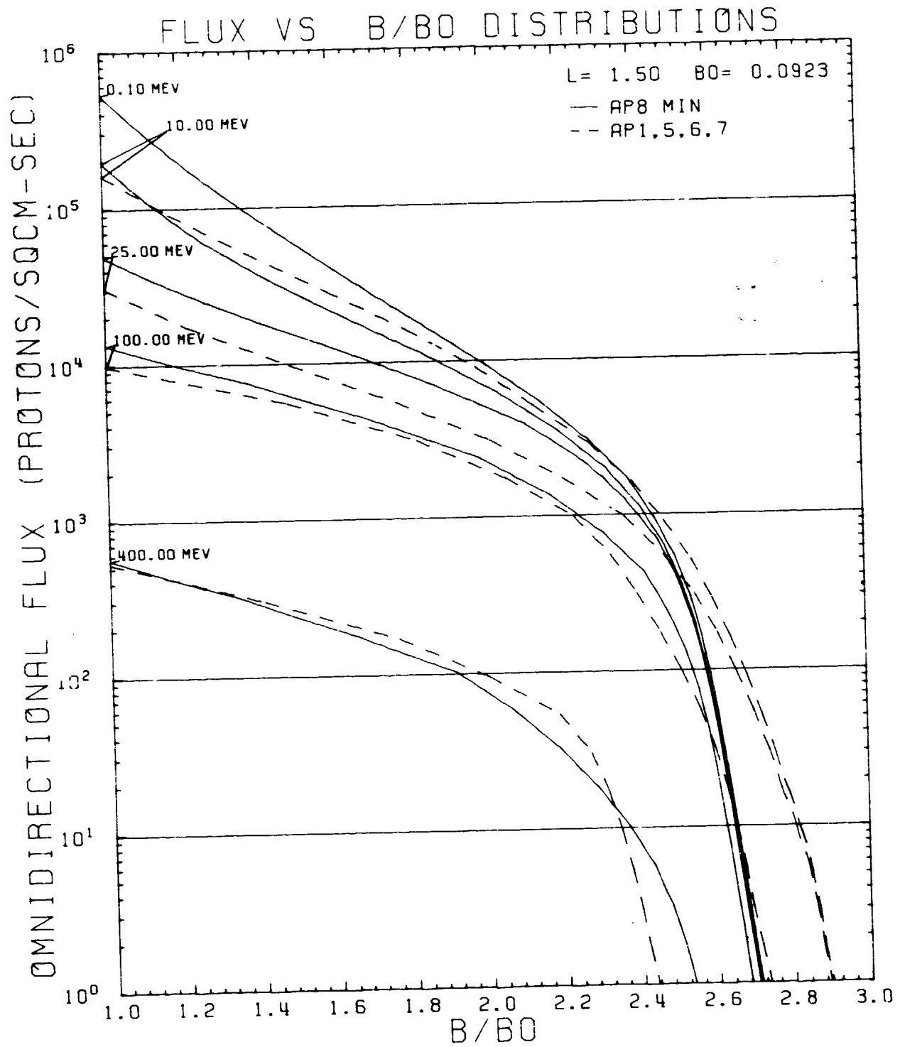
Figure 137. AP8MIN and AP-1, -5, -6, and -7 Flux vs B/B 0 Comparison Plot for L = 1.50 RE
