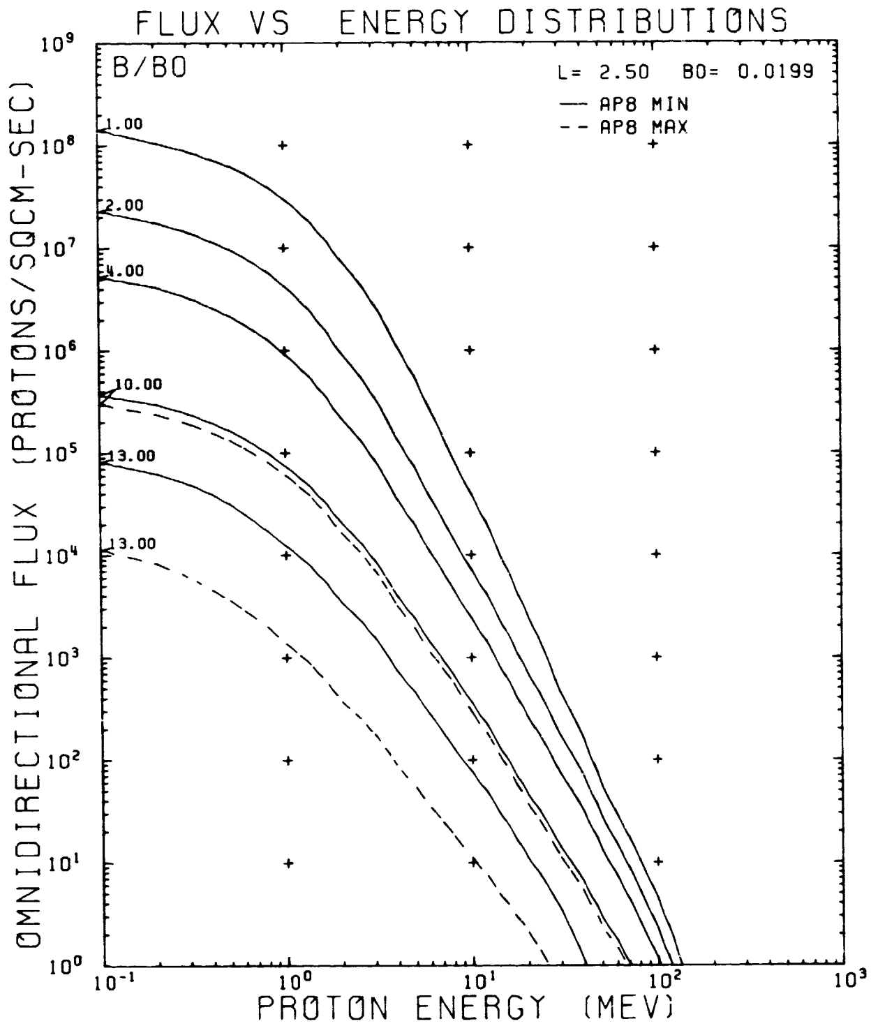
Figure 135. AP8MIN and AP8MAX Flux vs Energy Comparison Plot for L = 2.50 RE
