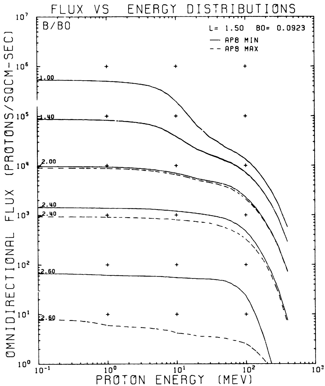
Figure 133. AP8MIN and AP8MAX Flux vs Energy Comparison Plot for L = 1.50 R E
