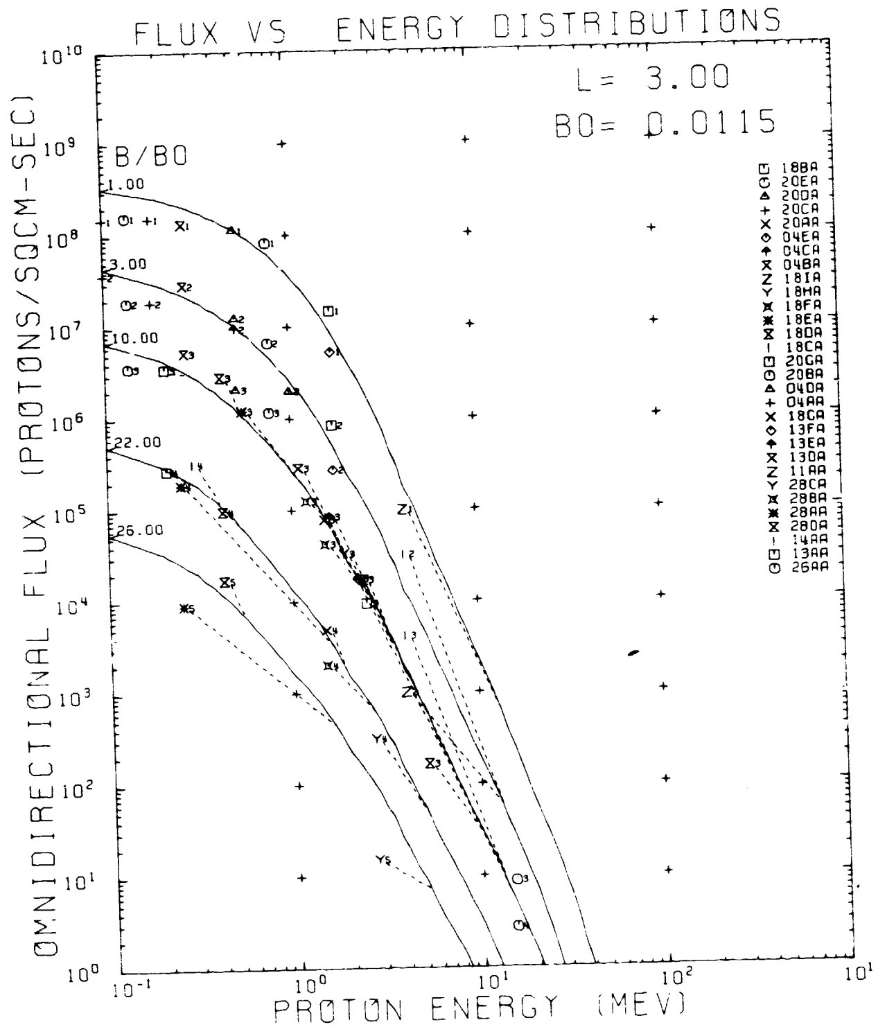
Figure 112. AP8MIN and Data Flux vs Energy Comparison Plot for L = 3.00 R E
