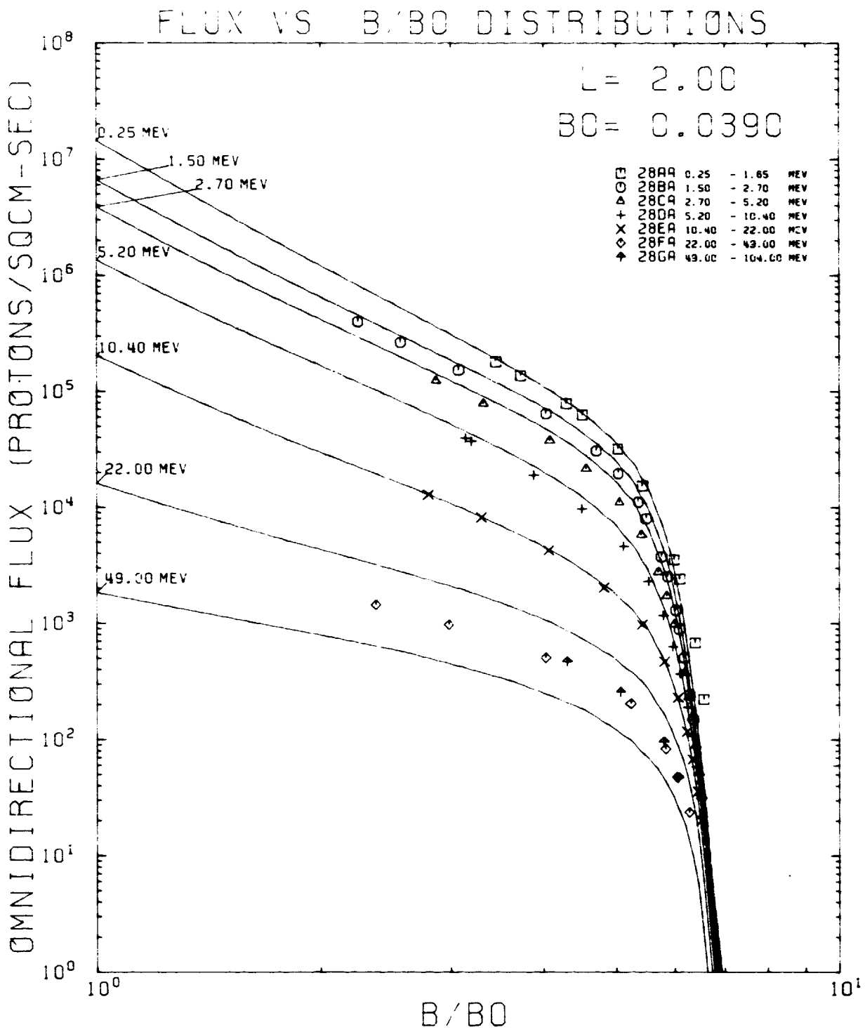
Figure 119. AP8MAX and Data Flux vs B/B 0 Comparison Plot for L = 2.00 R E
