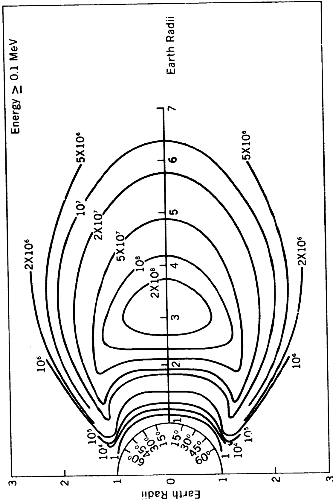
Figure 65. AP8MIN R-A Plot of Constant Intensity Flux Contours with an Energy of \geq 0.1 MeV
