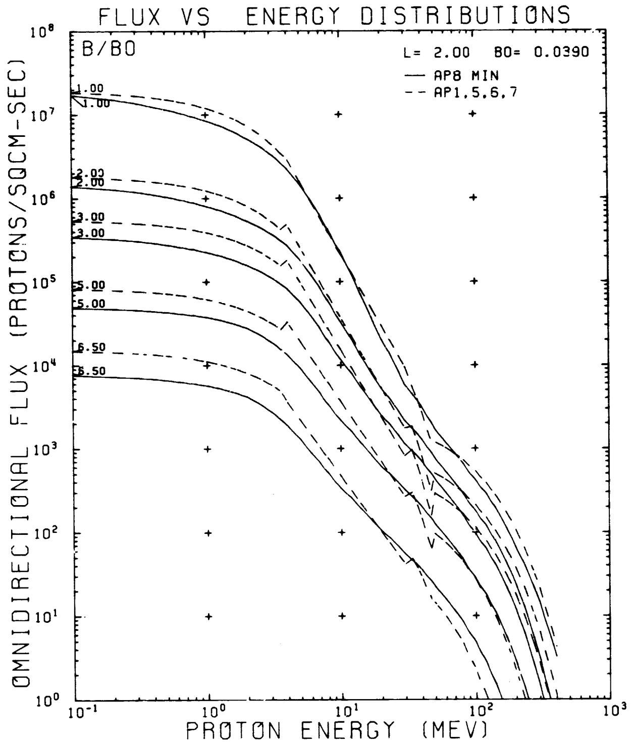
Figure 146. AP8MIN and AP-1 -5, -6, and -7 Flux vs Energy Comparison Plot for L = 2.00 R_E
