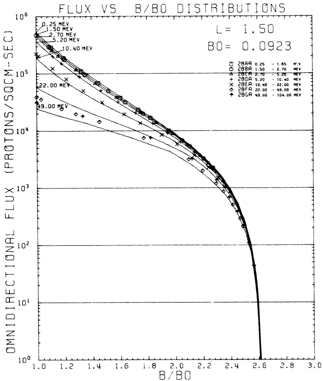
Figure 118. AP8MAX and Data Flux vs B/B_0 Comparison Plot for L = 1.50 R_E
