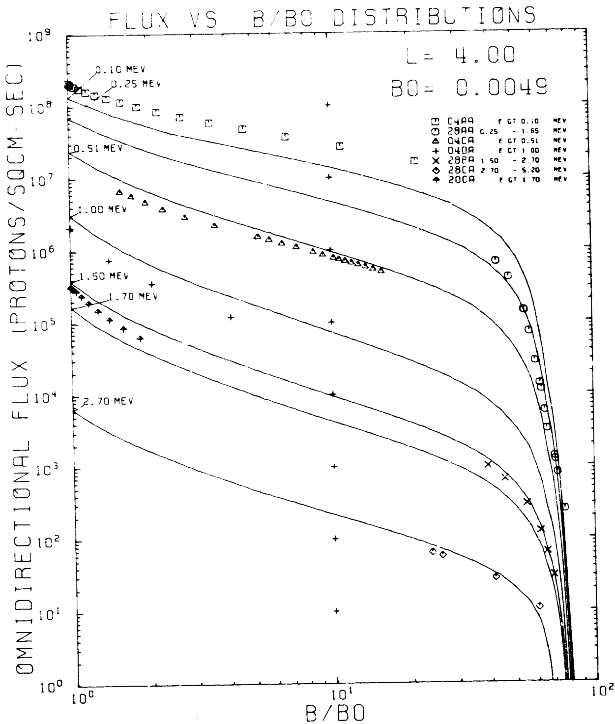
Figure 103. AP8MIN and Data Flux vs B/B_0 Comparison Plot for L = 4.00 R_E
