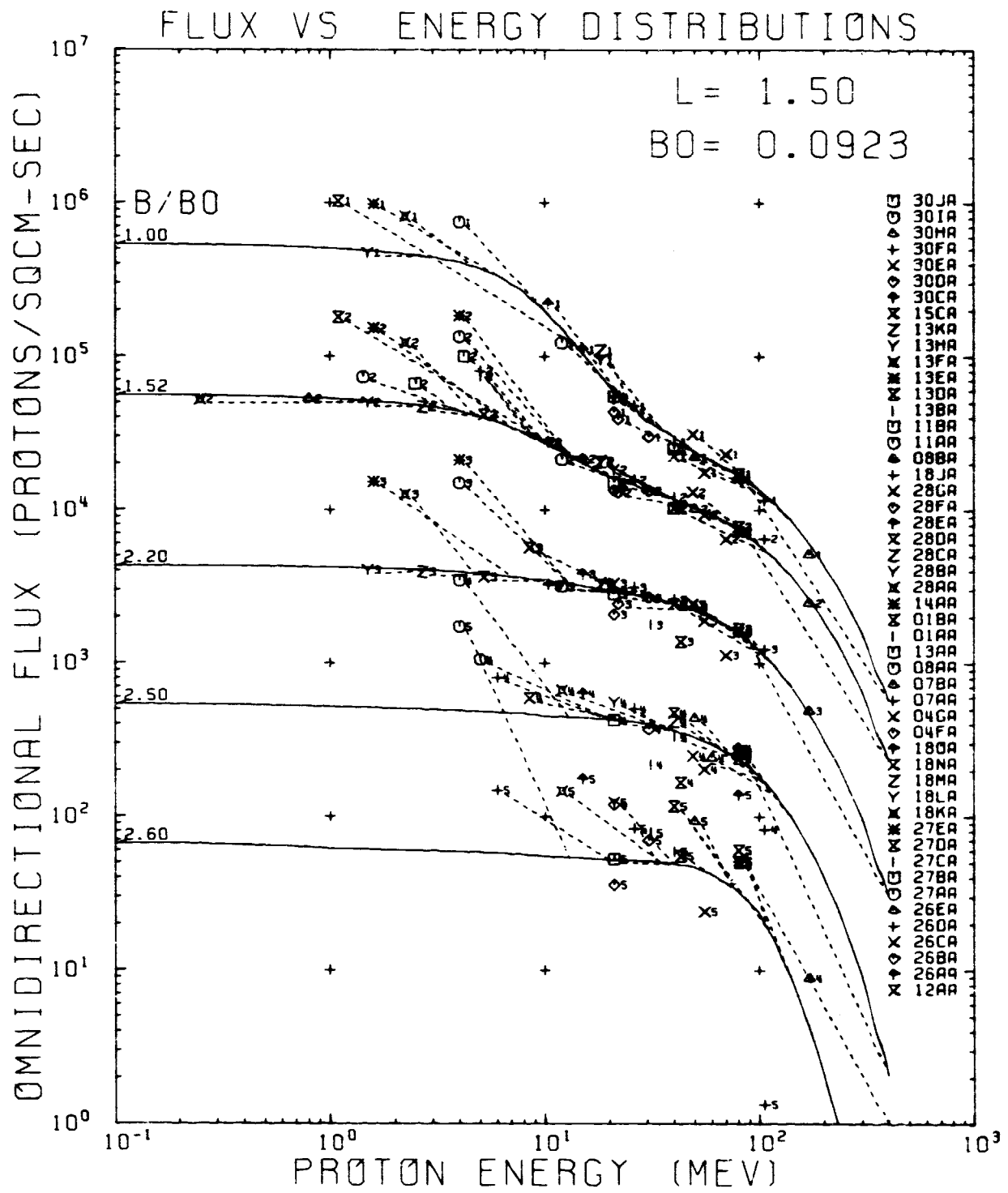
Figure 109. AP8MIN and Data Flux vs Energy Comparison Plot for L = 1.50 R_E
