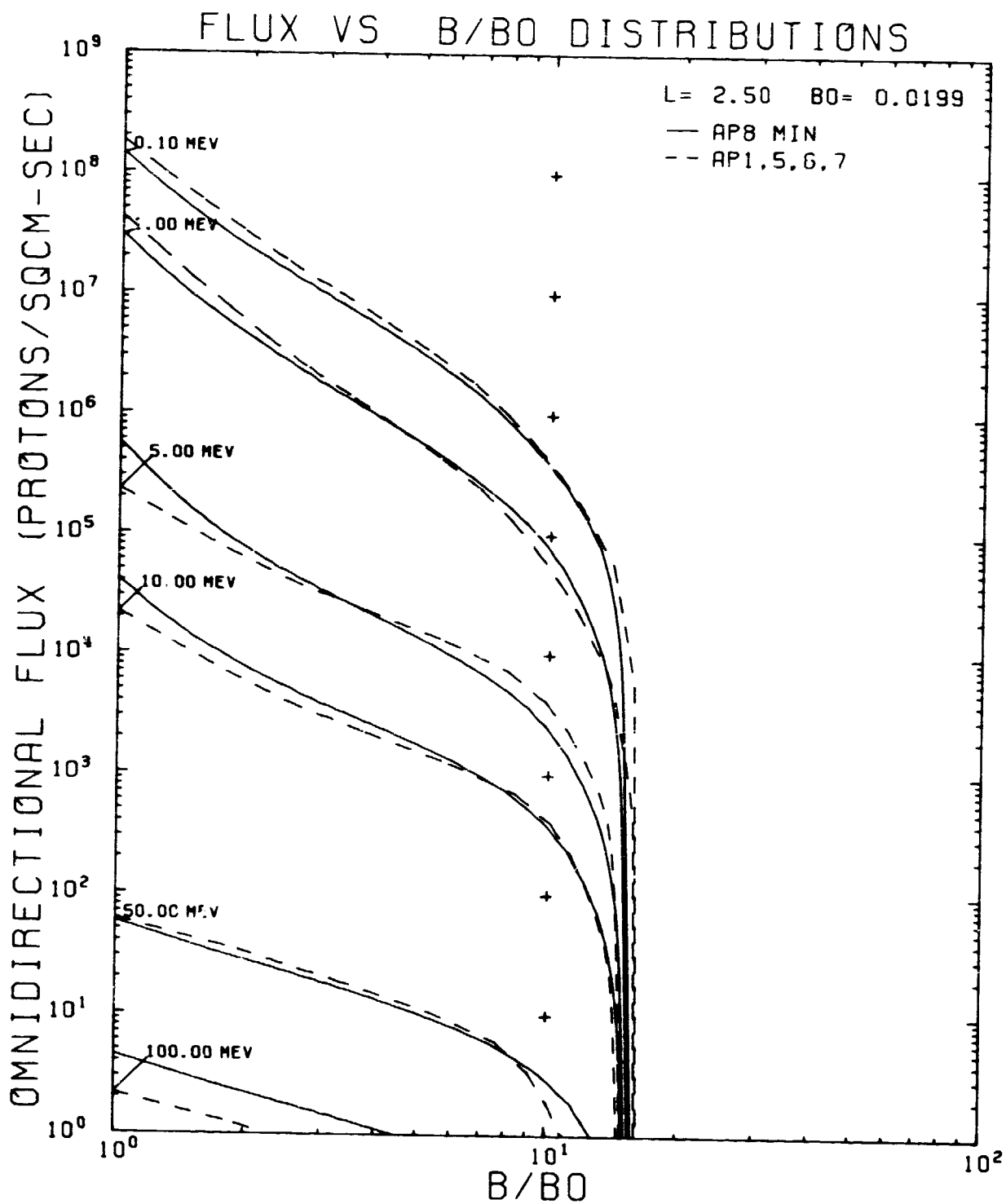
Figure 139. AP8MIN and AP-1, -5, -6, and -7 Flux vs B/B 0 Comparison Plot for L = 2.50 R E
