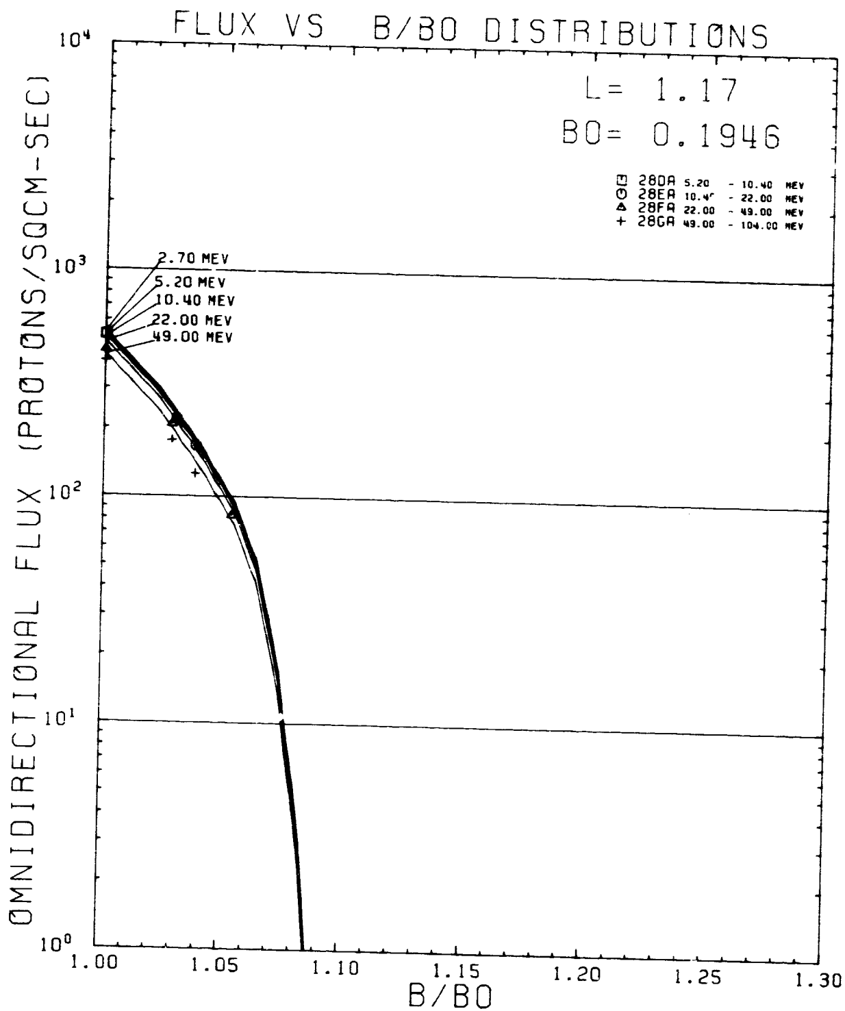
Figure 116. AP8MAX and Data Flux vs B/B 0 Comparison Plot for L = 1.17 R F
