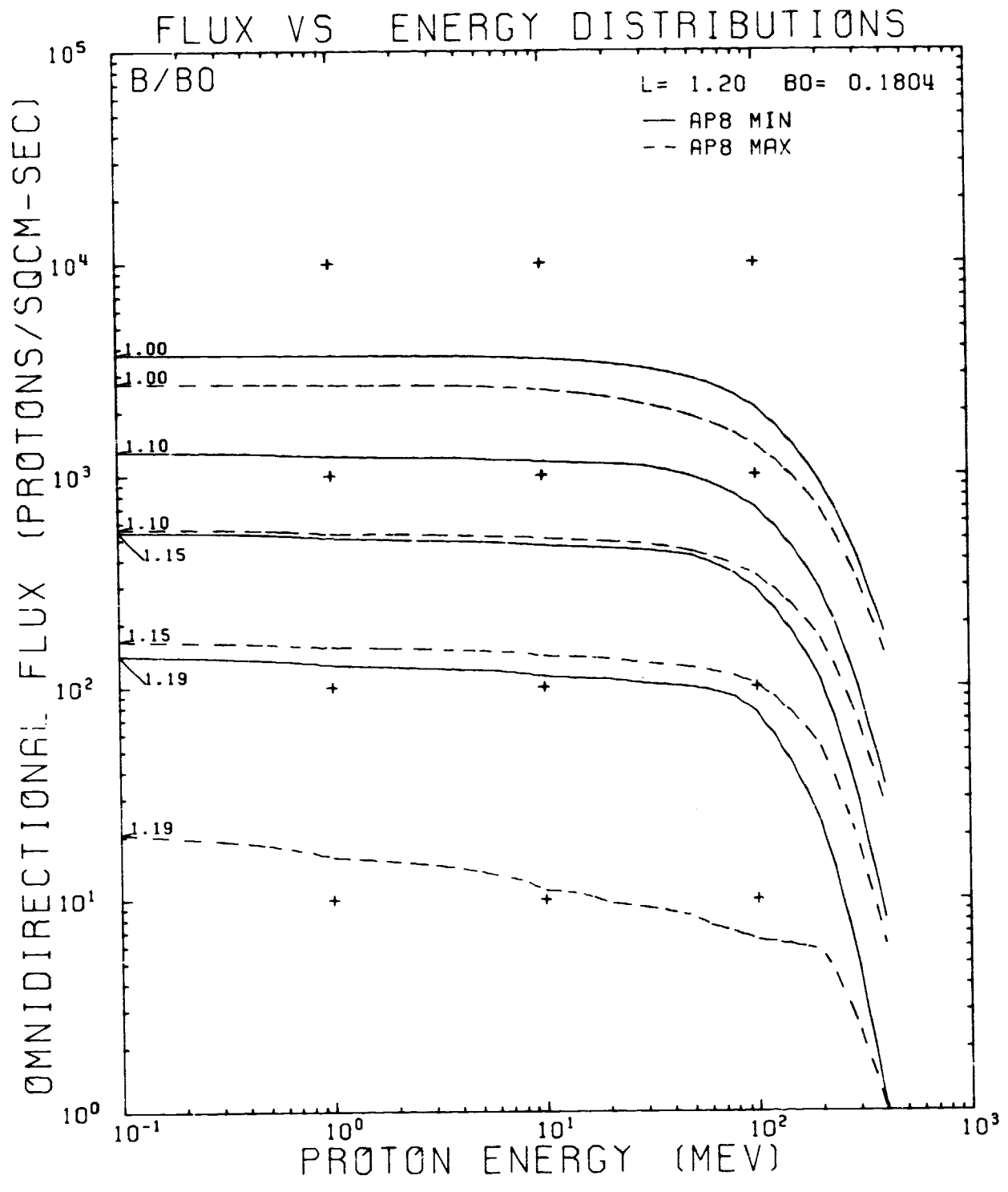
Figure 132. AP8MIN and AP8MAX Flux vs Energy Comparison Plot for L = 1.20 R E
