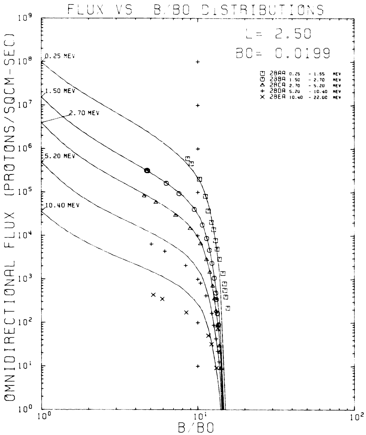
Figure 120. AP8MAX and Data Flux vs B/B 0 Comparison Plot for L = 2.50 R E
