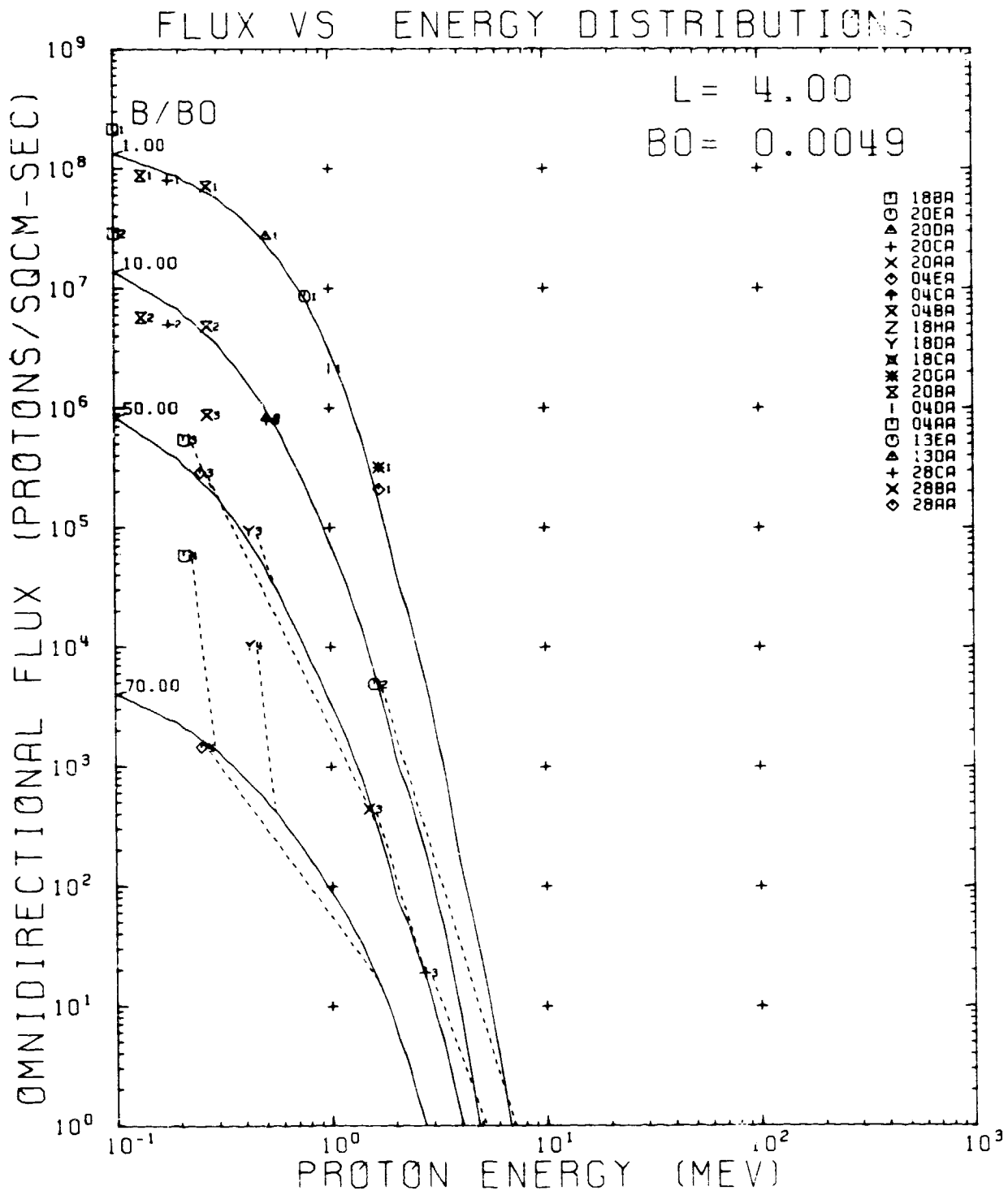
Figure 113. AP8MIN and Data Flux vs Energy Comparison Plot for L = 4.00 RE
