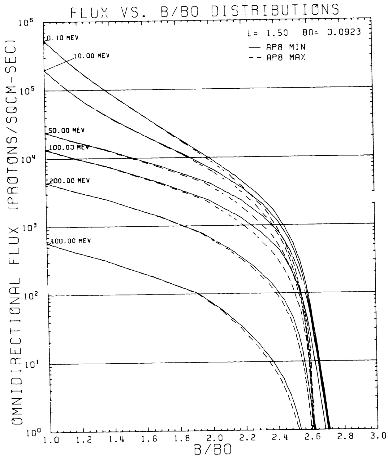
Figure 128. AP8MIN and AP8MAX Flux vs B/B 0 Comparison Plot for L = 1.50 RE
