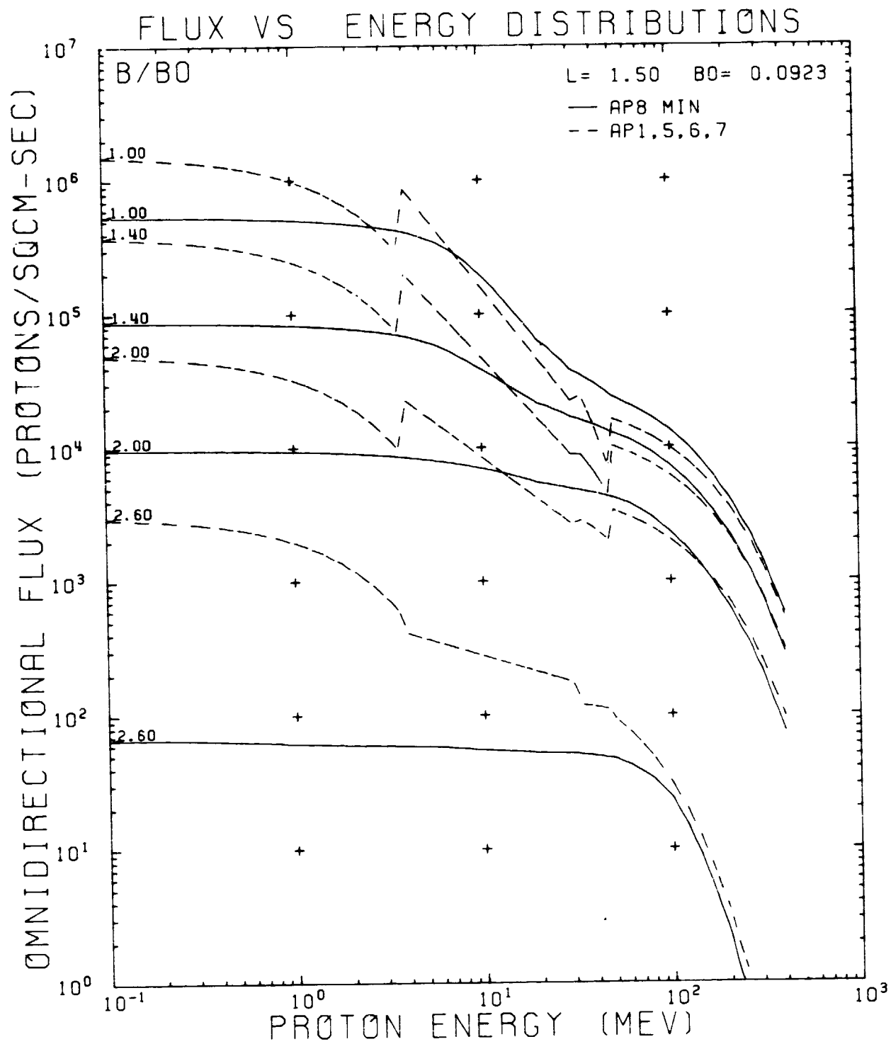
Figure 145. AP8MIN and AP-1, -5, -6, and -7 Flux vs Energy Comparison Plot for L = 1.50 RE
