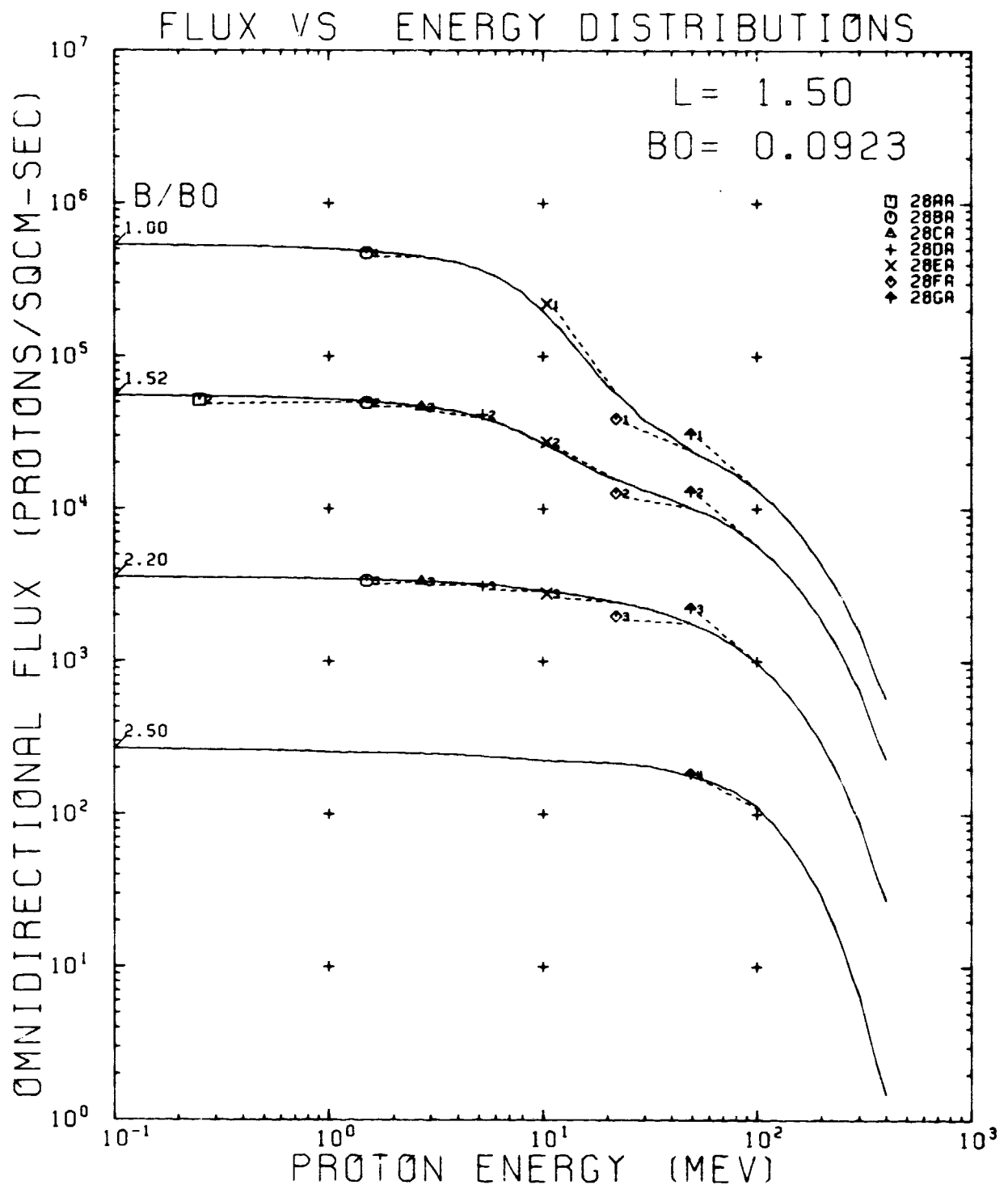
Figure 123. AP8MAX and Data Flux vs Energy Comparison Plot for L = 1.50 R E
