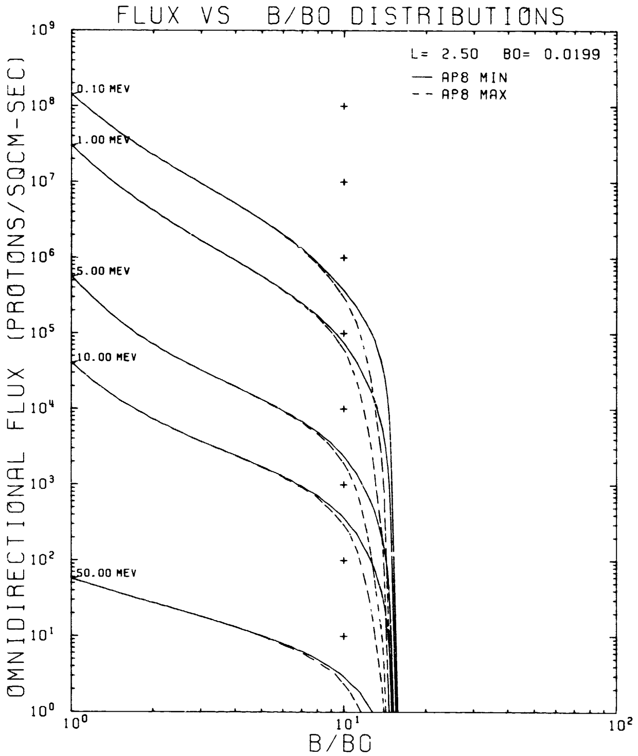
Figure 130. AP8MIN and AP8MAX Flux vs B/B 0 Comparison Plot for L = 2.50 R E
