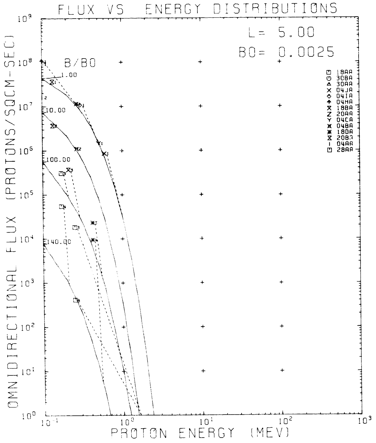
Figure 114. AP8MIN and Data Flux vs Energy Comparison Plot for L = 5.00 R_E
