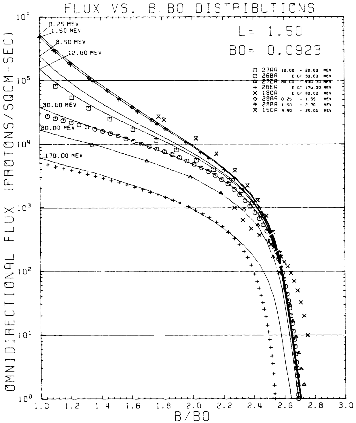
Figure 99. AP8MIN and Data Flux vs B/B_0 Comparison Plot for L = 1.50 R_E
