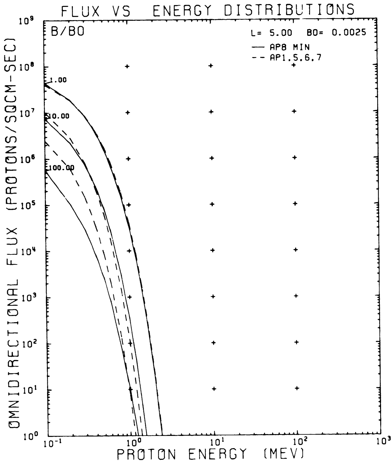
Figure 150. AP8MIN and AP-1, -5, -6, and -7 Flux vs Energy Comparison Plot for L = 5.00 R_E
