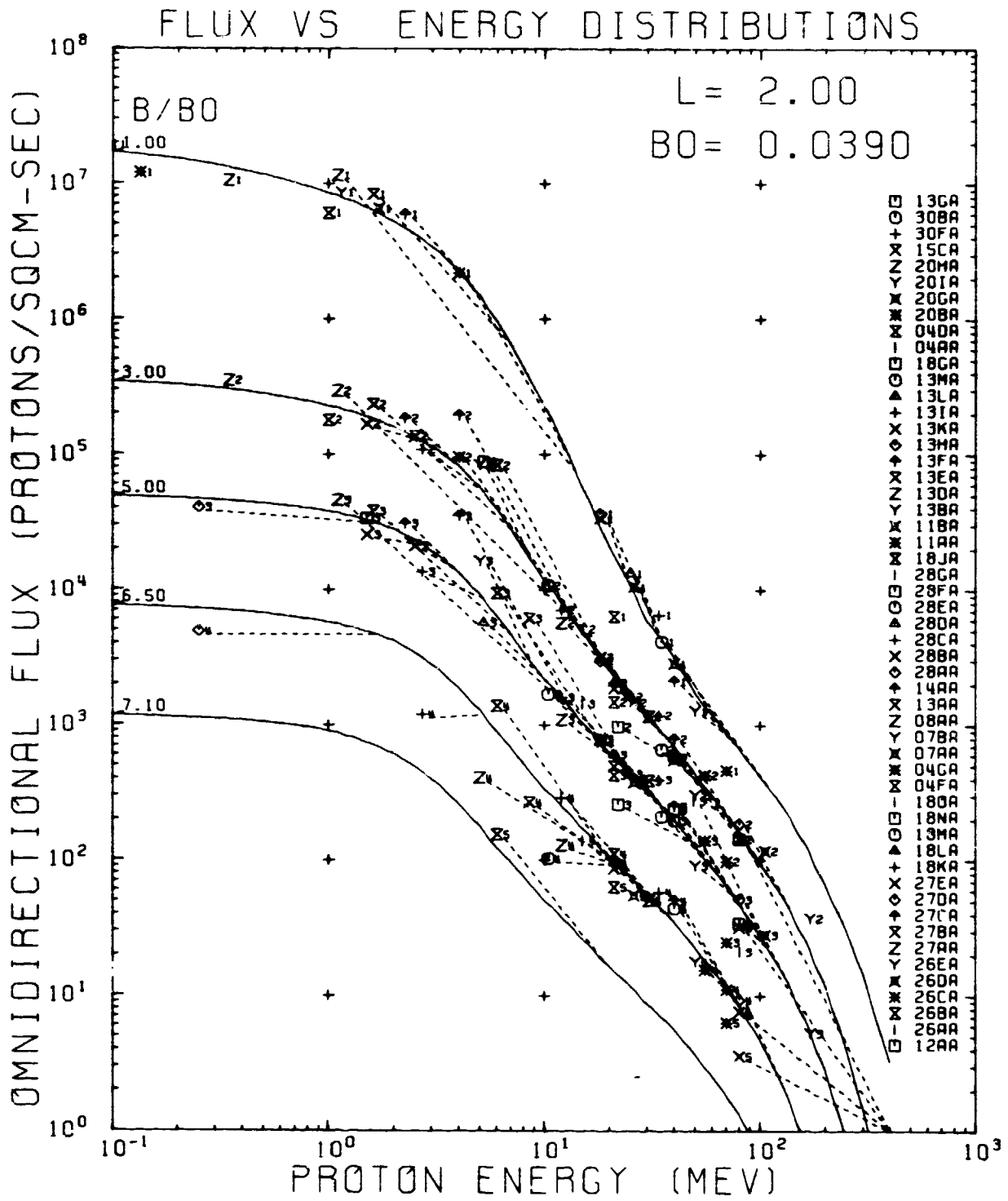
Figure 110. AP8MIN and Data Flux vs Energy Comparison Plot for L = 2.00 R E
