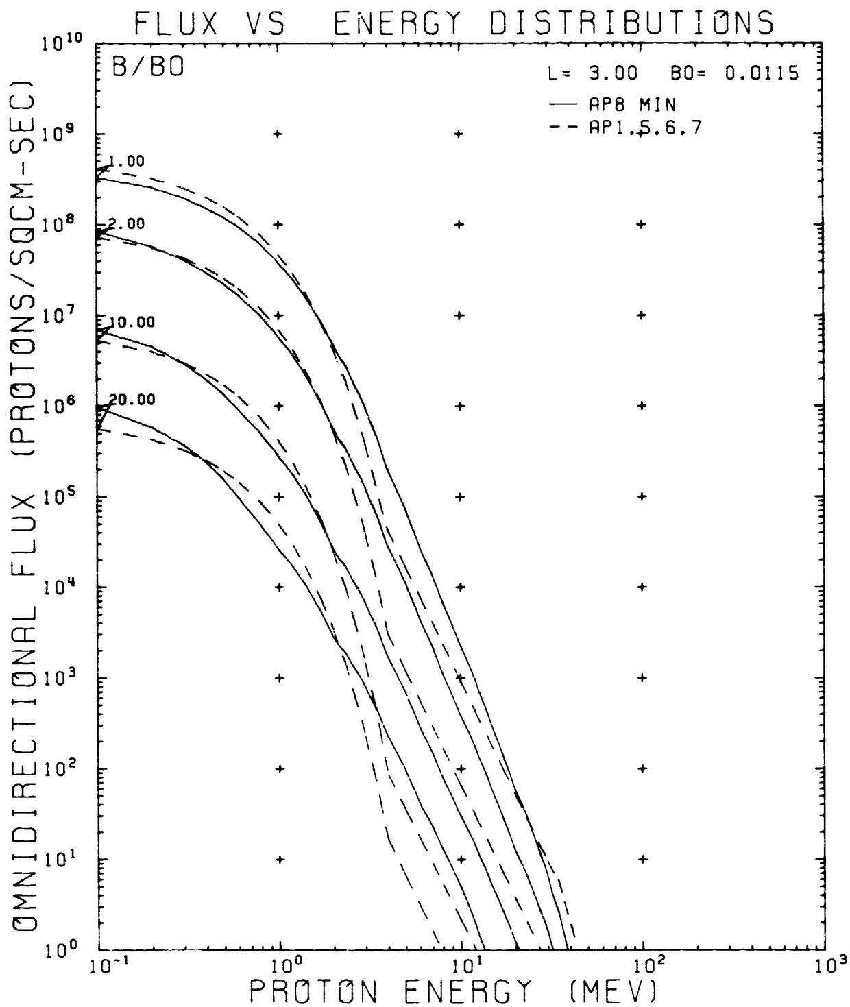
Figure 148. AP8MIN and AP-1, -5, -6, and -7 Flux vs Energy Comparison Plot for L = 3.00 R_E
