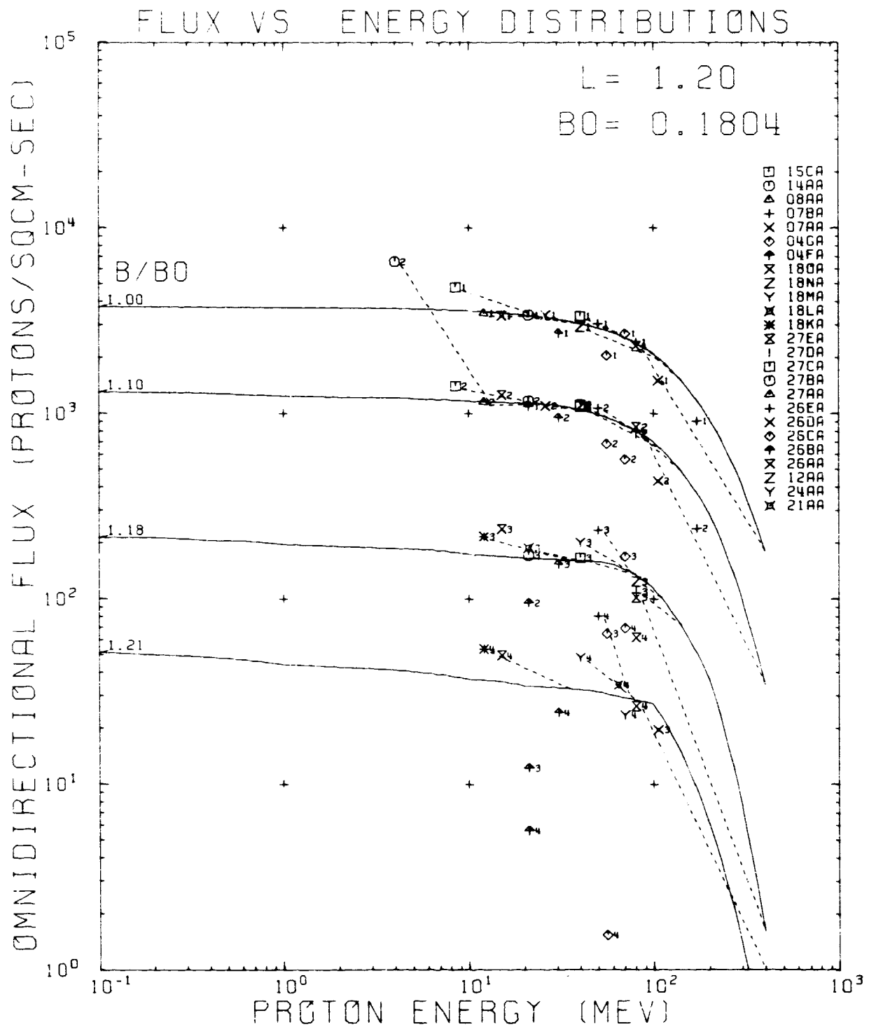
Figure 108. AP8MIN and Data Flux vs Energy Comparison Plot for L = 1.20 R_E
