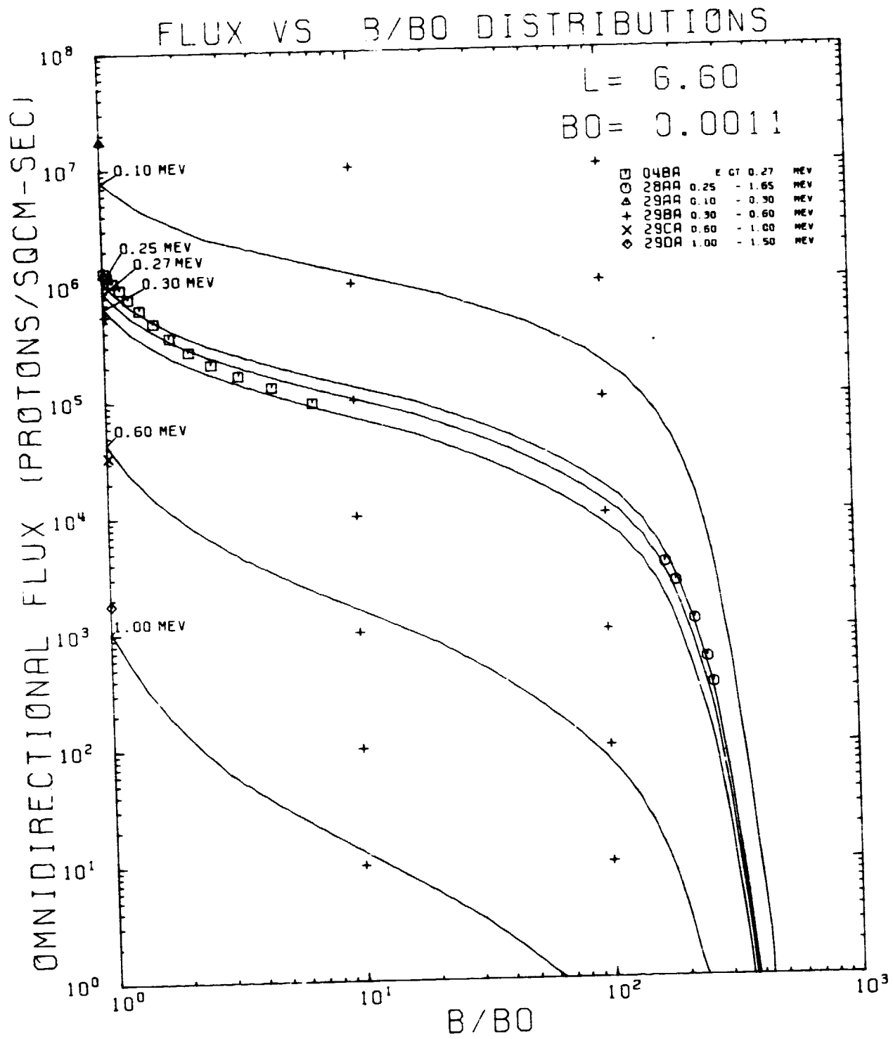
Figure 105. AP8MIN and Data Flux vs B/B 0 Comparison Plot for L = 6.60 RE
