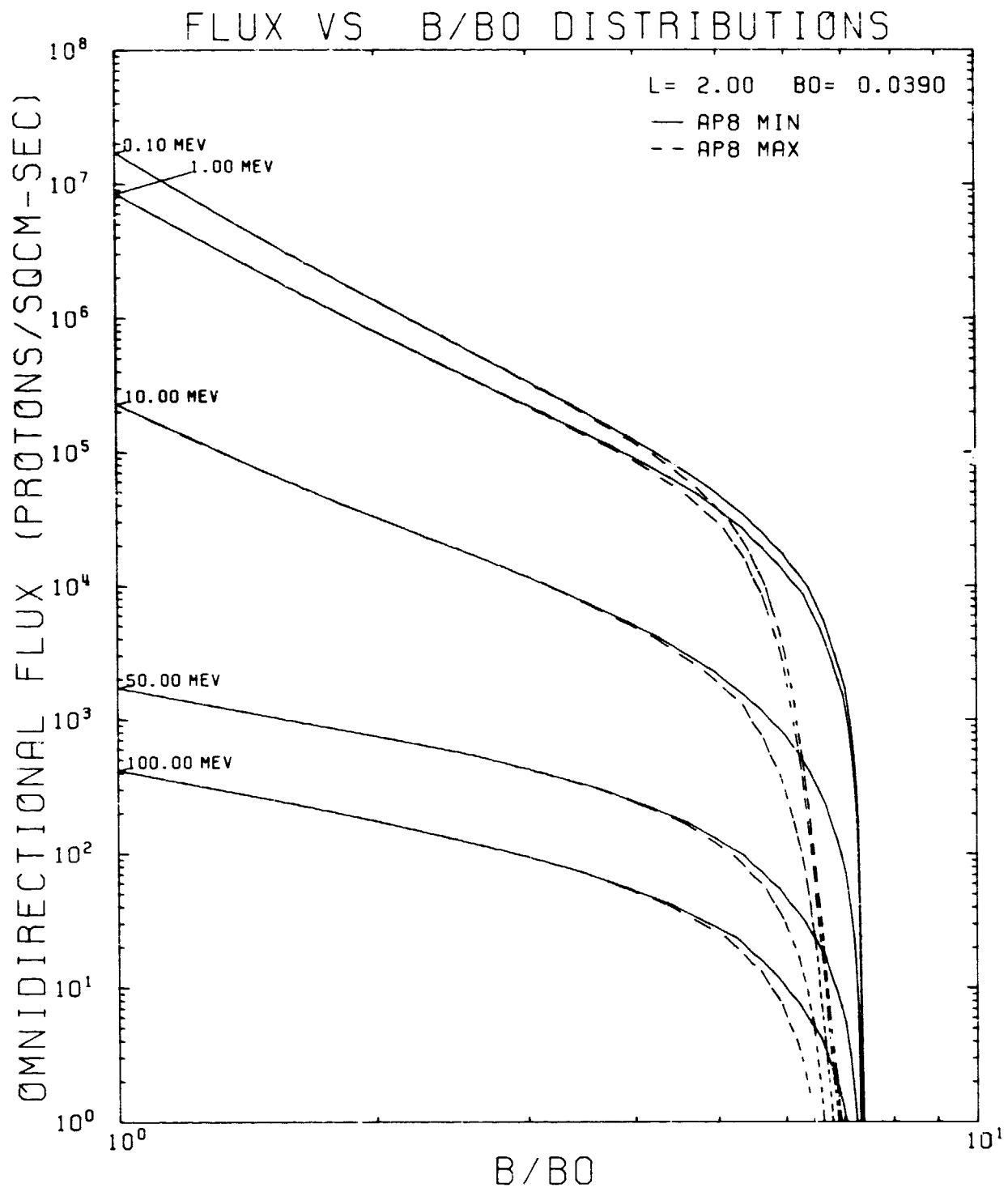
Figure 129. AP8MIN and AP8MAX Flux vs B/B 0 Comparison Plot for L = 2.00 R E
