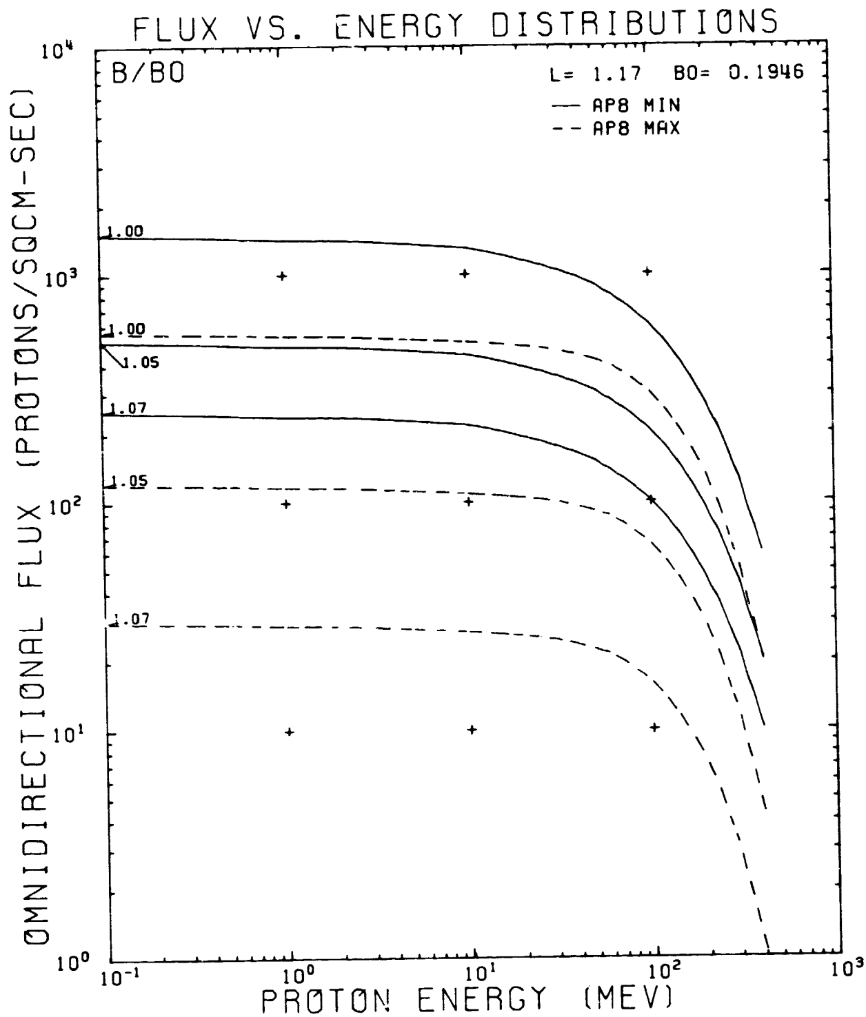
Figure 131. AP8MIN and AP8MAX Flux vs Energy Comparison Plot for L = 1.17 R_E
