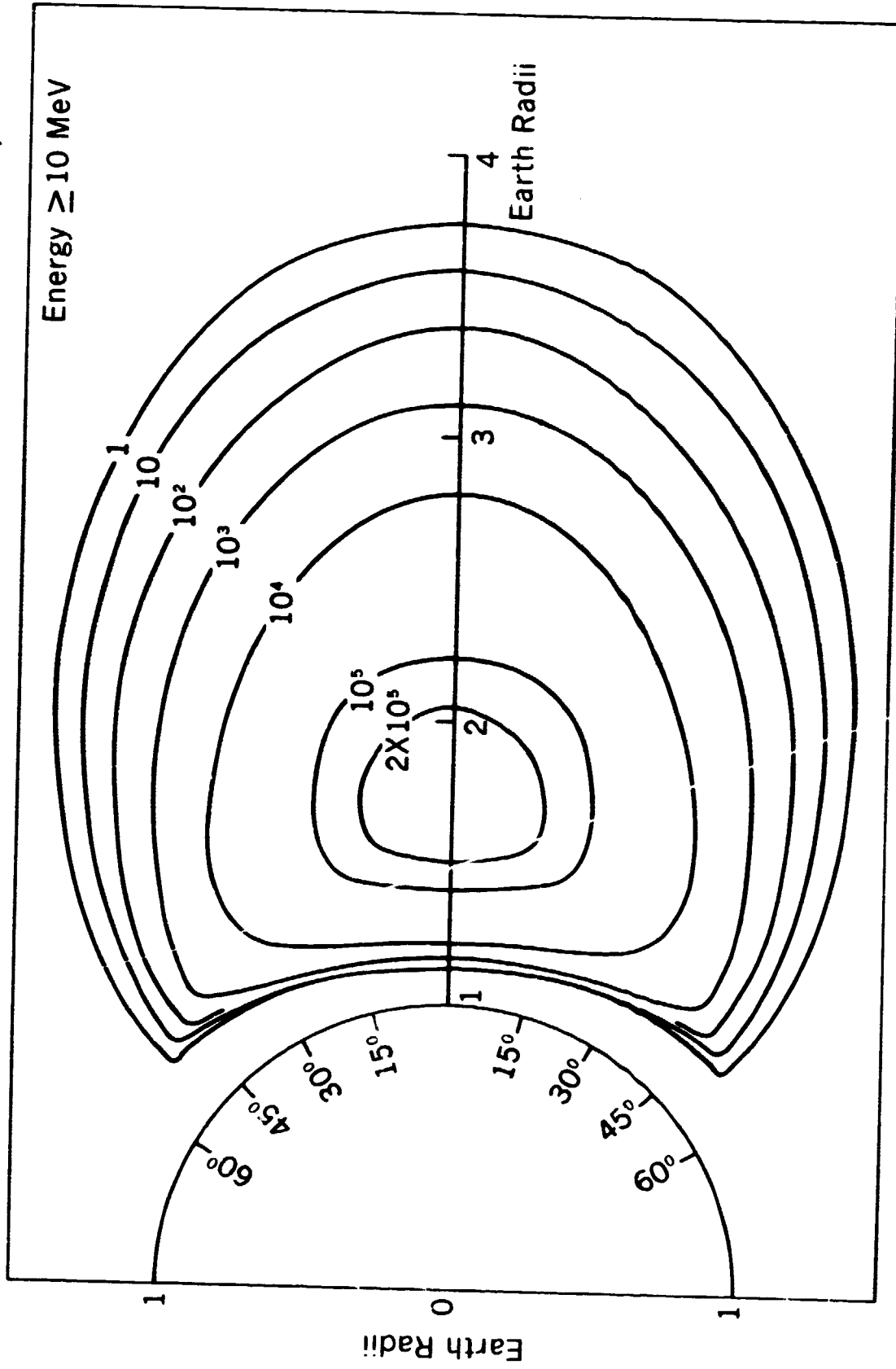
Figure 67. AP8MIN R- \lambda Plot of Constant Intensity Flux Contours with an Energy of \geq 10 MeV
