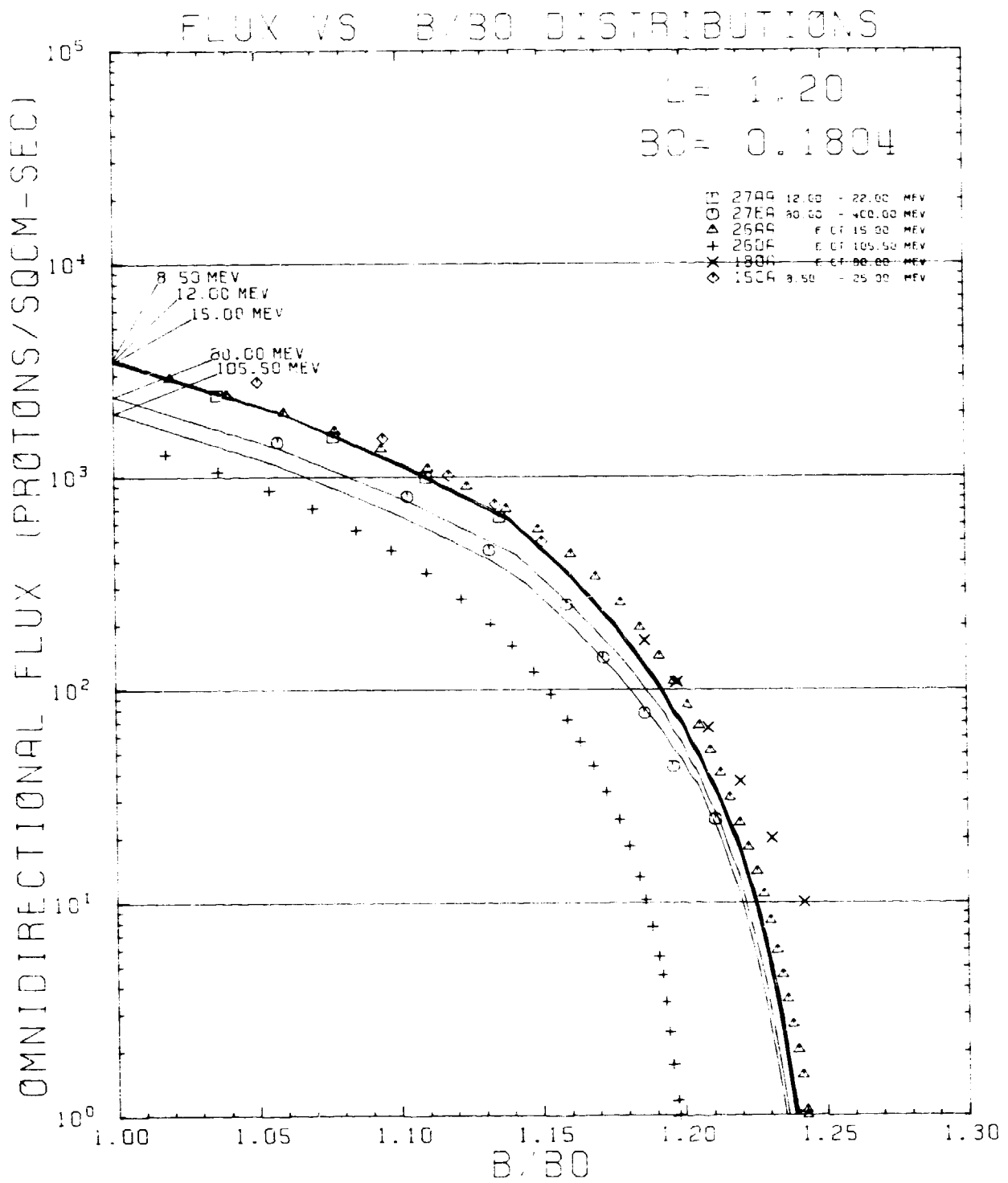
Figure 98. AP8MIN and Data Flux vs B/B 0 Comparison Plot for L = 1.20 R E
