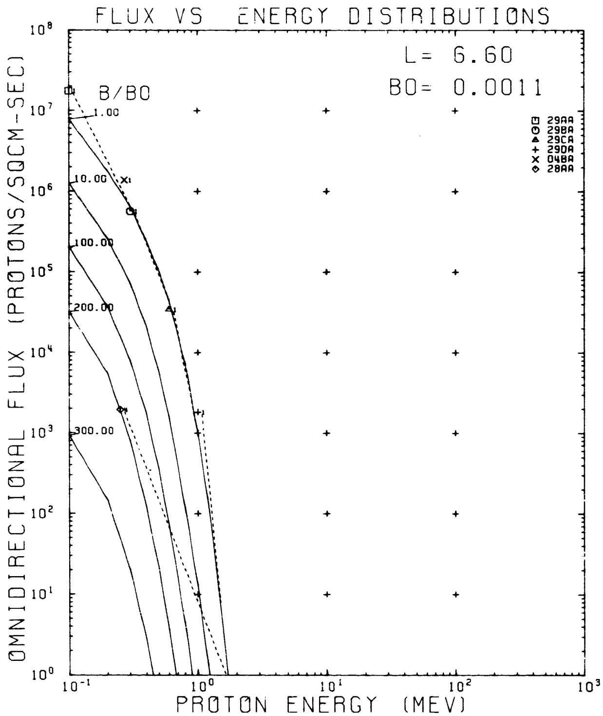
Figure 115. AP8MIN and Data Flux vs Energy Comparison Plot for L = 6.60 R E
