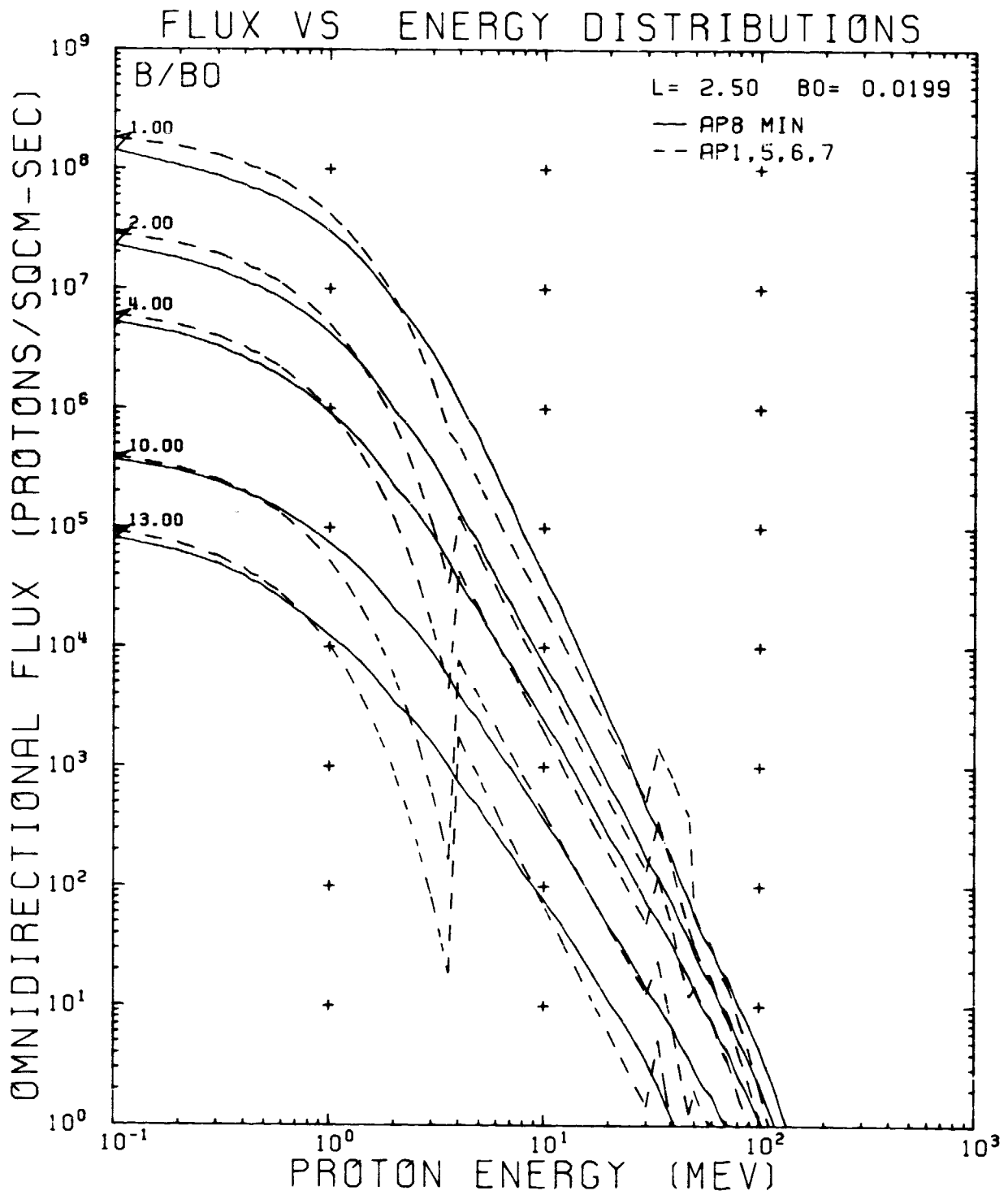
Figure 147. AP8MIN and AP-1, -5, -6, and -7 Flux vs Energy Comparison Plot for L = 2.50 R E
