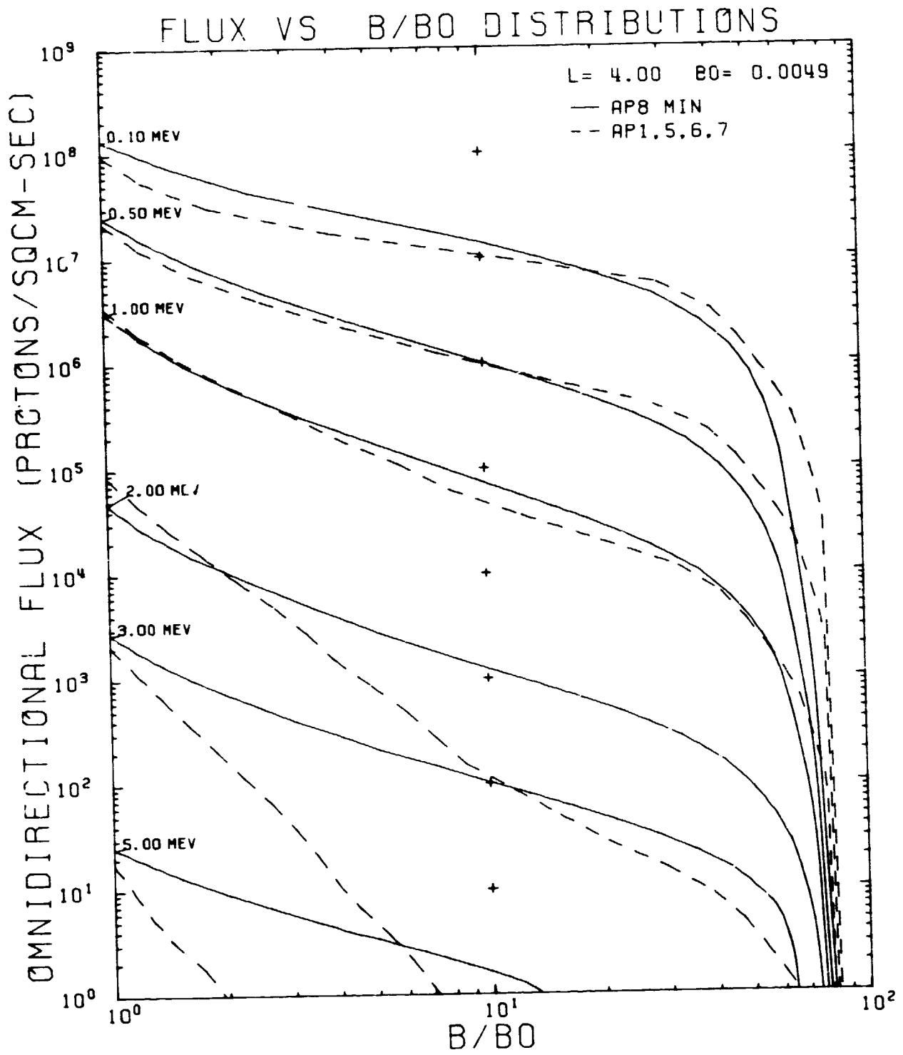
Figure 141. AP8MIN and AP-1, -5, -6, and -7 Flux vs B/B 0 Comparison Plot for L = 4.00 R E
