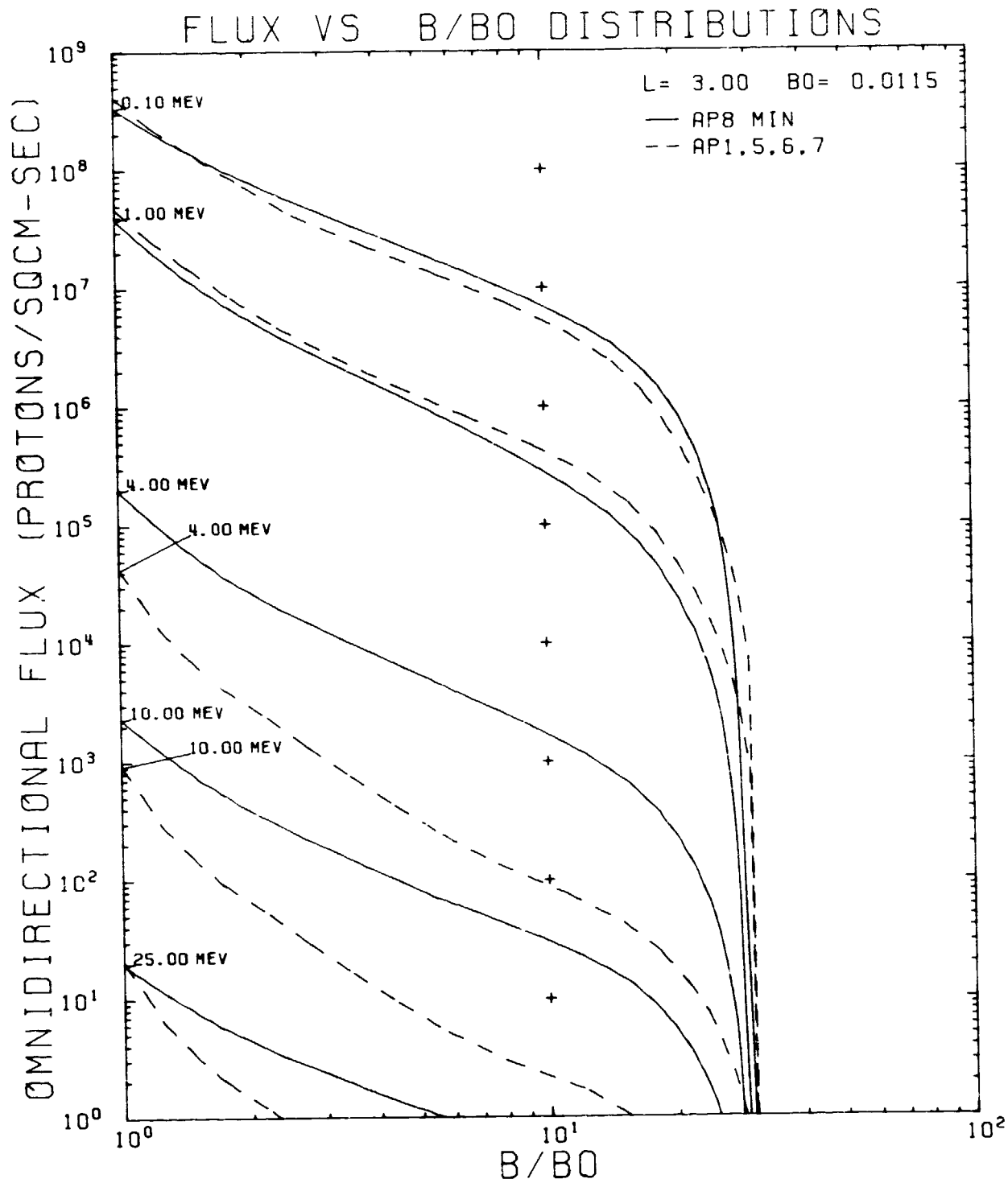
Figure 140. AP8MIN and AP -1, -5, -6, and -7 Flux vs B/B 0 Comparison Plot for L = 3.00 R E
