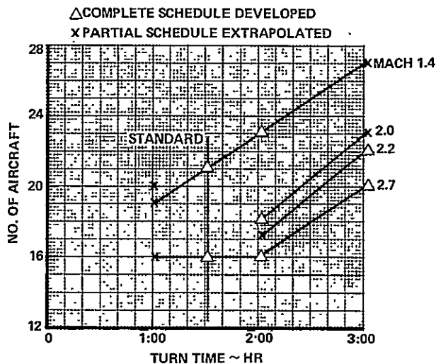
Figure 9. Effect of turn time on fleet size
