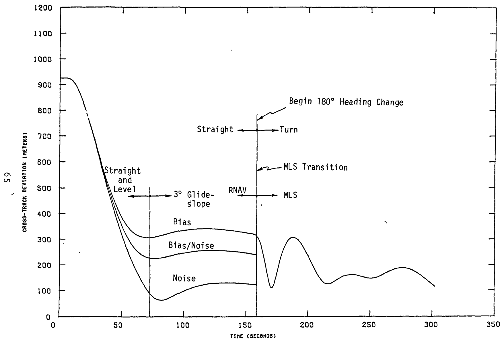
Figure 4.19 Cross-Track Deviation for 180° Turn to Final, DME/DME, Facilities A
