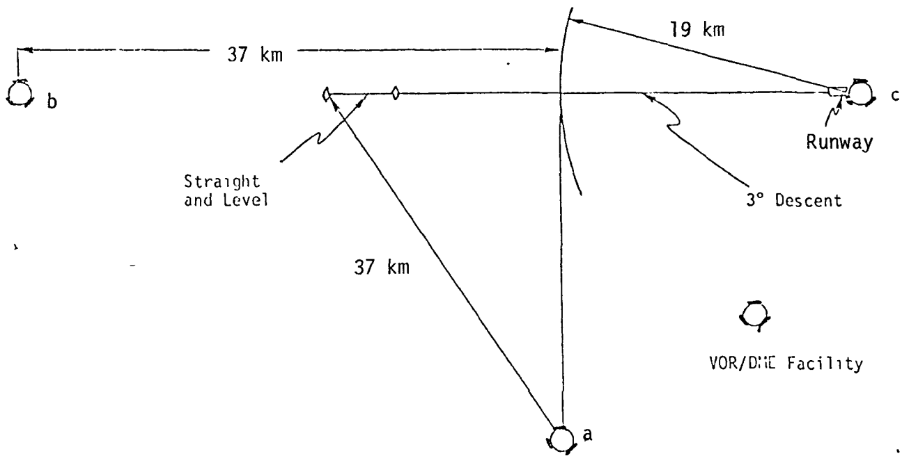
Figure B.4 Straight-In Approach for VOR/DME Navigation Mode
