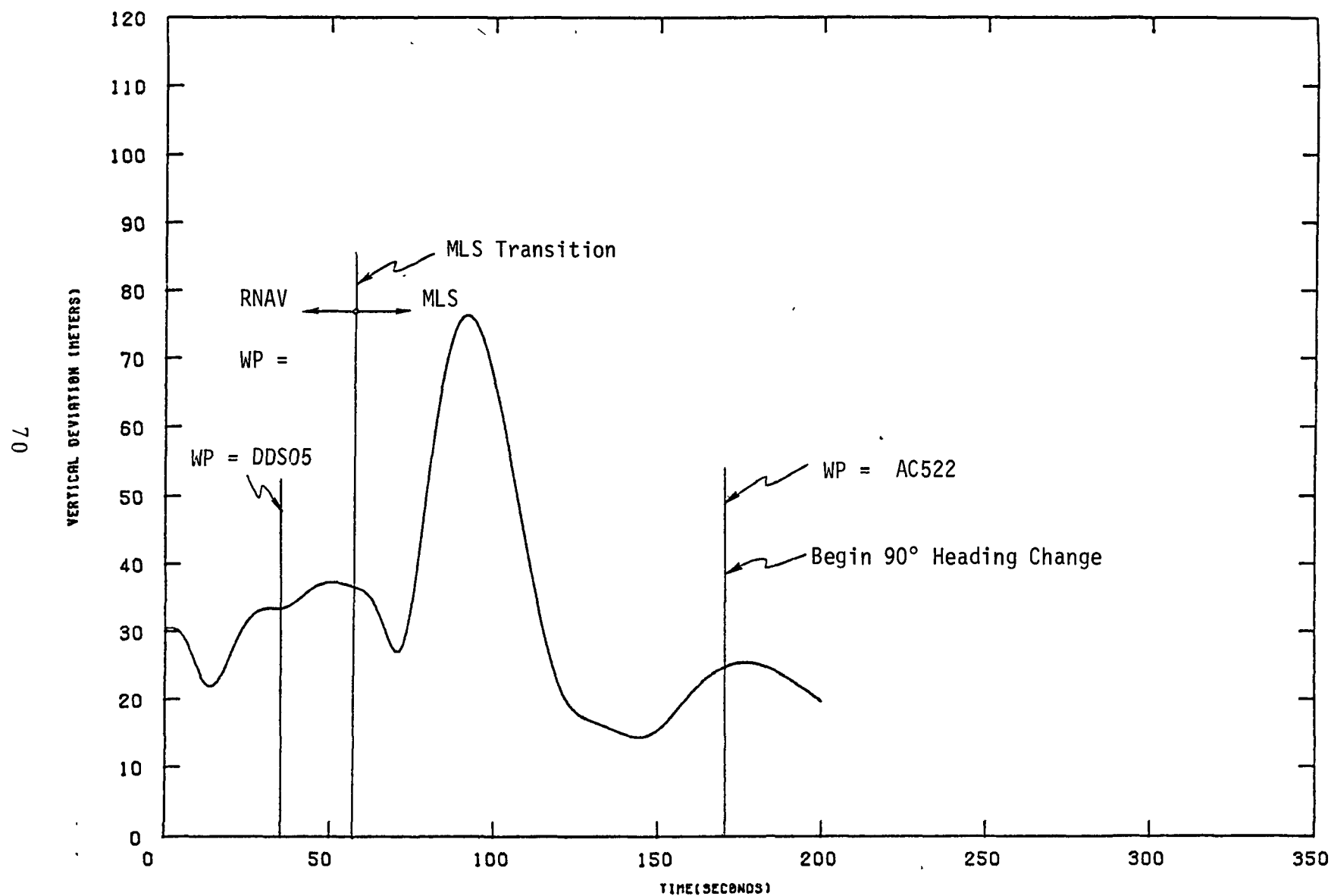
Figure 4.24 Vertical Deviation Time History for S-Turn ICAO Profile
