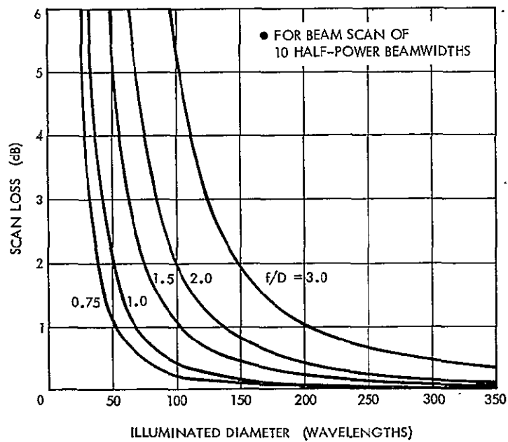
Figure B-6. Parabolid Scan Loss Due to Aperture Blockage
