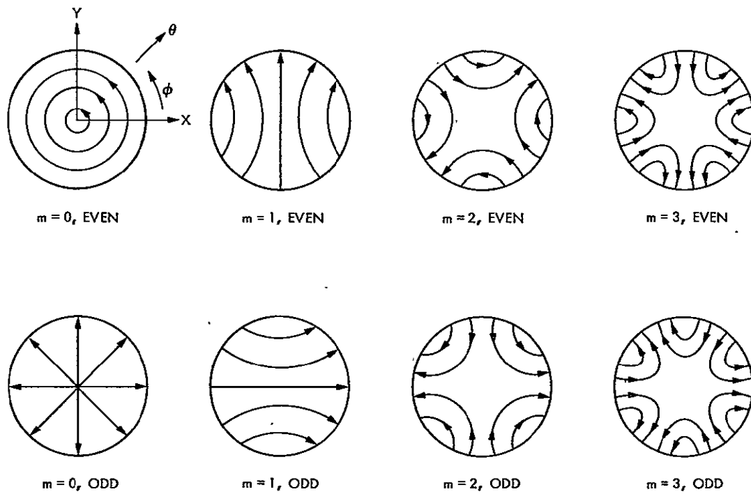
Figure 4-4. Field Lines, Fourier Components
