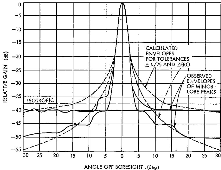
Figure 4-7. Surface Tolerance Effects on Radiation Patterns
