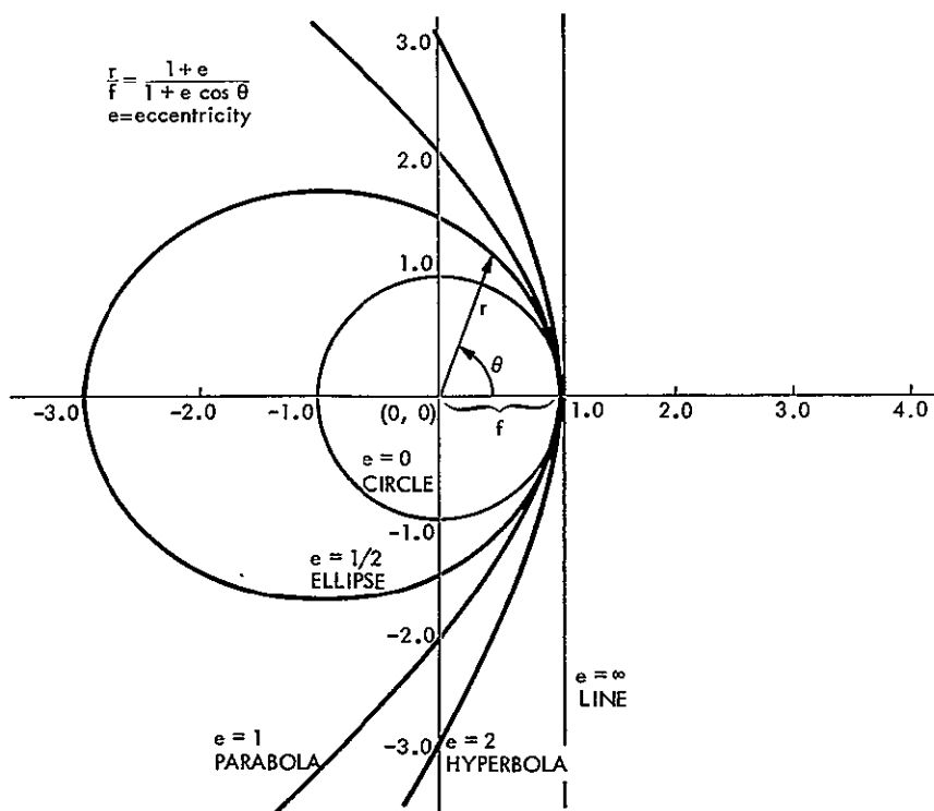
Figure 3-3. Conic Sections
