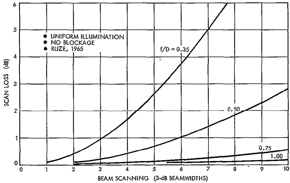
Figure B-5. Parabolid Scan Loss
