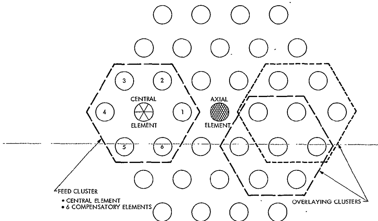
Figure A-1. Feed Array
