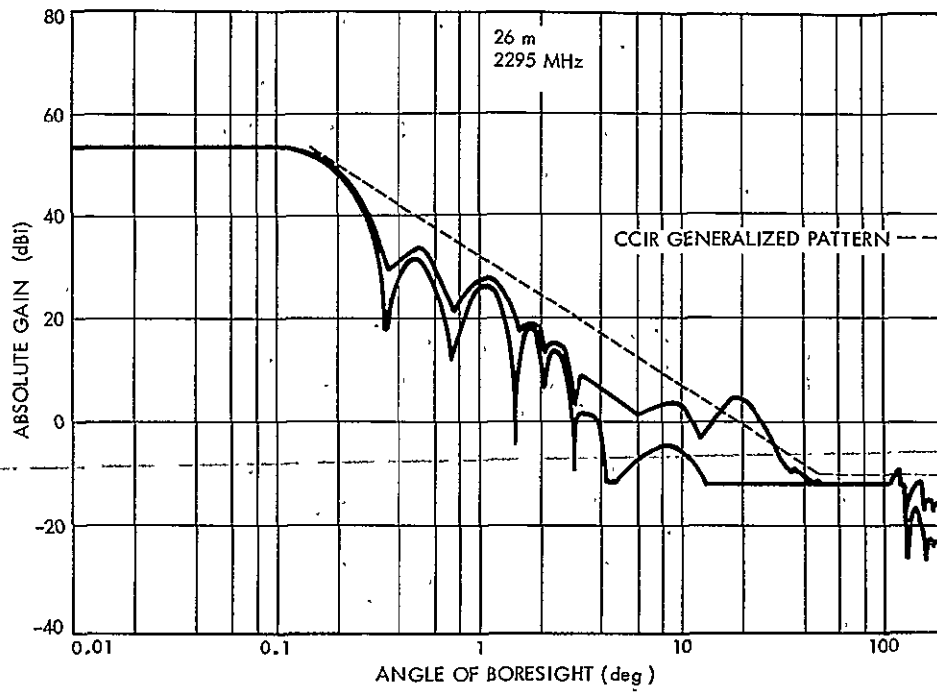
Figure 4-10. Calculated Radiation Pattern Envelopes, D/\lambda = 200
