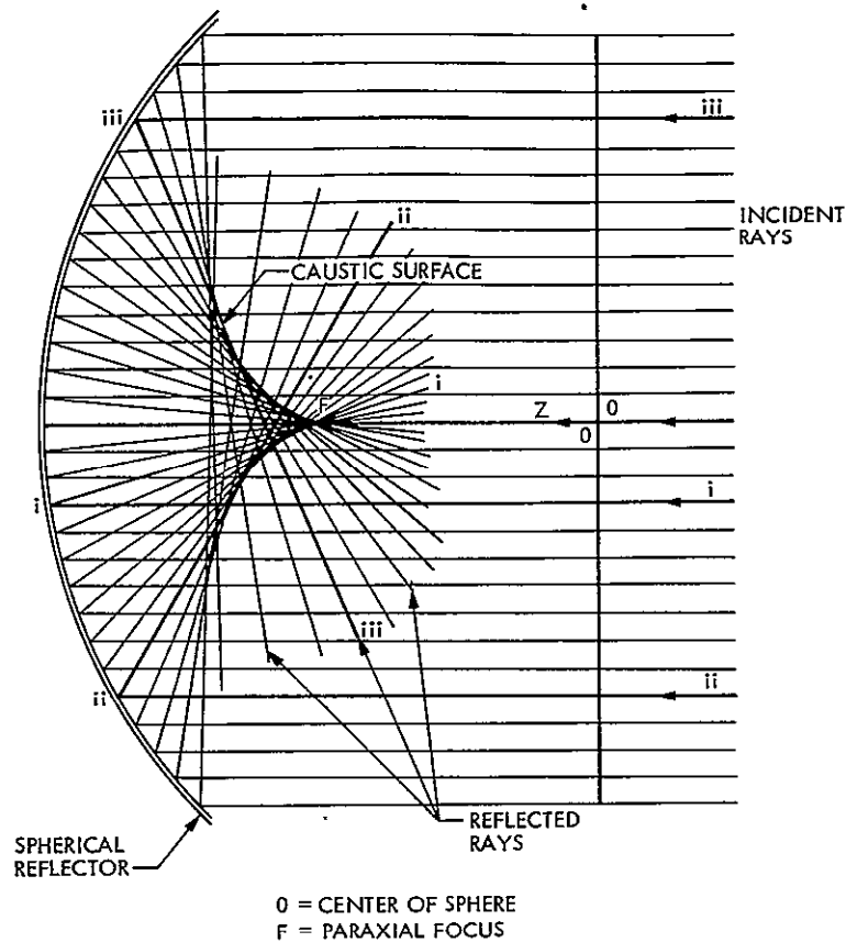
Figure 3-4. Spherical Reflector
