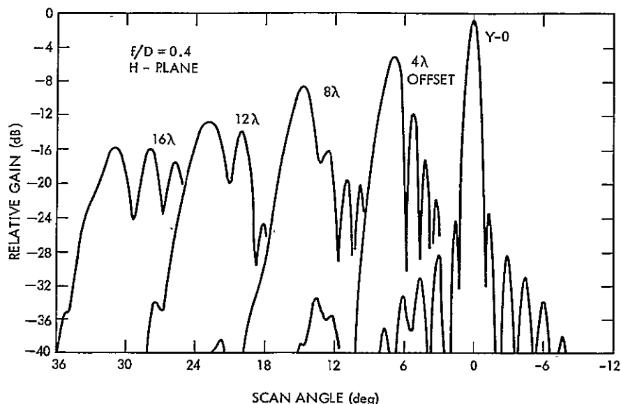
Figure 3-5. Measured Secondary Patterns as a Function of Lateral Primary Feed Displacement
