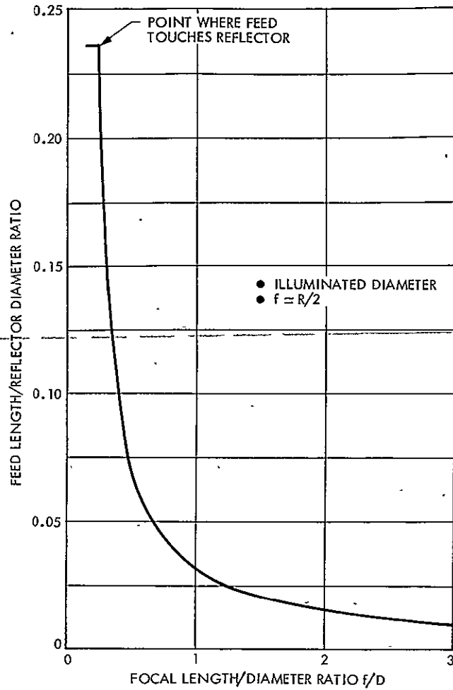
Figure B-4. Spherical Reflector Axial Focal Region Length
