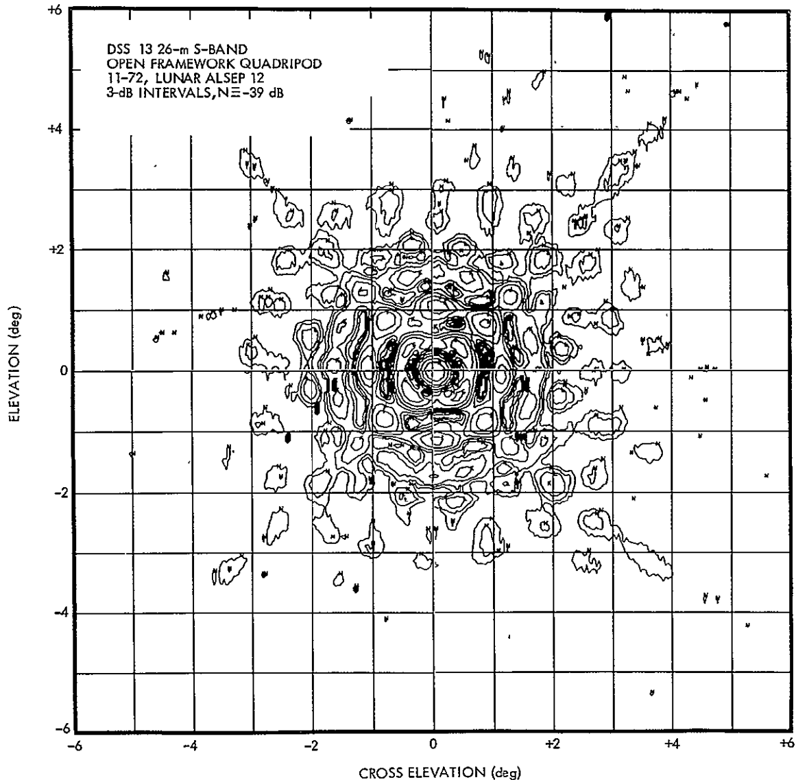
Figure 4-9. Antenna Pattern Contour
