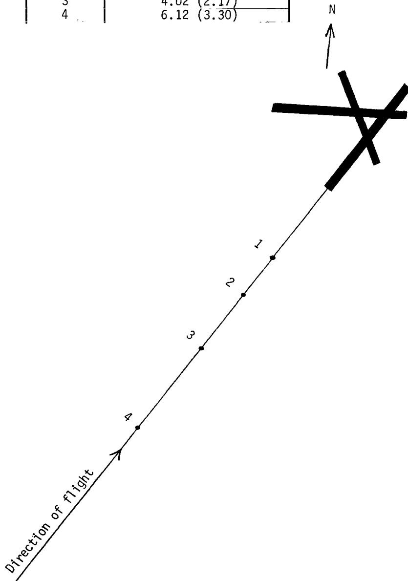
Figure 3.- Microphone locations.
