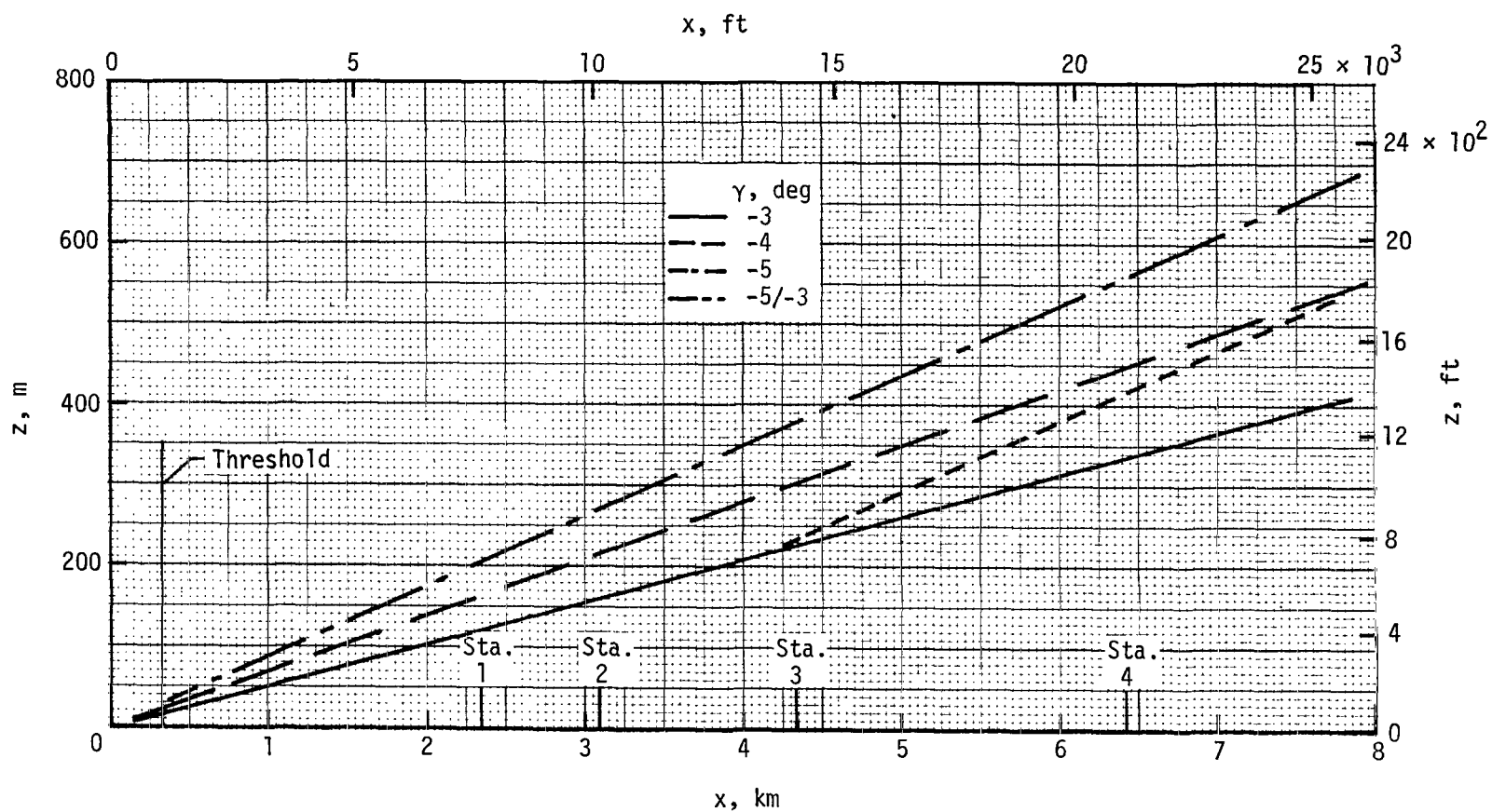
Figure 4.- Flight profiles.
