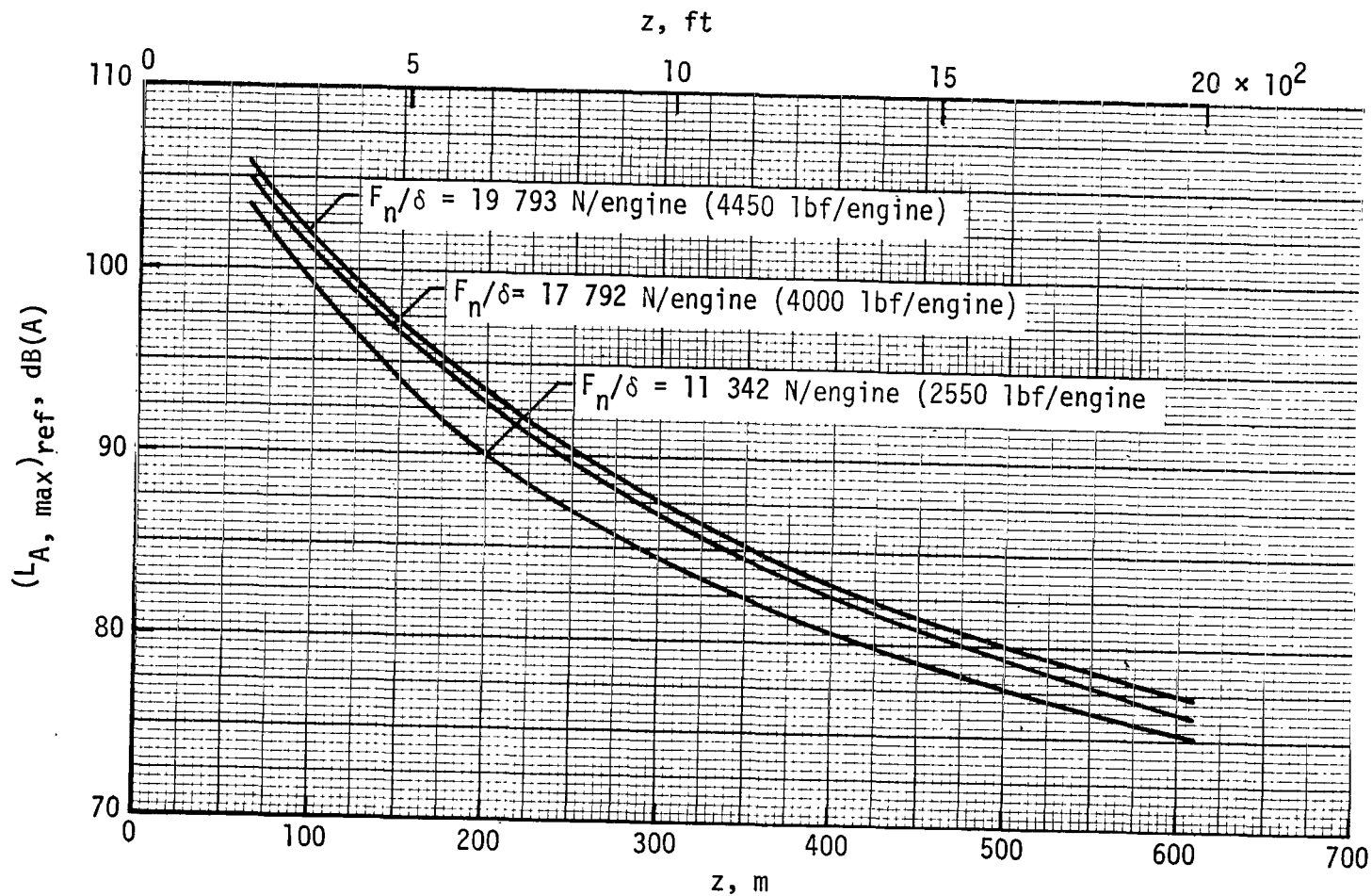
Figure 11.- Variation of (L_{A, \max})_{\text{ref}} with vertical distance for three thrust levels representative of current and advanced approach techniques.
