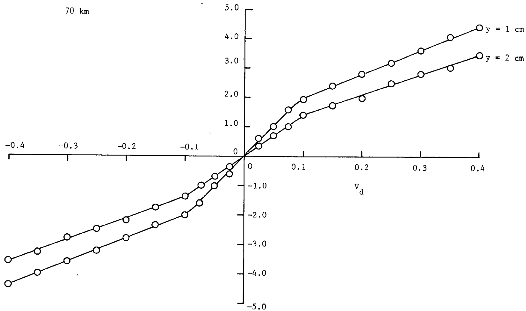
Figure 5.7 Current-Voltage Characteristics for Ion and Electron Collection in Static Plasma by the Scaled Blunt Probe at 70 km
