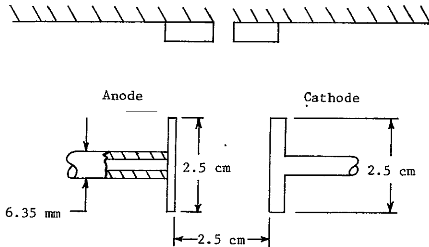
(B) Electrodes for 70 km Altitudes
