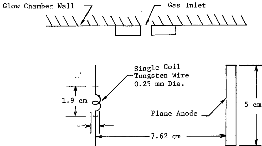
(A) Plane Anode and Coiled Tungsten Filament
