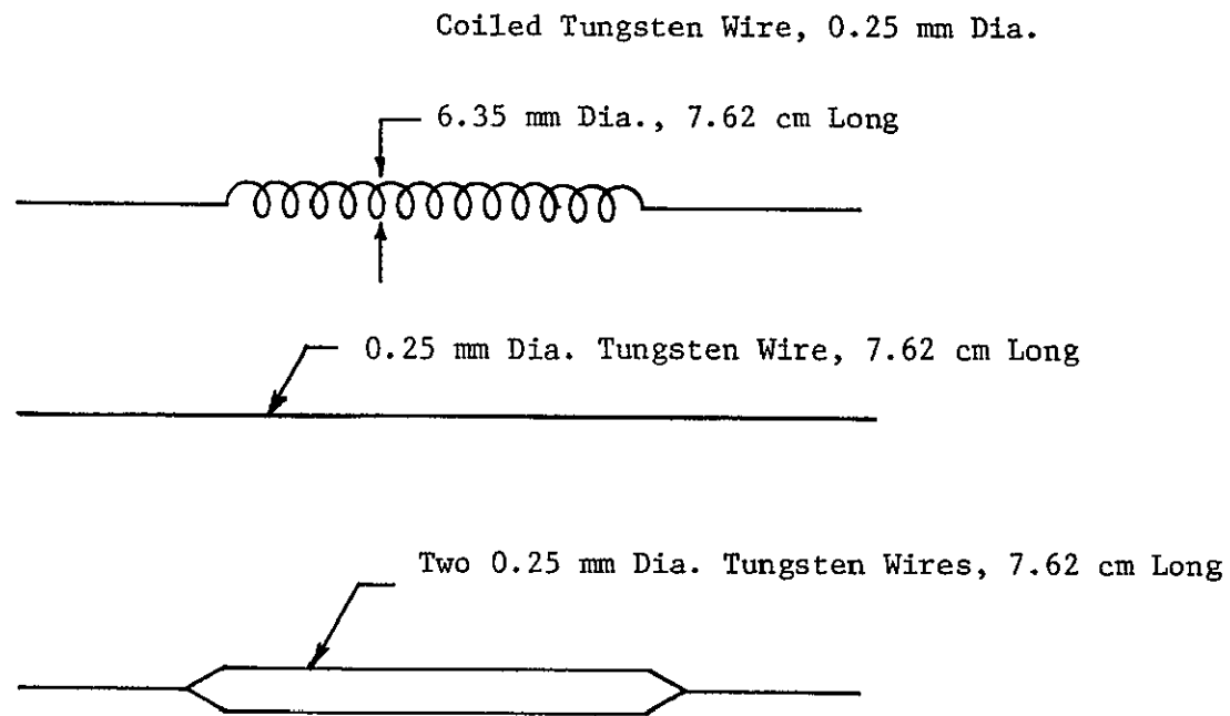
Figure 2.9 Resistance Heating Filaments
