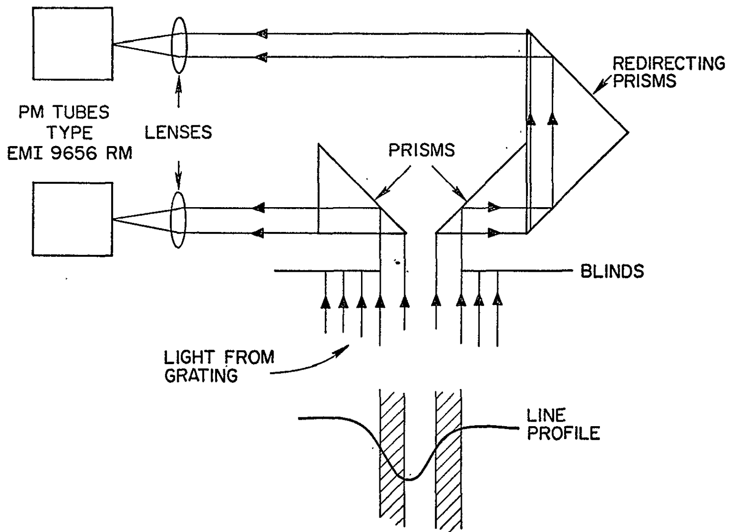
Figure 7. Diagram of exit slits used in the Stanford Solar Observatory. Light is collected from the wings of an absorption line and sent to each of two matched phototubes for measurement.
