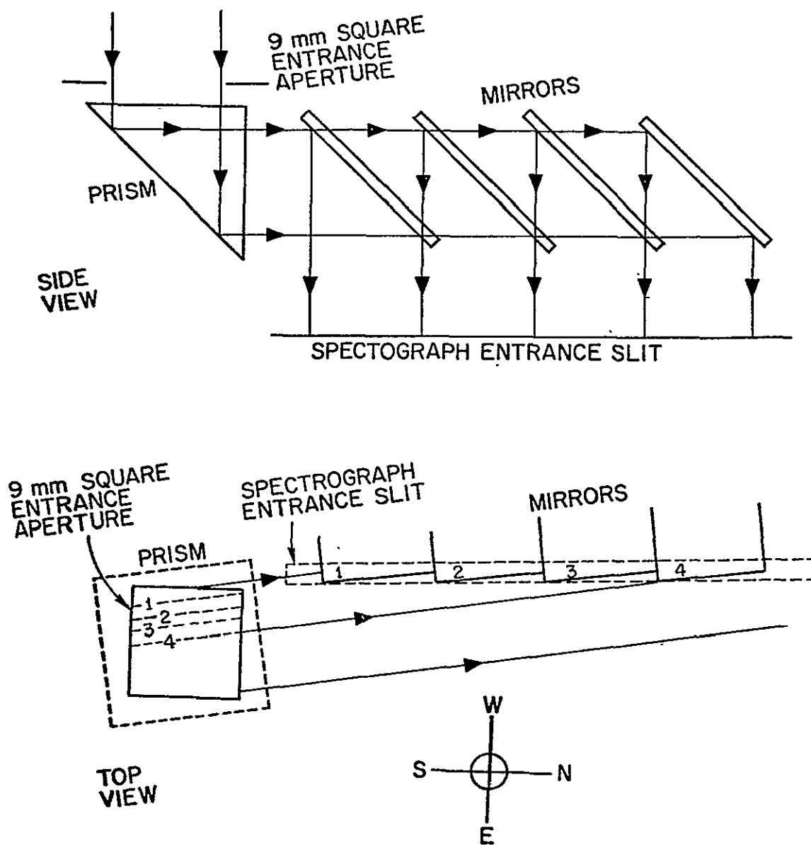
Figure 5. Diagram showing side view (top) and top view (bottom) of an image slicer. Only four of the ten slices are illustrated.
