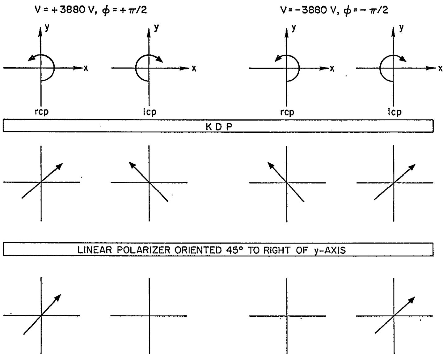
Figure 4. Diagram showing how a KDP with a linear polarizer oriented 45^\circ to the right of the slow axis can be used to pass only right circularly polarized light for a potential applied in one direction, and left circularly polarized light for the opposite potential.
