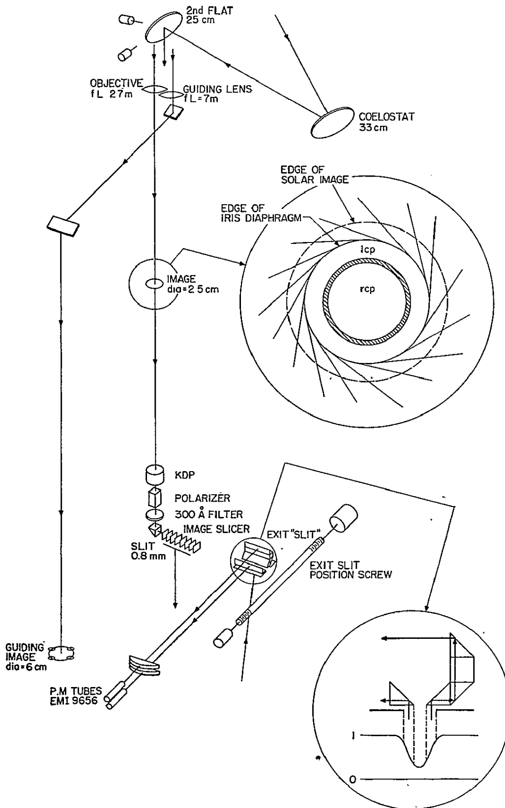
Figure 3. Optical diagram of the Stanford Solar Observatory
