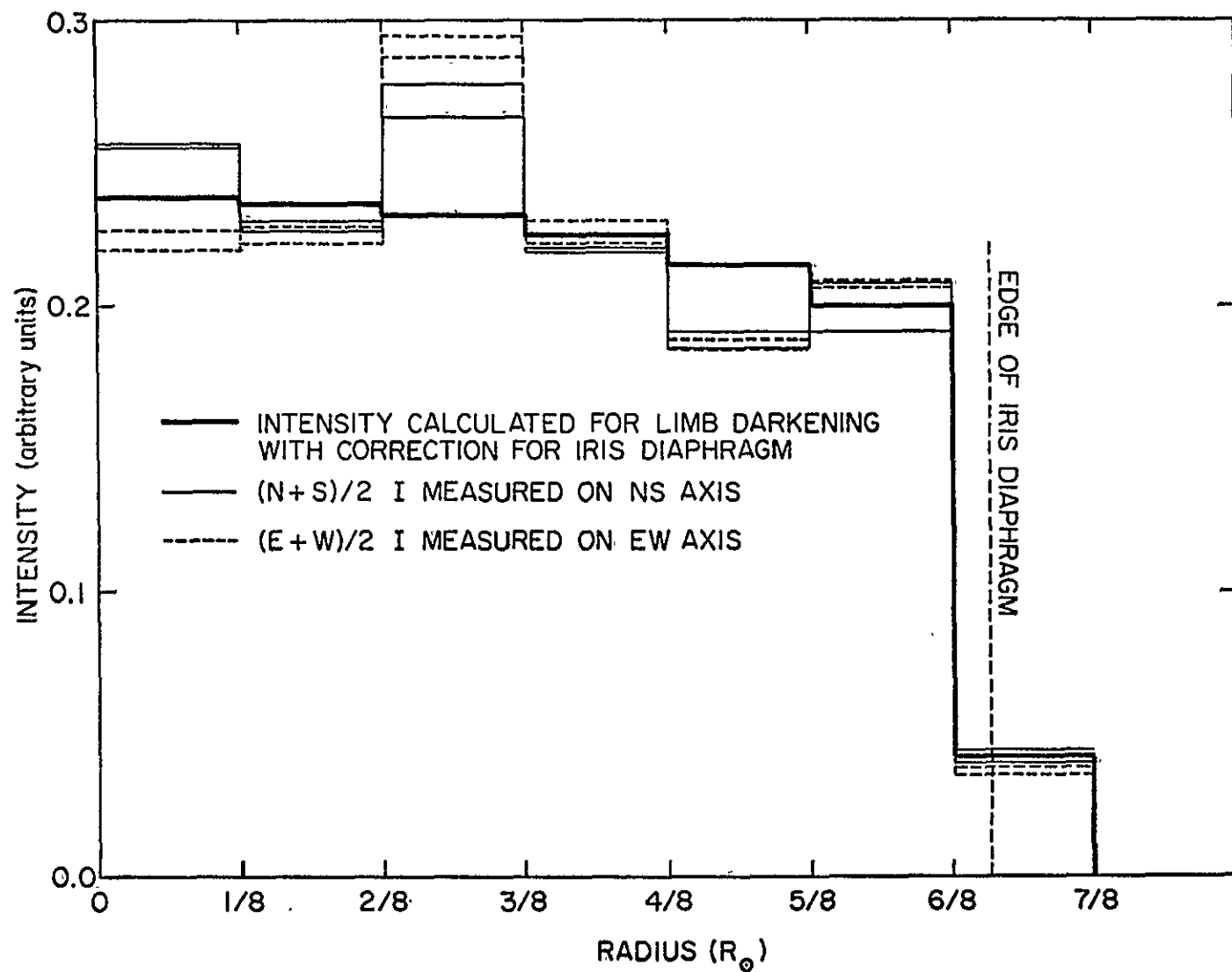
Figure 18b. Intensity as a function of radial position on the solar image, taken from the map shown in Figure 17. The value calculated from the limb darkening expression of Allen (1973) is again included for comparison.
