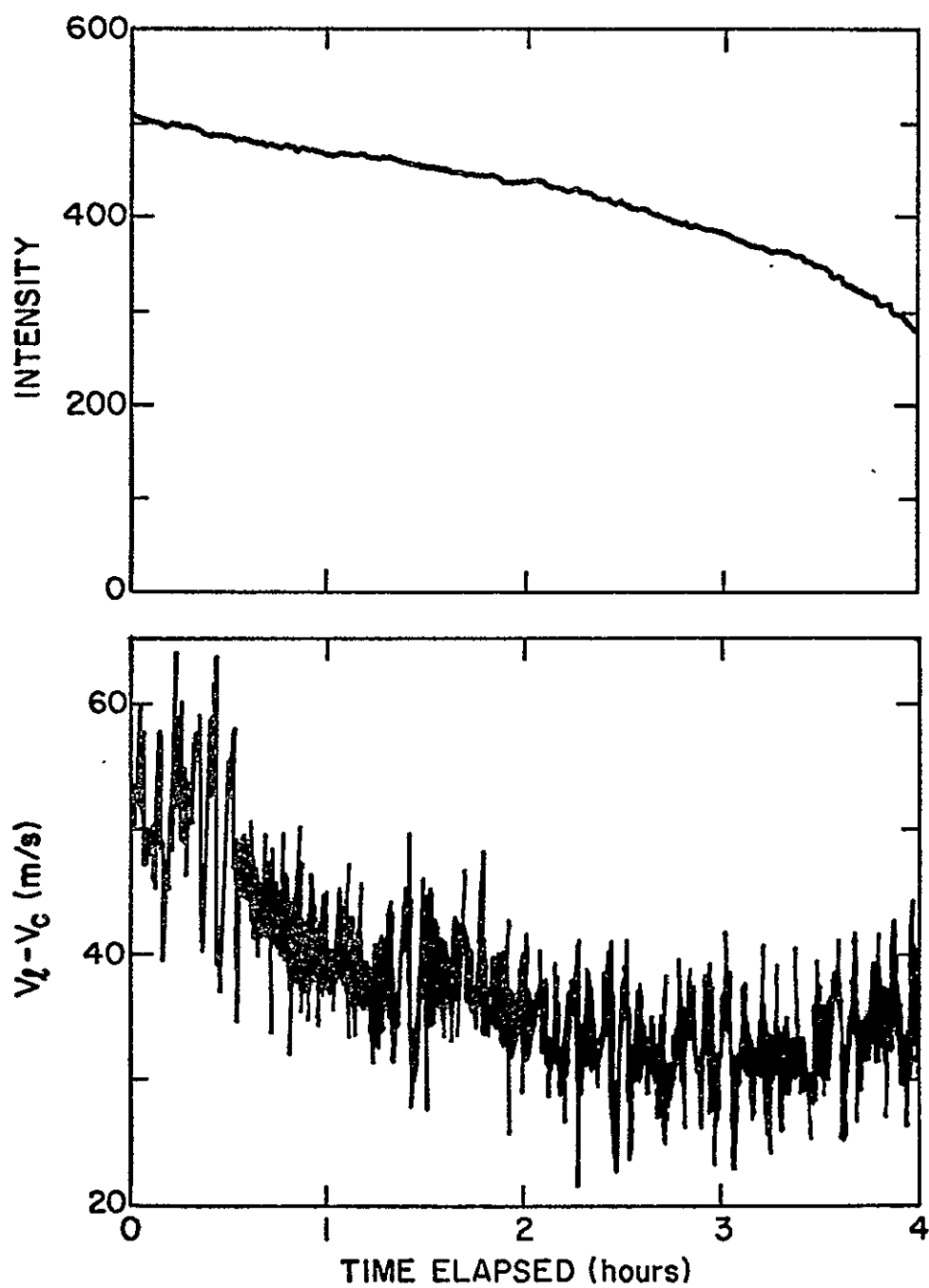
Figure 19. Plots of intensity (top) and ZI signal calibrated in relative velocity (bottom) for the May 23, 1976 observation.
