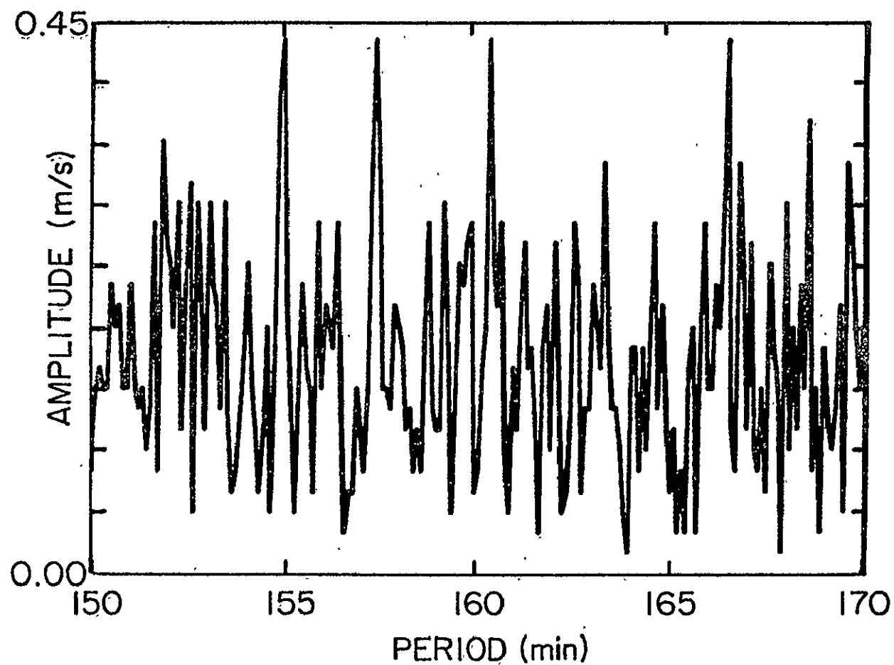
Figure 43. Scan of amplitudes obtained by fitting superposed epochs of 1976 Stanford data at periods from 150.0 min to 170.0 min to sinusoids. Values are multiplied by 1.68 to correct for different polarizer dimensions.
