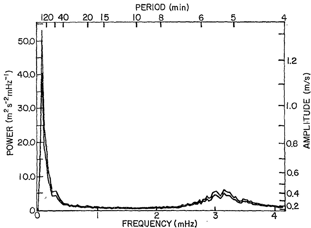
Figure 28. Average power spectrum of the Stanford observations. The power spectra have been computed using the fast Fourier transform algorithm, and observations shorter than three hours have been excluded. In averaging, power spectra are weighted for the length of the observation.
