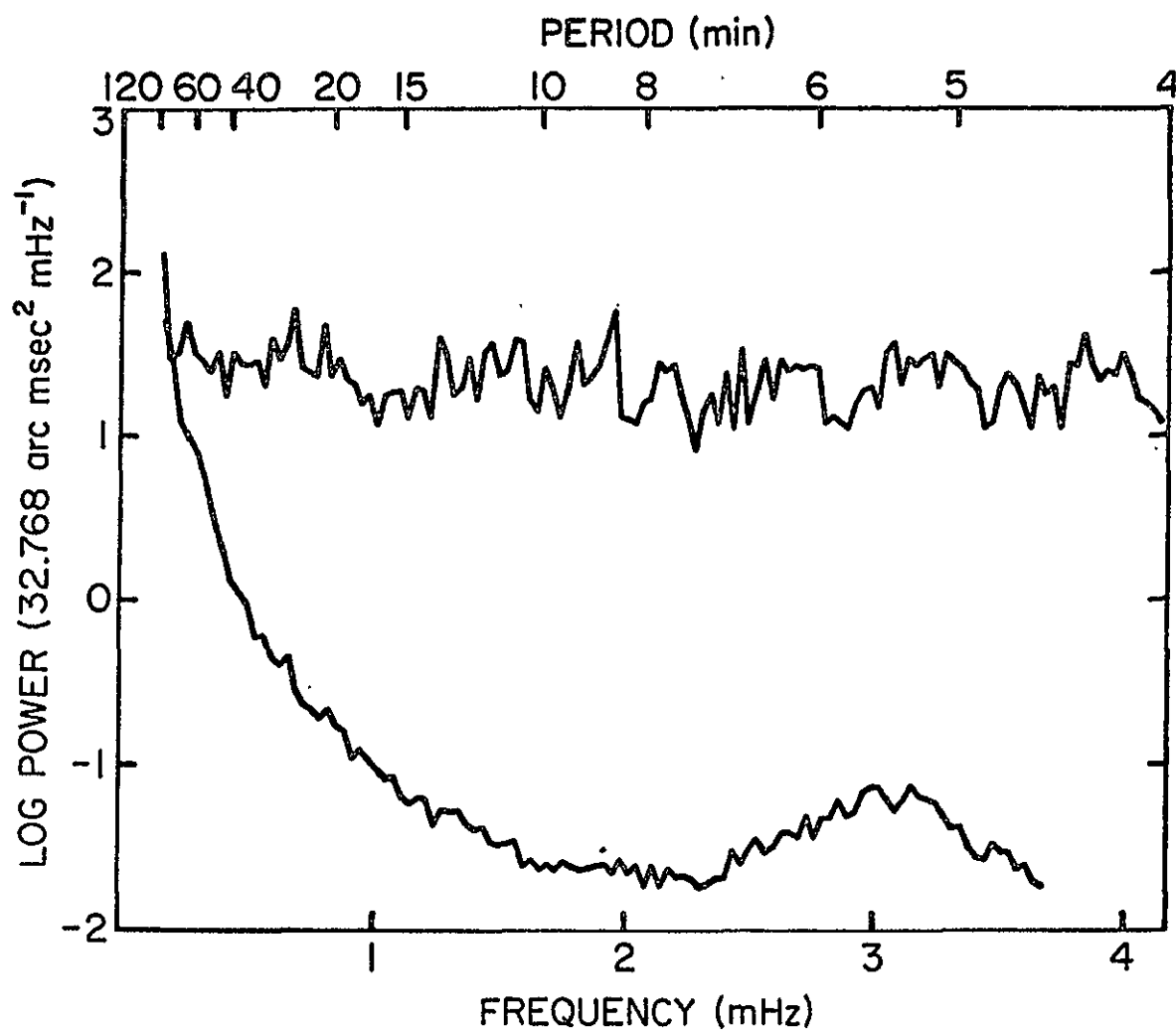
Figure 30. The upper line is the logarithm of the SCLERA power spectrum (Brown et al. , 1976). The lower line is the logarithm of the limb shift produced by mass motions computed from the power spectrum plotted in Figure 29.
