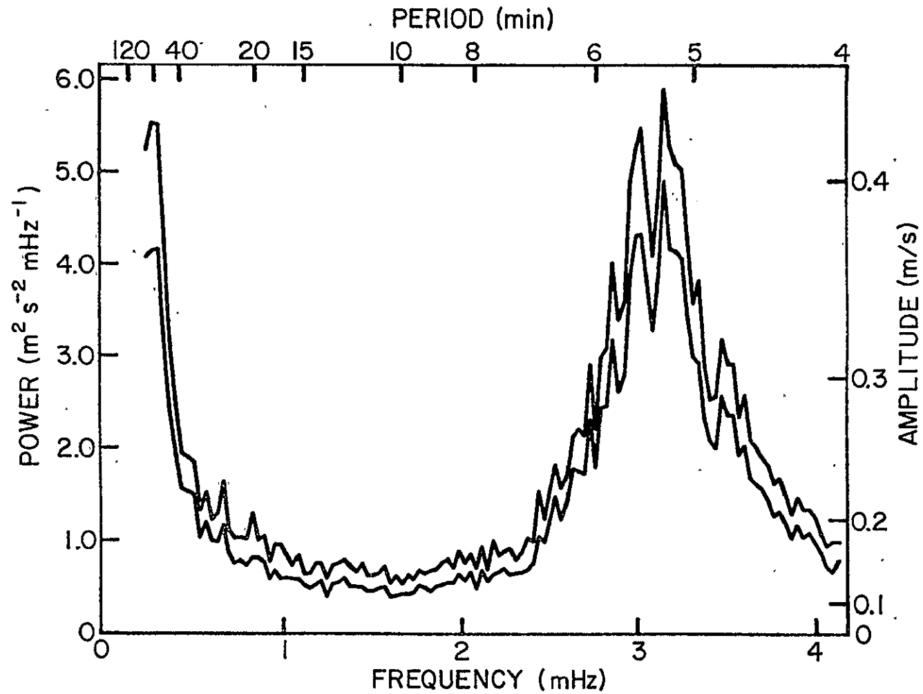
Figure 29. Same as Figure 28, with a different vertical scale. The two lines plotted are the average power plus or minus the standard error.
