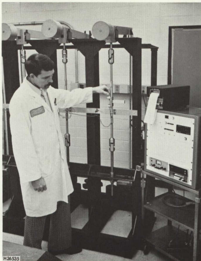
Figure 22. Direct load tests of DCB specimens
