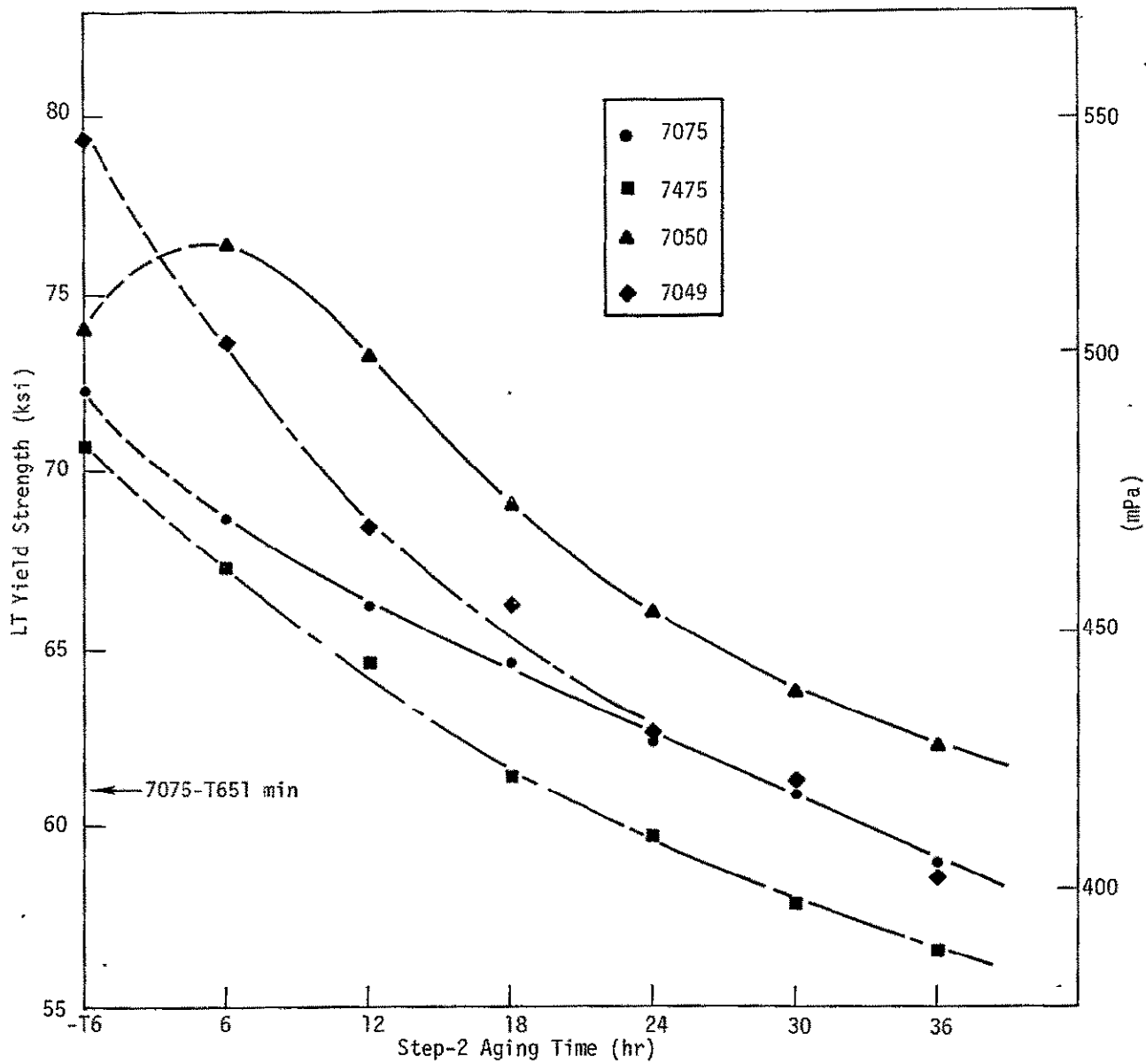
Figure 4. Overaging curves at 165°C (336°F) for 3.0-in. thick plates
