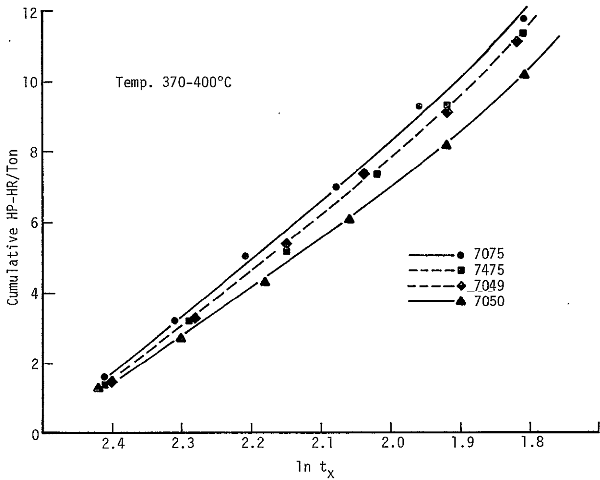
Figure 1. Cumulative deformation energy for hot rolling high-strength aluminum alloys from 12-in. ingot to 6-in. slab
