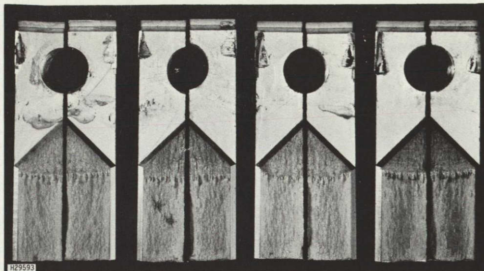
Fracture Surfaces 1X
