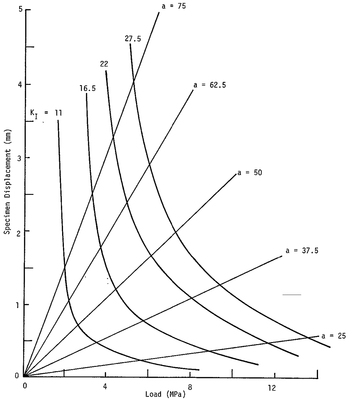
Figure C2. Compliance relationship for uniform DCB specimen
