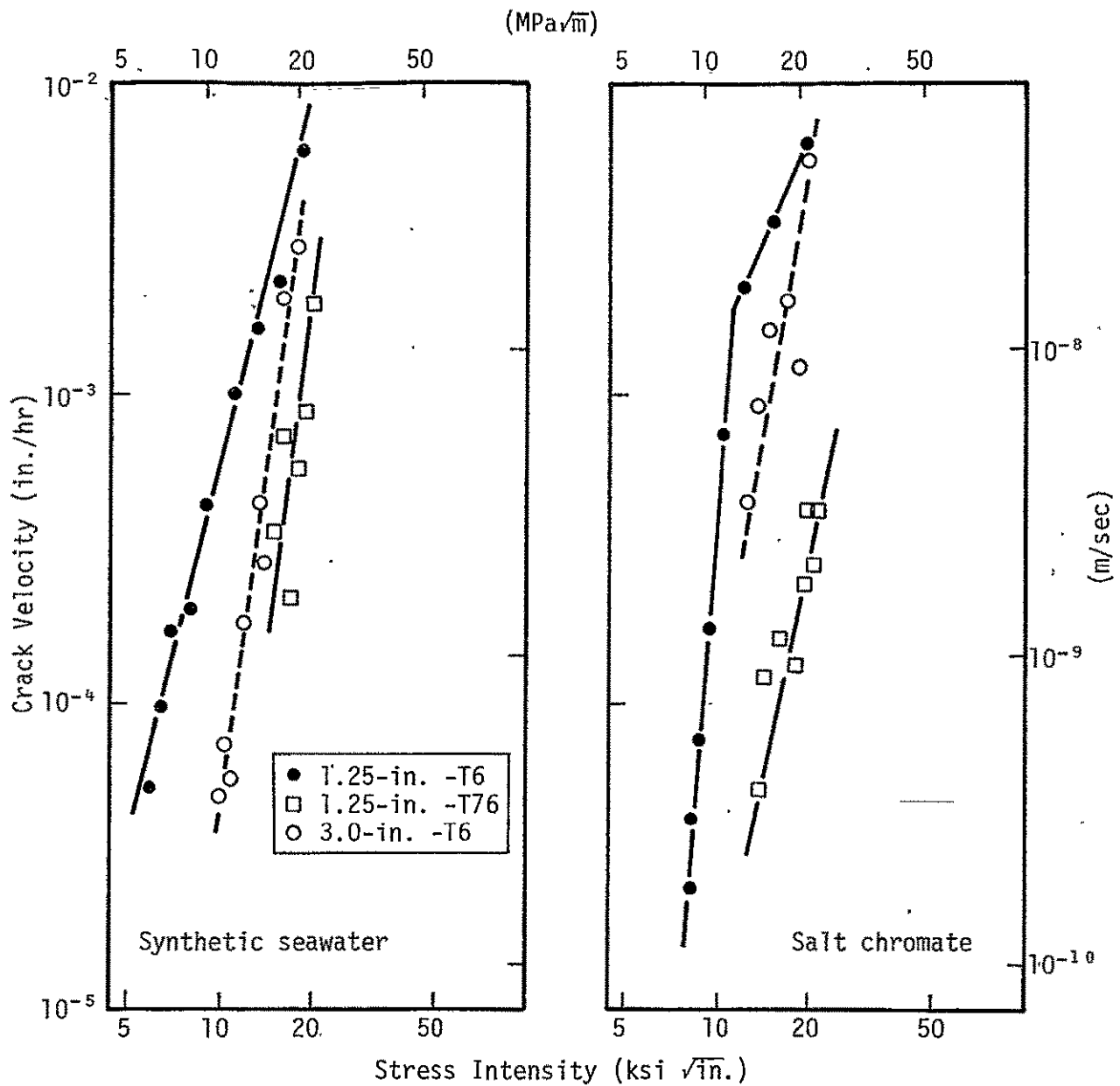
Figure 60. Comparison of crack velocity - stress intensity relationships for 7075-T6 and 7075-T76 in synthetic seawater and salt-chromate solution
