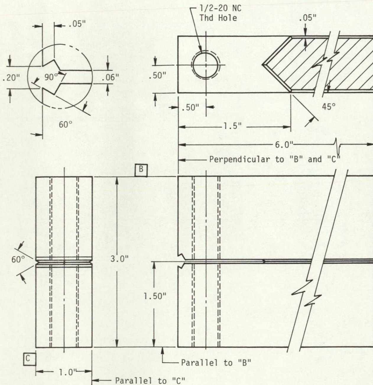
Figure 20. 75-mm constant deflection DCB specimen (All dimensions in inches)
