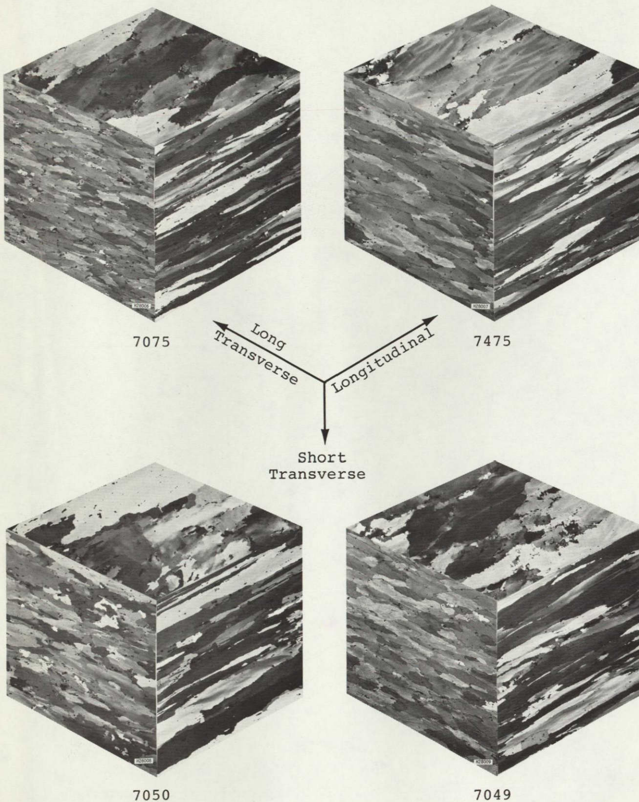
Figure 6. Grain structures of 3-in. thick plates (Barker's etch, polarized light, 25X)
