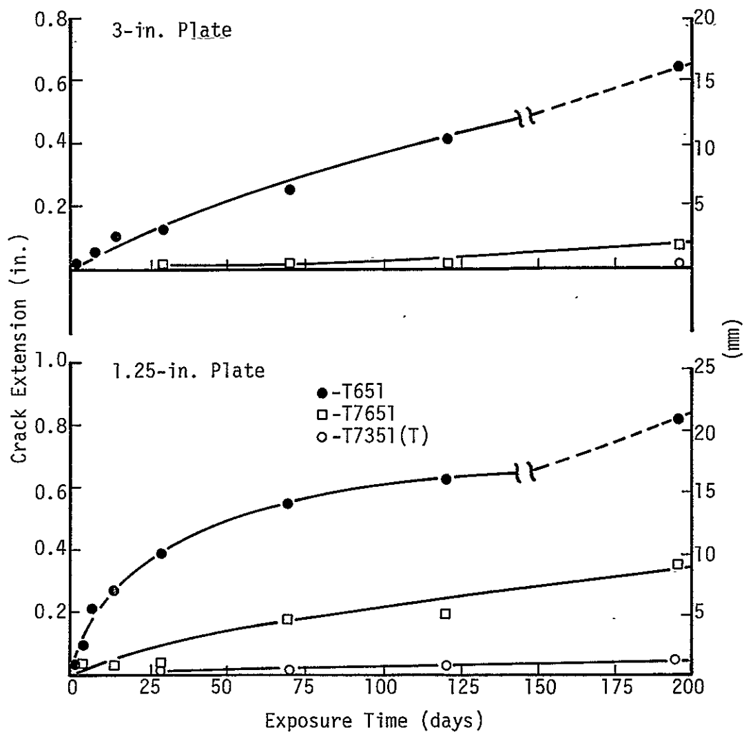
Figure 28. Crack growth in 7075 DCB specimens exposed to marine agmosphere (Daytona Beach): SL orientation, pop-in precrack
