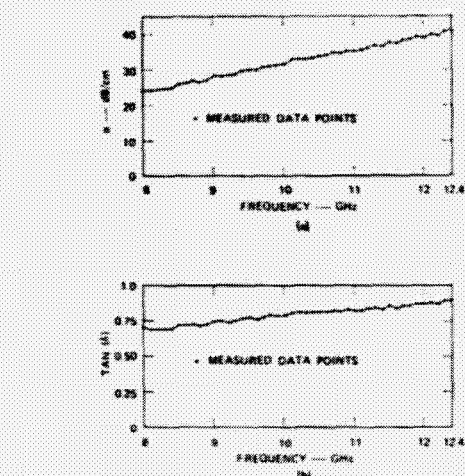
Fig. 4. Measured attenuation and loss tangent of Eccosorb SF-5.5 in the X-band region. (a) Attenuation ( \alpha ). (b) Loss tangent ( \tan \delta ).
