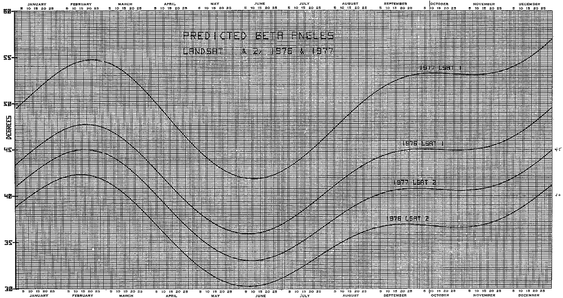
Figure 3-4. Predicted Beta Angles, Landsat 1 & 2, 1976 & 1977
