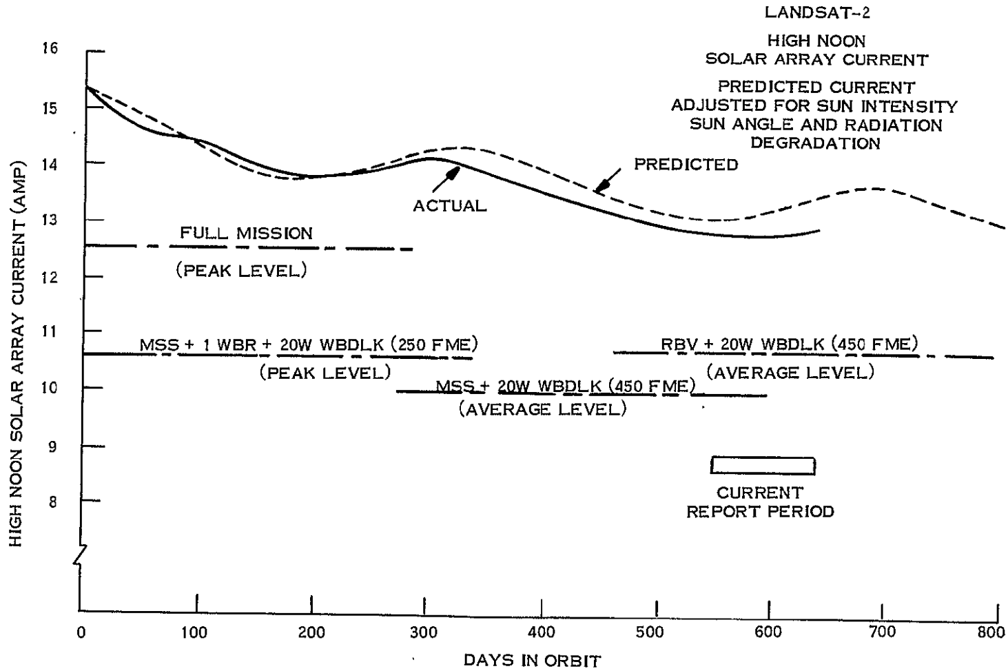
Figure 3-2. Landsat-2 Midday Solar Array Current
