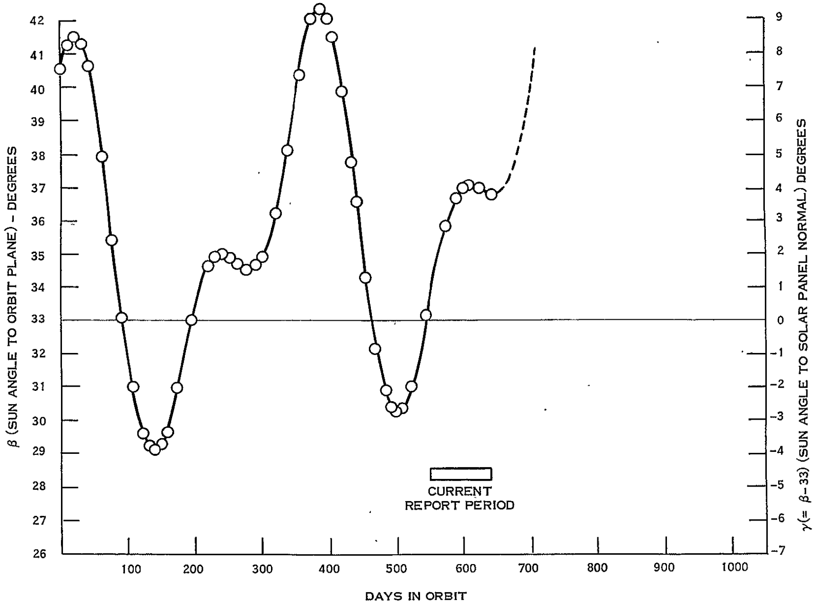
Figure 3-3. Landsat-2 Actual \beta and \alpha (Paddle) Sun Angles
