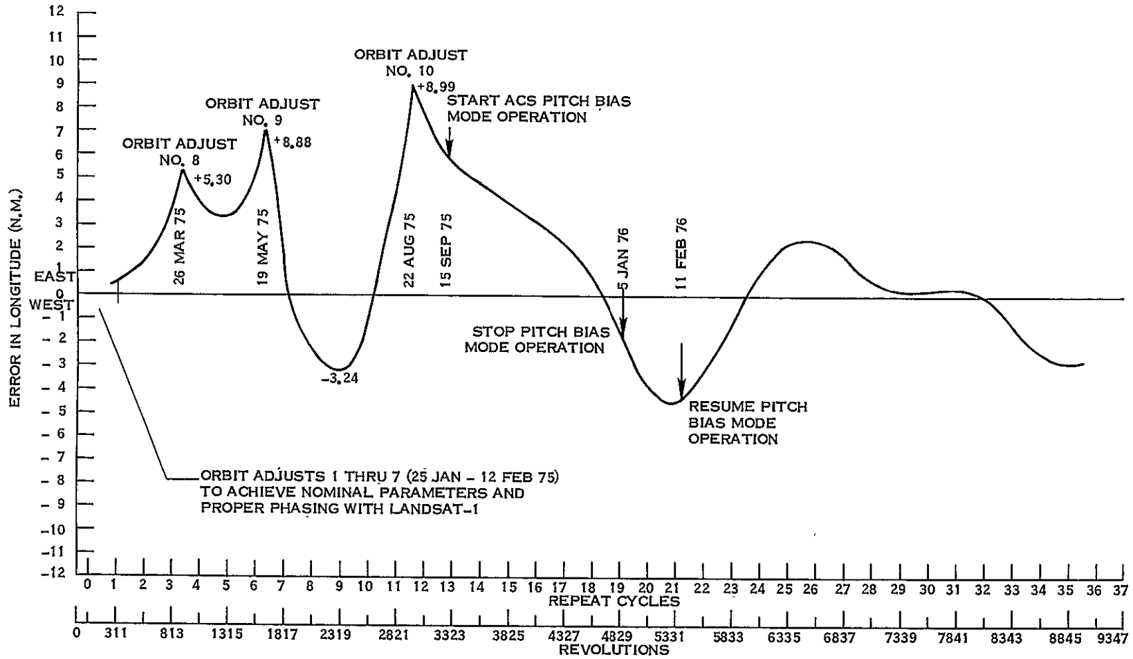
Figure 2-1. Effect of Orbit Adjusts and Pitch Position Bias Orbit Maintenance on Landsat-2's Ground Track
