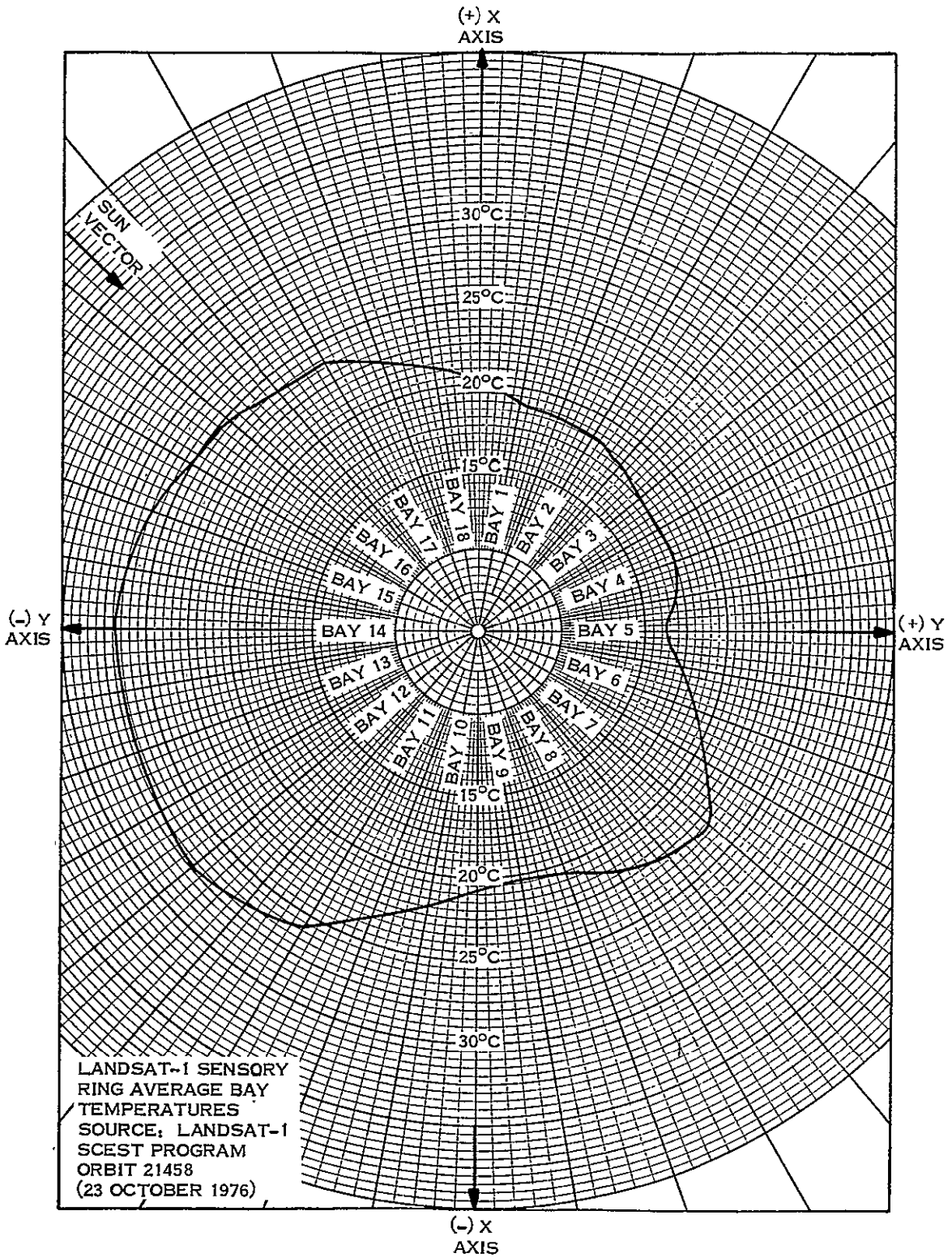
Figure 11-1. Sensory Ring Thermal Profile
