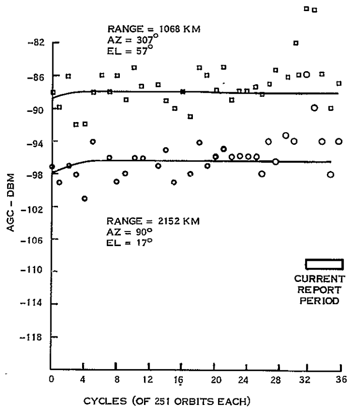
Figure 9-1. USB (Link) AGC Readings at Goldstone with 30' Antenna - Landsat-2
