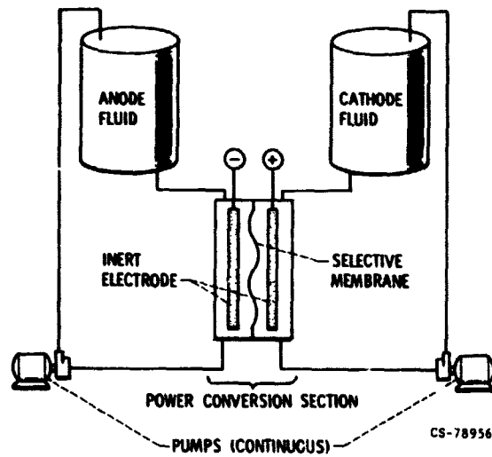
Figure 1. - REDOX system.
