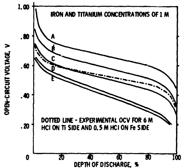
Figure 3. - Theoretical open-circuit voltages for the iron-titanium redox cell at varying acidities.
