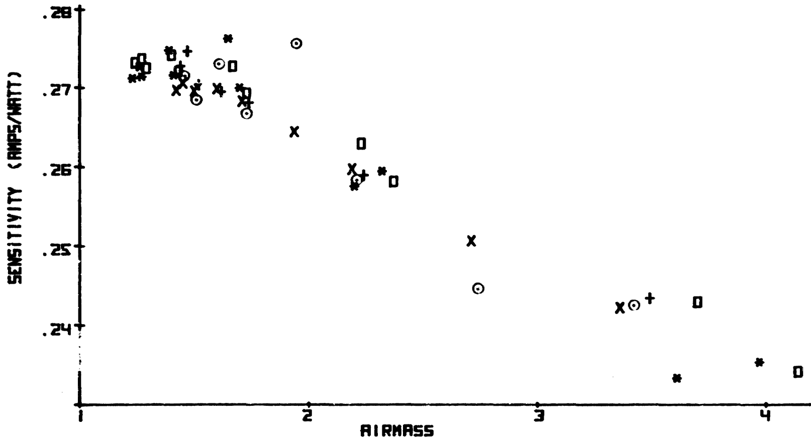
Figure 5. - Sensitivity versus air mass under clear sky (global - 0 tilt)
