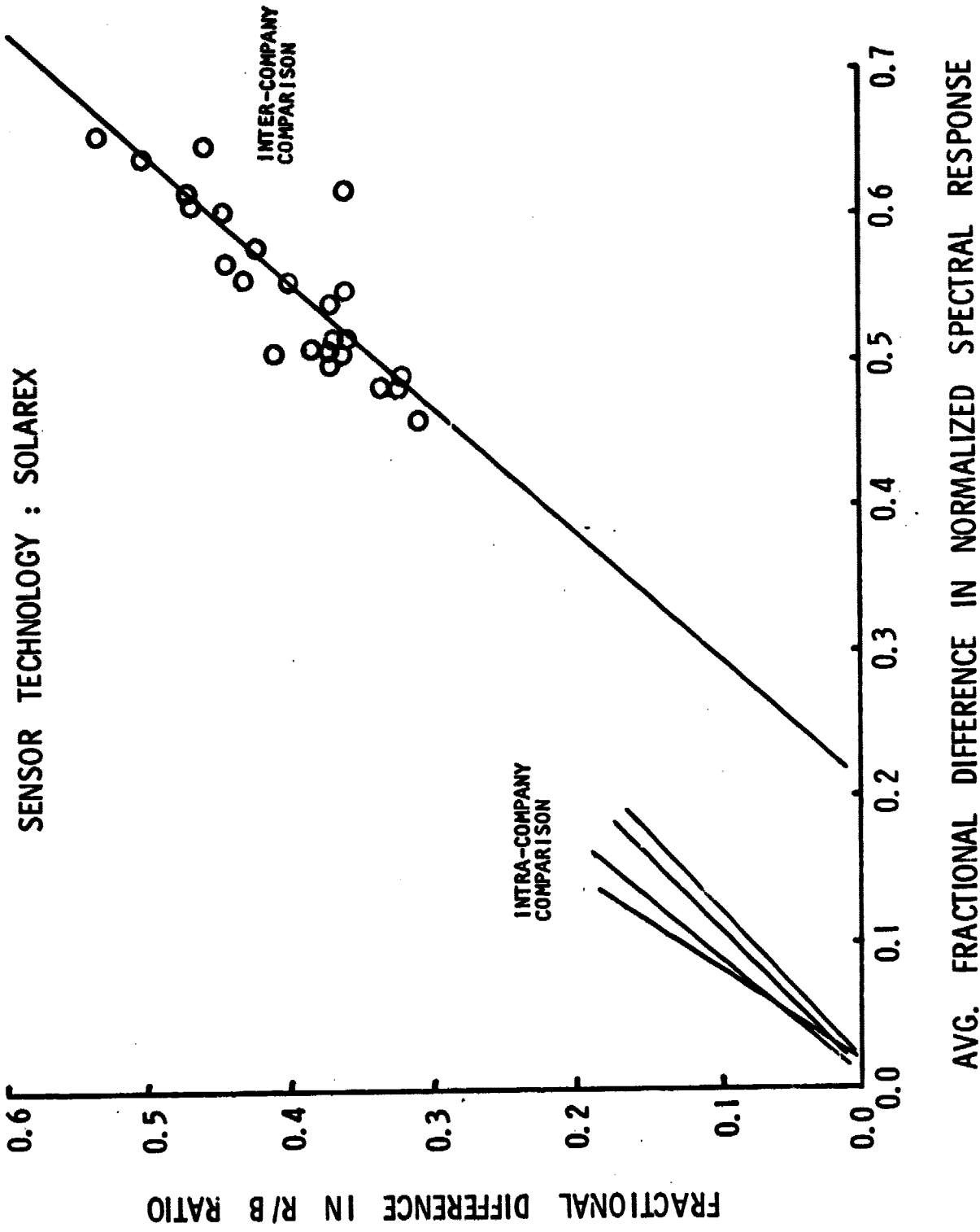
Figure 15. - Red/blue ratio, spectral response correlation for Sensor Technology cells compared with a Solarex reference
