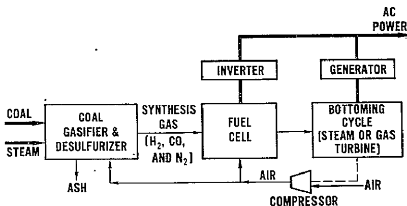
Figure 1 — System Concept
