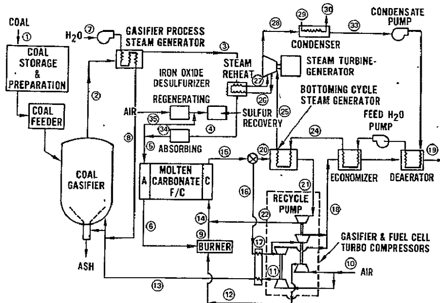
Figure 2 – Powerplant Flow Chart
