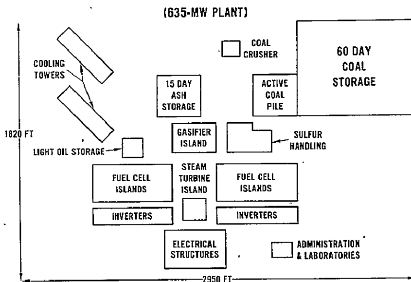
Figure 3 — Simplified Plant Layout
