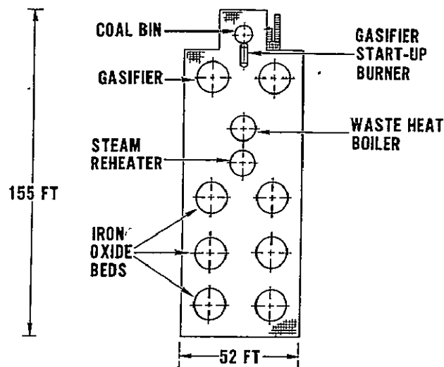
Figure 7 — Coal Gasifier Island Plan
