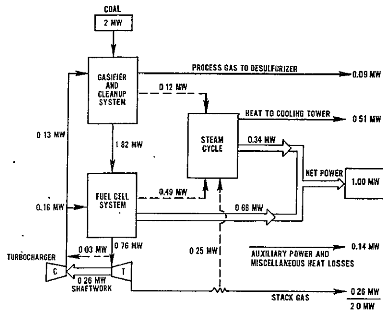
Figure 25 – Approximate System Energy Flow
