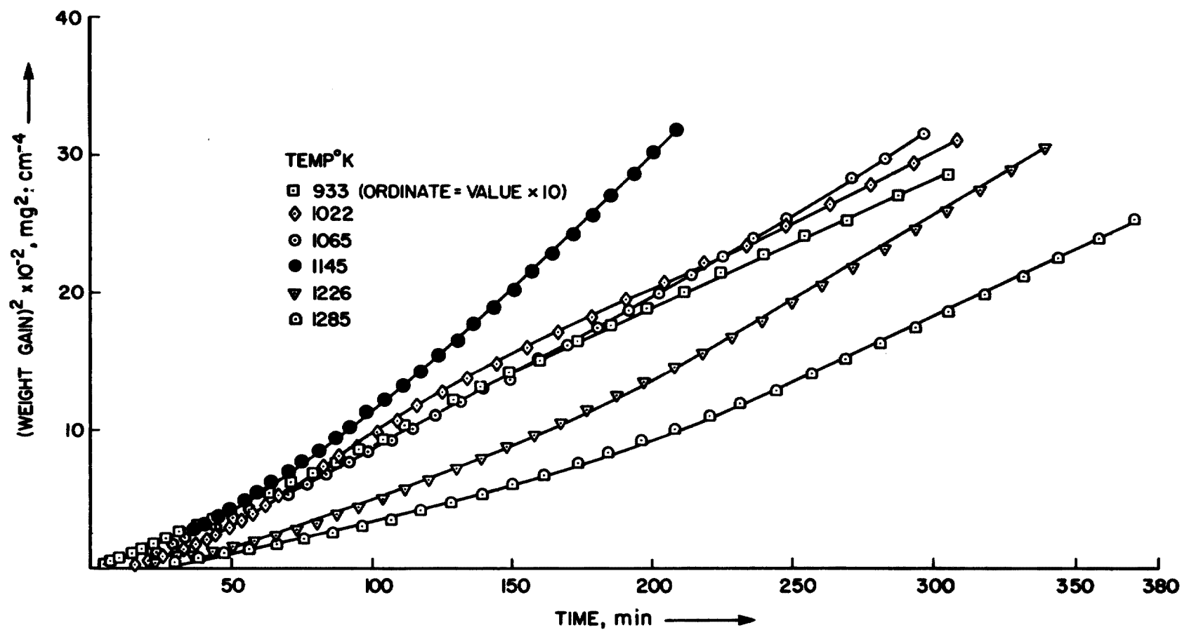
Fig. 2. Parabolic plots for the sulfidation of 310 stainless steel at a sulfur potential of 1.4 \times 10^{-2} Nm -2 . Filled circles indicate the formation of liquid in the OL-II.
