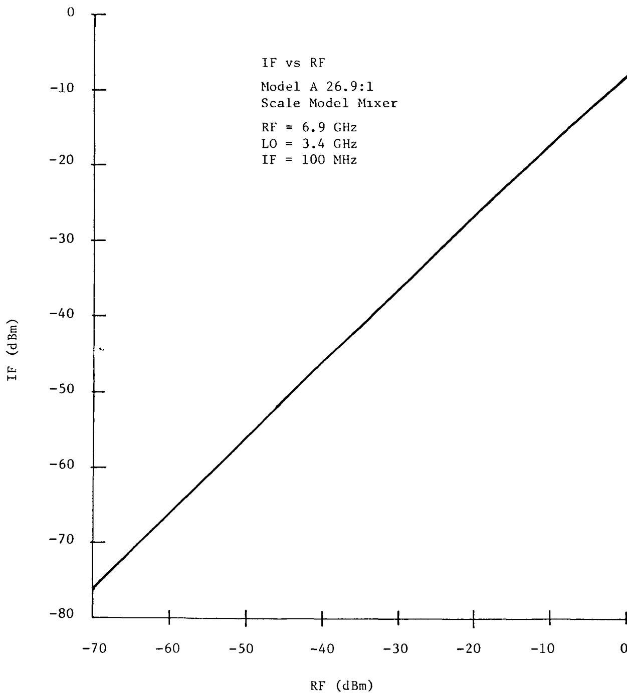
Figure 27. IF vs. RF (100MHz)
