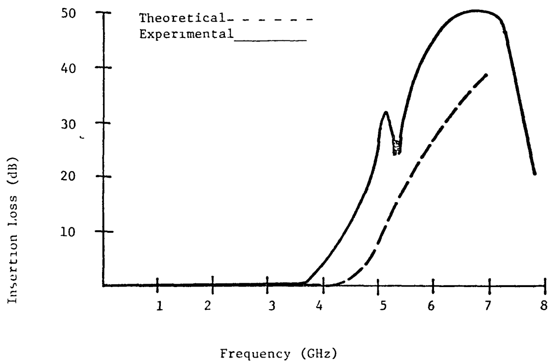
Figure 10. Measured Insertion Loss of the Scale Model L0 Filter (Linear dB Scale)
