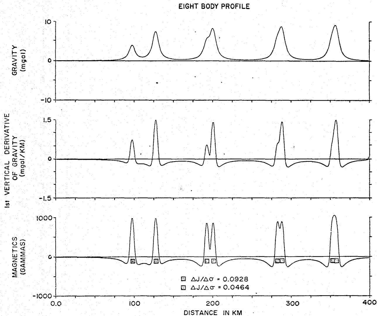
Figure 12. Eight body profile: gravity, first vertical derivative of gravity, and magnetic anomaly profiles due to four pairs of equivalent sources at decreasing distances of separation. Sampling interval is 1 km.
