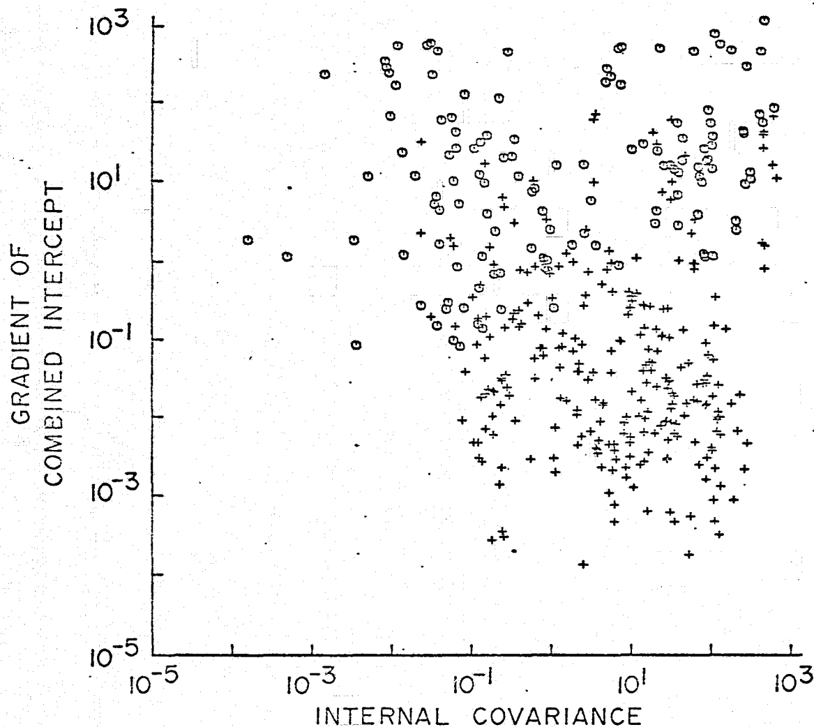
Figure 24. Log-log scatter diagram of the absolute values of internal covariance and gradient of combined intercept from mixed profile. Crosses represent window positions yielding \Delta J/\Delta \sigma estimates within 10% of known values. Zeros represent window positions yielding \Delta J/\Delta \sigma estimates that are outside of 10% range of known sources. Window size is 5 km.
