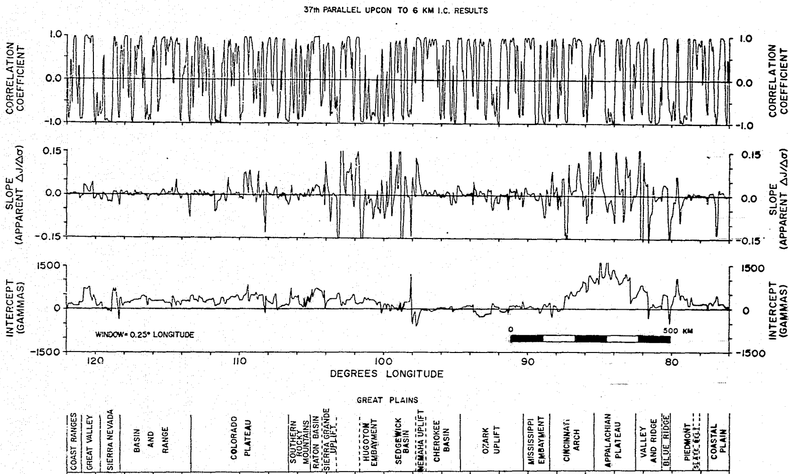
Figure 37. Internal correspondence results of 37th parallel anomaly data upward continued to 6 km.
