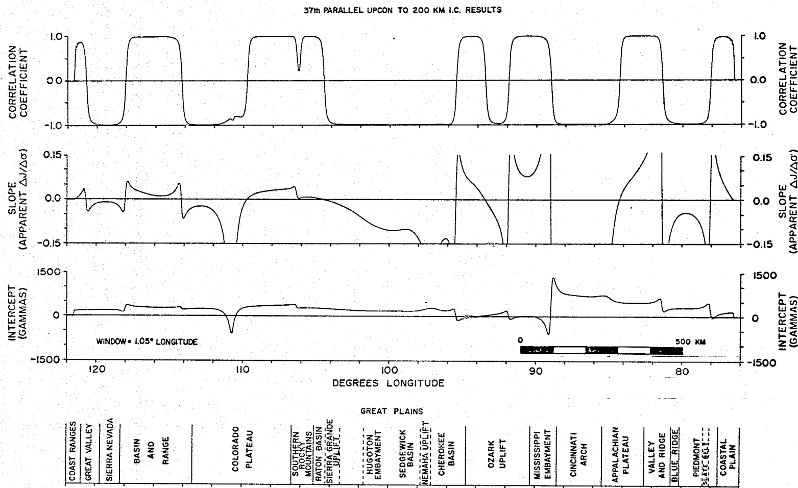
Figure 41. Internal correspondence results of 37th parallel of latitude anomaly data upward continued to 200 km.
