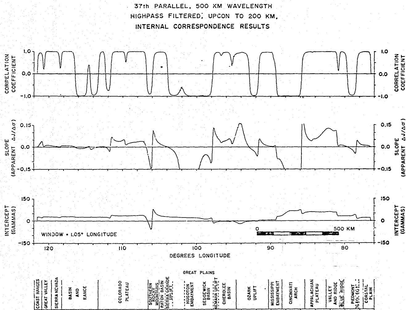
Figure 45. Internal correspondence results of 37th parallel of latitude anomaly data, 500 km highpass filtered and upward continued to 200 km.
