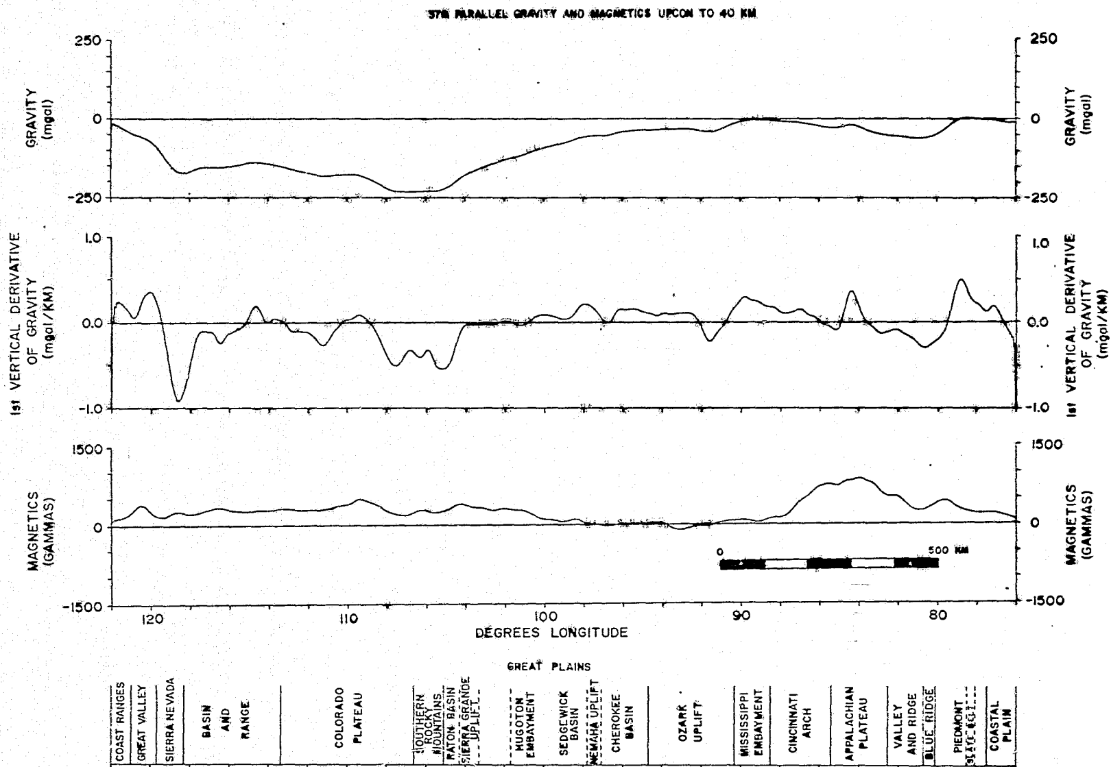
Figure 38. Transcontinental gravity, first vertical derivative of gravity, and reduced to pole magnetic anomaly profiles along the 37th parallel of latitude upward continued to 40 km.
