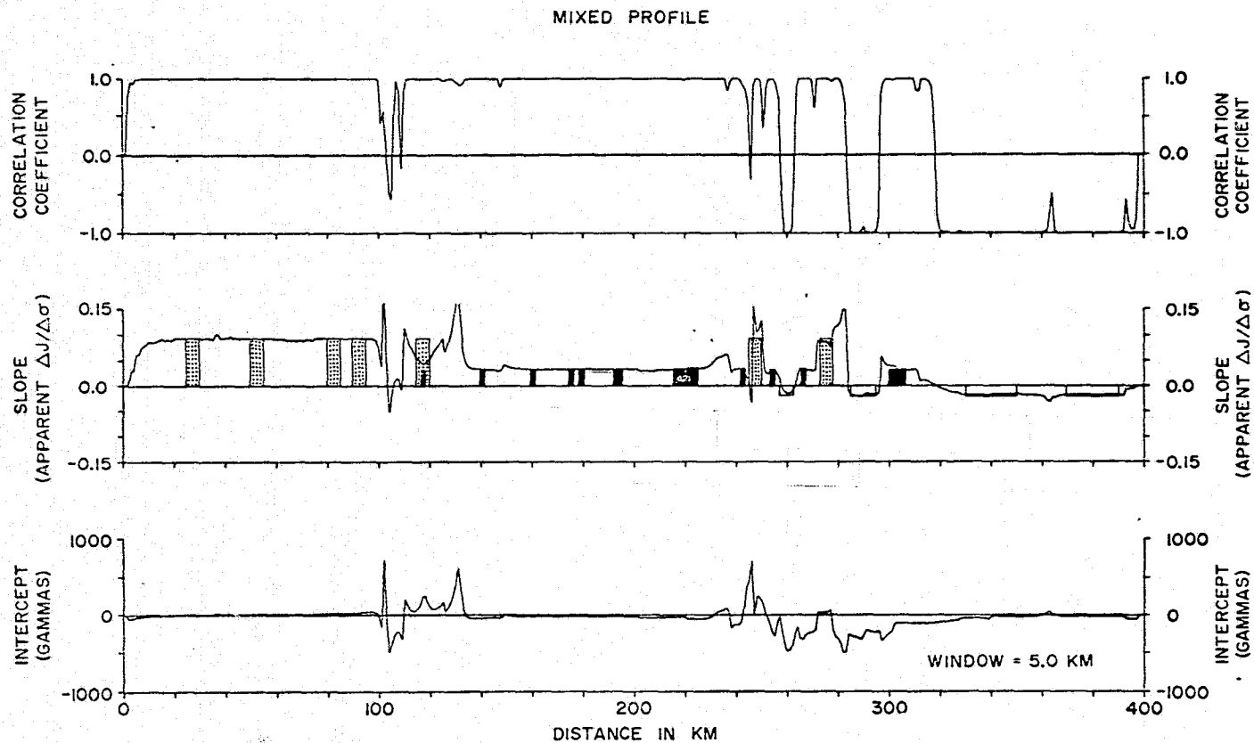
Figure 23. Mixed profile: internal correspondence results using a 5 km window. Position of shaded bars represent source positions and their levels represent actual source \Delta J/\Delta \sigma values.
