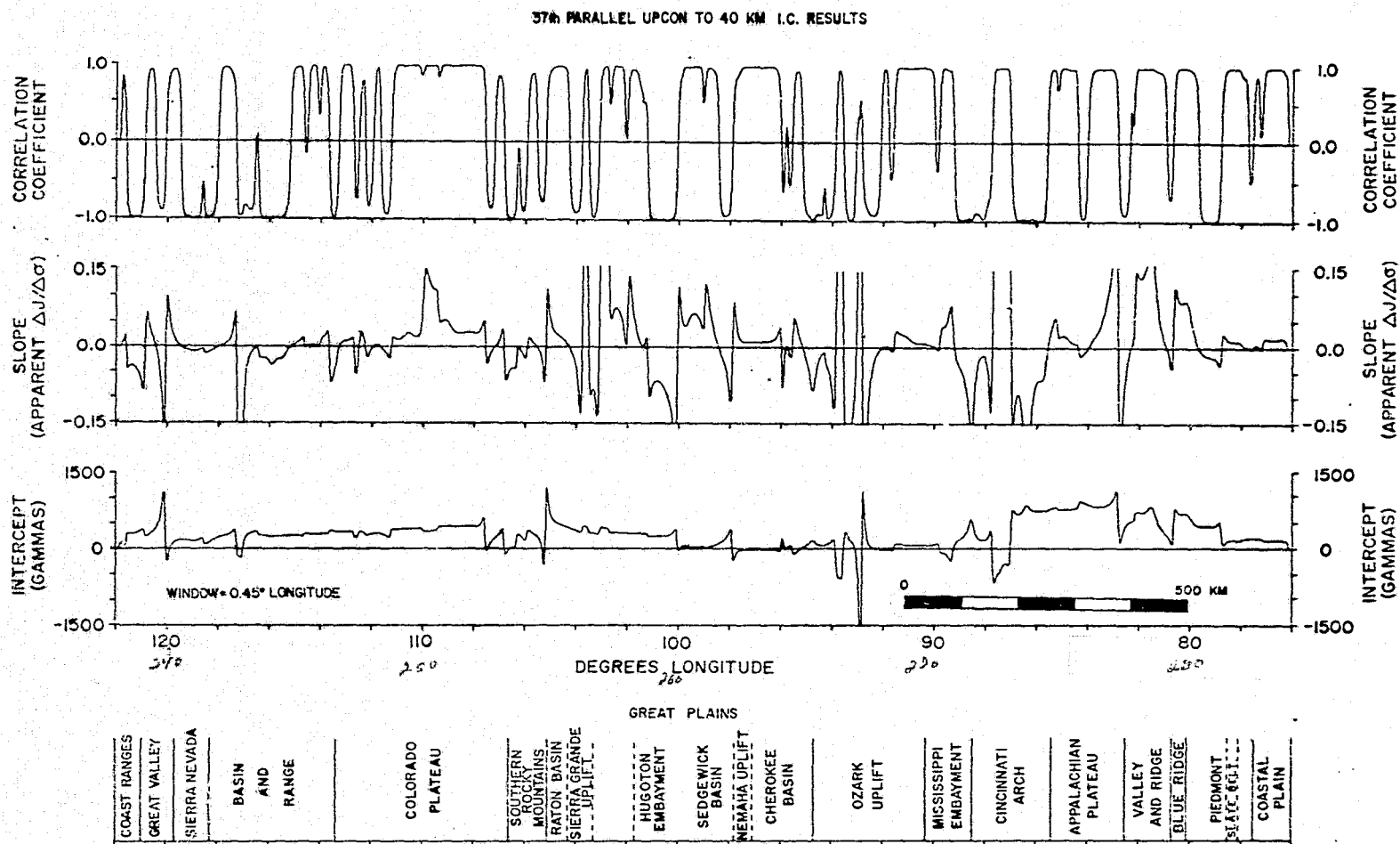
Figure 39. Internal correspondence results of 37th parallel of latitude anomaly data upward continued to 40 km.
