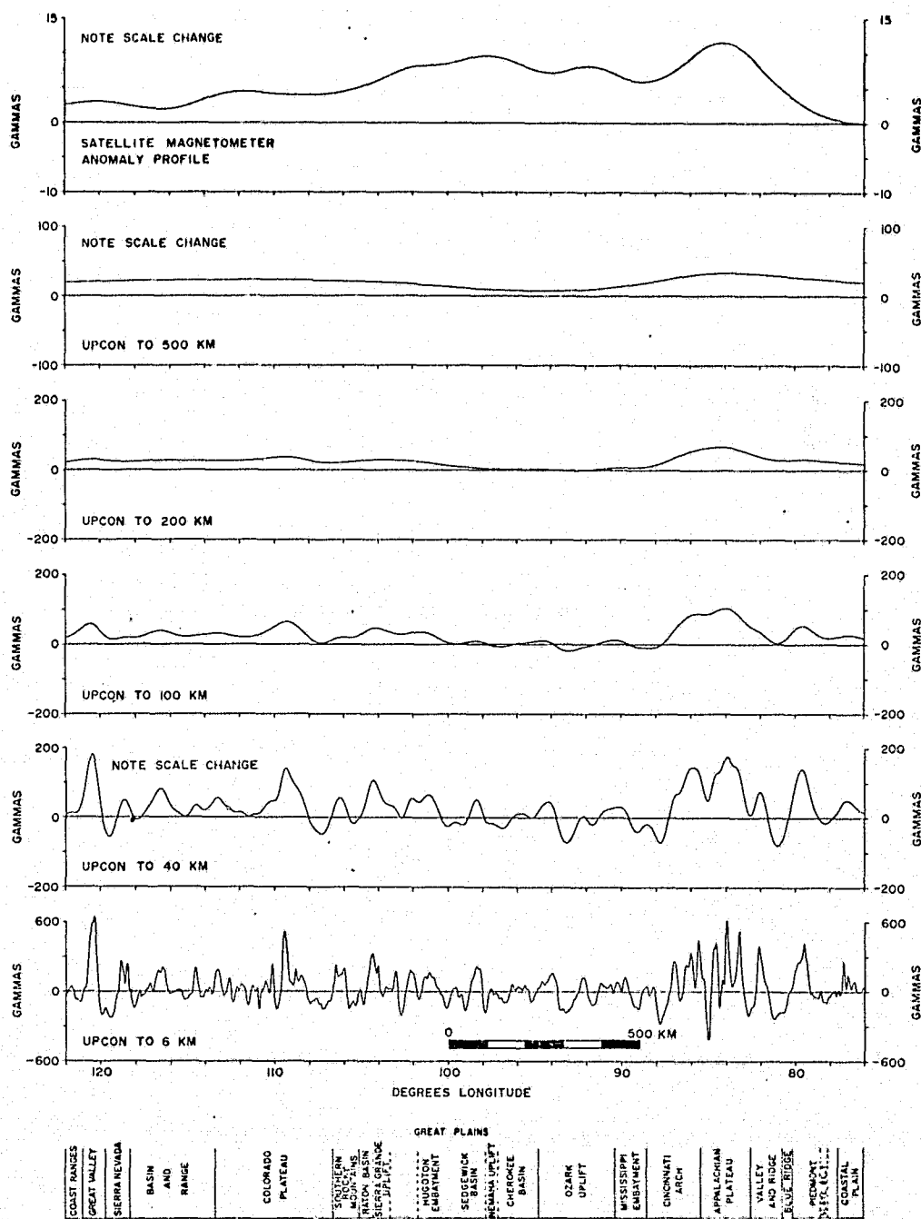
Figure 35. Aeromagnetic anomaly profiles, reduced to the pole and 500 km highpass filtered, and a satellite magnetic anomaly profile, along the 37th parallel across the continental United States. Aeromagnetic profiles are upward continued to 6, 40, 100, 200, and 500 km.
