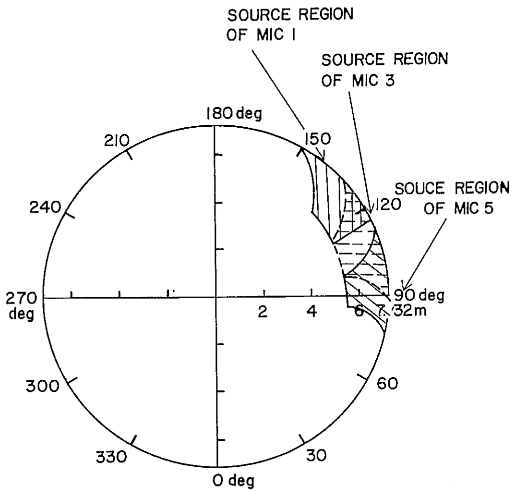
FIGURE 15.- SOURCE REGIONS OF THICKNESS NOISE
