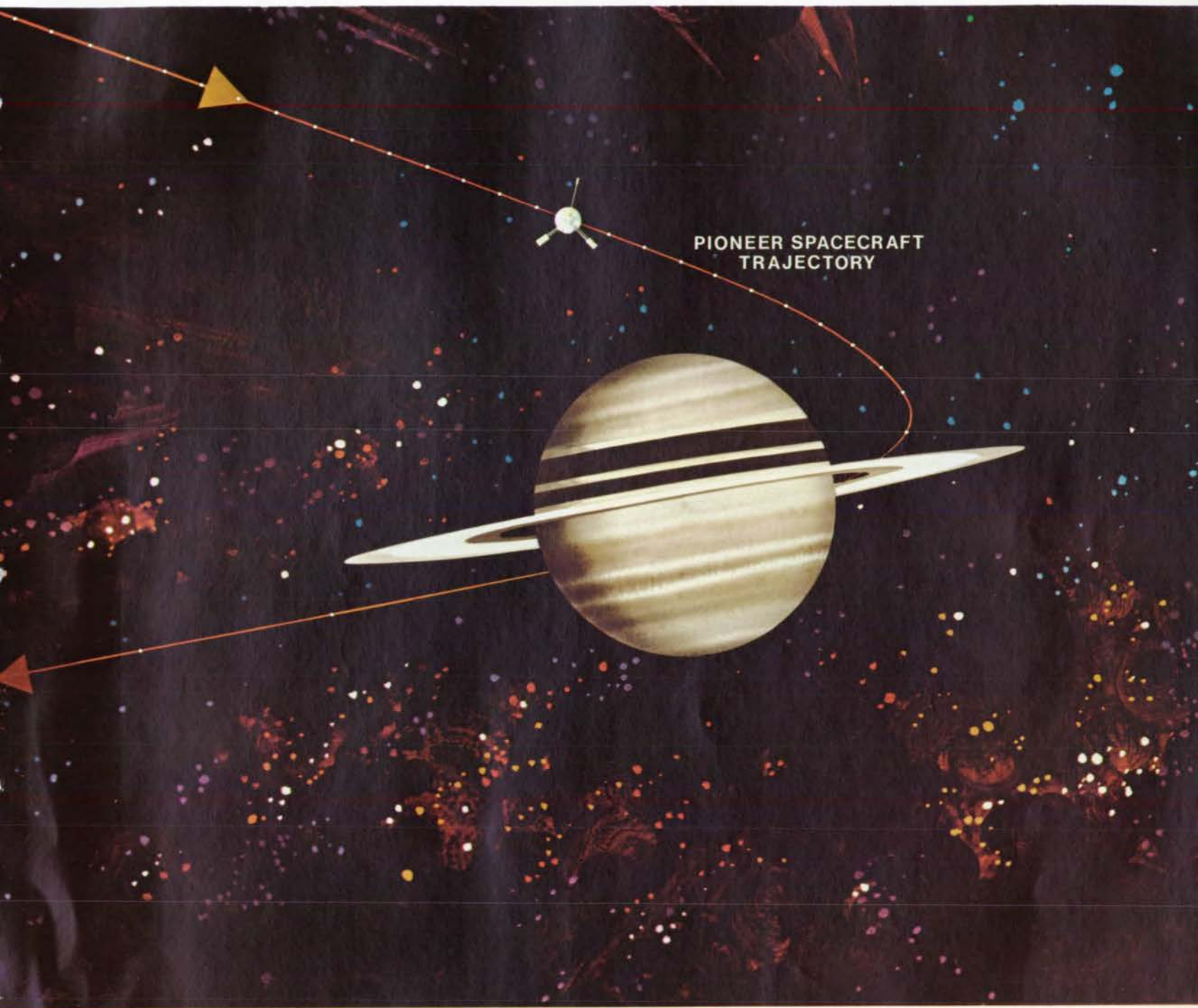
Figure 5-22. One of several options to fly by Saturn would carry the Pioneer spacecraft behind the rings as well as the planet and provide occultations to probe the rings and the planetary atmosphere with the radio signals from the spacecraft to Earth. The marks on the trajectory signify periods of one hour. The trajectory after encounter carries the spacecraft alongside Titan for an inspection of that large satellite.
