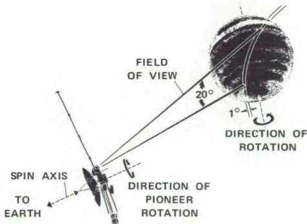
Figure 4-10. Ultraviolet light is sensed by this ultraviolet photometer to determine the quantities of hydrogen and helium in space and on Jupiter. (a) Is a photograph and (b) a diagram of the instrument. (c) Shows how it scans Jupiter.
