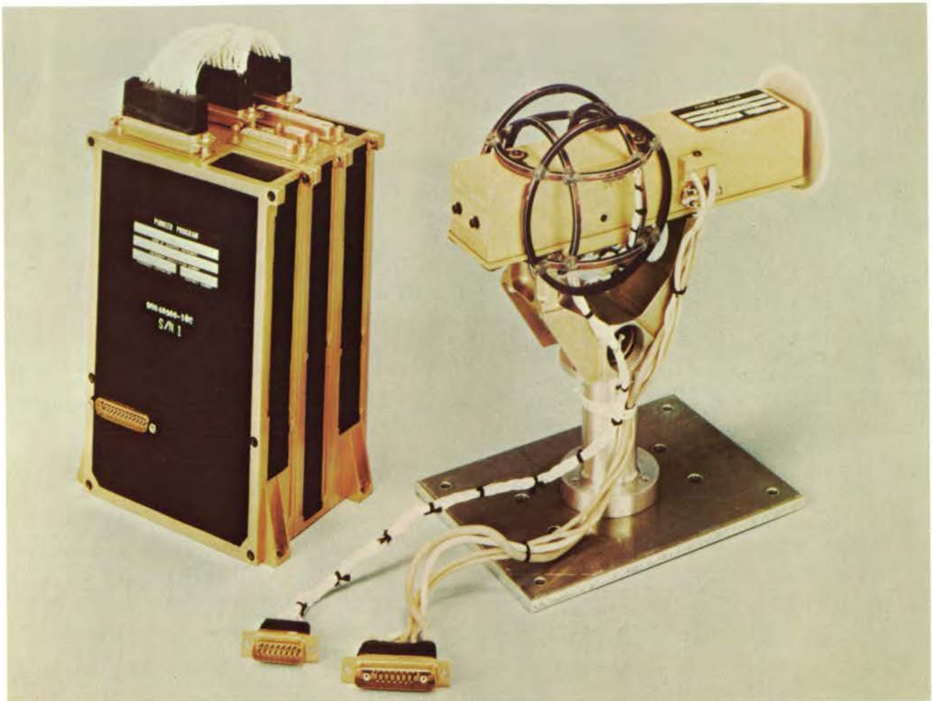
Figure 4-2. The magnetometer, mounted on a long boom to keep it far away from the RTGs measures magnetic fields in space and in the vicinity of Jupiter. The electronics at the left of the magnetometer are mounted in the spacecraft.
