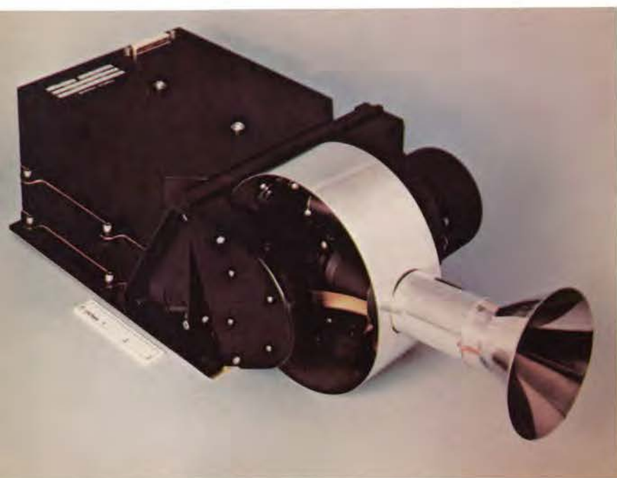
Figure 4-14. A special instrument observed the faint flows in interplanetary space of the Zodiacal Light, the Gegenschein, and the integrated starlight. At Jupiter this same instrument was used to look at the reflective properties of the Jovian atmosphere and of satellites and to build up spin-scan images of these bodies.
