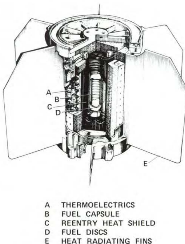
Figure 3-4. Electrical power is developed in Pioneer by several radioisotope thermoelectric generators (RTG).
