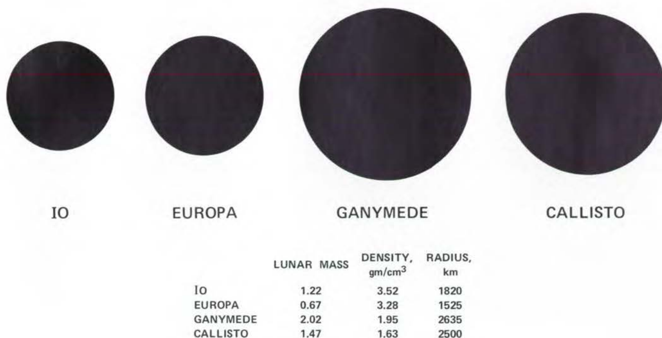
Figure 6-4. Pioneer 10 provided specific information on the physical characteristics of the Jovian satellites.
