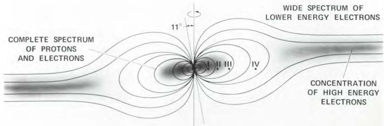
Figure 6-9. Radiation belts consist of particles trapped in Jupiter's magnetic field, and the satellites sweep up many of the charged particles.
