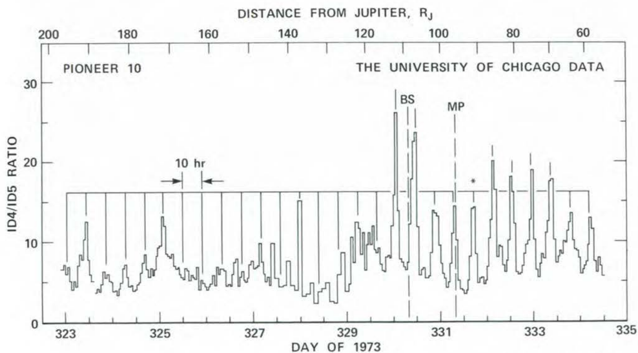
Figure 6-12. Both inside and outside of Jupiter's magnetosphere, the 10-hour modulation of electron intensity appears to be in phase. BS is the bow shock. MP is the magnetopause.
