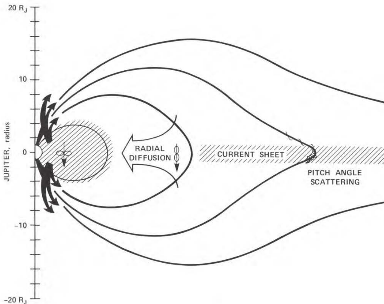
Figure 6-13. Energetic particles appear to be circulating in the magnetosphere and ejected at high latitudes.
