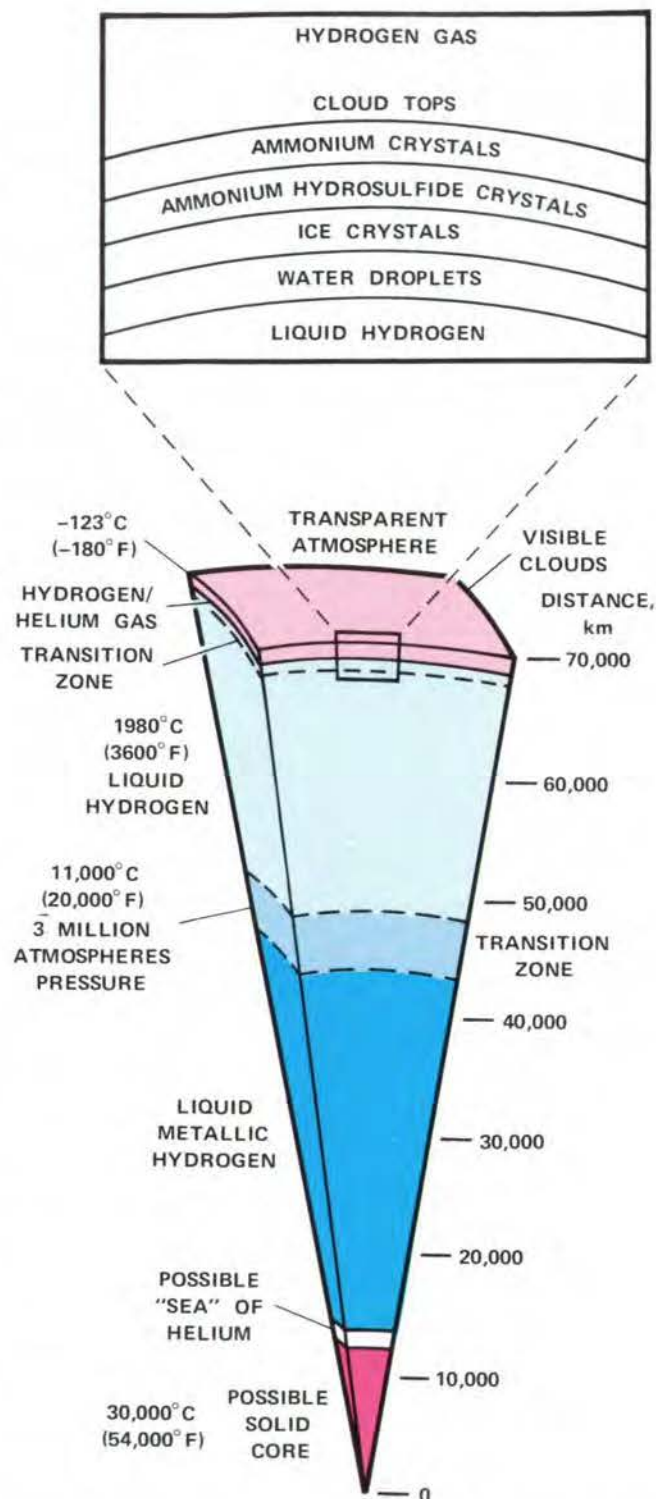
Figure 6-14. Pioneer 10 confirms models of Jupiter that suggest the planet is nearly all liquid with a very small core and a deep atmosphere.
