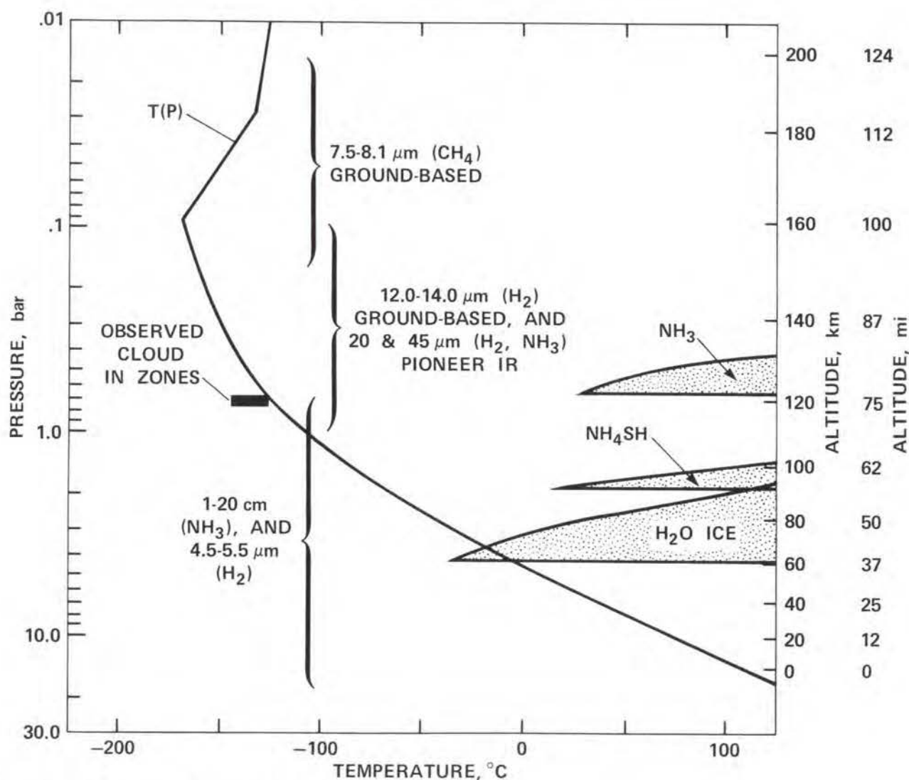
Figure 6-15. The temperature profile in the atmosphere of Jupiter and the location of various cloud layers are shown in this diagram from data of A. Ingersoll, Caltech.
