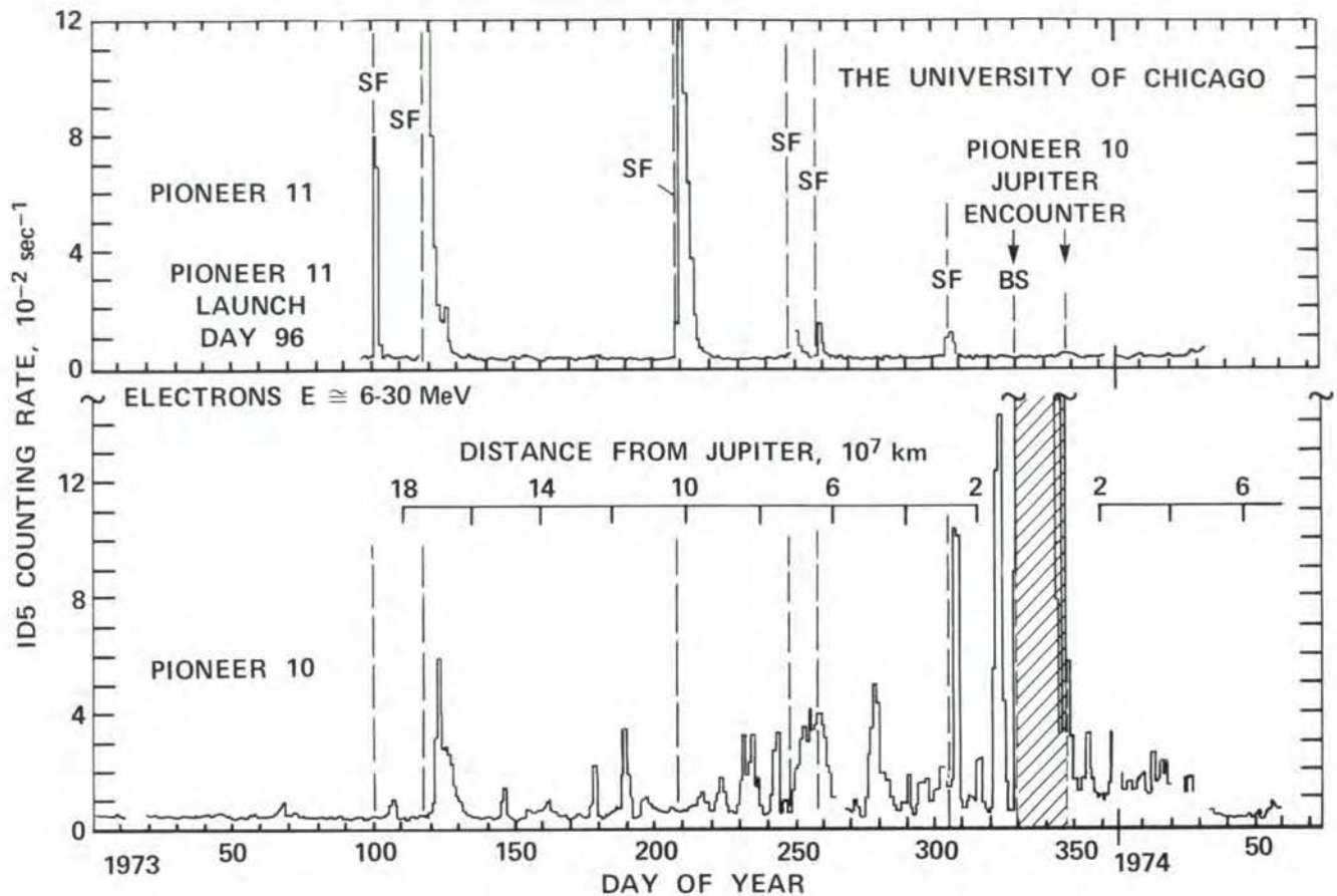
Figure 6-10. Comparisons of the number of energetic electron events observed by Pioneer 10 and Pioneer 11 during the encounter of Pioneer 10.
