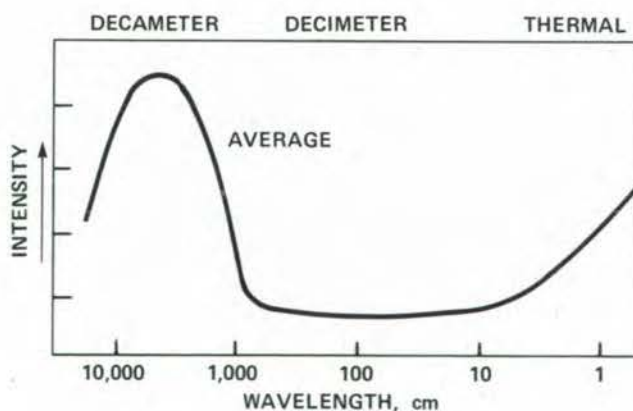
Figure 1-14. Jupiter emits radio waves which have been recorded and measured by radio astronomers for several decades. They are of three main types: thermal, decimetric and decametric. Each has a different origin.
