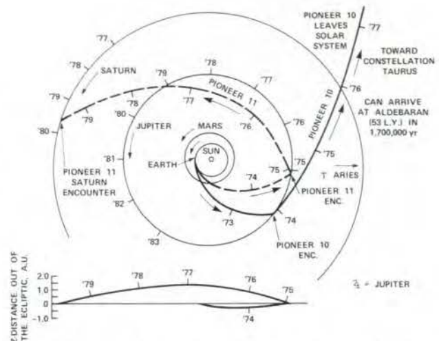
Figure 5-16. Pioneer 10 and 11 heliocentric trajectories. The time ticks shown along the trajectories and planetary orbits represent the distance traveled during each year.
