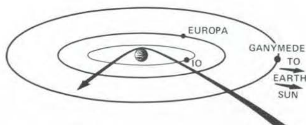
Figure 2-4. The first encounter trajectory with Jupiter was chosen to probe into the radiation belts and ensure that the spacecraft would have opportunities to obtain images of the terminator, the Great Red Spot, and several satellites, and would go into occultation behind Io as seen from Earth.
