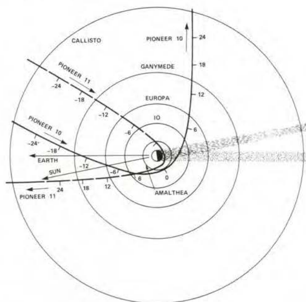
Figure 5-18. Pioneer 10 and 11 encounters with Jupiter as viewed from the celestial North Pole. Pioneer 10 swings around the giant in the counterclockwise direction, but Pioneer 11 attacks the planet in a clockwise course. Jupiter rotates counterclockwise in this view. The time in hours before and after closest approach is given by the numbers alongside each trajectory.
