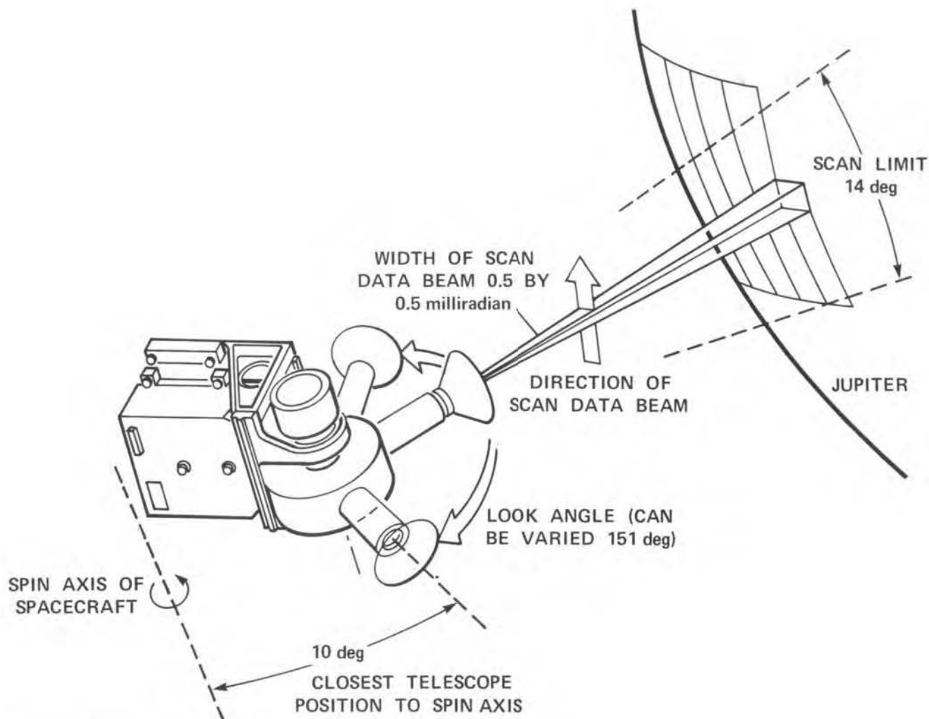
Figure 7-2. Diagram of the imaging photopolarimeter system.
