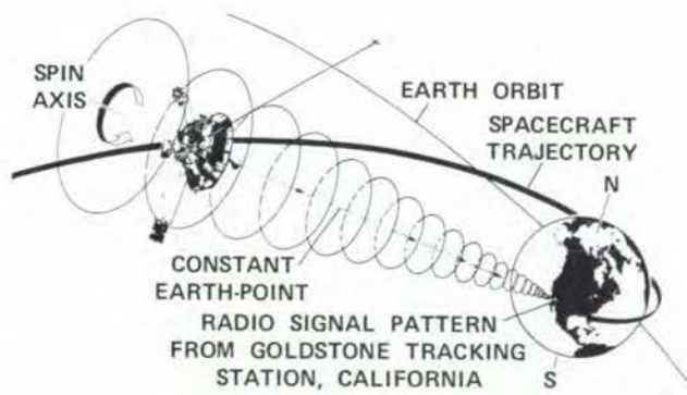
Figure 3-6. An automatic system in the spacecraft, known as CONSCAN, is used to help keep the spin axis of Pioneer pointing toward Earth. It relies upon a slight offset in the antenna feed axis to produce a wobbling signal at Earth when the antenna is not pointing exactly Earthwards. Controllers direct the spacecraft so that its antenna drifts past the optimum point and thereby they conserve thruster propellant. With more expenditure of propellant, CONSCAN could point the spacecraft's axis automatically.
