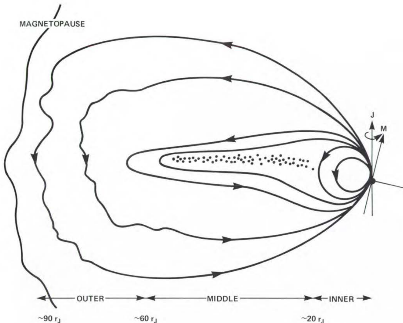
Figure 6-8. Jupiter's magnetosphere is differently shaped from that of Earth and has three distinct regions.
