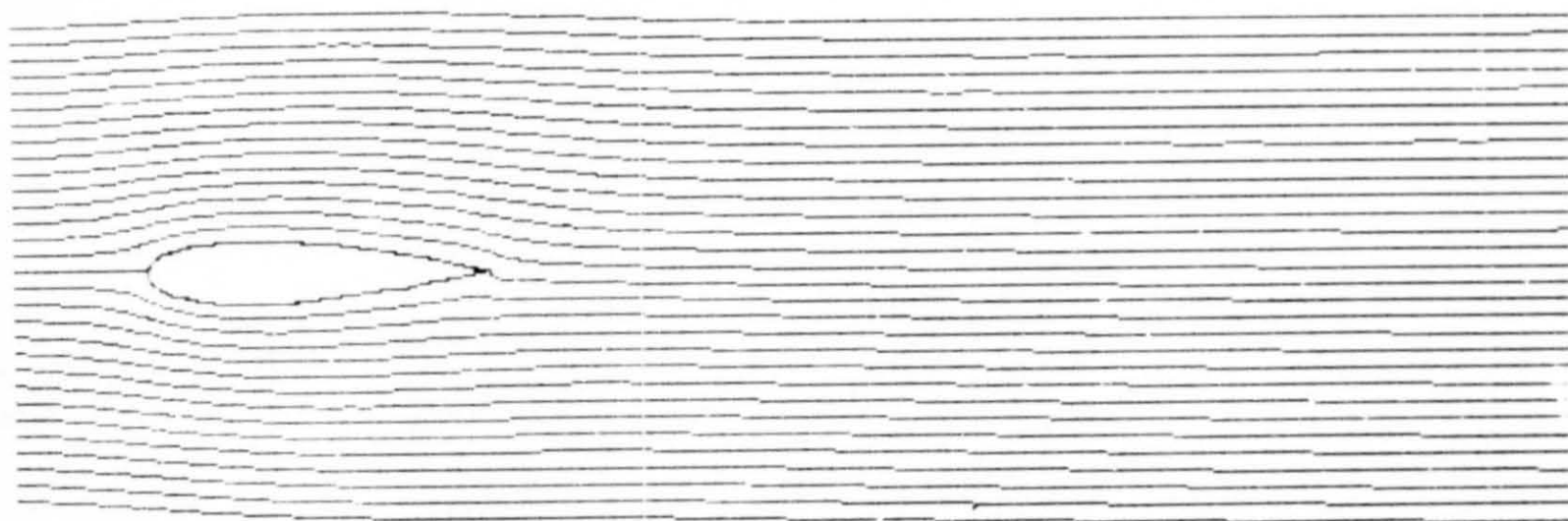
Figure 10. Streamlines ( t = 1.1 )
