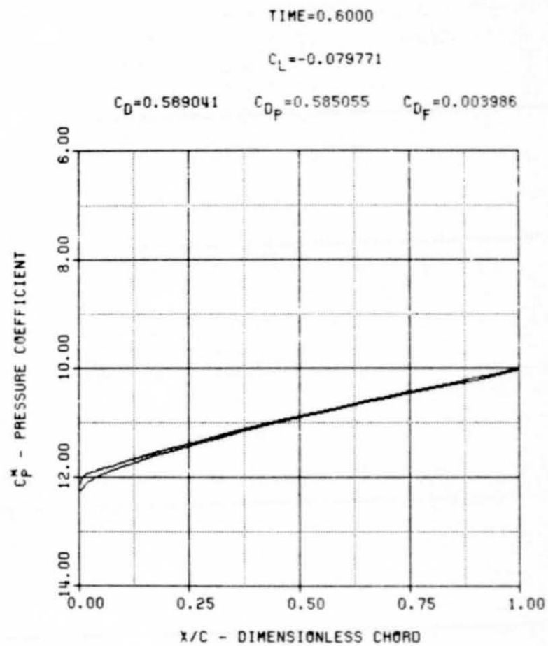
Figure 13. Pressure Distribution
