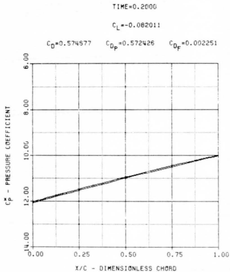
Figure 13. Pressure Distribution
