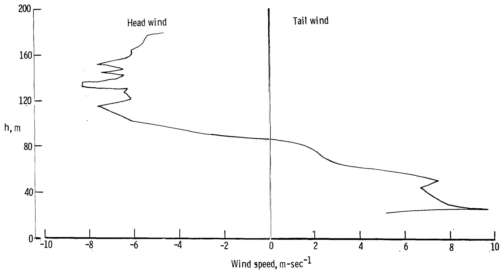
Figure 1.- Variation of wind speed with altitude for a strong wind shear. Head winds are negative.
