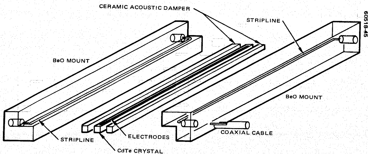
FIGURE 5-39. EXPLODED VIEW OF STRIPLINE TRANSMISSION LINE MODULATOR ASSEMBLY
