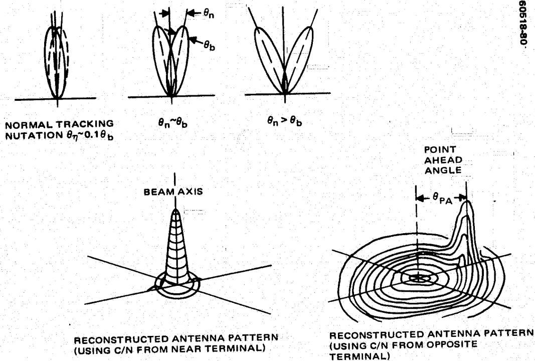
FIGURE 7-2. BEAM PROFILE MEASUREMENT EXPERIMENT
