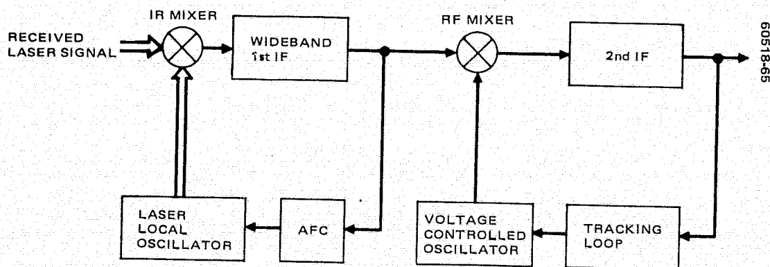
FIGURE 5-58. DOUBLE CONVERSION CO 2 LASER HETERODYNE RECEIVER
