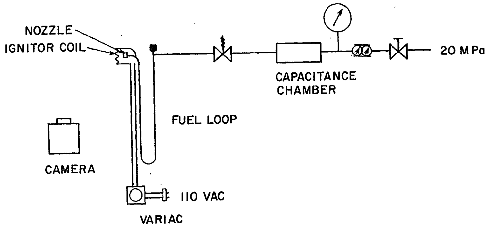
Figure 7 Sketch of the Low Pressure Apparatus
