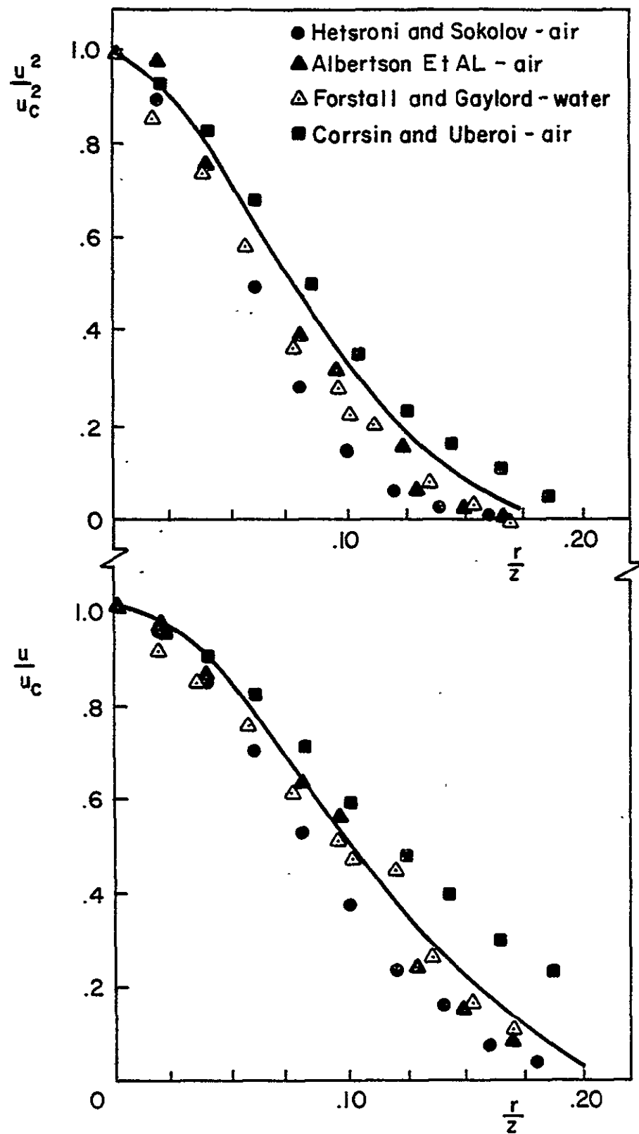
Figure 13 Correlation of Jet Velocity Spreading Characteristics
