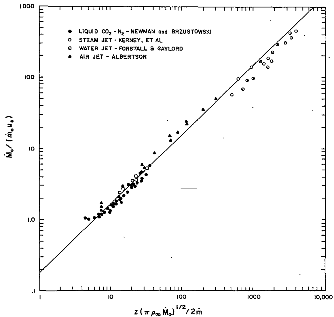
Figure 22 Correlation of Centerline Velocity Distribution for the \text{CO}_2 - \text{N}_2 System
