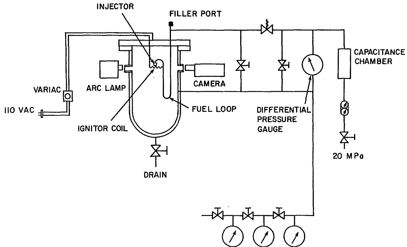
Figure 4 Sketch of the High Pressure Apparatus
