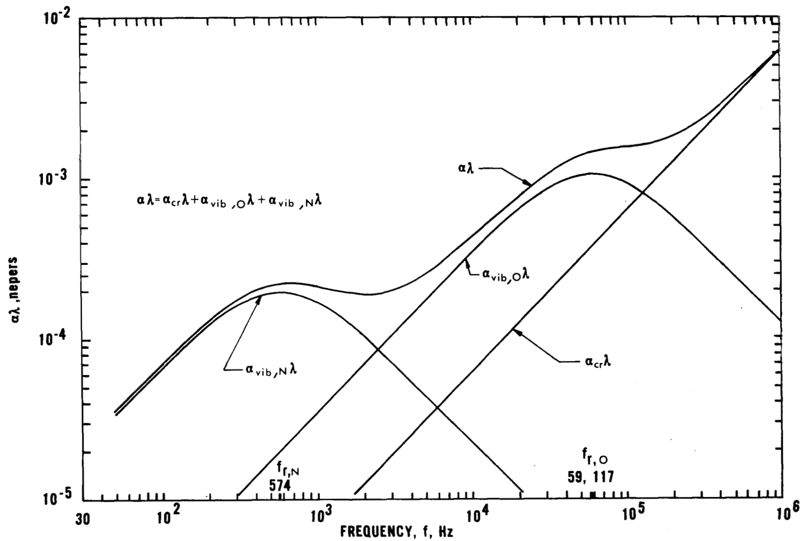
Figure 3.1 Absorption Components as a Function of Frequency, T = 293.15^\circ\text{K} , h = 1.6145\% , P = 1 atm.
