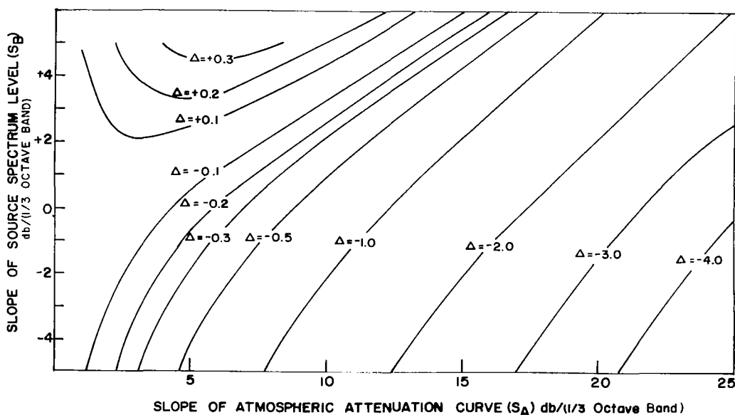
Figure 6.7 Curves of Constant Correction Factor ( \Delta in db) for a Perfect One Third Octave Band Filter in Terms of Source Spectrum Slope ( S_B ).
