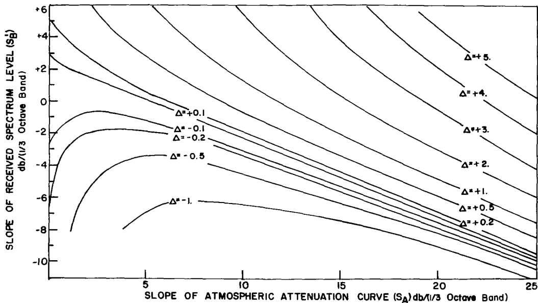
Figure 6.8 Curves of Constant Correction ( \Delta in db) for an ANSI Class III One Third Octave Band Filter in Terms of the Received Spectrum Slope, S_B'
