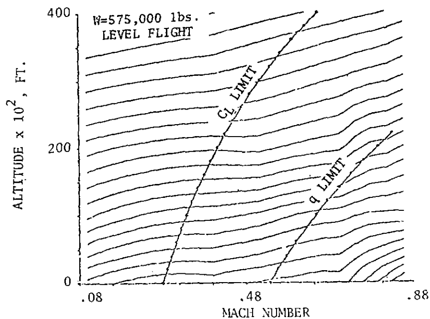
FIGURE 26. FUEL FLOW RATE MAP (COMPUTER DRAWN)
