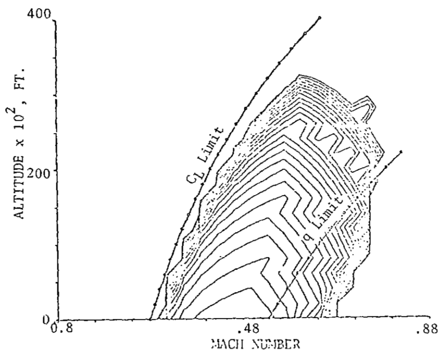
FIGURE 29. RADIUS OF TURN MAP (COMPUTER DRAWN)
