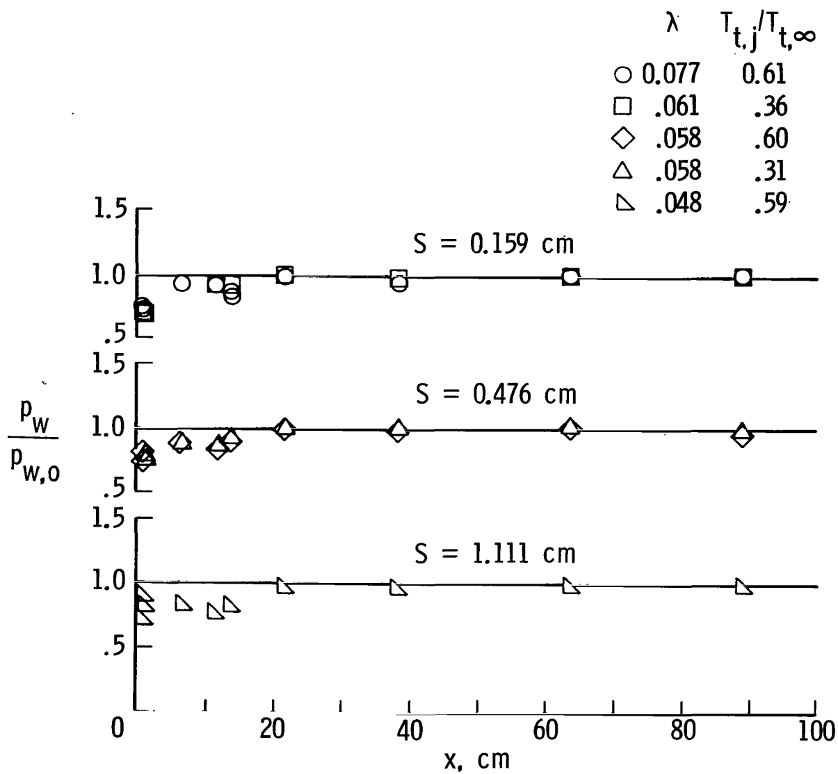
(d) Pressure distribution downstream of \Lambda = 45^\circ slot.
