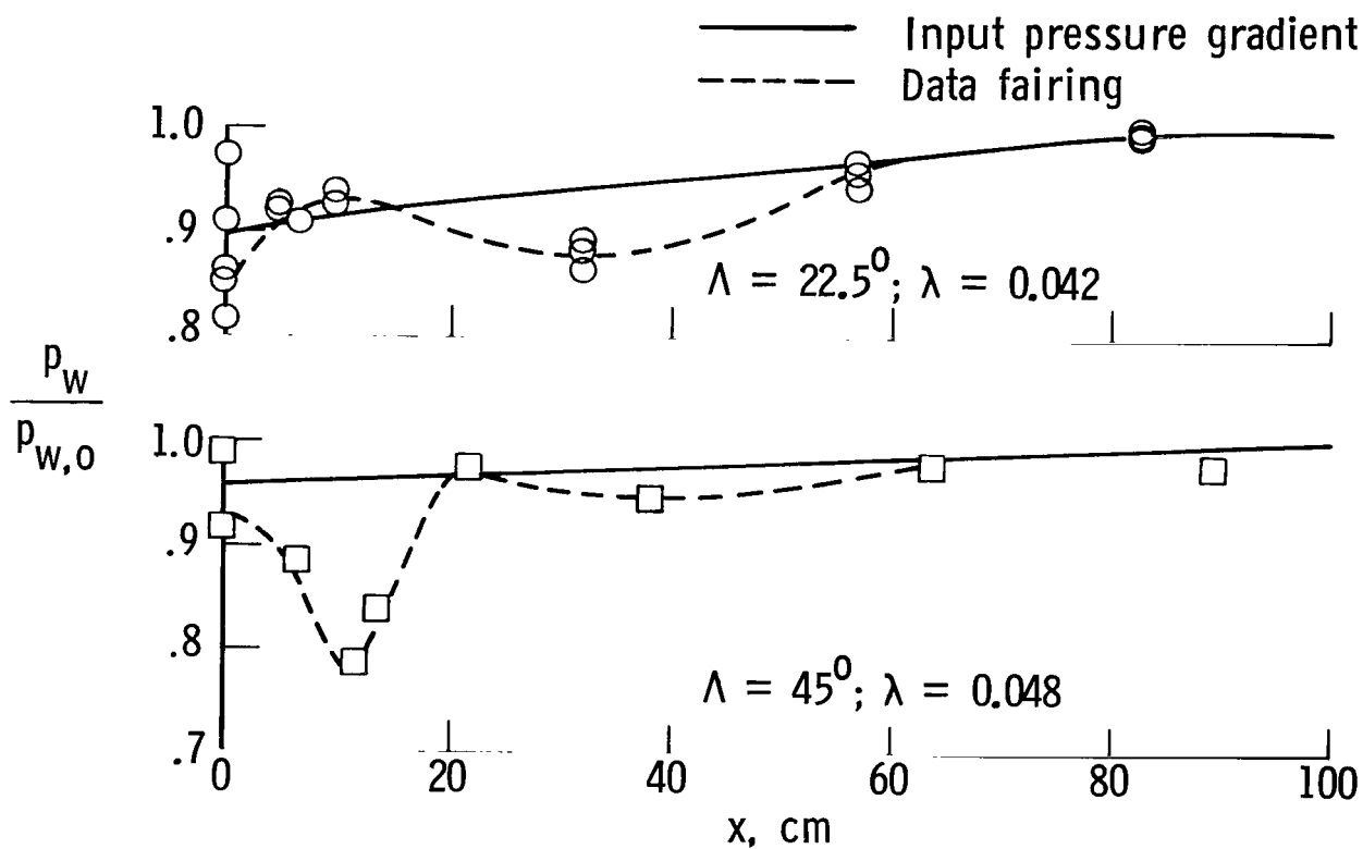
Figure 10.- Input pressure gradients for finite-difference program. T_{t,j}/T_{t,\infty} = 0.6 ; S = 1.111 cm.
