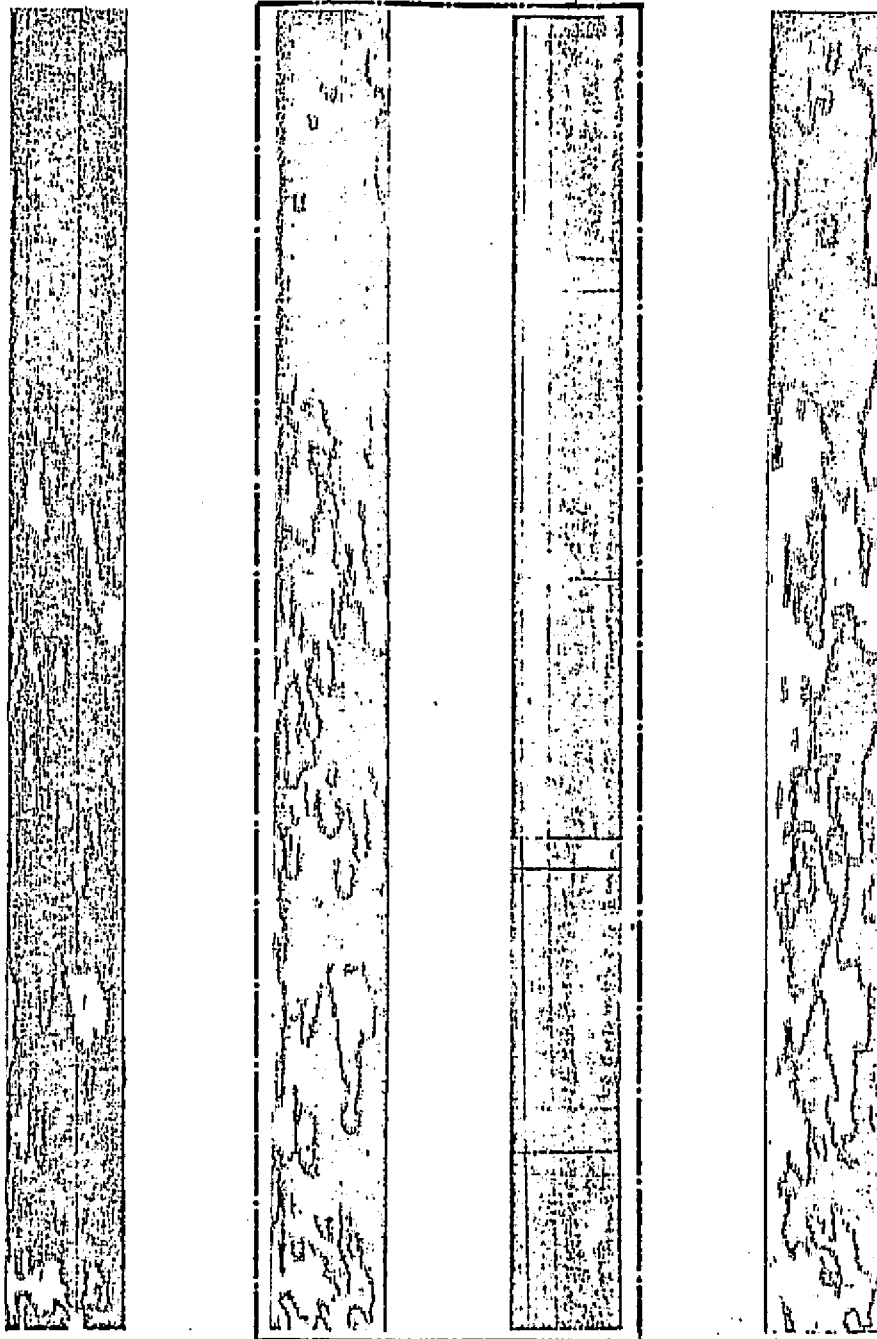
Fig. 5-15. C-scan of a defective laminate 4.6 mm thick for different threshold value settings (25%, 32.5%, 50%) in comparison with an x-ray photograph.
