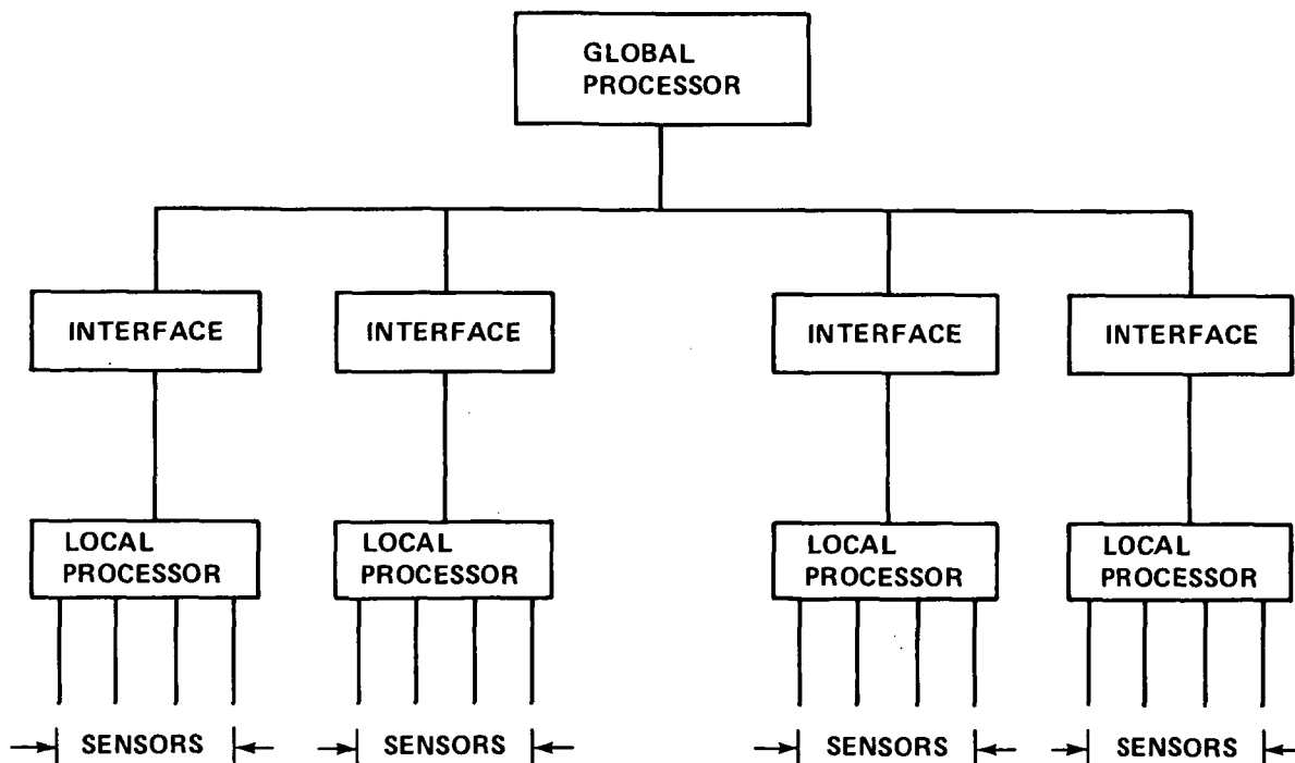
Figure 3. Multiprocessor system.
