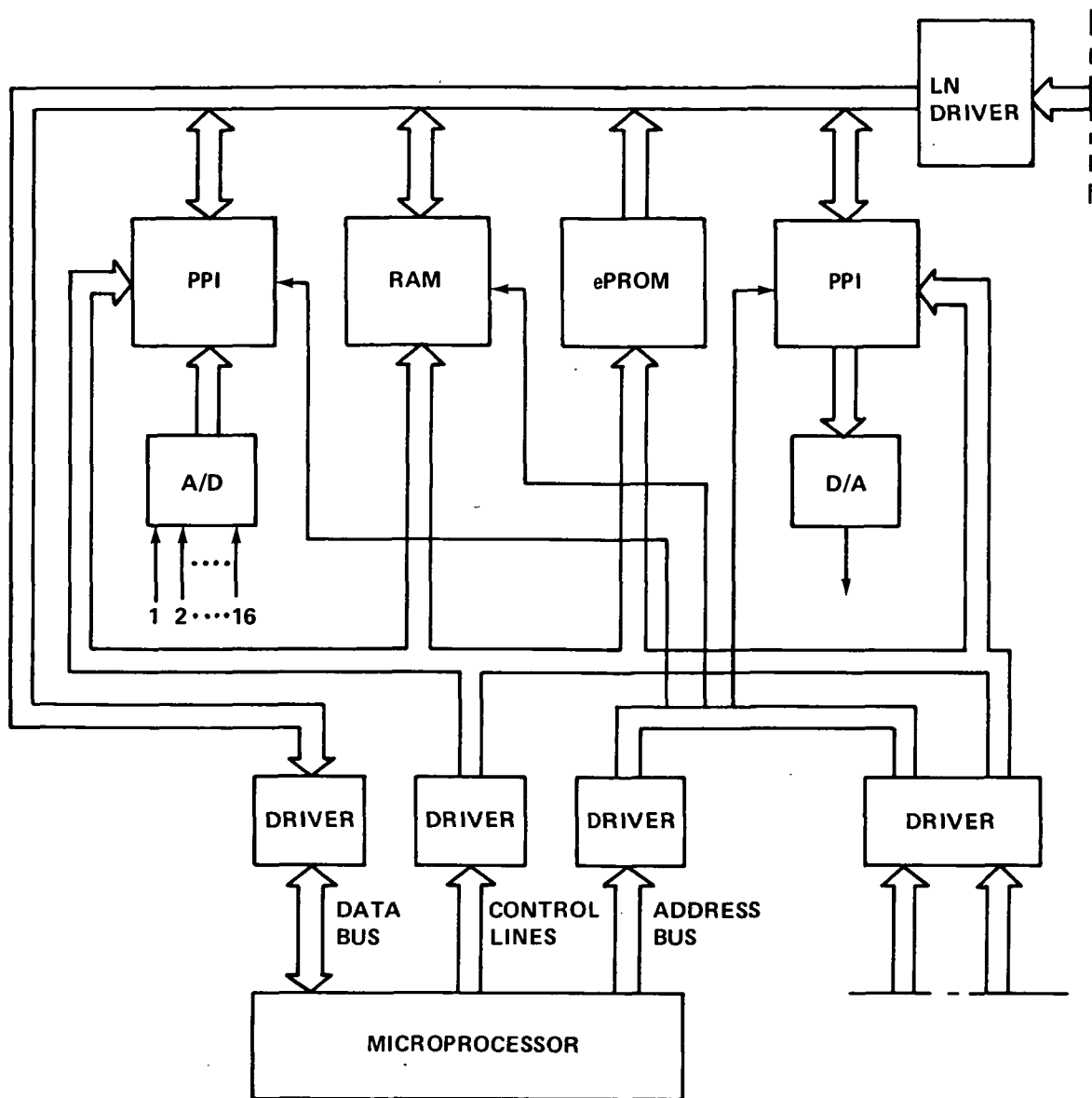
Figure 5. C/I subsystem.
