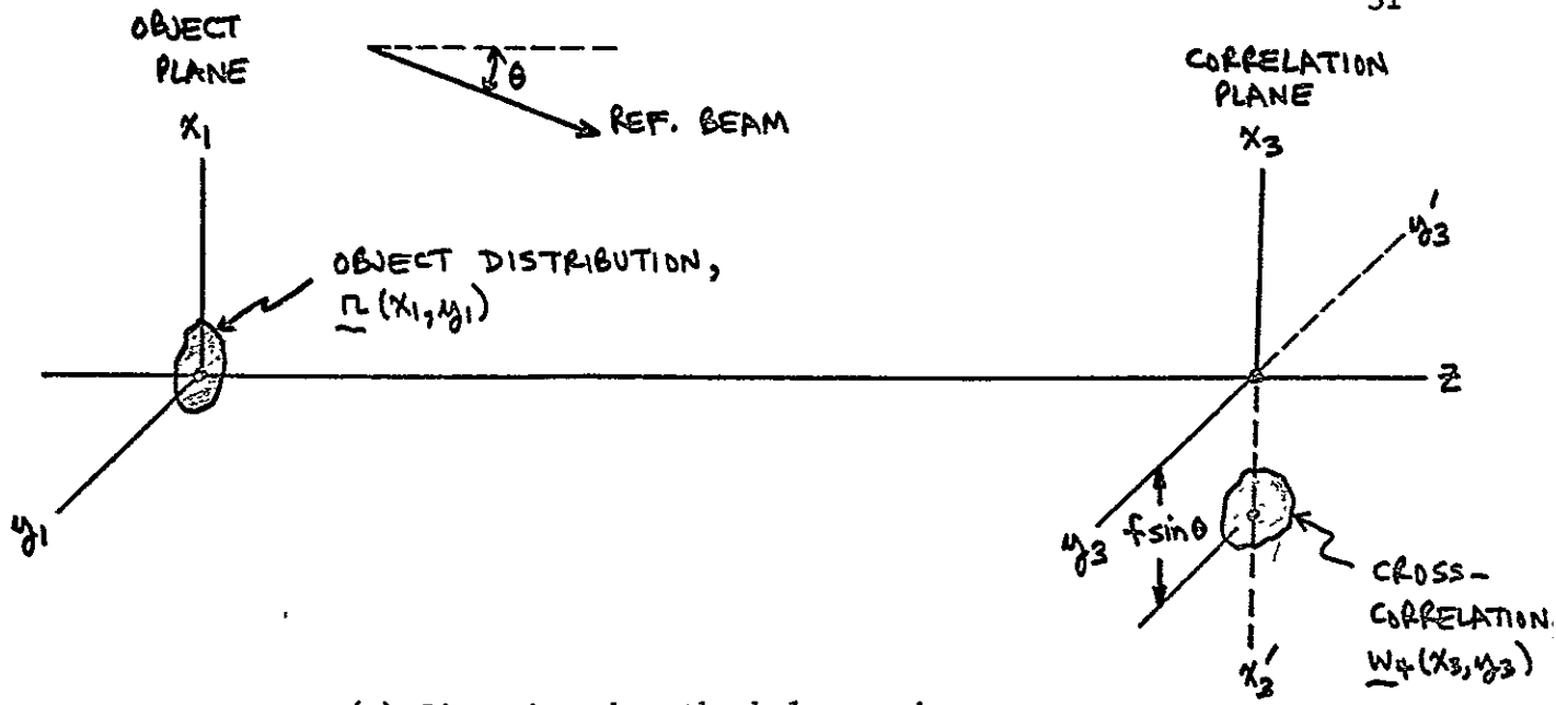
(a) Situation when the hologram is illuminated with the object distribution \underline{r}(x_1, y_1) .
