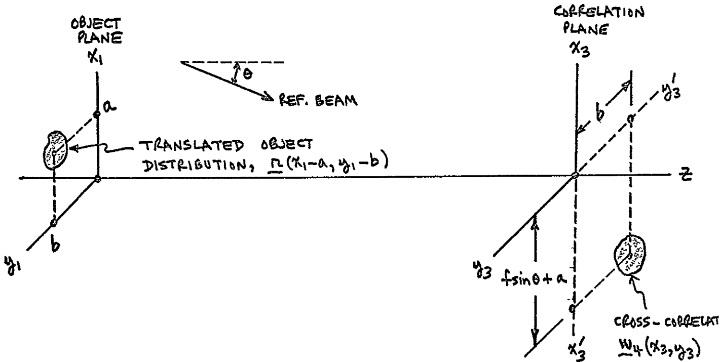
(b) Situation when the hologram is illuminated with the translated object distribution \underline{r}(x_1 - a, y_1 - b) .
