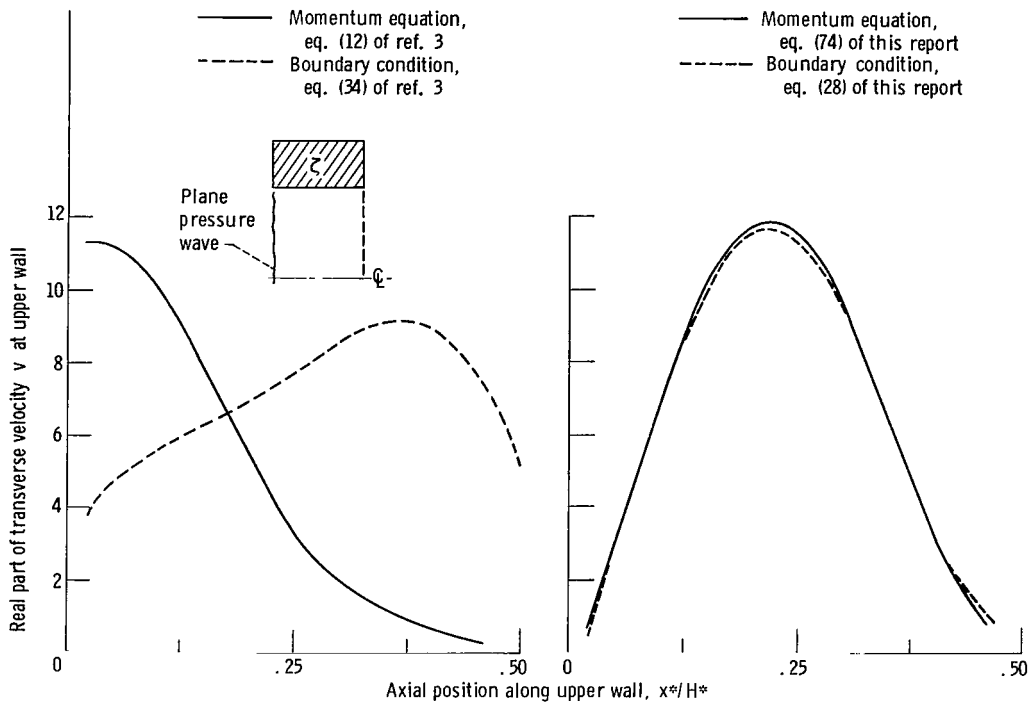
(a) Exit condition of reference 3. Sound attenuation, \Delta dB, 6.1 decibels.
